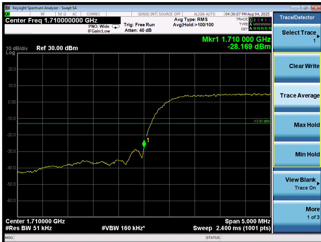
Band edge\B4\L
