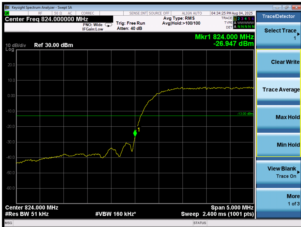
Band edge\B5\L
