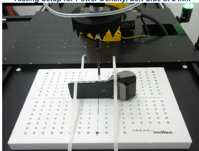
Testing Setup for Power Density, Left Side at 2 mm
