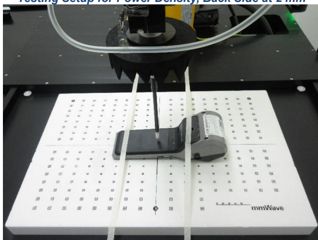
Testing Setup for Power Density, Back Side at 2 mm
