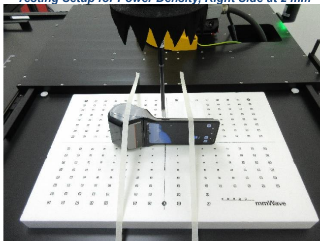
Testing Setup for Power Density, Right Side at 2 mm
