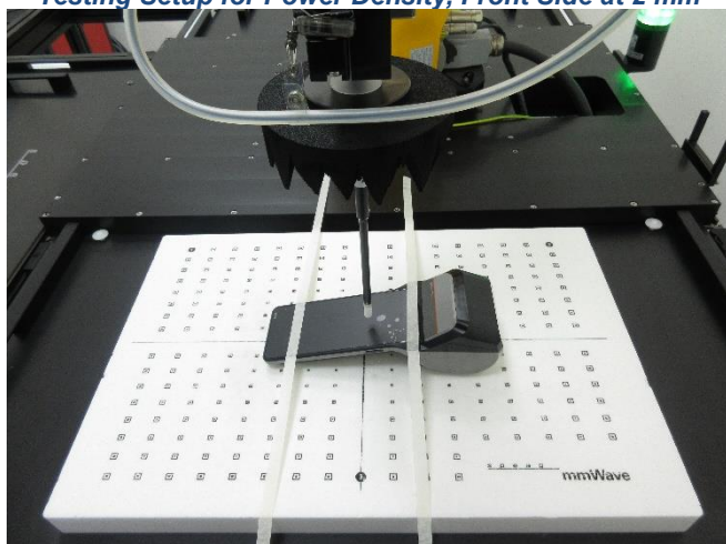
Testing Setup for Power Density, Front Side at 2 mm
