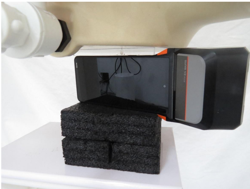
Picture 6: WLAN Antenna Left Edge, the distance from EUT to the bottom of the Phantom is 10mm
