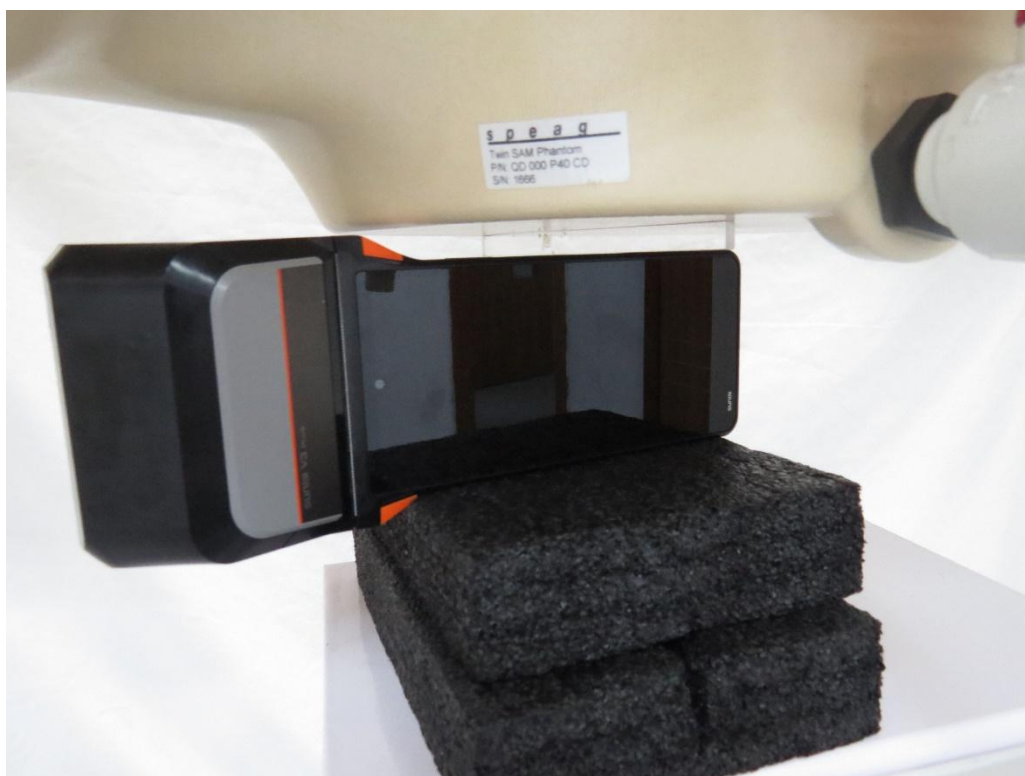
Picture 8: WLAN Antenna Right Edge, the distance from EUT to the bottom of the Phantom is 10mm
