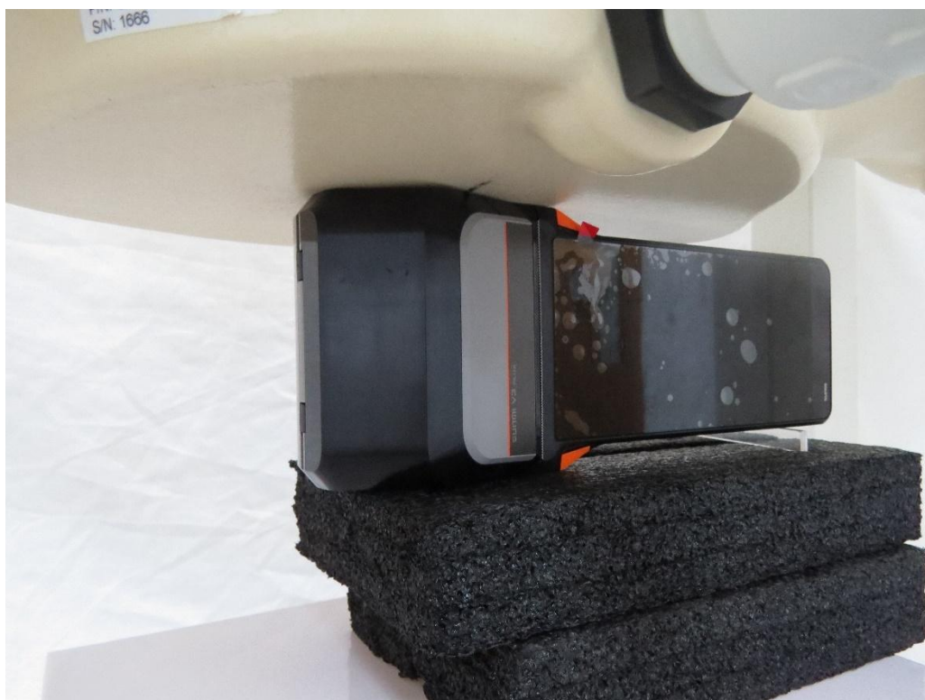
Picture 16: Mian Antenna Right Edge, the distance from EUT to the bottom of the Phantom is 0mm
