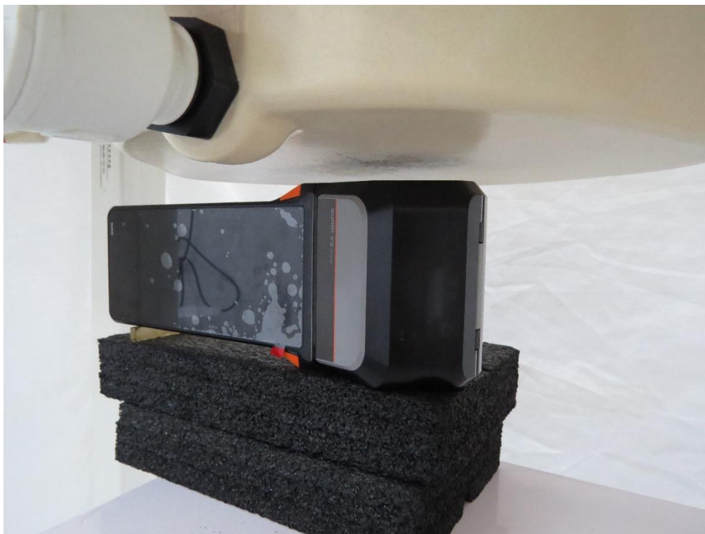
Picture 5: Mian Antenna Left Edge, the distance from EUT to the bottom of the Phantom is 10mm
