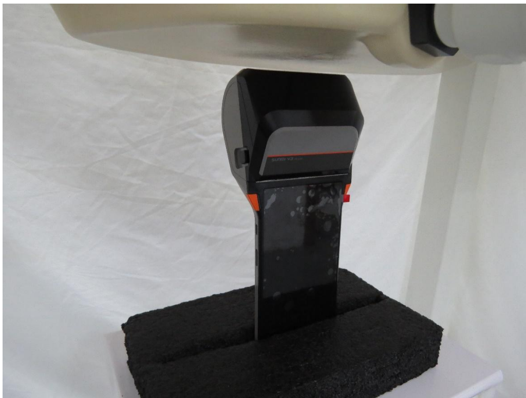
Picture 9: Mian Antenna Top Edge, the distance from EUT to the bottom of the Phantom is 10mm
