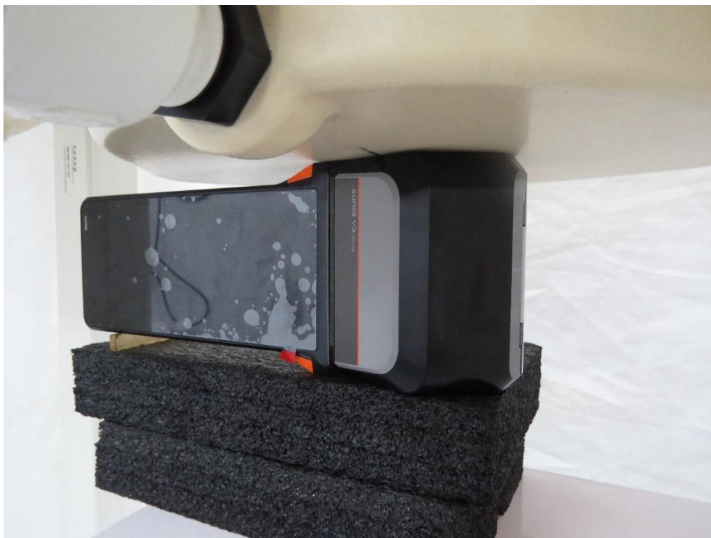
Picture 14: Mian Antenna Left Edge, the distance from EUT to the bottom of the Phantom is 0mm
