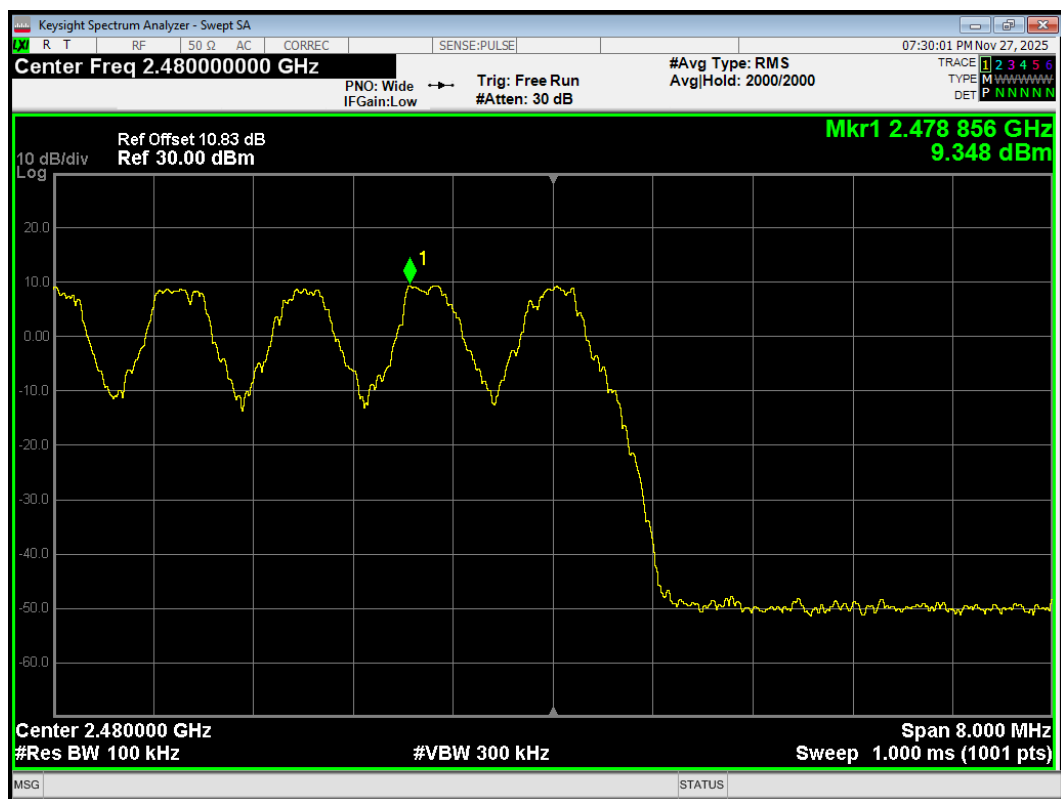
Band Edge(Hopping) 1-DH5 2480MHz Hopping Emission
