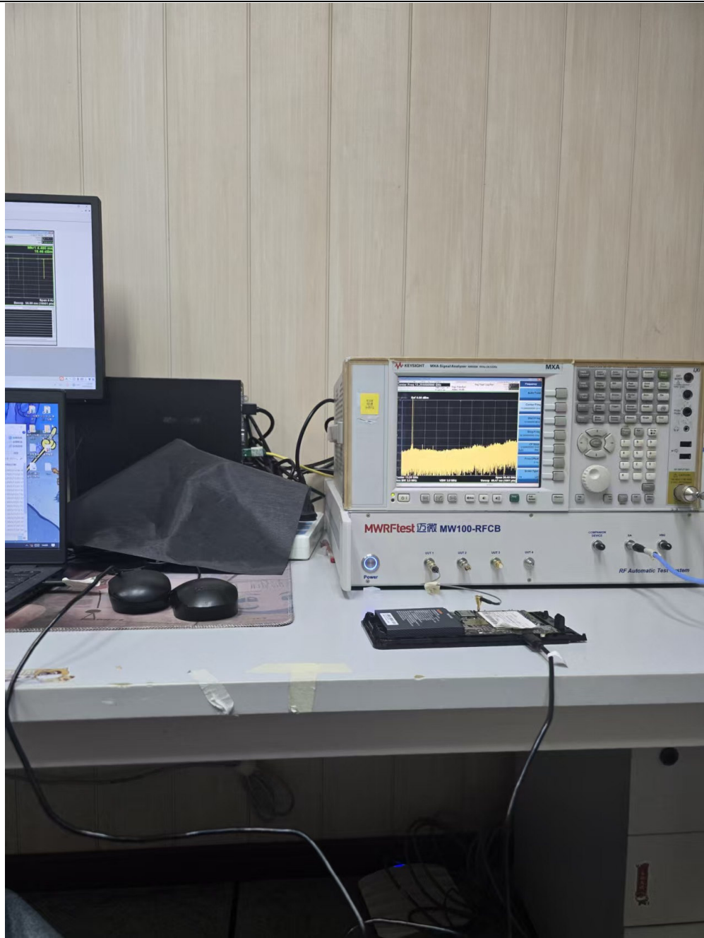
WLAN Test Setup
