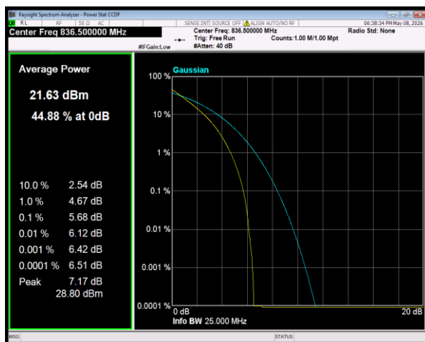
Band5 QPSK BW=10MHz Channel=20525 RB Size=50 Position=#0
