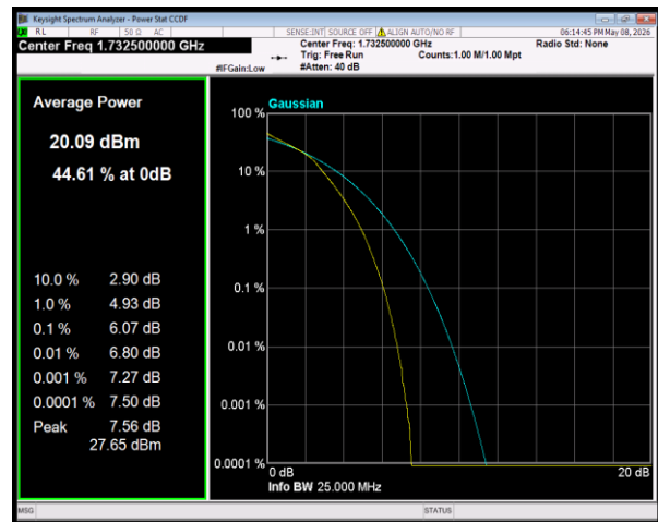
Band4 16QAM BW=20MHz Channel=20175 RB Size=100 Position=#0
