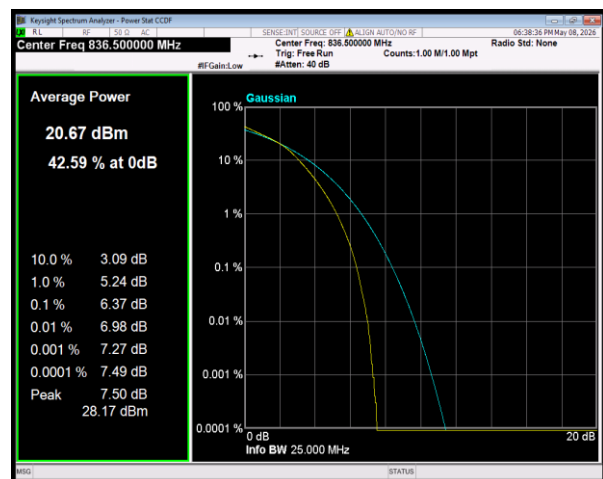
Band5 16QAM BW=10MHz Channel=20525 RB Size=50 Position=#0
