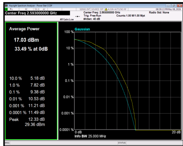
Band41 16QAM BW=20MHz Channel=40620 RB Size=100 Position=#0
