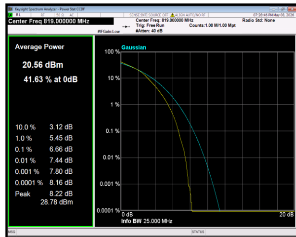
Band26(814-824) 16QAM BW=10MHz Channel=26740 RB Size=50 Position=#0
