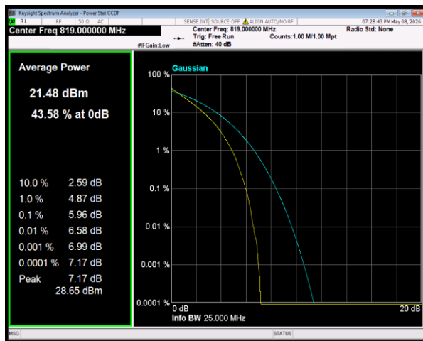
Band26(814-824) QPSK BW=10MHz Channel=26740 RB Size=50 Position=#0
