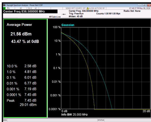
Band26(824-849) QPSK BW=15MHz Channel=26915 RB Size=75 Position=#0
