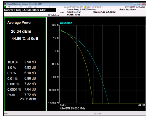
Band7 16QAM BW=20MHz Channel=21100 RB Size=100 Position=#0
