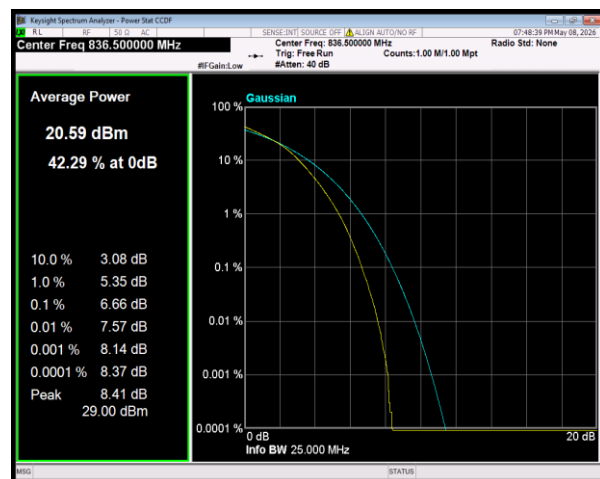
Band26(824-849) 16QAM BW=15MHz Channel=26915 RB Size=75 Position=#0
