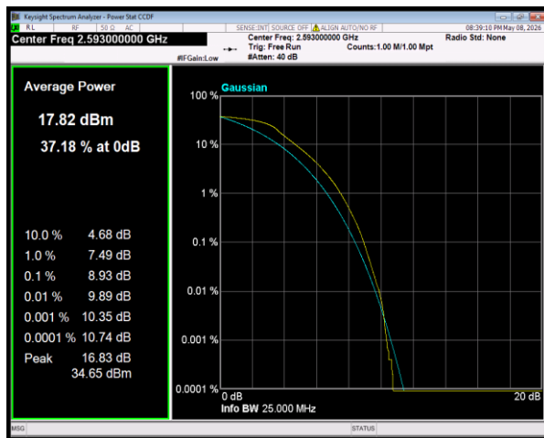
Band41 QPSK BW=20MHz Channel=40620 RB Size=100 Position=#0
