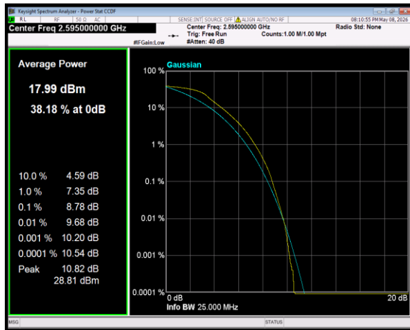
Band38 QPSK BW=20MHz Channel=38000 RB Size=100 Position=#0
