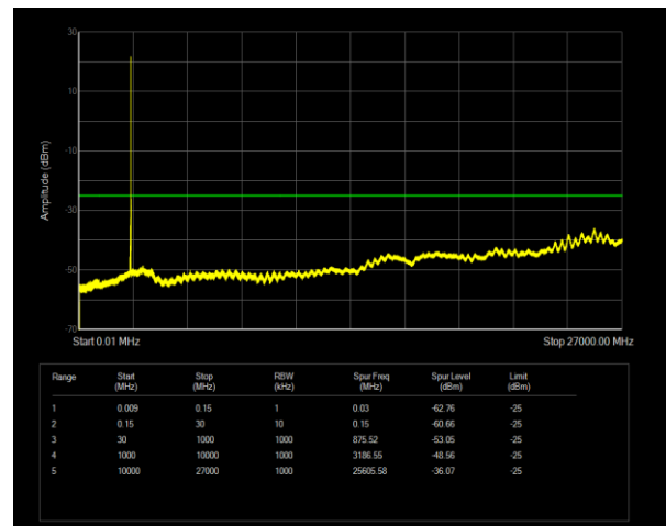
Band7 QPSK BW=5MHz Channel=21425 RB Size=1 Position=#0
