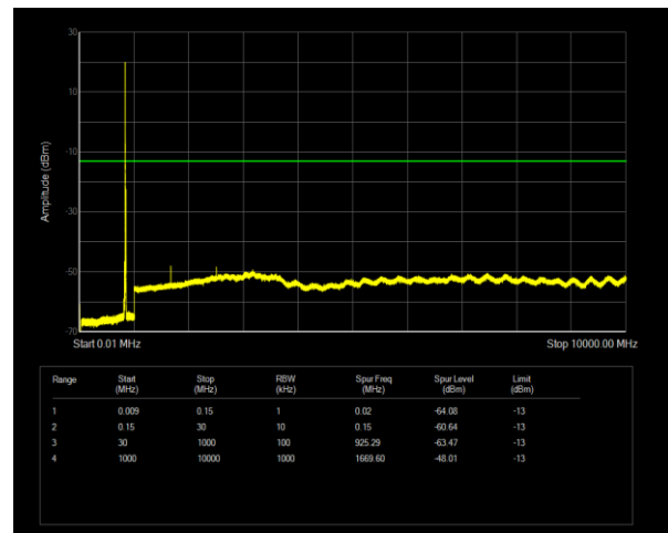
Band26(824-849) QPSK BW=15MHz Channel=26965 RB Size=1 Position=#0
