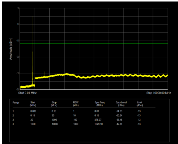
Band26(814-824) QPSK BW=10MHz Channel=26740 RB Size=1 Position=#0
