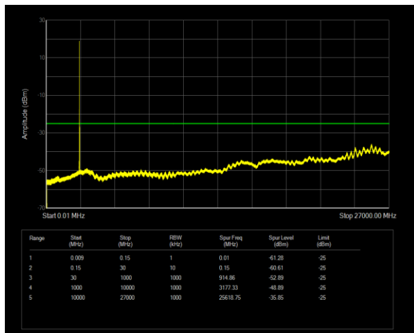
Band38 QPSK BW=10MHz Channel=38000 RB Size=1 Position=#0
