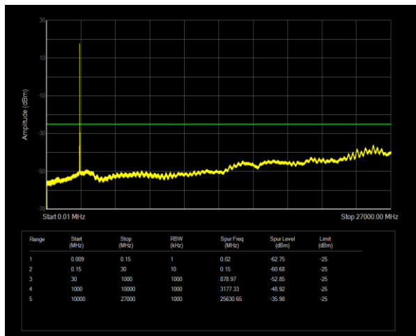
Band41 QPSK BW=20MHz Channel=40620 RB Size=1 Position=#0
