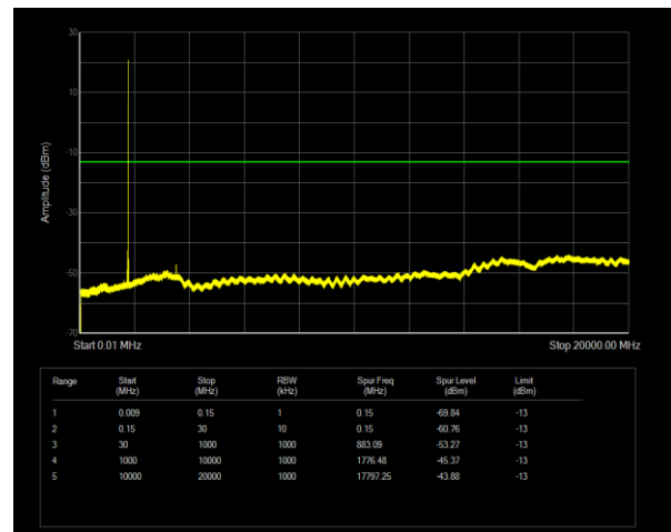
Band4 QPSK BW=1.4MHz Channel=20393 RB Size=1 Position=#0
