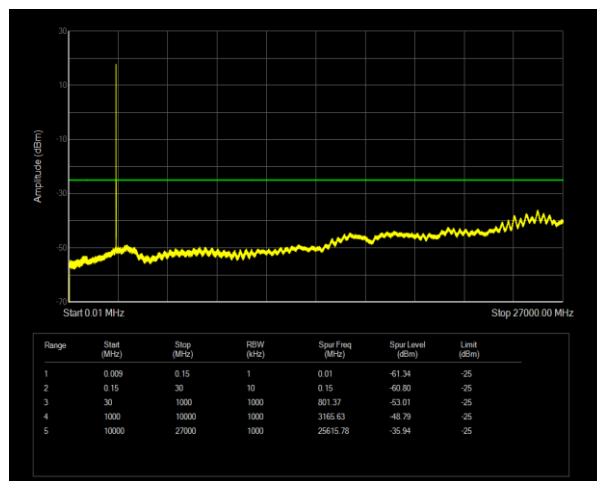
Band38 QPSK BW=5MHz Channel=37775 RB Size=1 Position=#0
