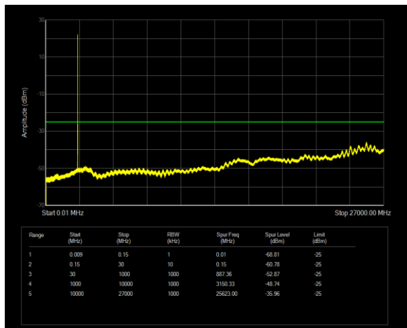
Band7 QPSK BW=5MHz Channel=21100 RB Size=1 Position=#0
