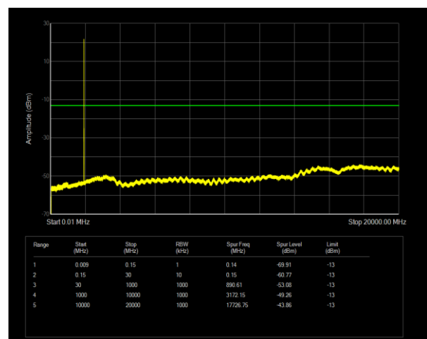
Band2 QPSK BW=5MHz Channel=19175 RB Size=1 Position=#0
