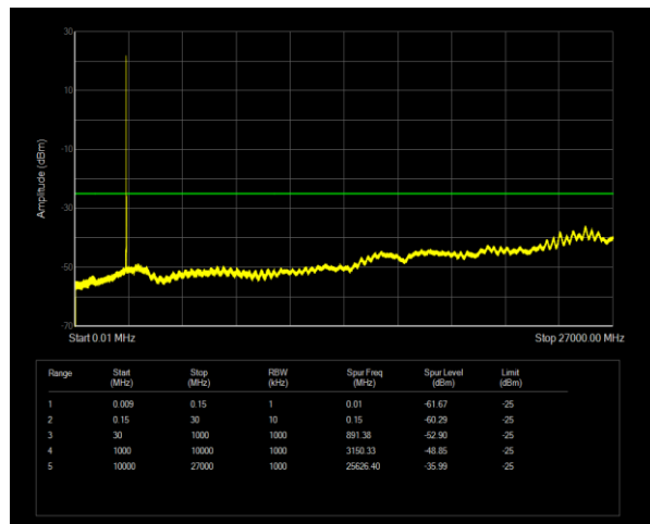
Band7 QPSK BW=10MHz Channel=21400 RB Size=1 Position=#0
