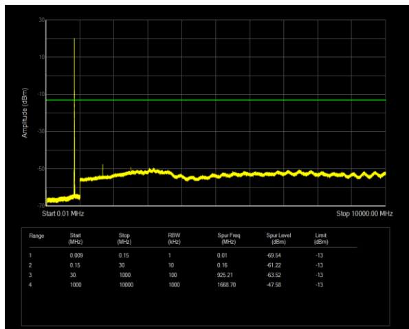
Band5 QPSK BW=5MHz Channel=20525 RB Size=1 Position=#0
