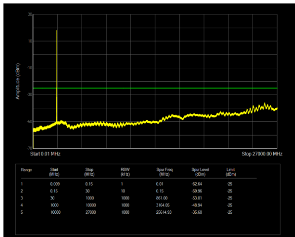
Band38 QPSK BW=20MHz Channel=37850 RB Size=1 Position=#0
