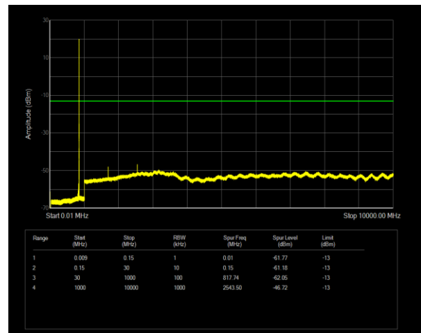
Band26(824-849) QPSK BW=1.4MHz Channel=27033 RB Size=1 Position=#0
