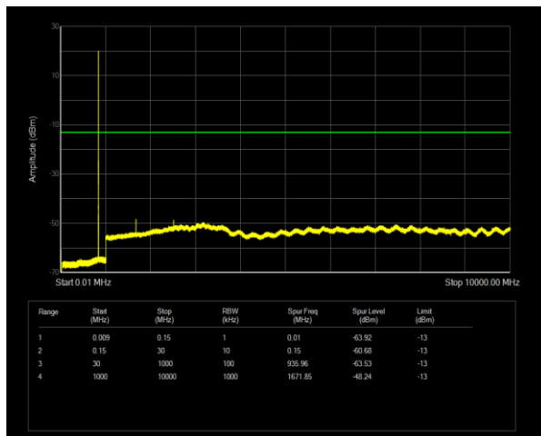
Band26(824-849) QPSK BW=1.4MHz Channel=26915 RB Size=1 Position=#0
