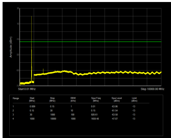
Band26(824-849) QPSK BW=15MHz Channel=26915 RB Size=1 Position=#0
