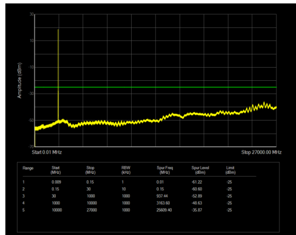
Band38 QPSK BW=10MHz Channel=38200 RB Size=1 Position=#0
