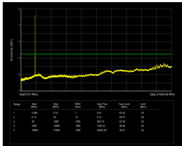
Band7 QPSK BW=10MHz Channel=20800 RB Size=1 Position=#0
