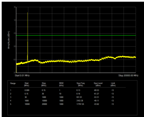
Band2 QPSK BW=20MHz Channel=19100 RB Size=1 Position=#0
