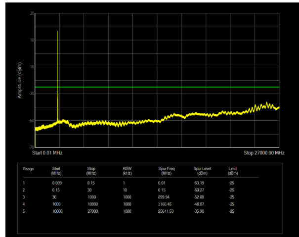
Band41 QPSK BW=20MHz Channel=39750 RB Size=1 Position=#0
