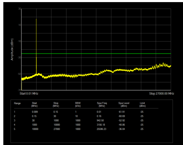
Band41 QPSK BW=20MHz Channel=41490 RB Size=1 Position=#0
