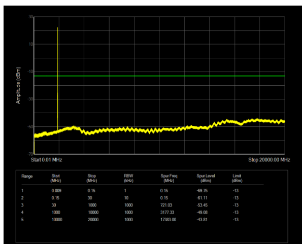
Band2 QPSK BW=5MHz Channel=18900 RB Size=1 Position=#0
