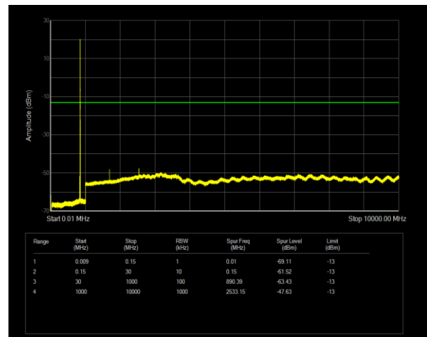
Band5 QPSK BW=5MHz Channel=20625 RB Size=1 Position=#0
