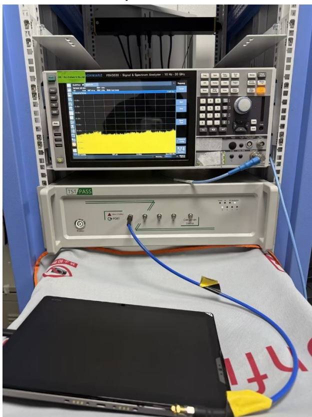
RF Conducted setup
