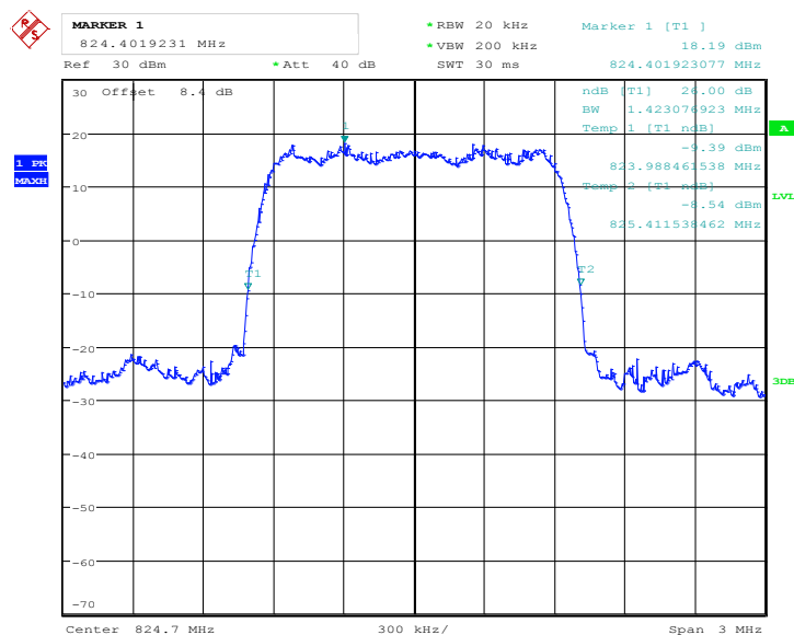
Fig.13 Channel 384- Emission Bandwidth (-26dBc BW)
