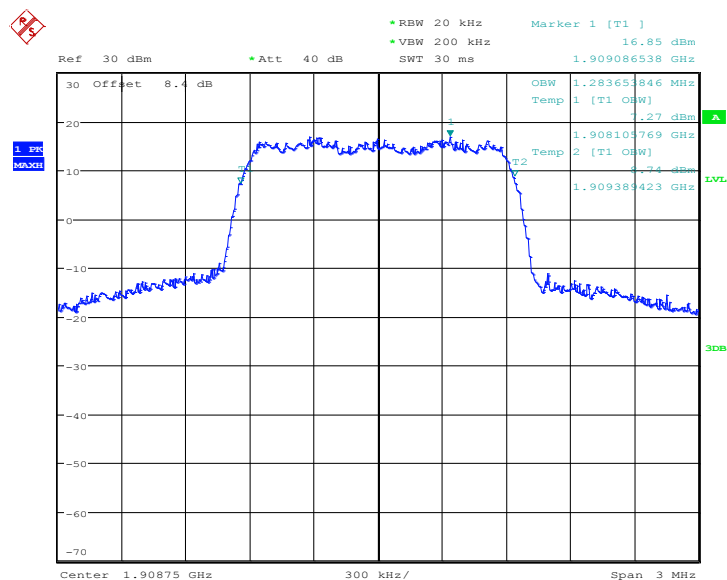
Fig.11 Channel 25-Occupied Bandwidth
