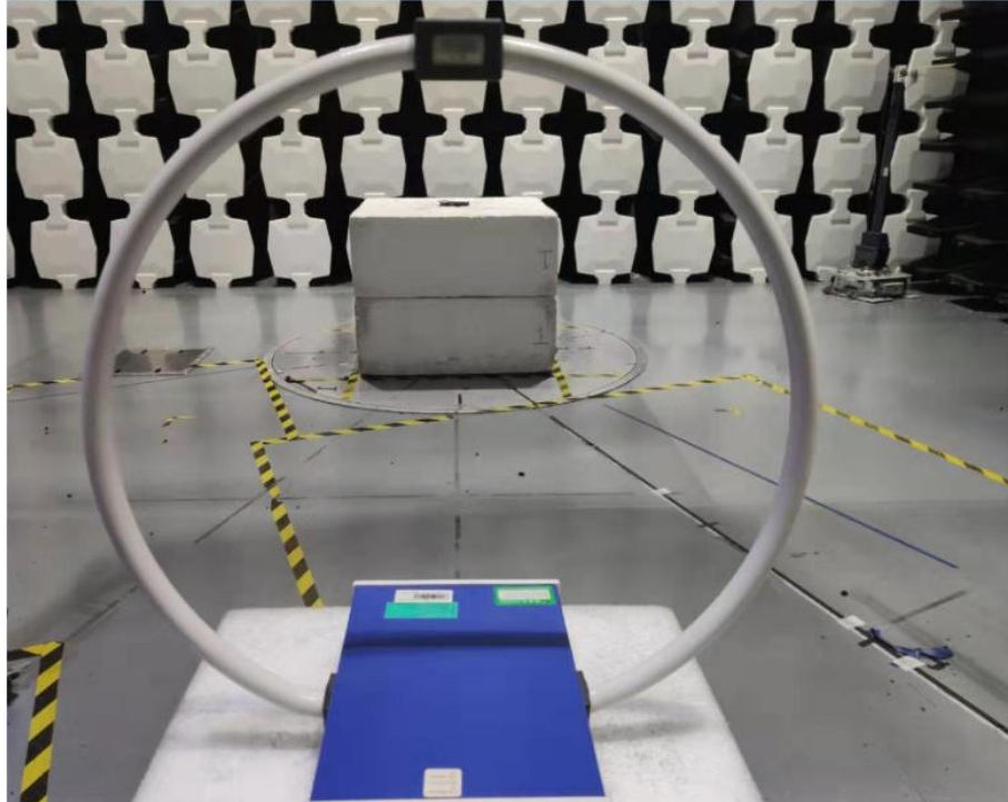
Picture1: Field Radiated Emissions (Below 30MHz)
