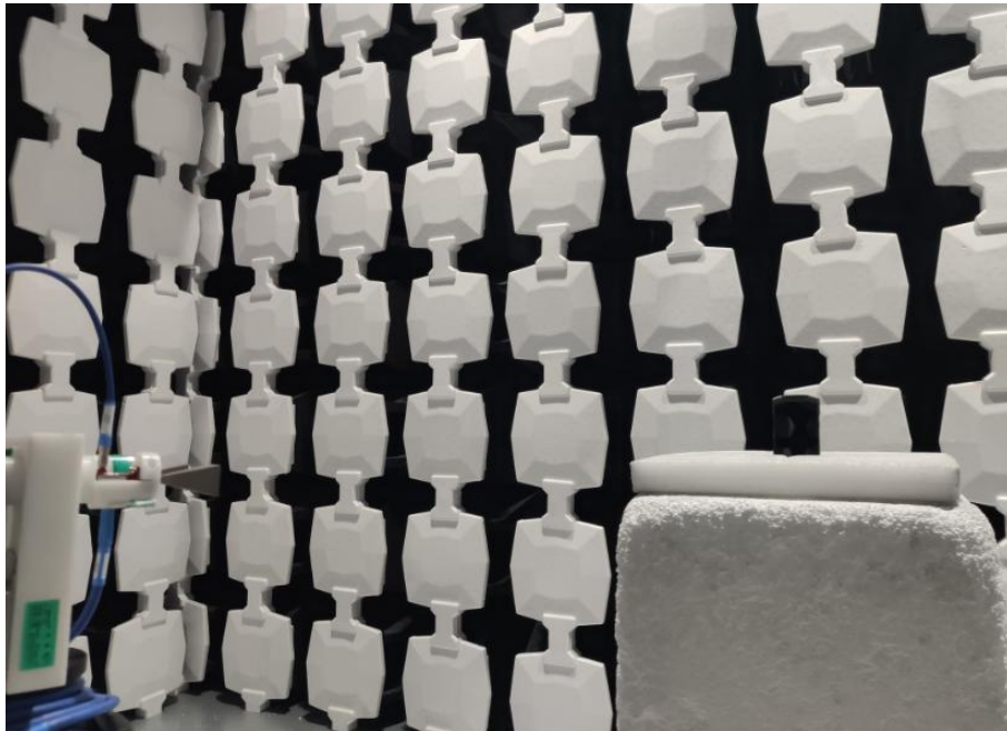
Description: Radiated Emission Test Setup (Above 18GHz)
