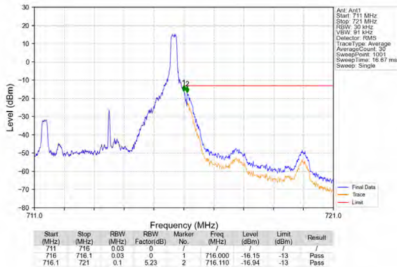
Band12_5MHz_QPSK_HCH_713.5MHz_RB_1_24_NTNV
