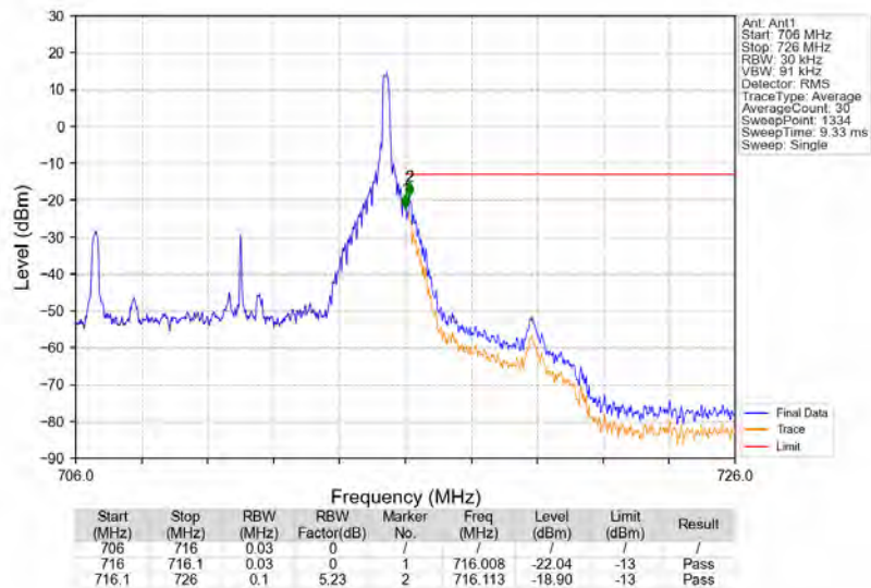
Band12_10MHz_16QAM_HCH_711MHz_RB_1_49_NTNV
