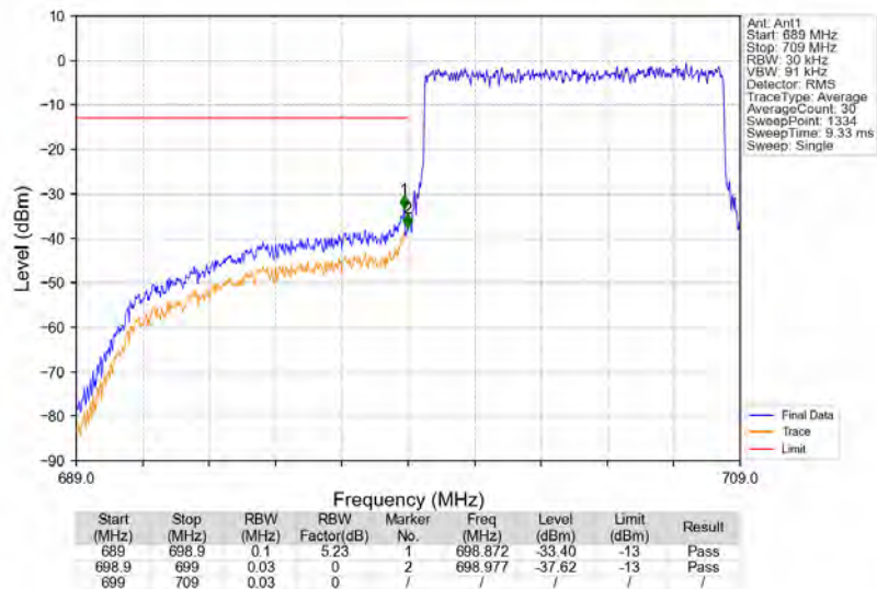
Band12_10MHz_QPSK_LCH_704MHz_RB_50_0_NTNV
