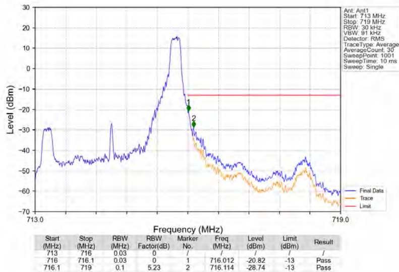
Band12_3MHz_QPSK_HCH_714.5MHz_RB_1_14_NTNV
