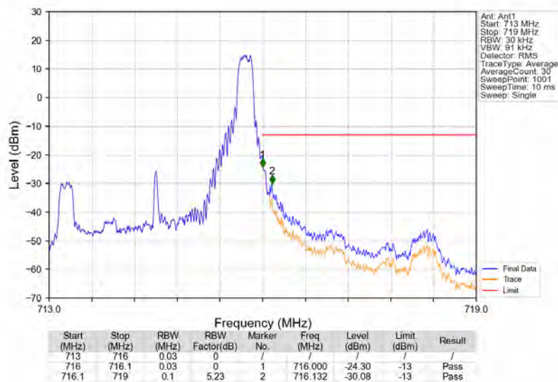
Band12_3MHz_16QAM_HCH_714.5MHz_RB_1_14_NTNV
