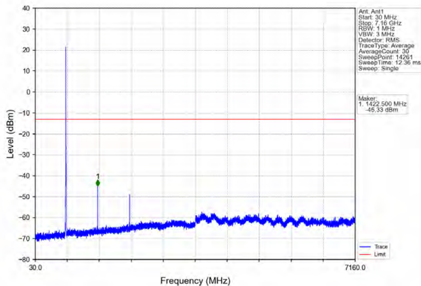
Band12_5MHz_QPSK_HCH_713.5MHz_RB_1_24_NTNV
