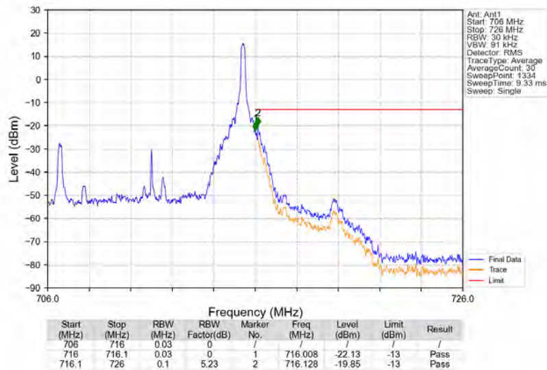
Band12_10MHz_QPSK_HCH_711MHz_RB_1_49_NTNV
