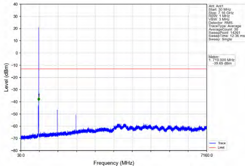
Band12_1.4MHz_QPSK_HCH_715.3MHz_RB_1_5_NTNV
