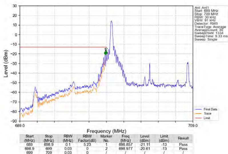
Band12 10MHz 16QAM LCH 704MHz RB 1 0 NTNV
