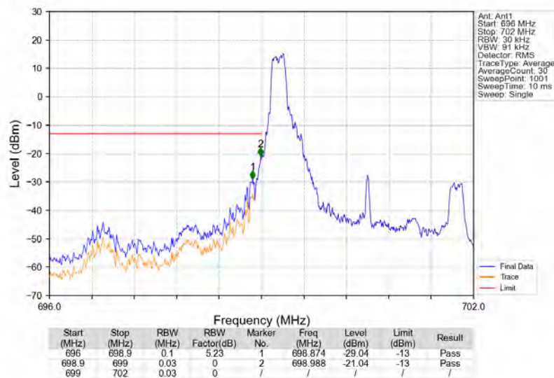
Band12_3MHz_16QAM_LCH_700.5MHz_RB_1_0_NTNV
