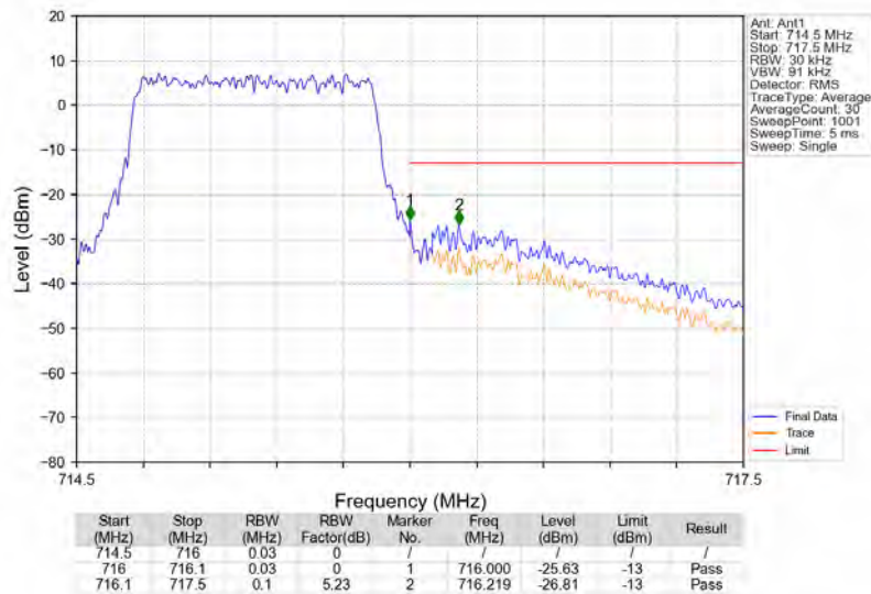
Band12_1.4MHz_16QAM_HCH_715.3MHz_RB_6_0_NTNV
