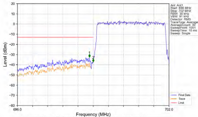
Band12_3MHz_16QAM_LCH_700.5MHz_RB_15_0_NTNV
