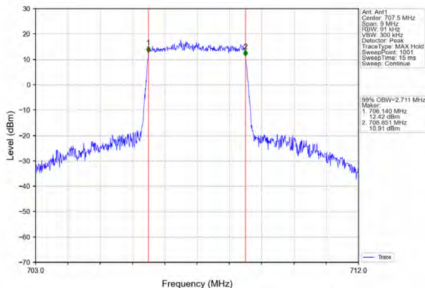
Band12_3MHz_QPSK_MCH_707.5MHz_RB_15_0_NTNV
