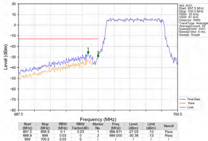
Band12_1.4MHz_16QAM_LCH_699.7MHz_RB_6_0_NTNV
