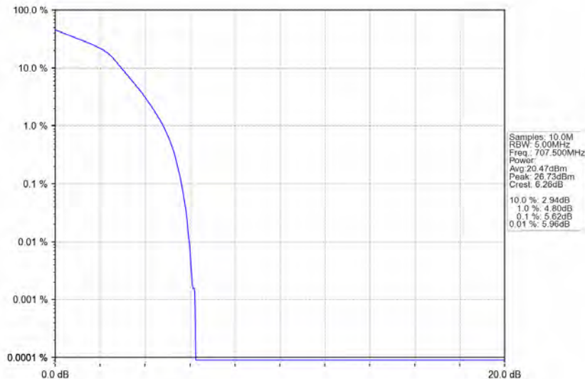
Band12_1.4MHz_16QAM_MCH_707.5MHz_RB_6_0_NTNV
