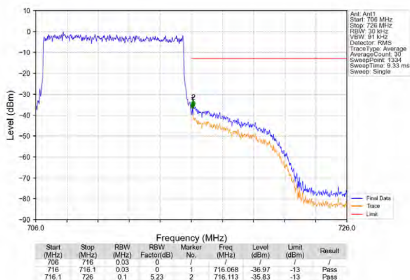
Band12 10MHz QPSK HCH 711MHz RB 50 0 NTVV
