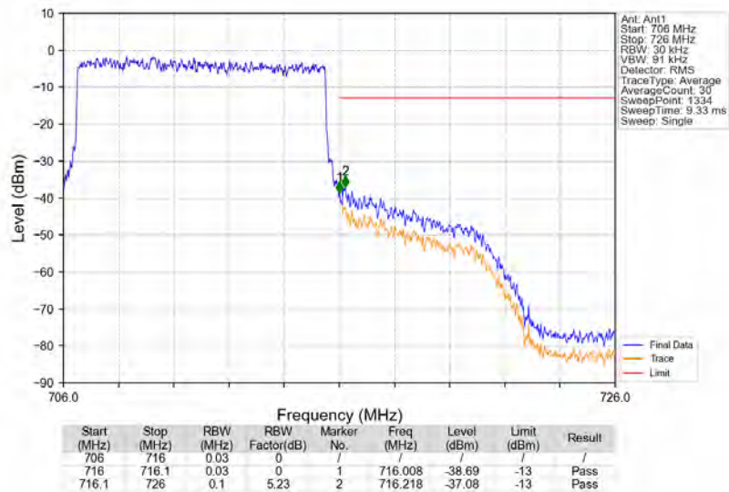
Band12_10MHz_16QAM_HCH_711MHz_RB_50_0_NTNV
