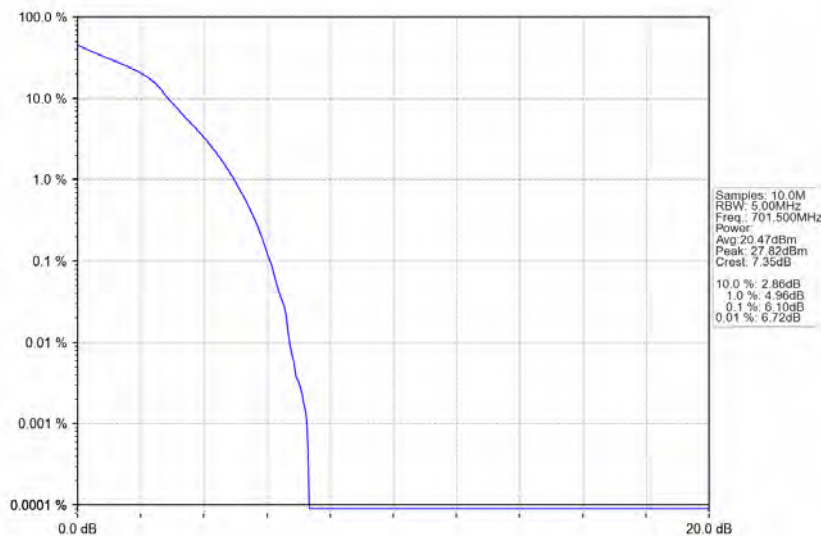
Band12_5MHz_16QAM_LCH_701.5MHz_RB_25_0_NTNV
