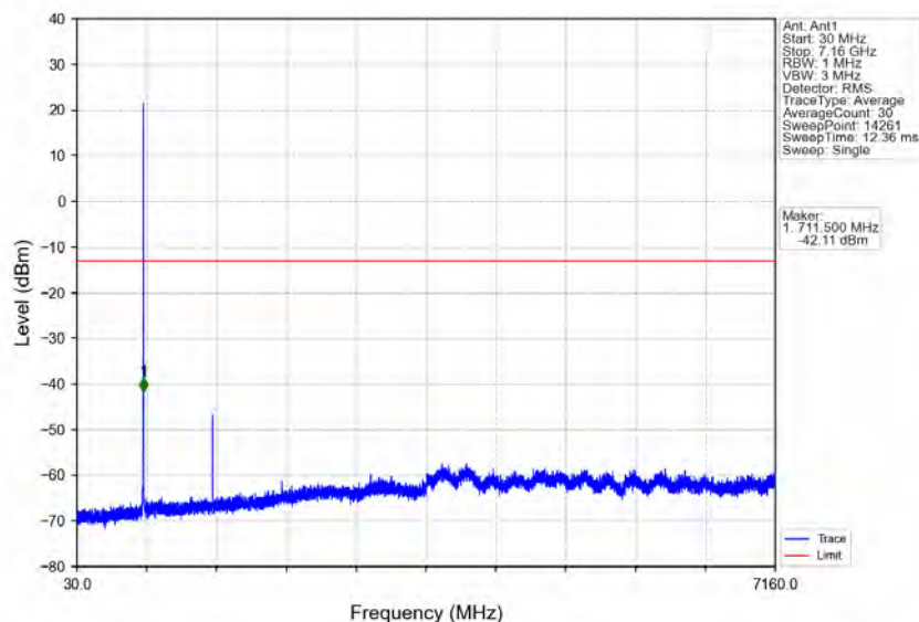
Band12_1.4MHz_QPSK_MCH_707.5MHz_RB_1_0_NTNV
