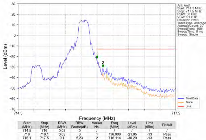
Band12_1.4MHz_16QAM_HCH_715.3MHz_RB_1_5_NTNV
