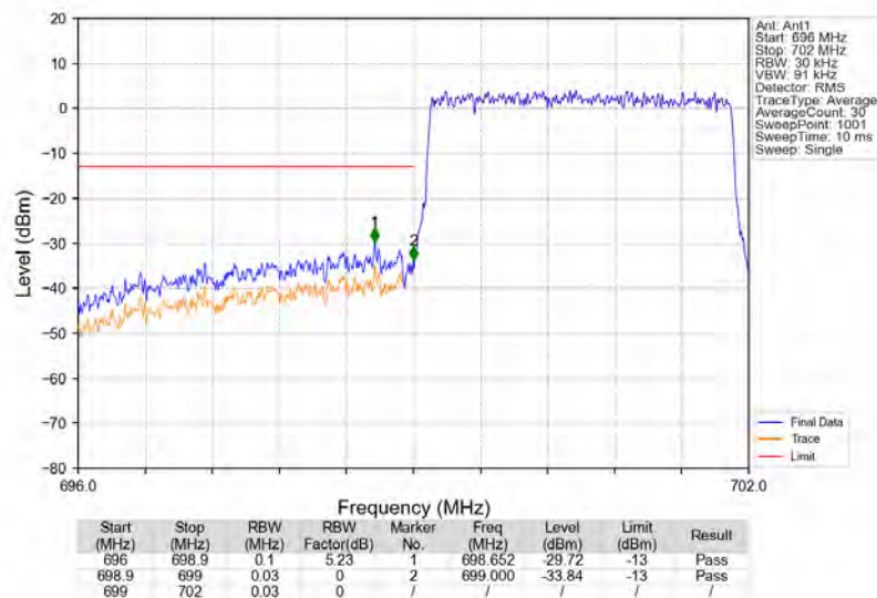
Band12_3MHz_QPSK_LCH_700.5MHz_RB_15_0_NTNV
