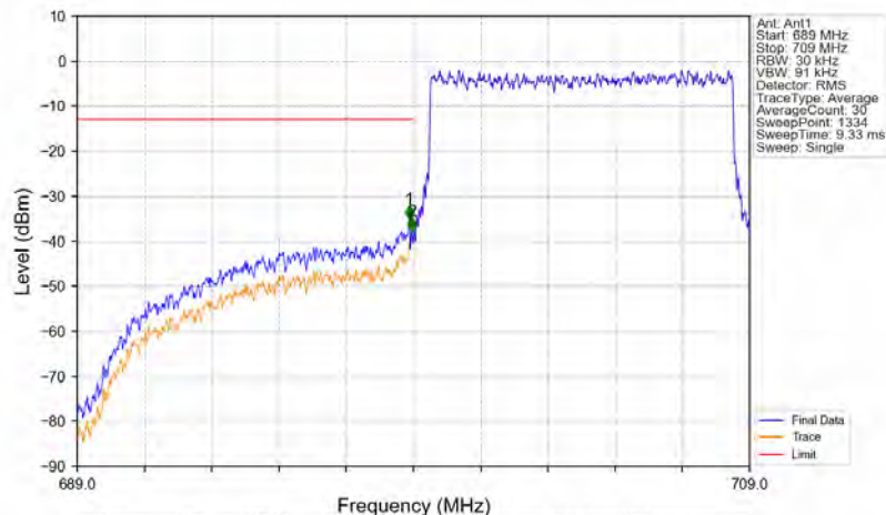
Band12_10MHz_16QAM_LCH_704MHz_RB_50_0_NTNV
