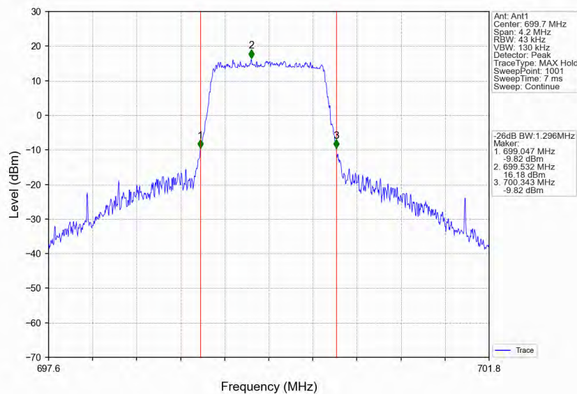
Band12_1.4MHz_16QAM_LCH_699.7MHz_RB_6_0_NTNV
