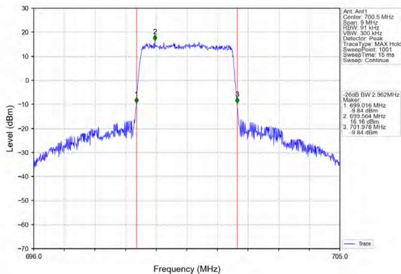
Band12_3MHz_16QAM_LCH_700.5MHz_RB_15_0_NTNV
