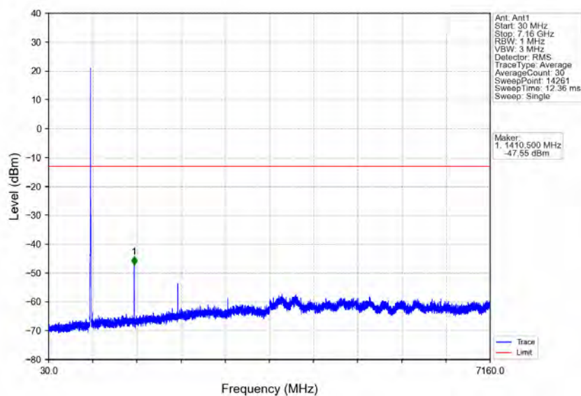
Band12_5MHz_QPSK_MCH_707.5MHz_RB_1_0_NTNV
