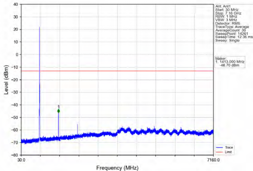
Band12_10MHz_QPSK_HCH_711MHz_RB_1_49_NTNV
