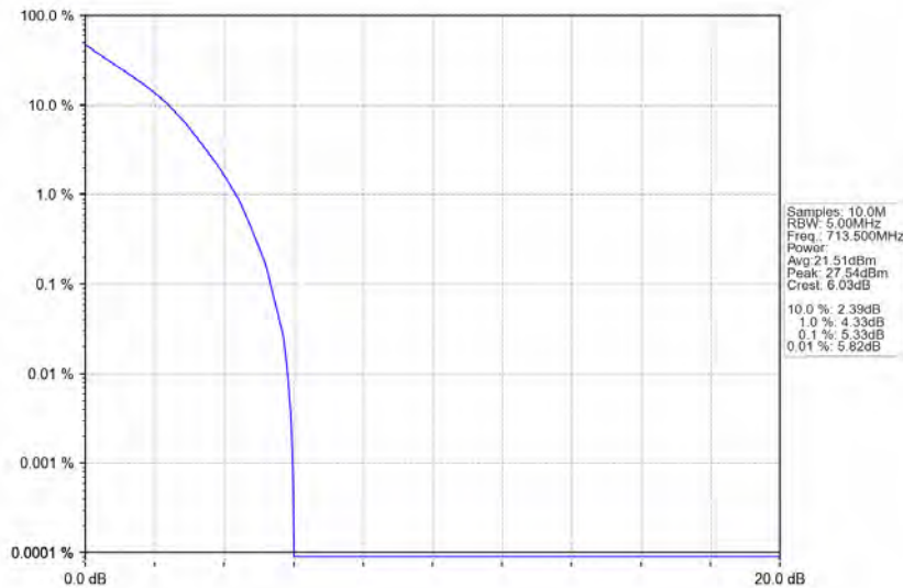
Band12_5MHz_QPSK_HCH_713.5MHz_RB_25_0_NTNV
