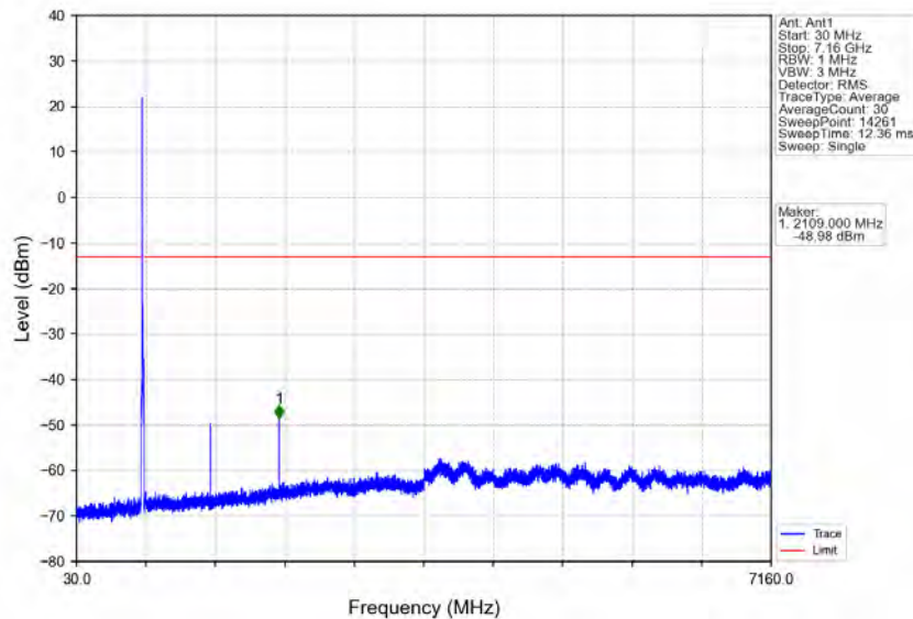
Band12_10MHz_16QAM_HCH_711MHz_RB_1_0_NTNV
