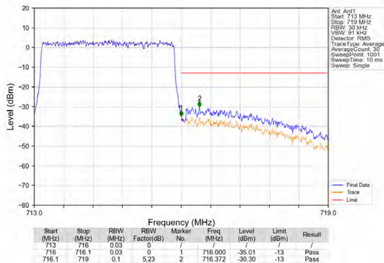
Band12_3MHz_QPSK_HCH_714.5MHz_RB_15_0_NTNV
