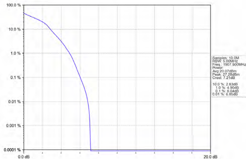
Band2_5MHz_16QAM_HCH_1907.5MHz_RB_25_0_NTNV
