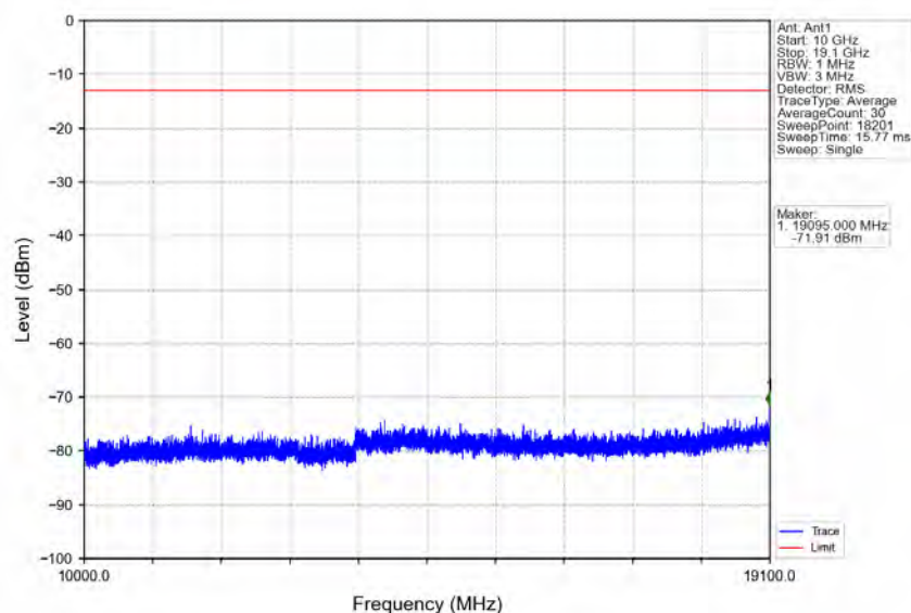
Band2_5MHz_16QAM_MCH_1880MHz_RB_1_0_NTNV
