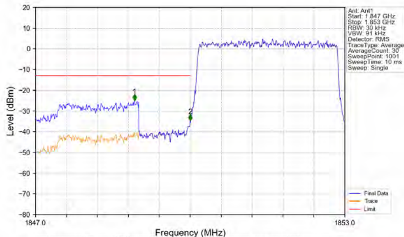
Band2_3MHz_QPSK_LCH_1851.5MHz_RB_15_0_NTNV
