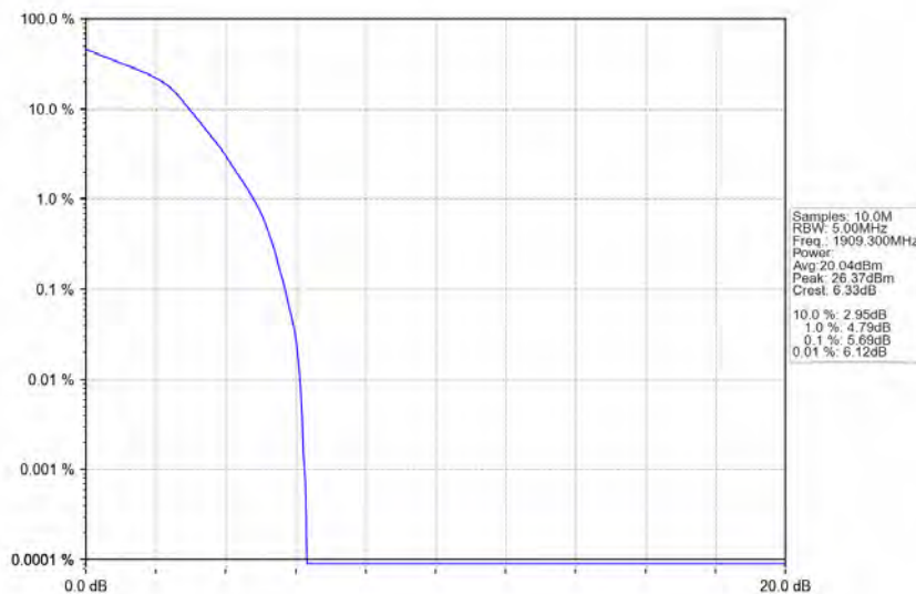
Band2_1.4MHz_16QAM_HCH_1909.3MHz_RB_6_0_NTNV
