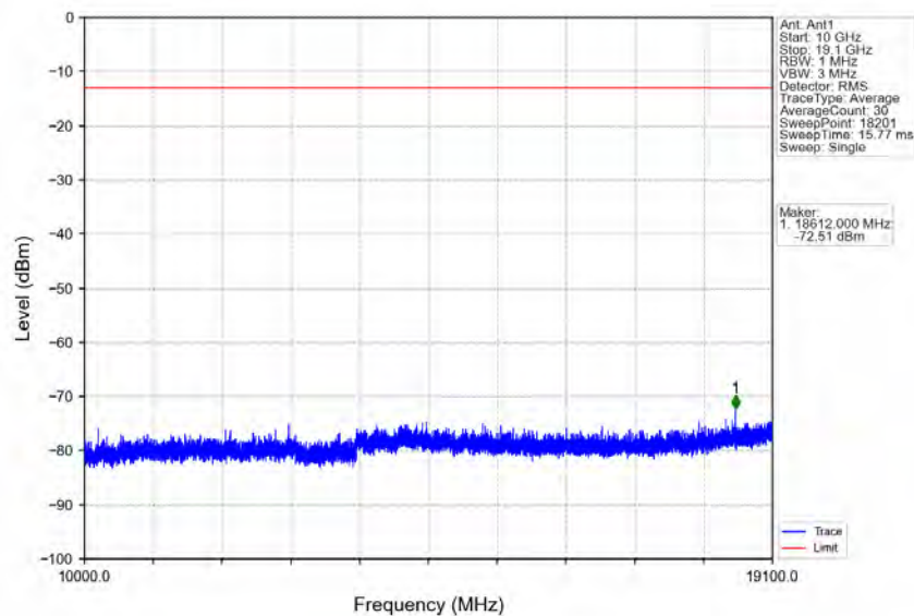
Band2_15MHz_QPSK_LCH_1857.5MHz_RB_75_0_NTNV
