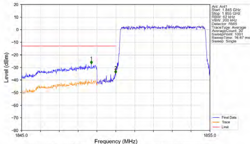
Band2_5MHz_16QAM_LCH_1852.5MHz_RB_25_0_NTNV
