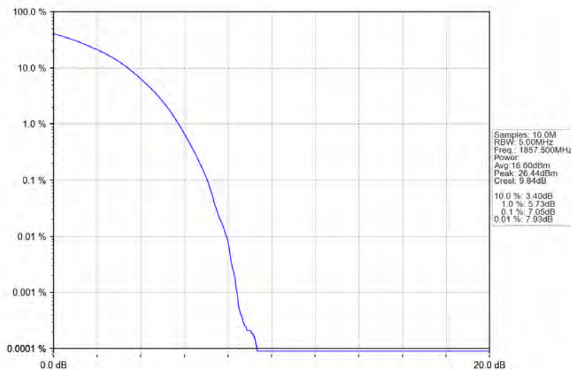
Band2_15MHz_16QAM_LCH_1857.5MHz_RB_75_0_NTNV
