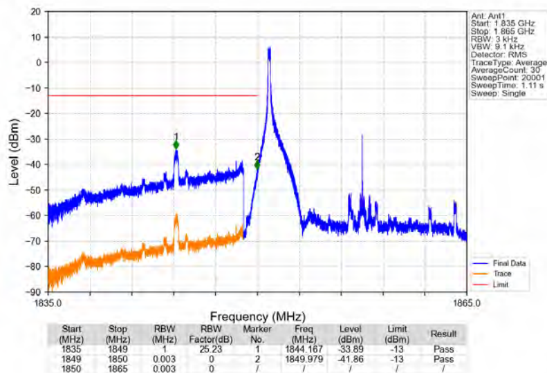
Band2_15MHz_16QAM_LCH_1857.5MHz_RB_1_0_NTNV
