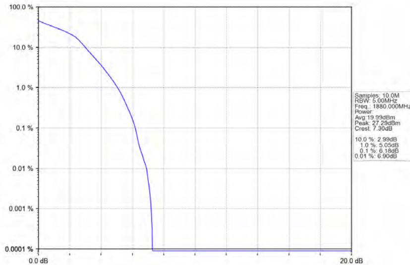
Band2_1.4MHz_16QAM_MCH_1880MHz_RB_6_0_NTNV
