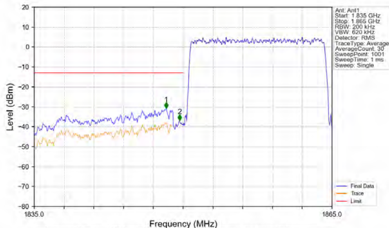
Band2_15MHz_QPSK_LCH_1857.5MHz_RB_75_0_NTNV
