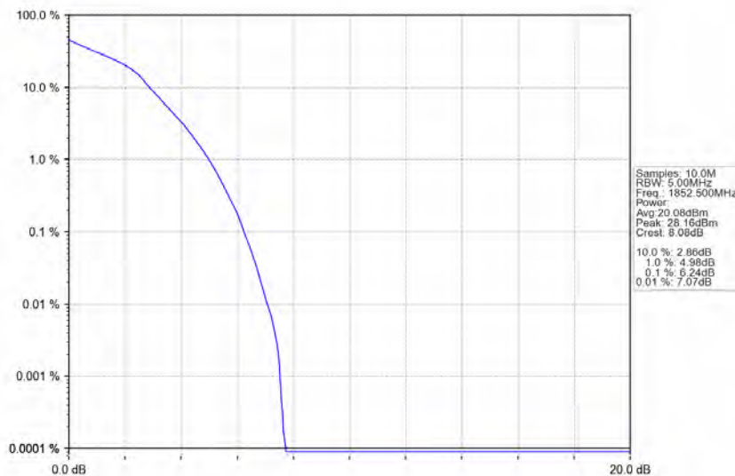
Band2_5MHz_16QAM_LCH_1852.5MHz_RB_25_0_NTNV
