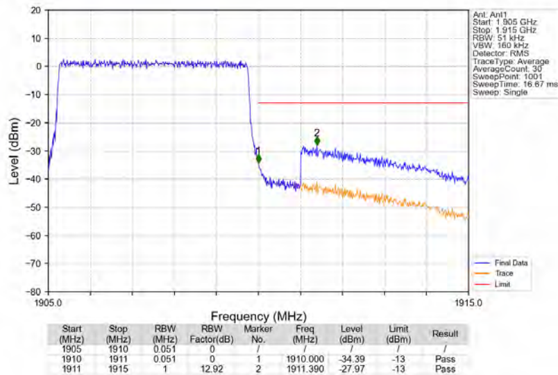
Band2_5MHz_16QAM_HCH_1907.5MHz_RB_25_0_NTNV
