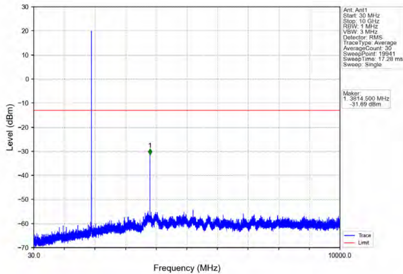
Band2_3MHz_16QAM_HCH_1908.5MHz_RB_1_0_NTNV
