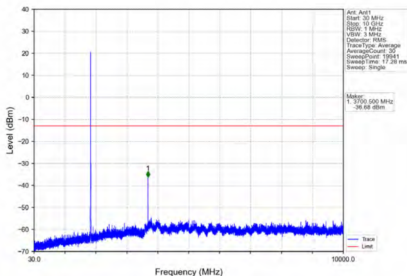
Band2_5MHz_16QAM_LCH_1852.5MHz_RB_1_0_NTNV
