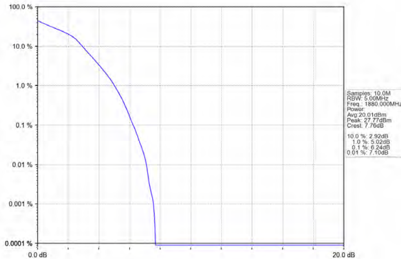
Band2_3MHz_16QAM_MCH_1880MHz_RB_15_0_NTNV
