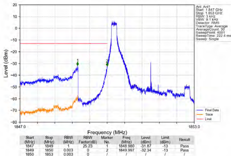
Band2_3MHz_16QAM_LCH_1851.5MHz_RB_1_0_NTNV
