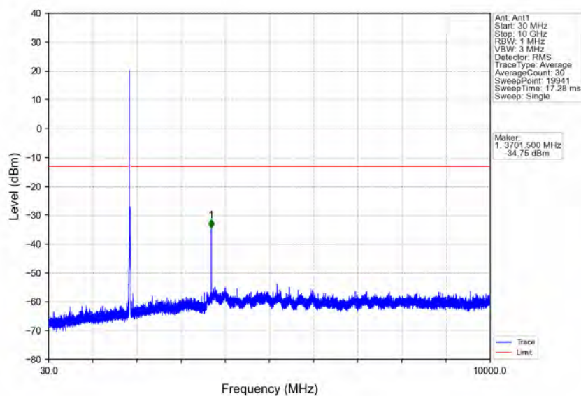
Band2_15MHz_16QAM_LCH_1857.5MHz_RB_1_0_NTNV
