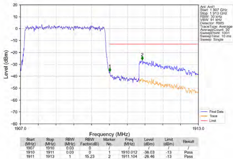
Band2_3MHz_16QAM_HCH_1908.5MHz_RB_15_0_NTNV
