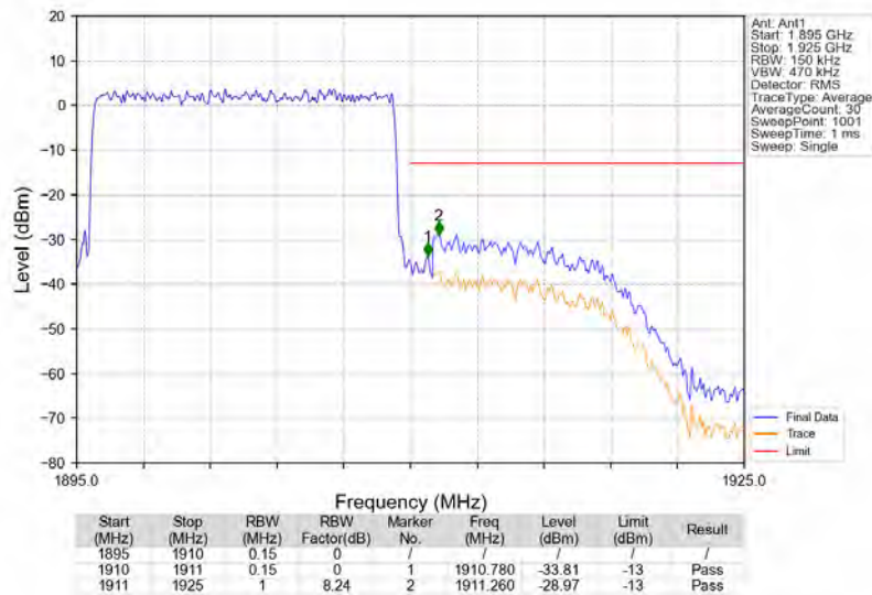
Band2_15MHz_QPSK_HCH_1902.5MHz_RB_75_0_NTNV
