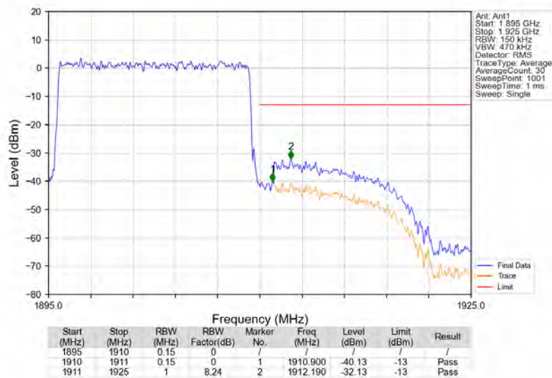
Band2_15MHz_16QAM_HCH_1902.5MHz_RB_75_0_NTNV
