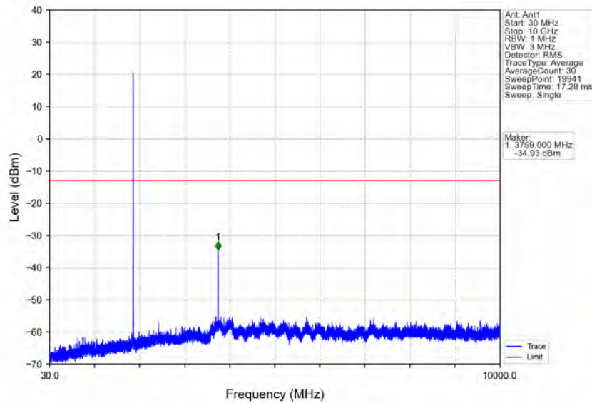
Band2_1.4MHz_16QAM_MCH_1880MHz_RB_1_0_NTNV
