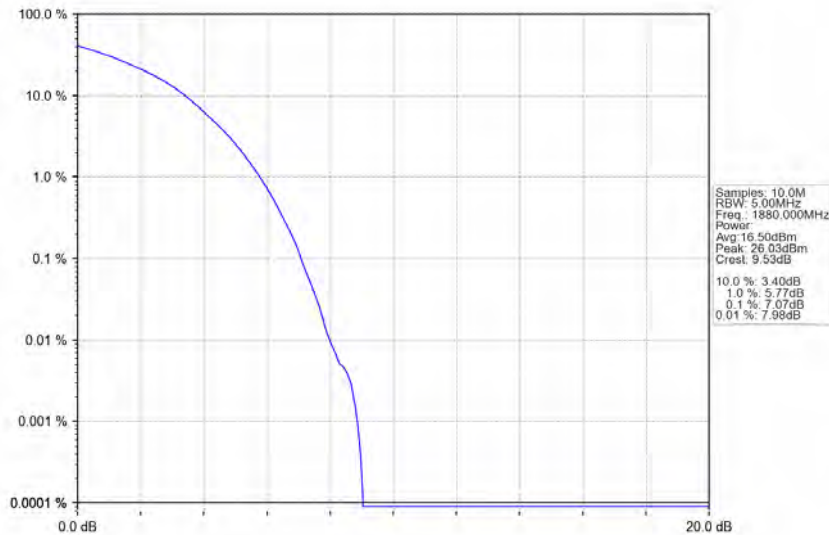
Band2_15MHz_16QAM_MCH_1880MHz_RB_75_0_NTNV
