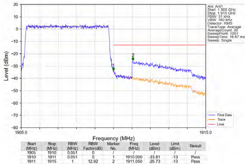
Band2_5MHz_QPSK_HCH_1907.5MHz_RB_25_0_NTNV
