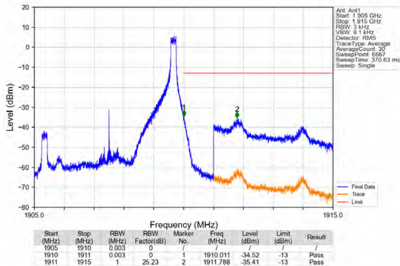
Band2_5MHz_16QAM_HCH_1907.5MHz_RB_1_24_NTNV
