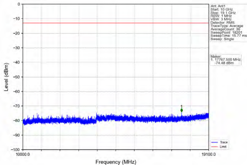
Band2_1.4MHz_QPSK_LCH_1850.7MHz_RB_6_0_NTNV
