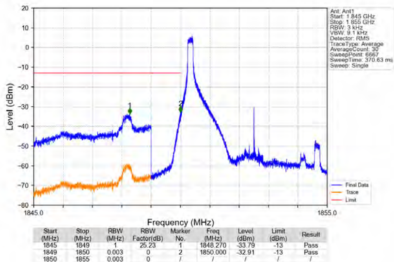
Band2_5MHz_16QAM_LCH_1852.5MHz_RB_1_0_NTNV
