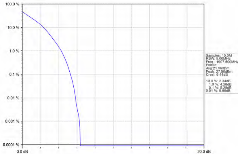
Band2_5MHz_QPSK_HCH_1907.5MHz_RB_25_0_NTNV
