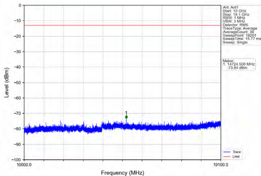
Band2_1.4MHz_16QAM_MCH_1880MHz_RB_1_0_NTNV
