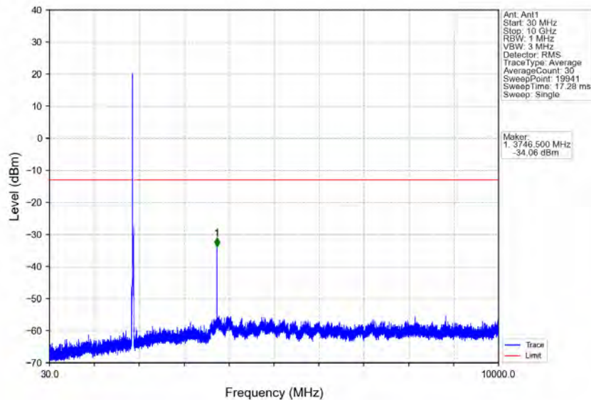
Band2_15MHz_16QAM_MCH_1880MHz_RB_1_0_NTNV
