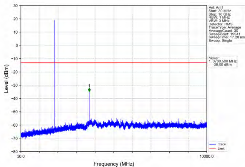
Band2_1.4MHz_16QAM_LCH_1850.7MHz_RB_1_0_NTNV
