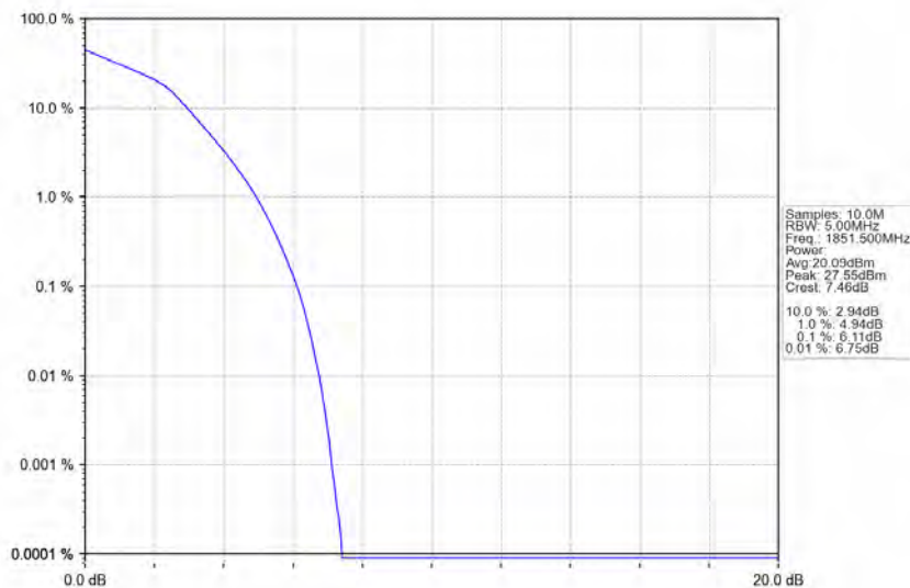
Band2_3MHz_16QAM_LCH_1851.5MHz_RB_15_0_NTNV
