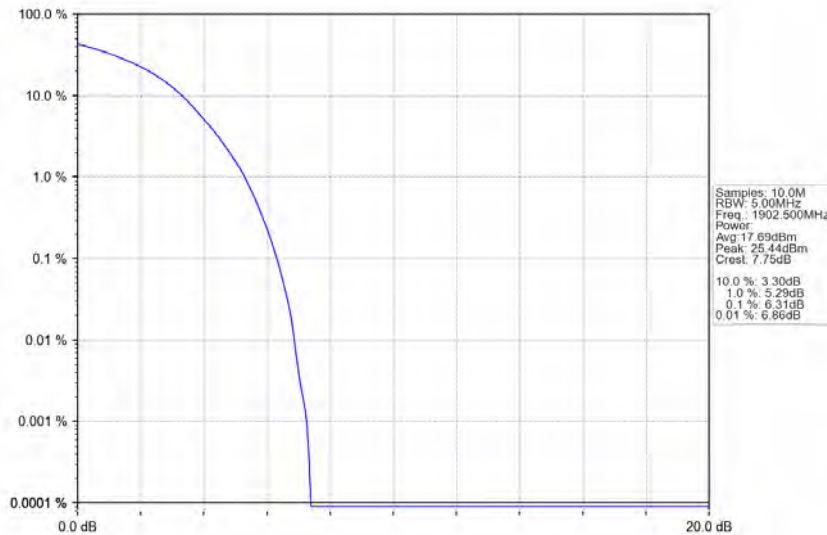
Band2_15MHz_QPSK_HCH_1902.5MHz_RB_75_0_NTNV
