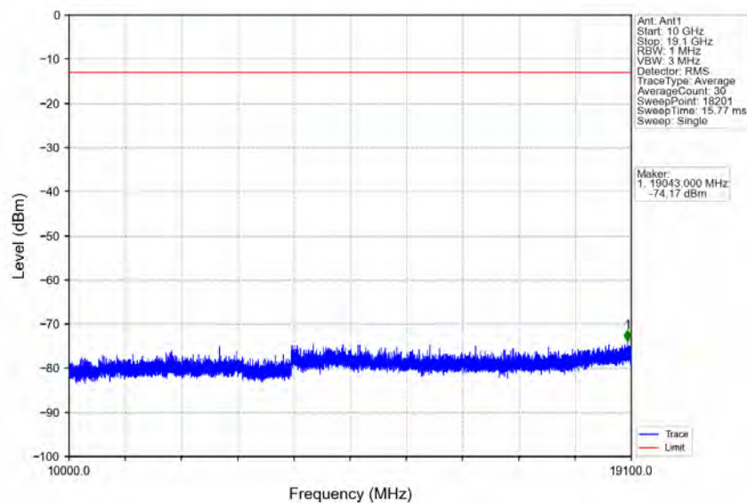
Band2_15MHz_16QAM_MCH_1880MHz_RB_1_0_NTNV
