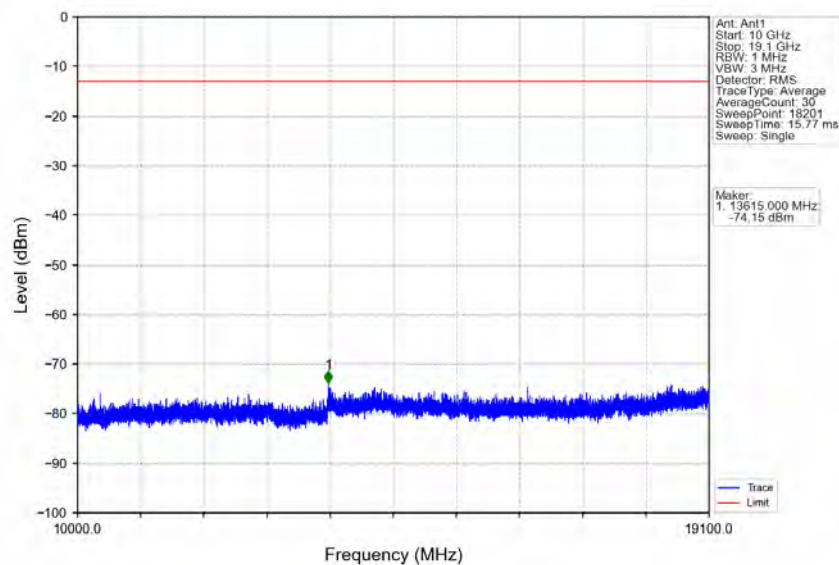
Band2_3MHz_16QAM_HCH_1908.5MHz_RB_1_0_NTNV
