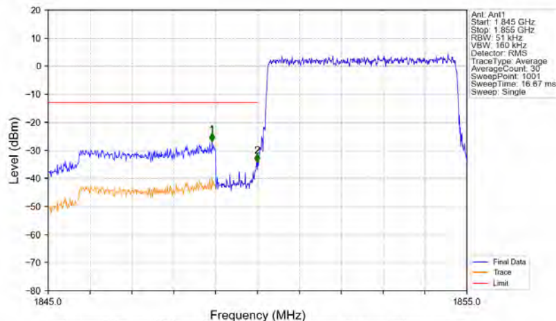
Band2_5MHz_QPSK_LCH_1852.5MHz_RB_25_0_NTNV
