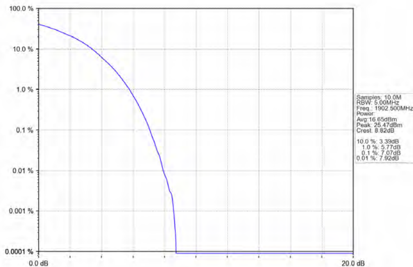
Band2_15MHz_16QAM_HCH_1902.5MHz_RB_75_0_NTNV
