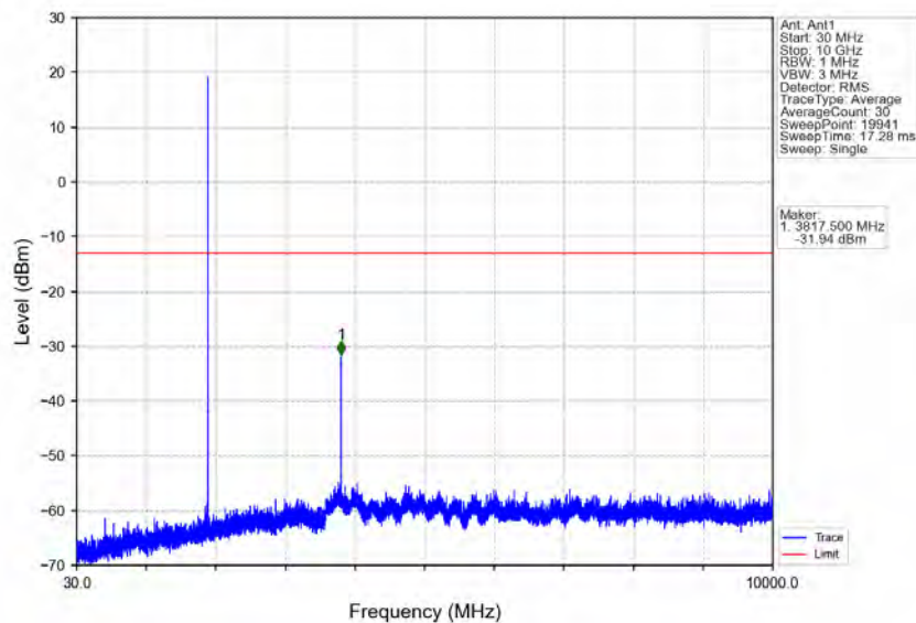
Band2_1.4MHz_16QAM_HCH_1909.3MHz_RB_1_0_NTNV
