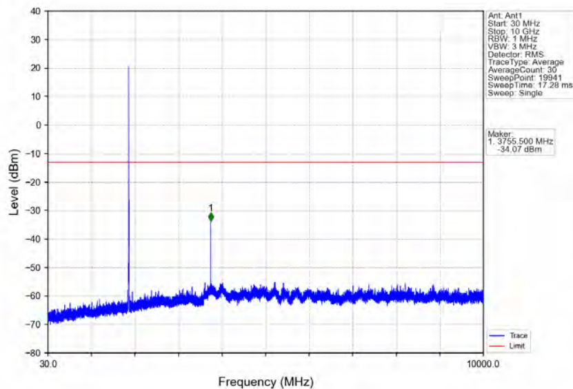
Band2_5MHz_16QAM_MCH_1880MHz_RB_1_0_NTNV
