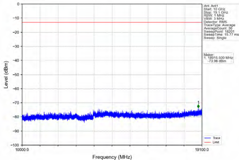
Band2_1.4MHz_16QAM_LCH_1850.7MHz_RB_6_0_NTNV
