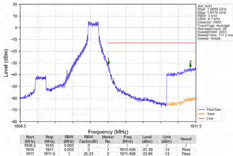
Band2_1.4MHz_16QAM_HCH_1909.3MHz_RB_1_5_NTNV
