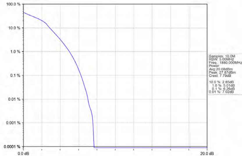
Band2_5MHz_16QAM_MCH_1880MHz_RB_25_0_NTNV
