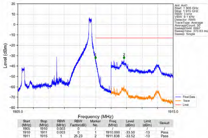
Band2_5MHz_QPSK_HCH_1907.5MHz_RB_1_24_NTNV
