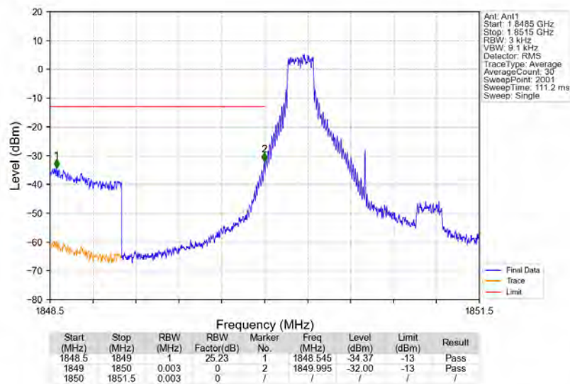
Band2_1.4MHz_16QAM_LCH_1850.7MHz_RB_1_0_NTNV
