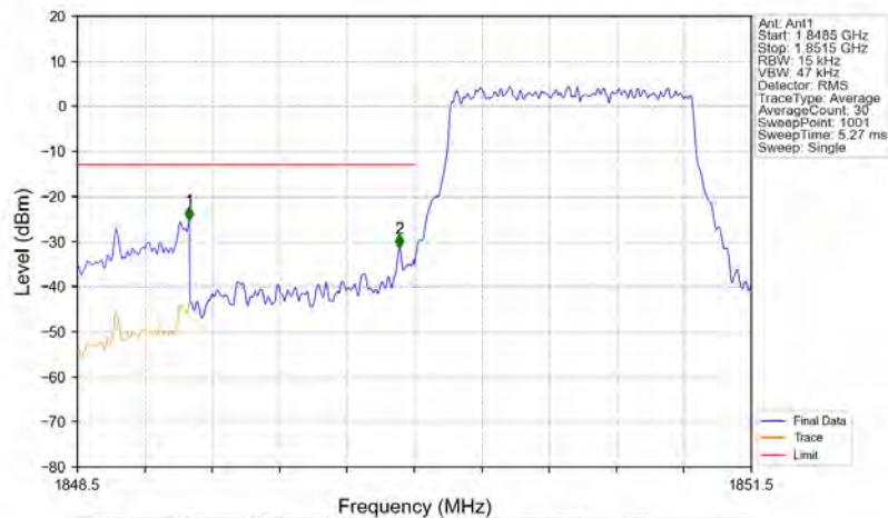
Band2_1.4MHz_QPSK_LCH_1850.7MHz_RB_6_0_NTNV
