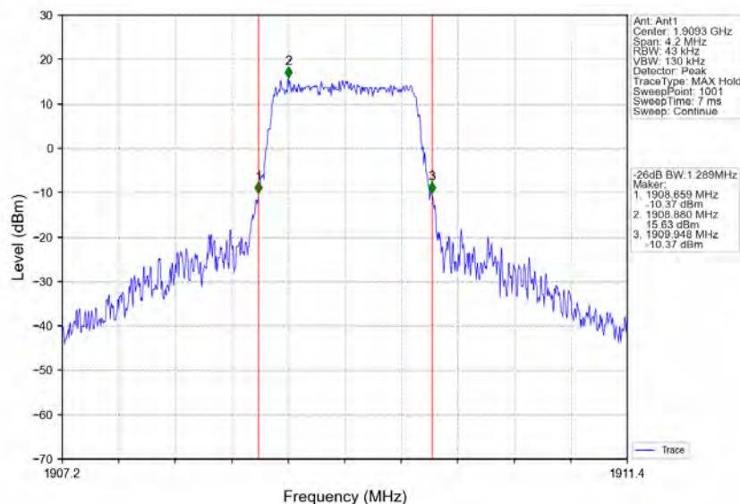
Band2_1.4MHz_16QAM_HCH_1909.3MHz_RB_6_0_NTNV
