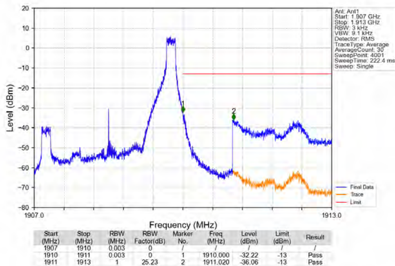
Band2_3MHz_16QAM_HCH_1908.5MHz_RB_1_14_NTNV
