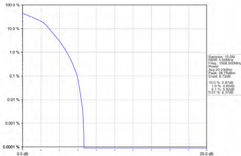
Band2_3MHz_16QAM_HCH_1908.5MHz_RB_15_0_NTNV
