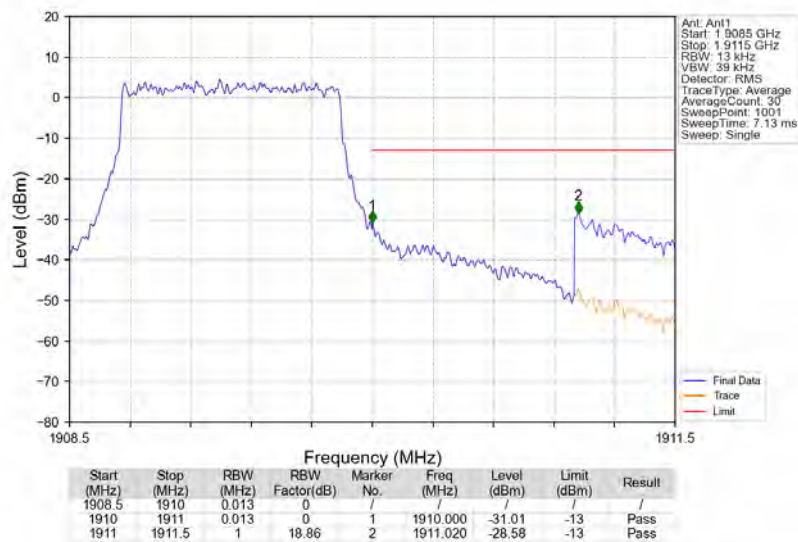
Band2_1.4MHz_QPSK_HCH_1909.3MHz_RB_6_0_NTNV
