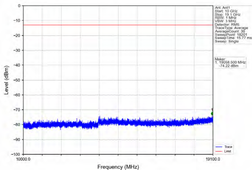
Band2_1.4MHz_16QAM_HCH_1909.3MHz_RB_1_0_NTNV
