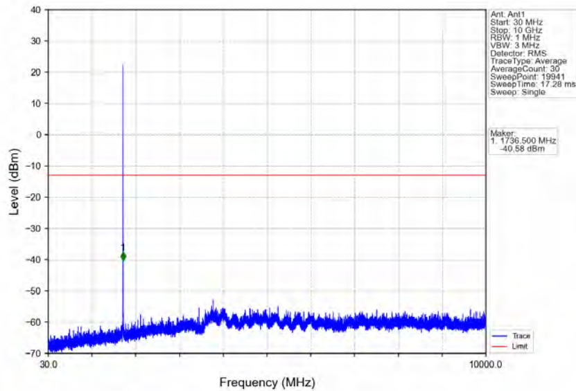
Band4_1.4MHz_16QAM_MCH_1732.5MHz_RB_1_0_NTNV
