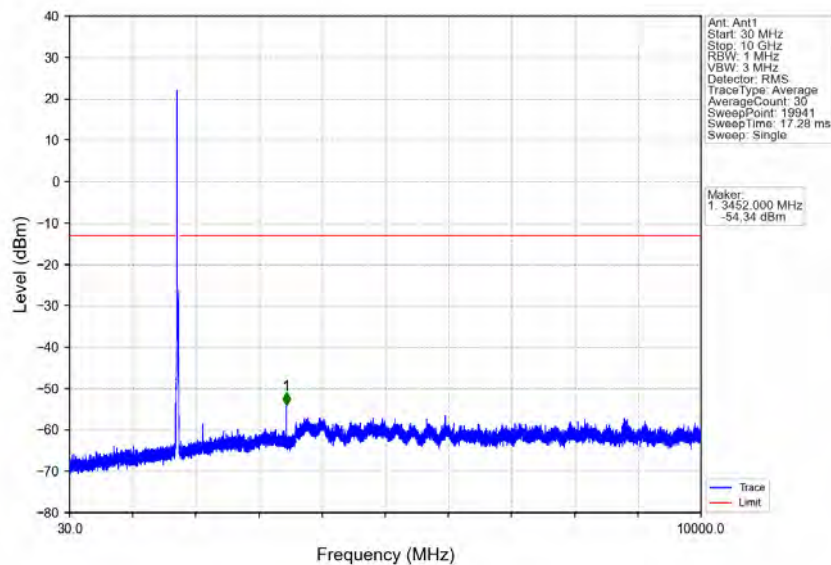
Band4_15MHz_QPSK_MCH_1732.5MHz_RB_1_0_NTNV
