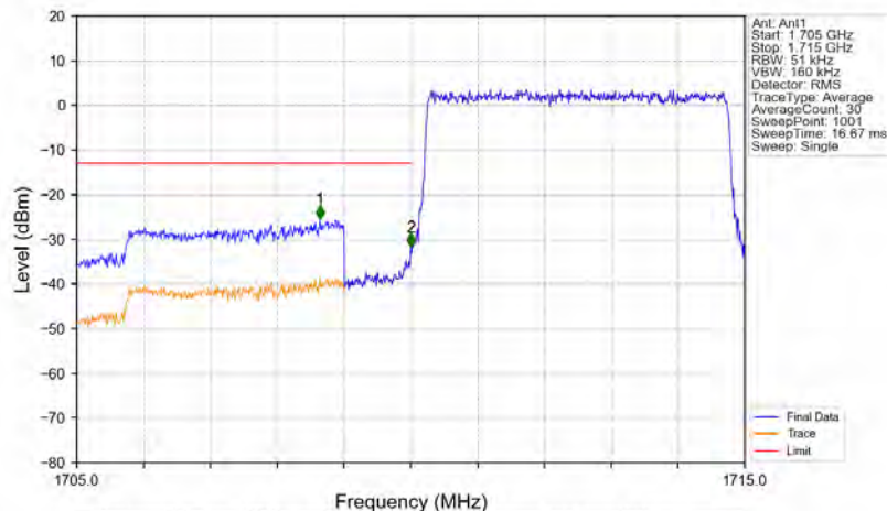
Band4_5MHz_QPSK_LCH_1712.5MHz_RB_25_0_NTNV
