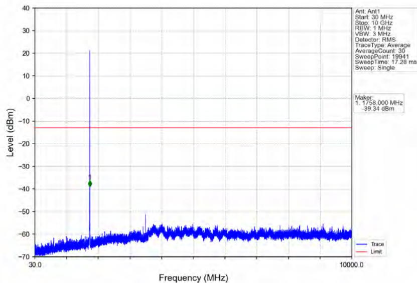
Band4_1.4MHz_16QAM_HCH_1754.3MHz_RB_1_0_NTNV
