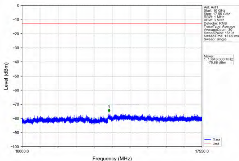
Band4_5MHz_16QAM_HCH_1752.5MHz_RB_1_0_NTNV
