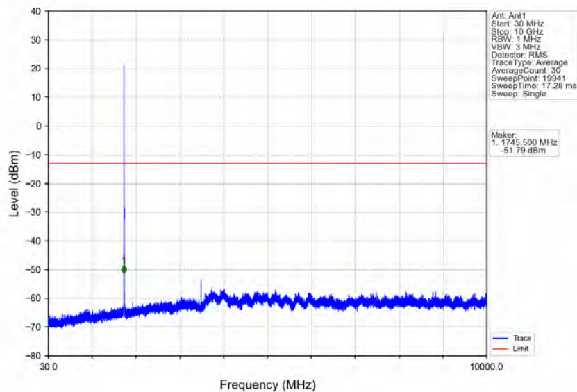
Band4_3MHz_16QAM_HCH_1753.5MHz_RB_1_0_NTNV
