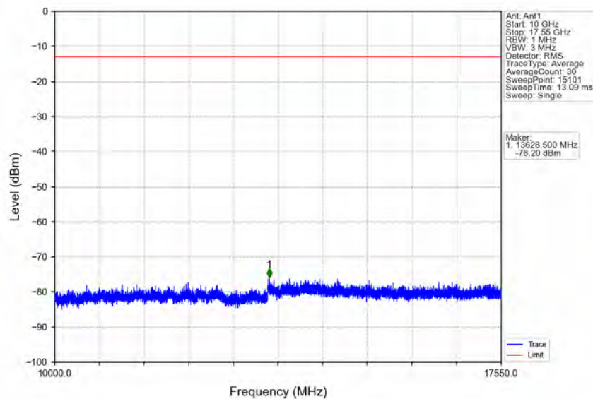
Band4_15MHz_QPSK_LCH_1717.5MHz_RB_75_0_NTNV
