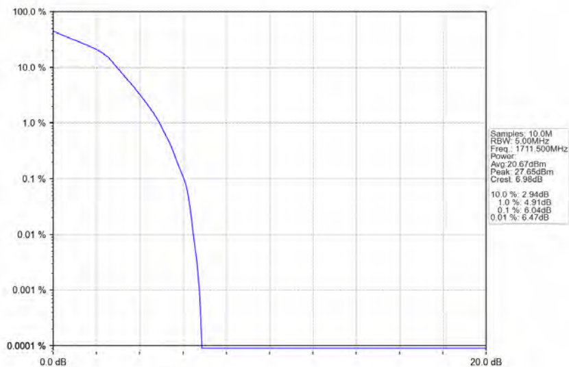
Band4_3MHz_16QAM_LCH_1711.5MHz_RB_15_0_NTNV
