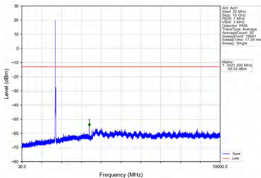
Band4_15MHz_16QAM_LCH_1717.5MHz_RB_1_0_NTNV
