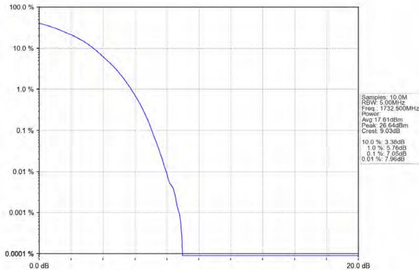
Band4_15MHz_16QAM_MCH_1732.5MHz_RB_75_0_NTNV
