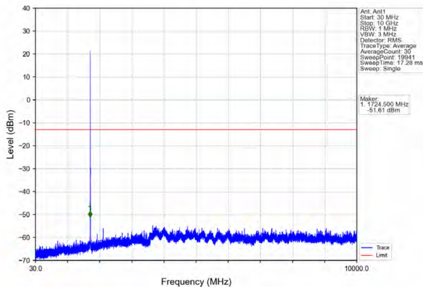
Band4_3MHz_16QAM_MCH_1732.5MHz_RB_1_0_NTNV
