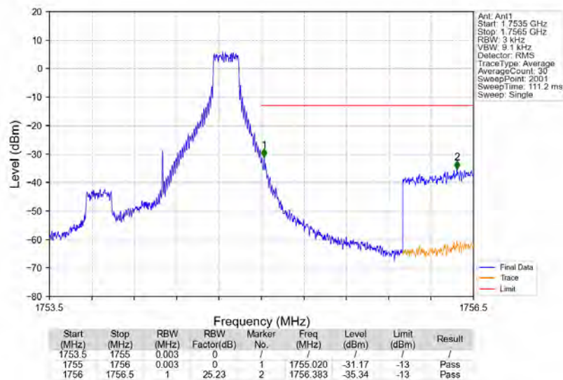
Band4 1.4MHz 16QAM HCH 1754.3MHz RB 1 5 NTNV
