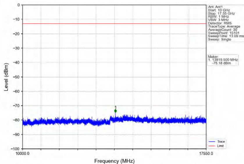
Band4_5MHz_QPSK_HCH_1752.5MHz_RB_1_0_NTNV
