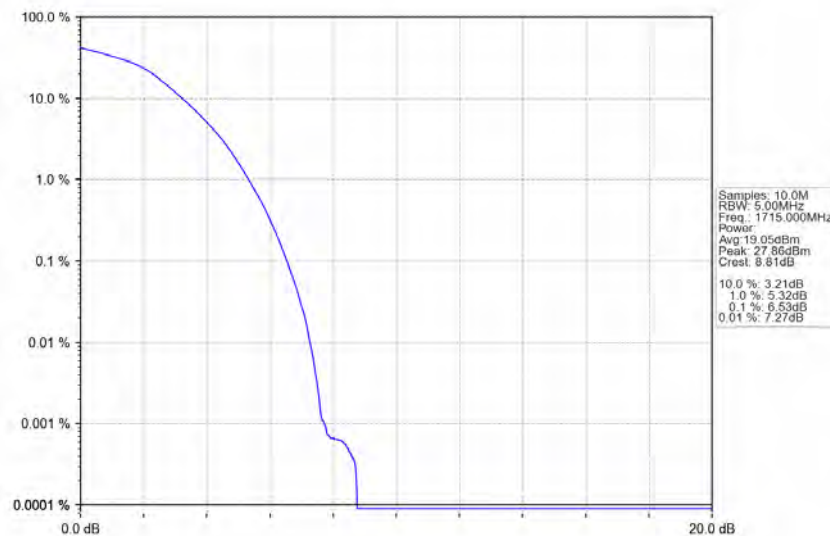
Band4_10MHz_16QAM_LCH_1715MHz_RB_50_0_NTNV
