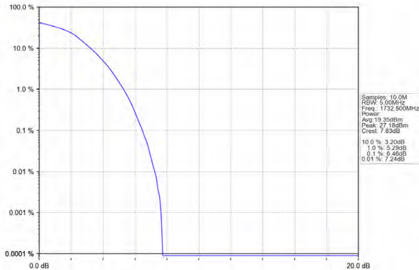
Band4_10MHz_16QAM_MCH_1732.5MHz_RB_50_0_NTNV
