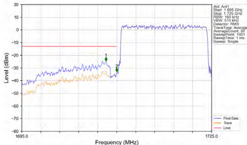
Band4_15MHz_QPSK_LCH_1717.5MHz_RB_75_0_NTNV
