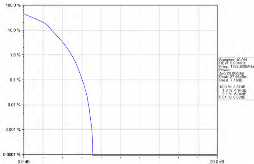
Band4_5MHz_16QAM_HCH_1752.5MHz_RB_25_0_NTNV
