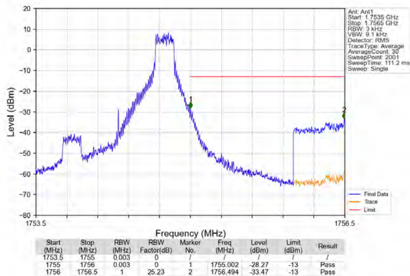
Band4_1.4MHz_QPSK_HCH_1754.3MHz_RB_1_5_NTNV
