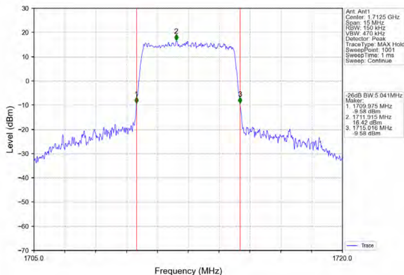
Band4_5MHz_16QAM_LCH_1712.5MHz_RB_25_0_NTNV
