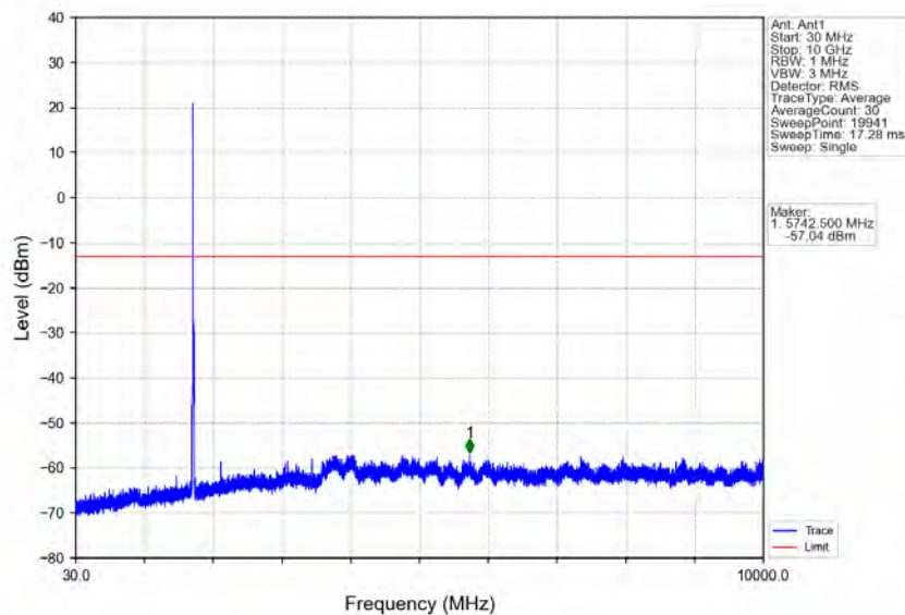
Band4_10MHz_16QAM_MCH_1732.5MHz_RB_1_0_NTNV
