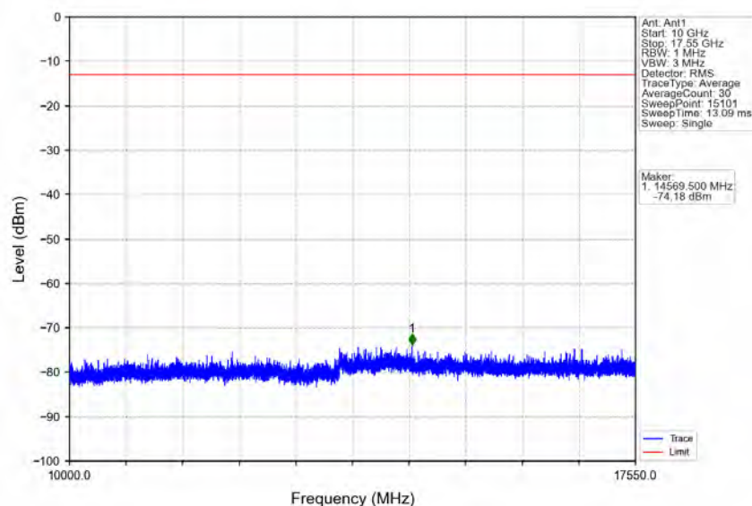
Band4 1.4MHz QPSK HCH 1754.3MHz RB 1 0 NTN
