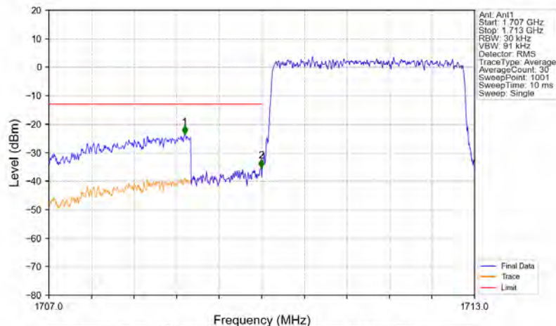
Band4_3MHz_16QAM_LCH_1711.5MHz_RB_15_0_NTNV
