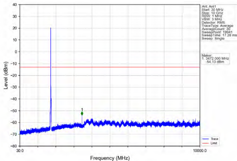
Band4_20MHz_16QAM_HCH_1745MHz_RB_1_0_NTNV
