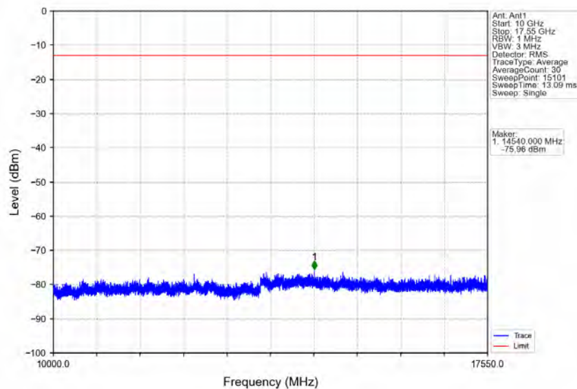
Band4_10MHz_16QAM_LCH_1715MHz_RB_50_0_NTNV
