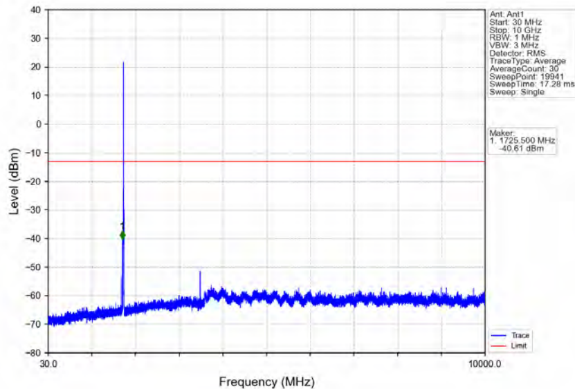
Band4_5MHz_QPSK_HCH_1752.5MHz_RB_1_0_NTNV
