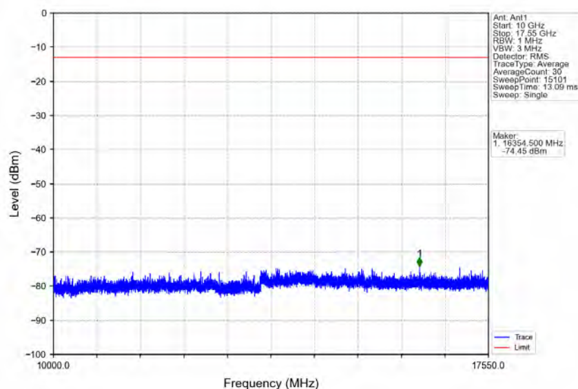
Band4_1.4MHz_16QAM_HCH_1754.3MHz_RB_1_0_NTNV
