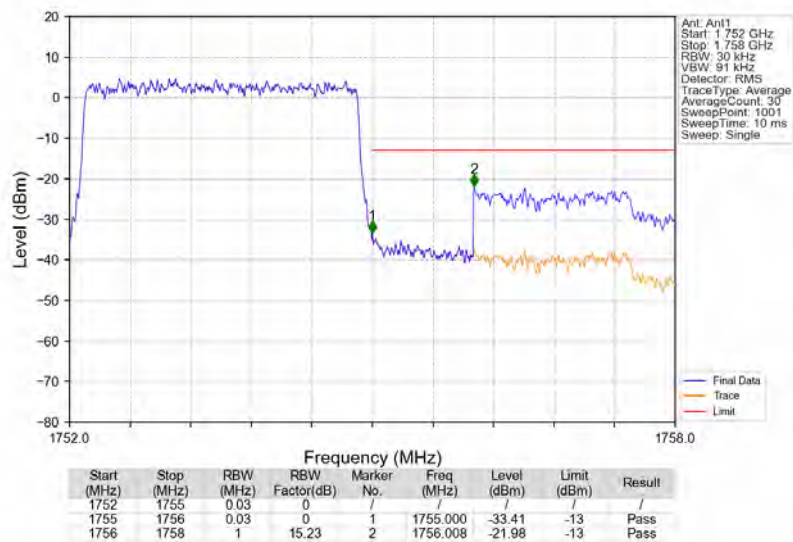
Band4_3MHz_QPSK_HCH_1753.5MHz_RB_15_0_NTNV
