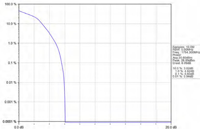
Band4_1.4MHz_16QAM_HCH_1754.3MHz_RB_6_0_NTNV
