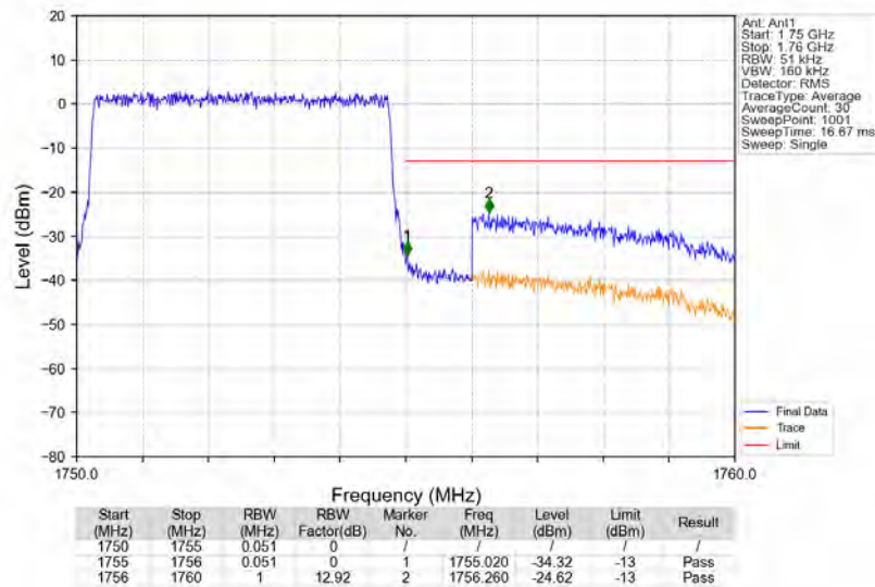
Band4_5MHz_16QAM_HCH_1752.5MHz_RB_25_0_NTNV
