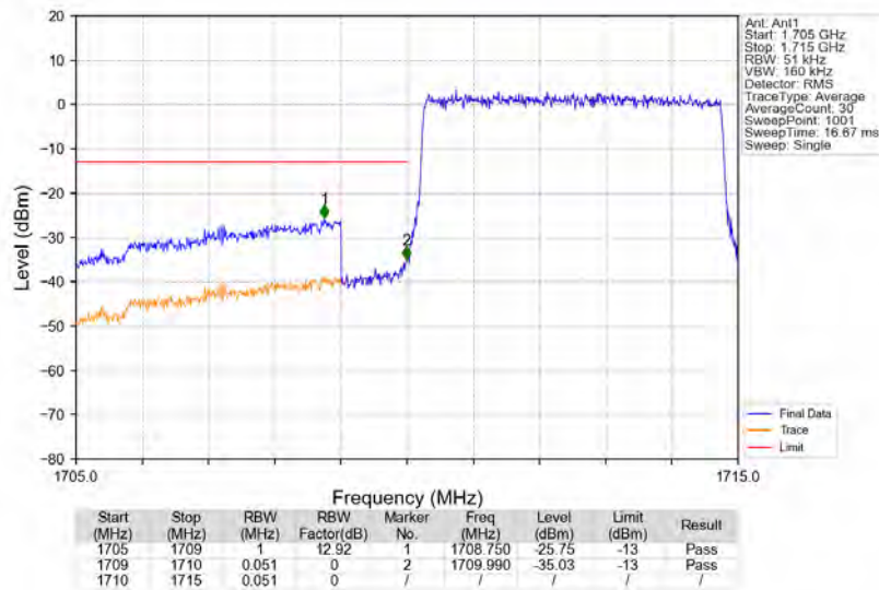
Band4_5MHz_16QAM_LCH_1712.5MHz_RB_25_0_NTNV
