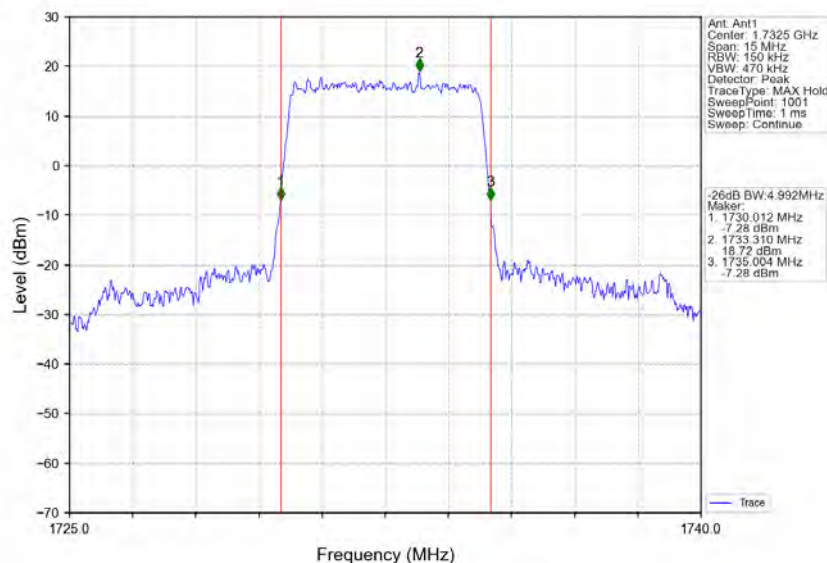
Band4_5MHz_QPSK_MCH_1732.5MHz_RB_25_0_NTNV
