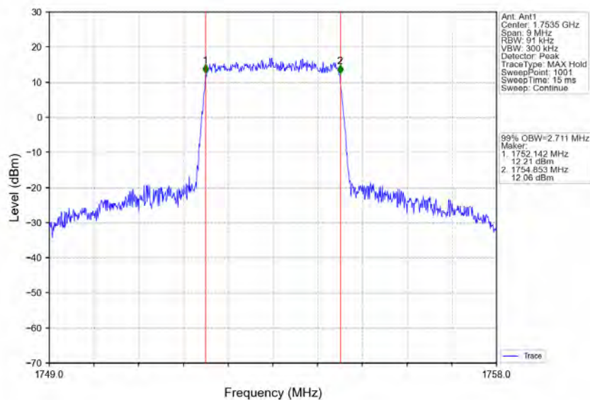
Band4_3MHz_16QAM_HCH_1753.5MHz_RB_15_0_NTNV
