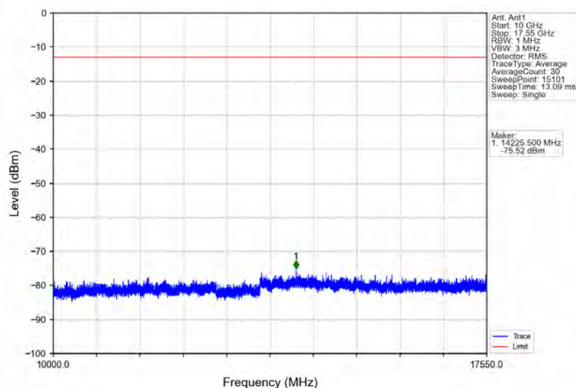
Band4_15MHz_16QAM_HCH_1747.5MHz_RB_1_0_NTNV
