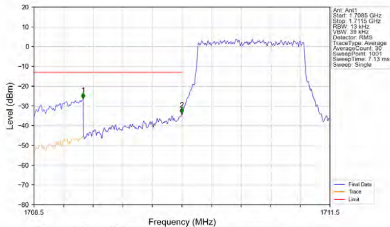
Band4_1.4MHz_16QAM_LCH_1710.7MHz_RB_6_0_NTNV
