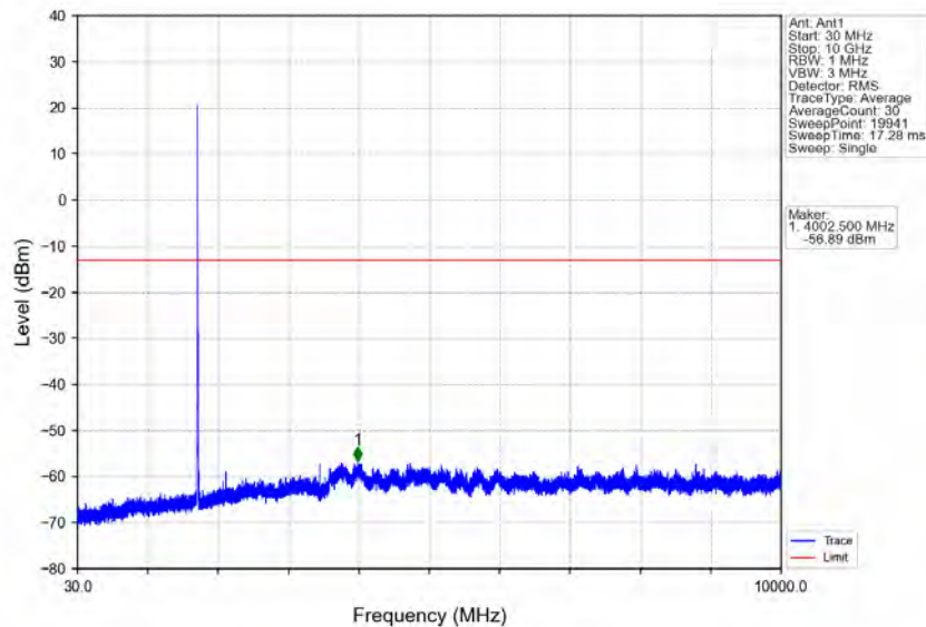
Band4_5MHz_16QAM_MCH_1732.5MHz_RB_1_0_NTNV
