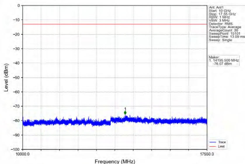
Band4_5MHz_QPSK_MCH_1732.5MHz_RB_1_0_NTNV
