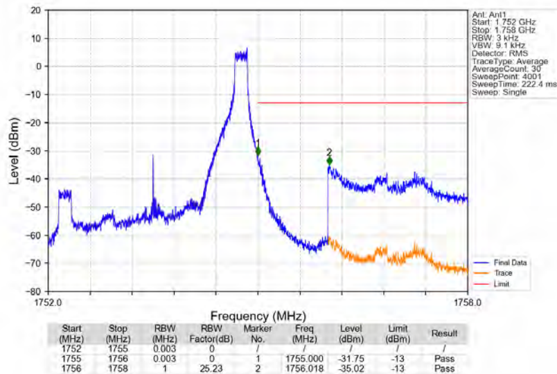
Band4_3MHz_16QAM_HCH_1753.5MHz_RB_1_14_NTNV
