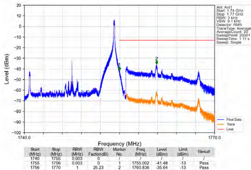
Band4_15MHz_16QAM_HCH_1747.5MHz_RB_1_74_NTNV
