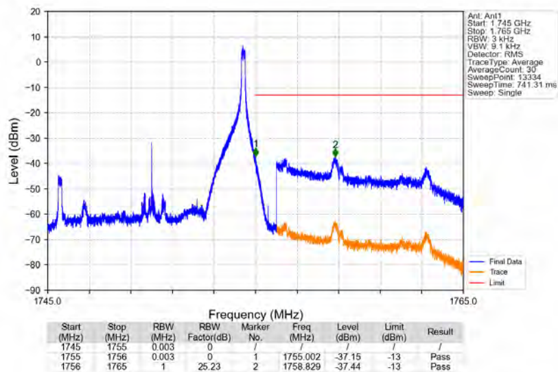
Band4_10MHz_16QAM_HCH_1750MHz_RB_1_49_NTNV
