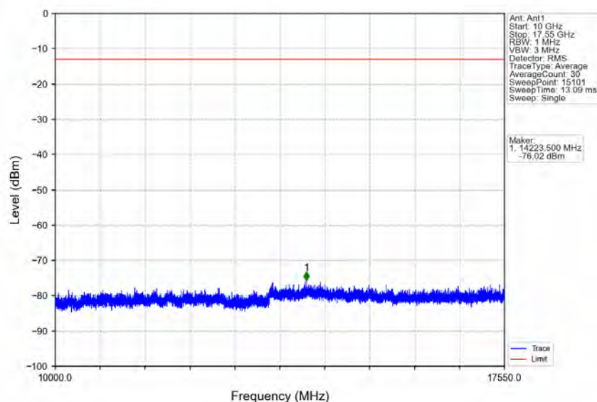
Band4_20MHz_16QAM_MCH_1732.5MHz_RB_1_0_NTNV
