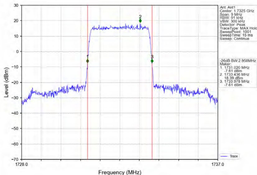
Band4_3MHz_QPSK_MCH_1732.5MHz_RB_15_0_NTNV
