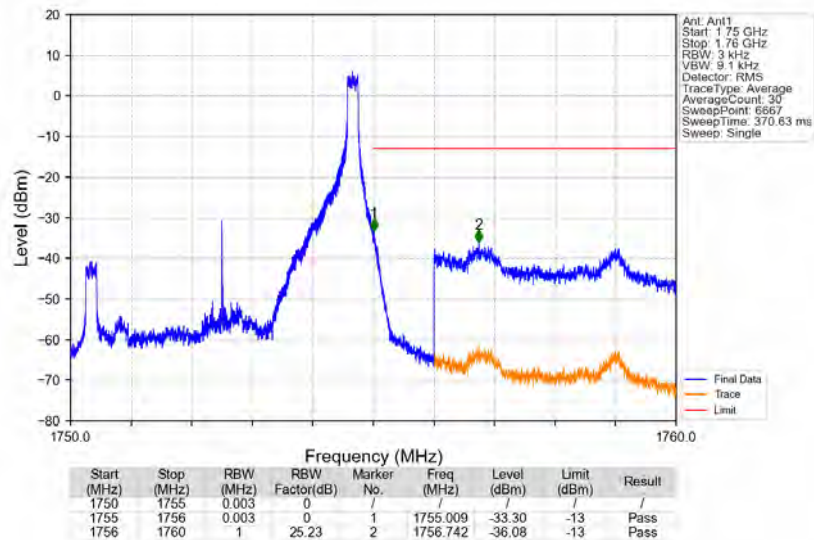
Band4_5MHz_16QAM_HCH_1752.5MHz_RB_1_24_NTNV
