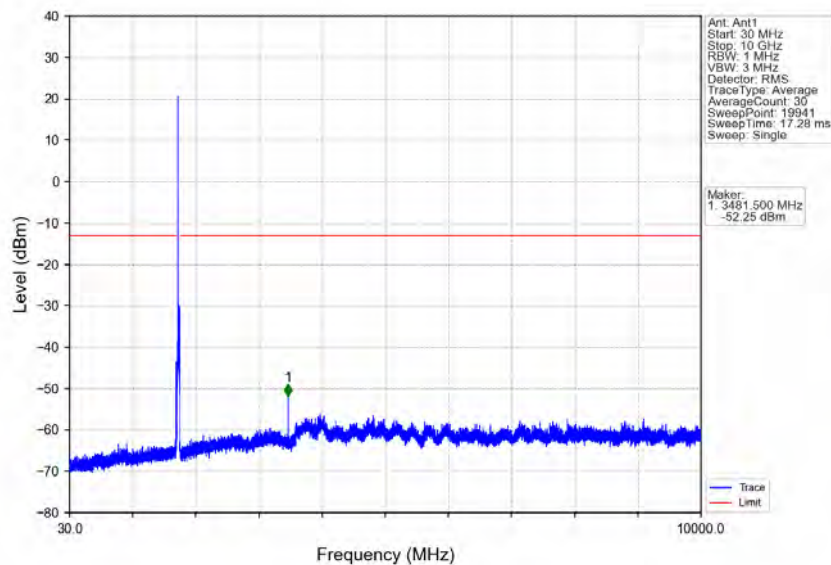
Band4_15MHz_QPSK_HCH_1747.5MHz_RB_1_0_NTNV
