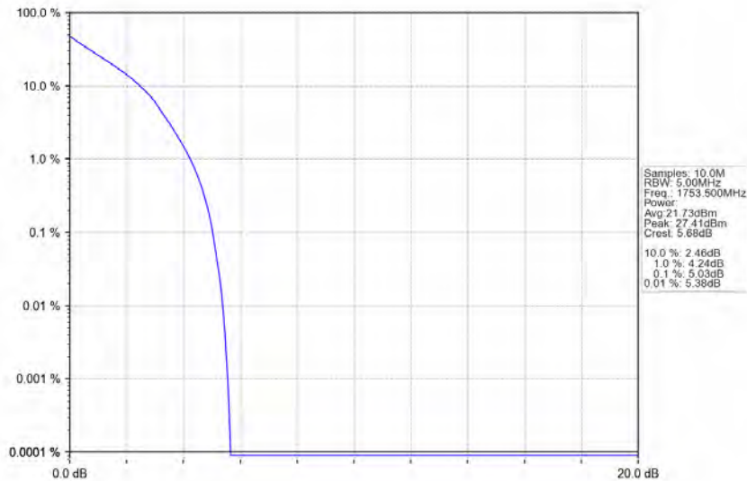
Band4_3MHz_QPSK_HCH_1753.5MHz_RB_15_0_NTNV
