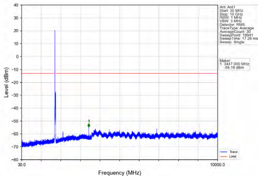
Band4_20MHz_16QAM_MCH_1732.5MHz_RB_1_0_NTNV
