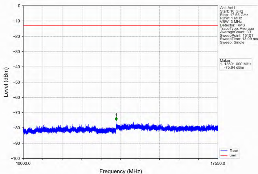
Band4_10MHz_16QAM_HCH_1750MHz_RB_1_0_NTNV
