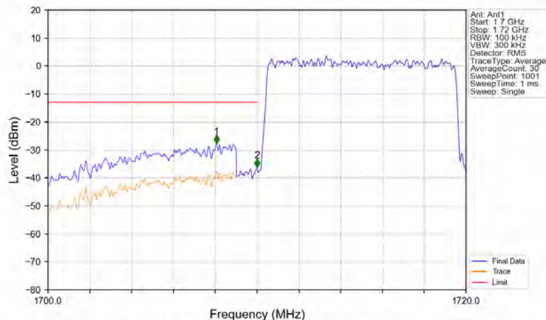
Band4_10MHz_16QAM_LCH_1715MHz_RB_50_0_NTNV
