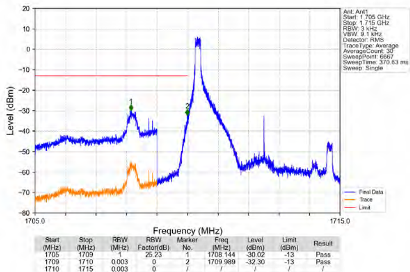
Band4_5MHz_16QAM_LCH_1712.5MHz_RB_1_0_NTNV
