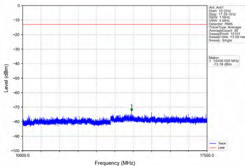
Band4_3MHz_QPSK_HCH_1753.5MHz_RB_1_0_NTNV
