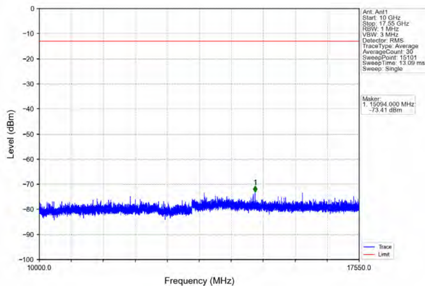
Band4_1.4MHz_16QAM_MCH_1732.5MHz_RB_1_0_NTNV
