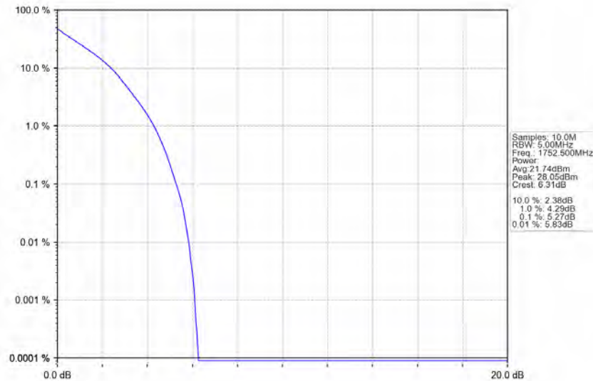
Band4_5MHz_QPSK_HCH_1752.5MHz_RB_25_0_NTNV
