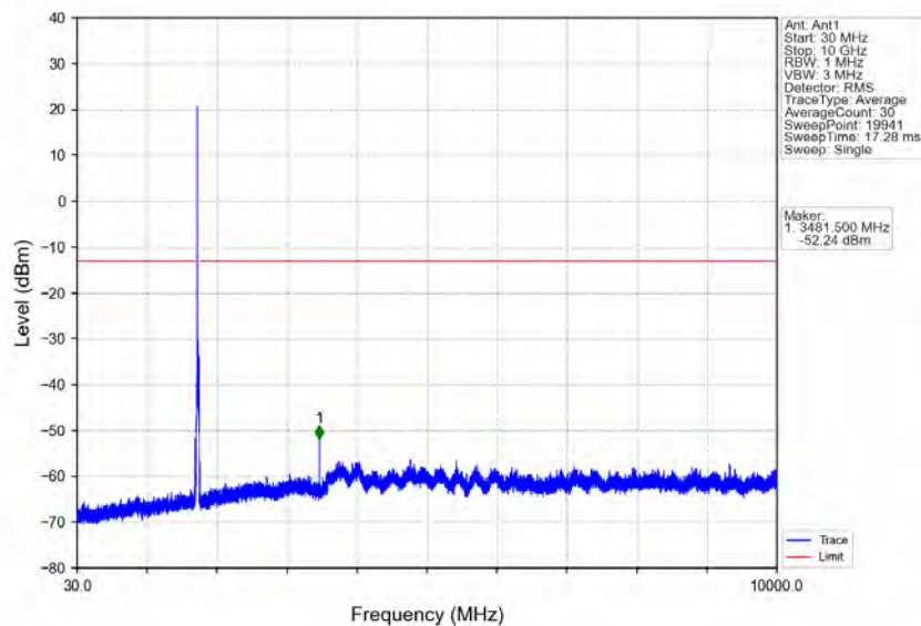
Band4_15MHz_16QAM_HCH_1747.5MHz_RB_1_0_NTNV
