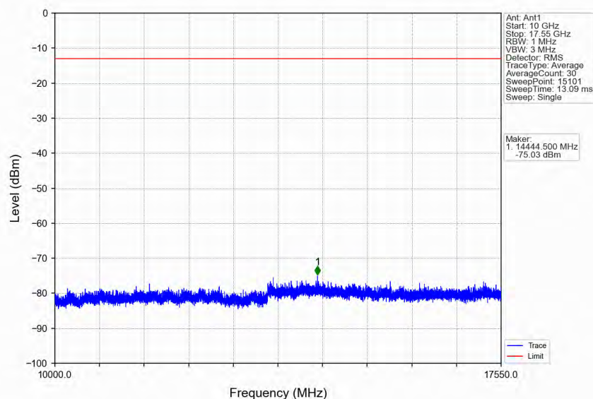
Band4_20MHz_16QAM_HCH_1745MHz_RB_1_0_NTNV
