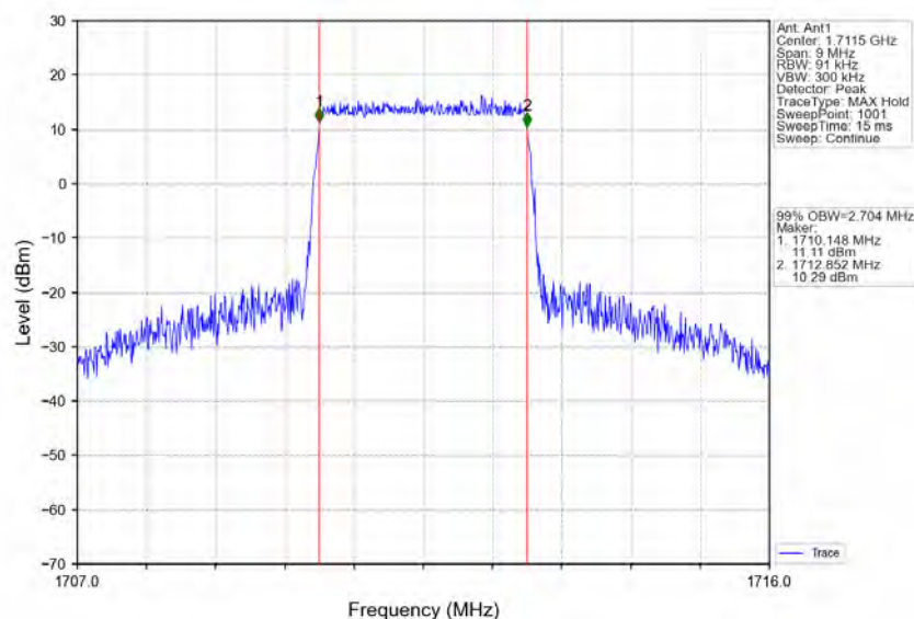
Band4_3MHz_16QAM_LCH_1711.5MHz_RB_15_0_NTNV
