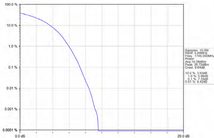
Band4_20MHz_16QAM_HCH_1745MHz_RB_100_0_NTNV
