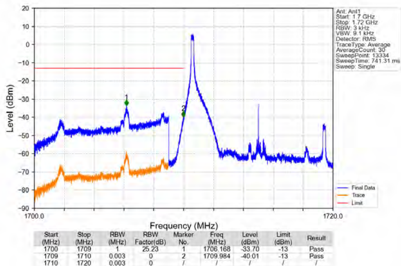
Band4_10MHz_16QAM_LCH_1715MHz_RB_1_0_NTNV
