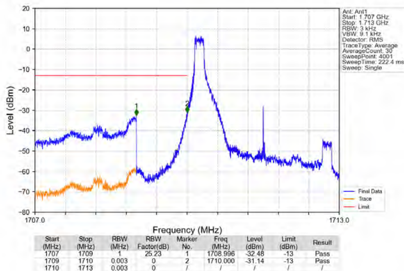
Band4_3MHz_16QAM_LCH_1711.5MHz_RB_1_0_NTNV
