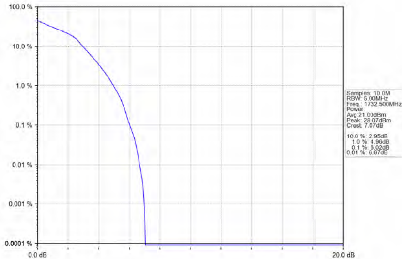
Band4_3MHz_16QAM_MCH_1732.5MHz_RB_15_0_NTNV
