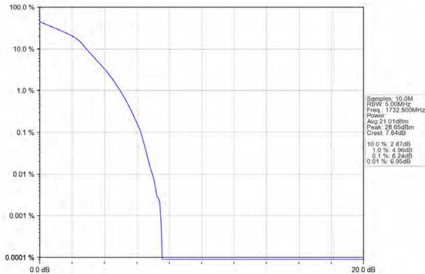
Band4_5MHz_16QAM_MCH_1732.5MHz_RB_25_0_NTNV
