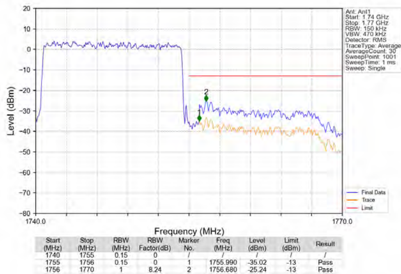
Band4_15MHz_QPSK_HCH_1747.5MHz_RB_75_0_NTNV
