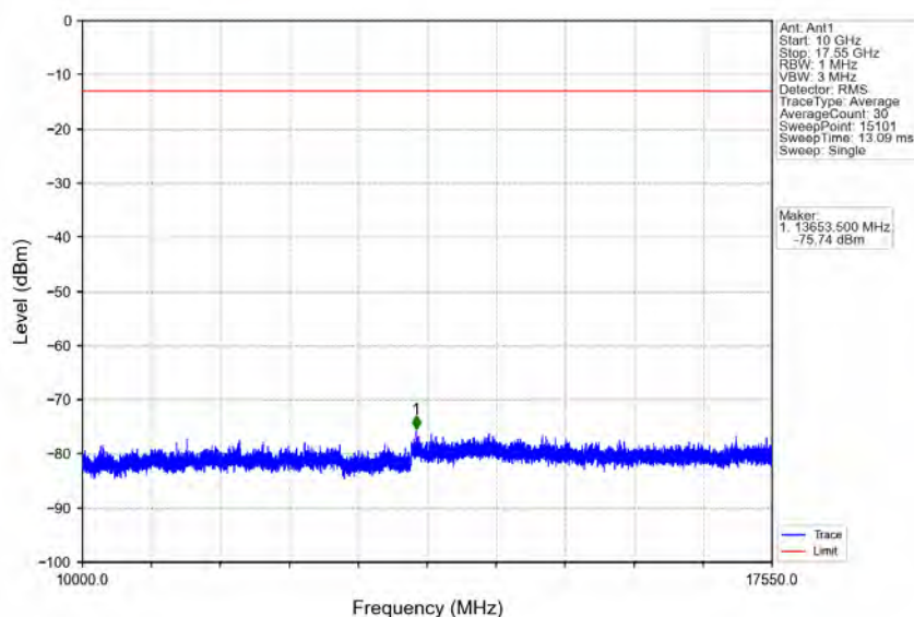
Band4_10MHz_16QAM_MCH_1732.5MHz_RB_1_0_NTNV
