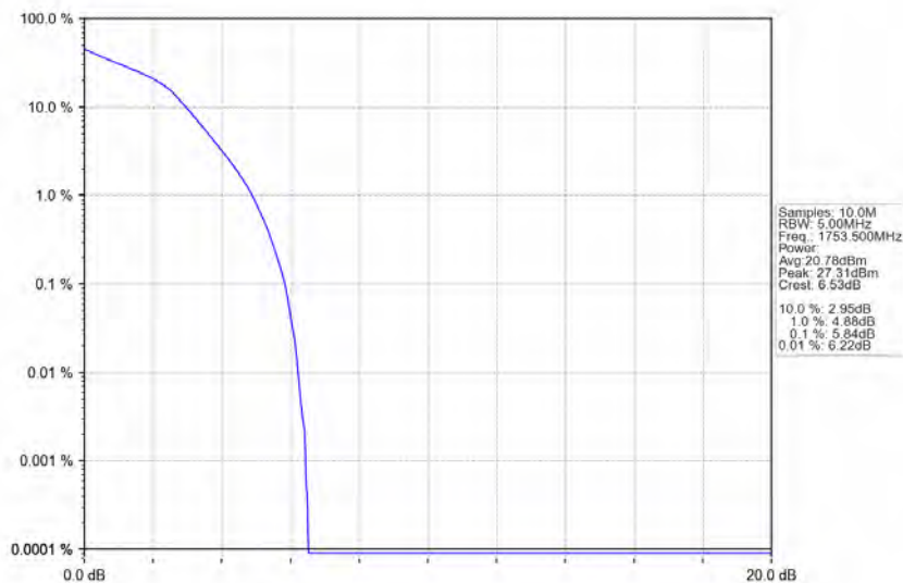
Band4_3MHz_16QAM_HCH_1753.5MHz_RB_15_0_NTNV
