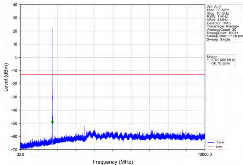
Band4_3MHz_QPSK_HCH_1753.5MHz_RB_1_0_NTNV
