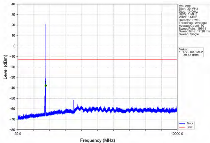
Band4_5MHz_16QAM_HCH_1752.5MHz_RB_1_0_NTNV
