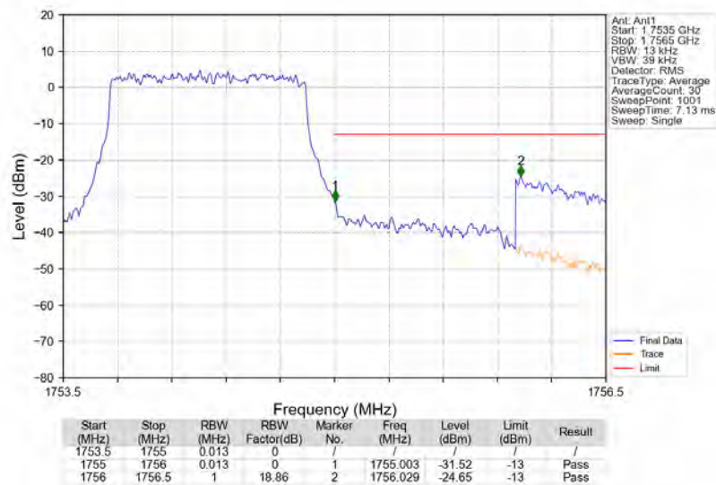
Band4_1.4MHz_QPSK_HCH_1754.3MHz_RB_6_0_NTNV
