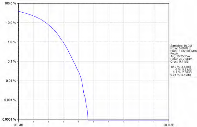
Band4_20MHz_16QAM_MCH_1732.5MHz_RB_100_0_NTNV
