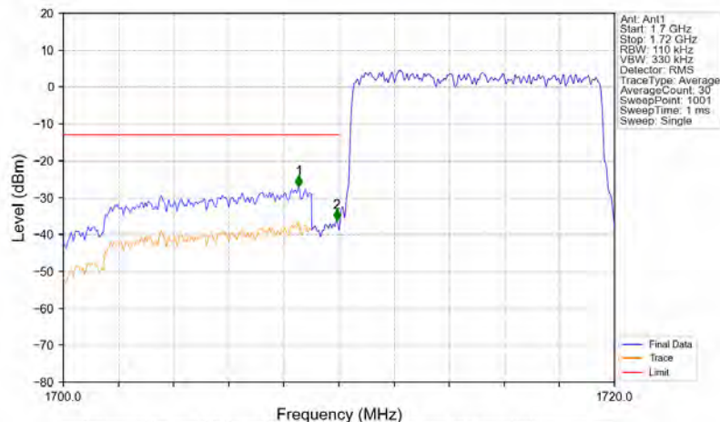
Band4_10MHz_QPSK_LCH_1715MHz_RB_50_0_NTNV
