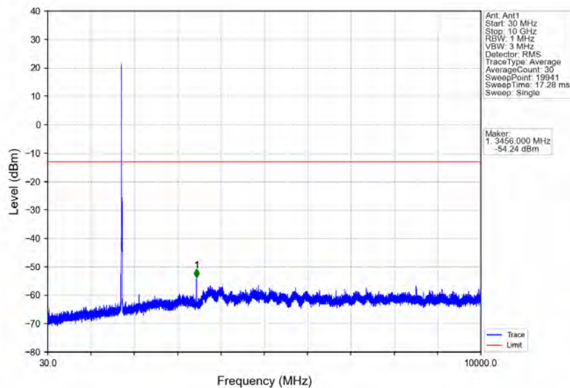
Band4_10MHz_QPSK_MCH_1732.5MHz_RB_1_0_NTNV
