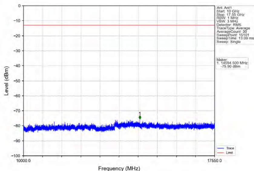
Band4_15MHz_QPSK_MCH_1732.5MHz_RB_1_0_NTNV
