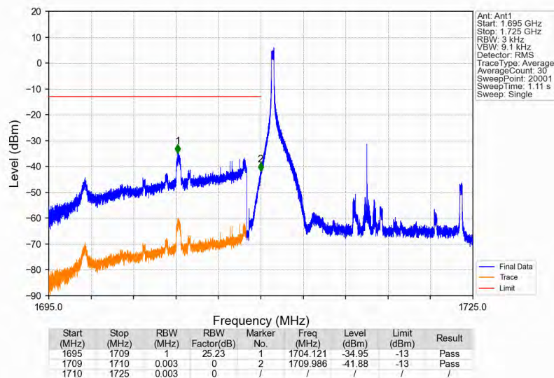
Band4_15MHz_16QAM_LCH_1717.5MHz_RB_1_0_NTNV
