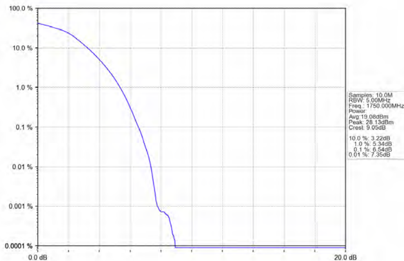
Band4_10MHz_16QAM_HCH_1750MHz_RB_50_0_NTNV
