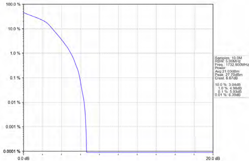
Band4_1.4MHz_16QAM_MCH_1732.5MHz_RB_6_0_NTNV
