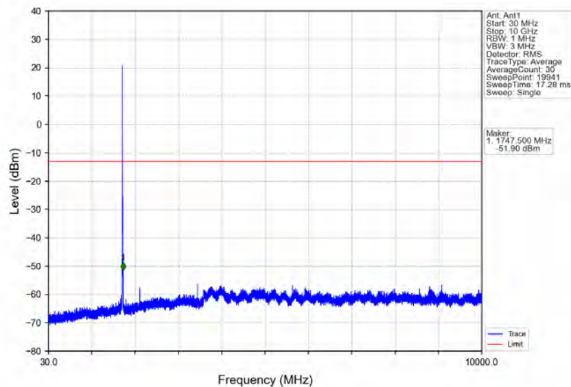
Band4_5MHz_QPSK_MCH_1732.5MHz_RB_1_0_NTNV
