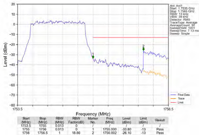
Band4 1.4MHz 16QAM HCH 1754.3MHz RB 6 0 NTNV
