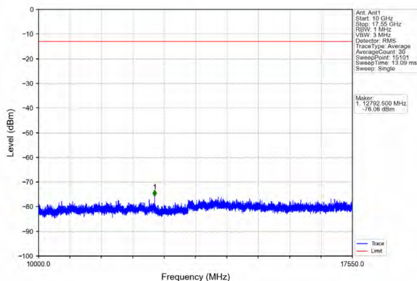
Band4_3MHz_16QAM_HCH_1753.5MHz_RB_1_0_NTNV
