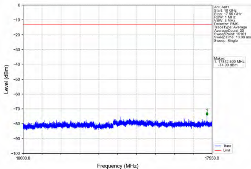
Band4_5MHz_16QAM_MCH_1732.5MHz_RB_1_0_NTNV
