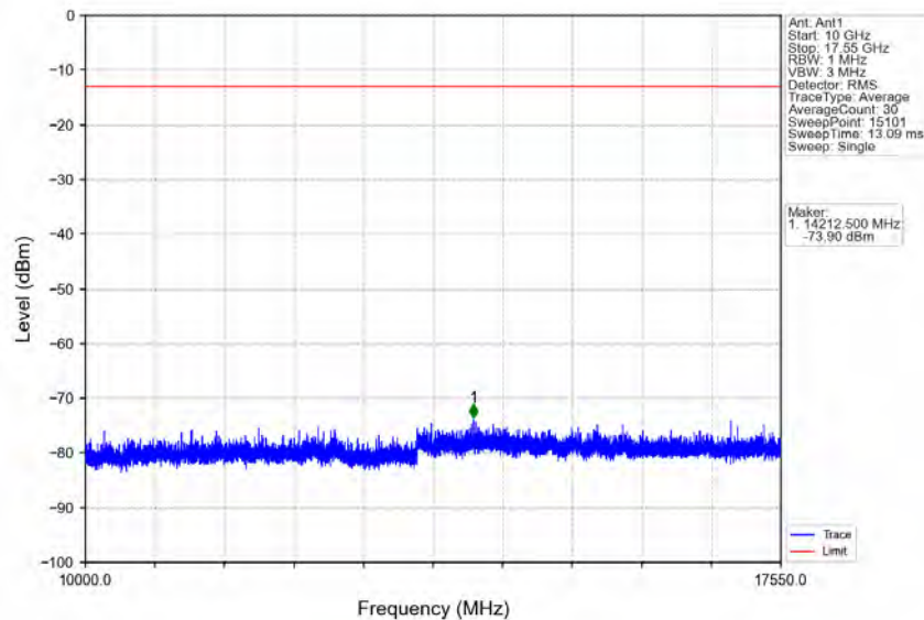
Band4_1.4MHz_16QAM_LCH_1710.7MHz_RB_6_0_NTNV
