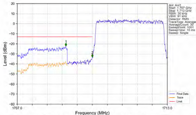
Band4_3MHz_QPSK_LCH_1711.5MHz_RB_15_0_NTNV
