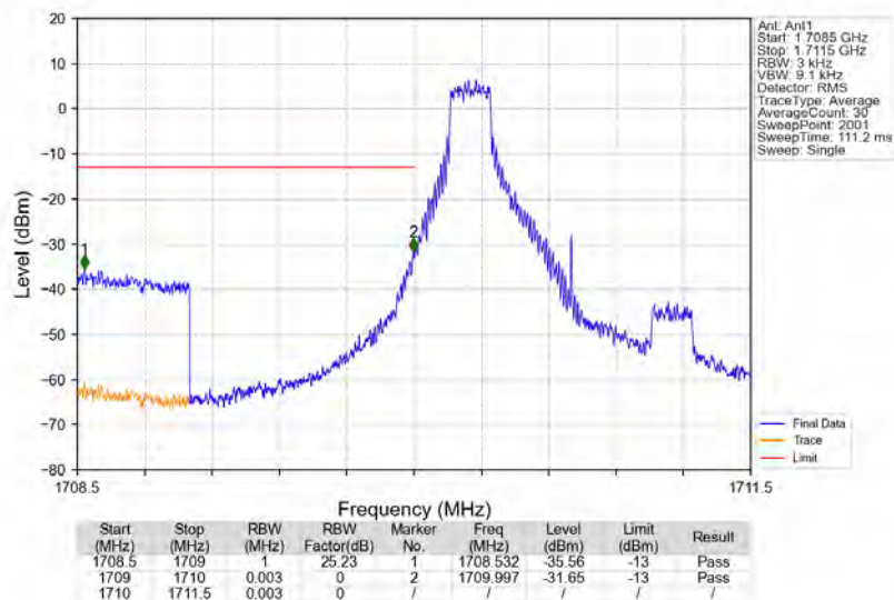
Band4_1.4MHz_16QAM_LCH_1710.7MHz_RB_1_0_NTNV
