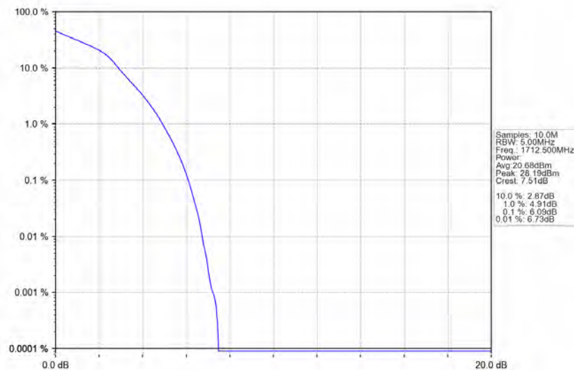
Band4_5MHz_16QAM_LCH_1712.5MHz_RB_25_0_NTNV
