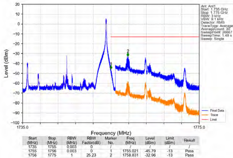
Band4_20MHz_16QAM_HCH_1745MHz_RB_1_99_NTNV
