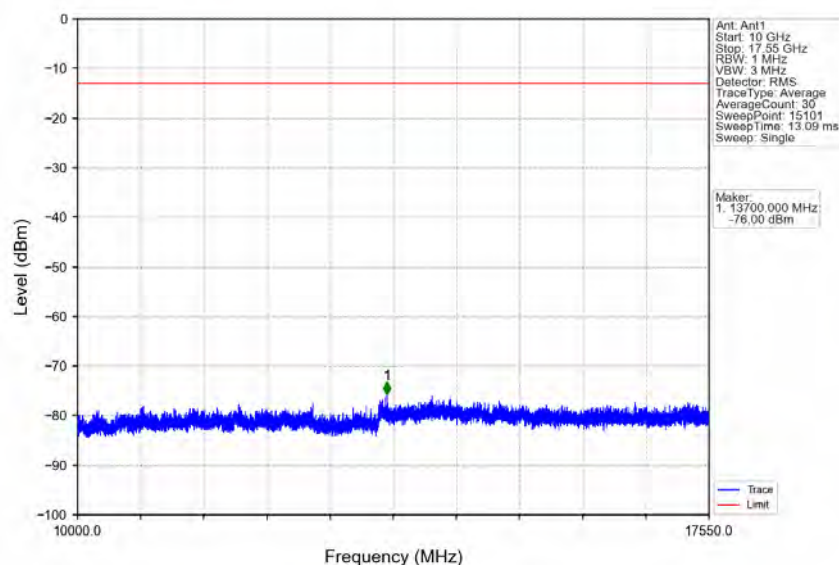
Band4_10MHz_QPSK_MCH_1732.5MHz_RB_1_0_NTNV
