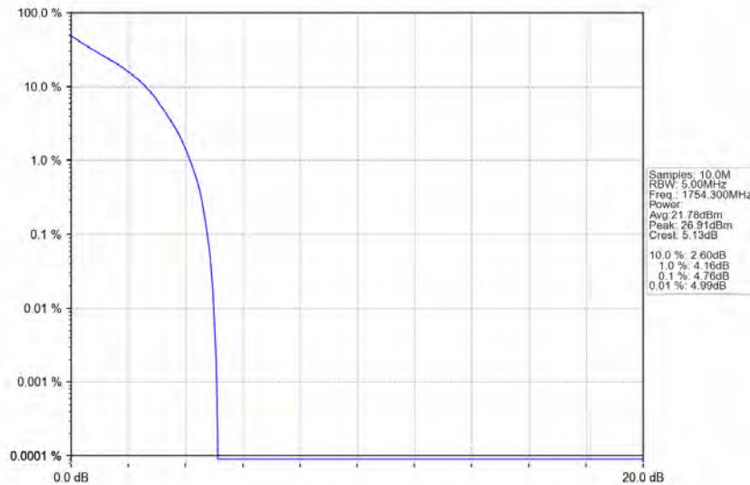
Band4 1.4MHz QPSK HCH 1754.3MHz RB 6 0 NTNV
