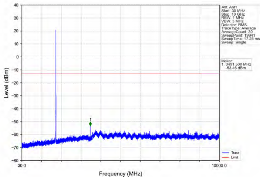
Band4_10MHz_16QAM_HCH_1750MHz_RB_1_0_NTNV
