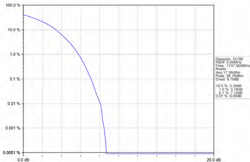
Band4_15MHz_16QAM_HCH_1747.5MHz_RB_75_0_NTNV
