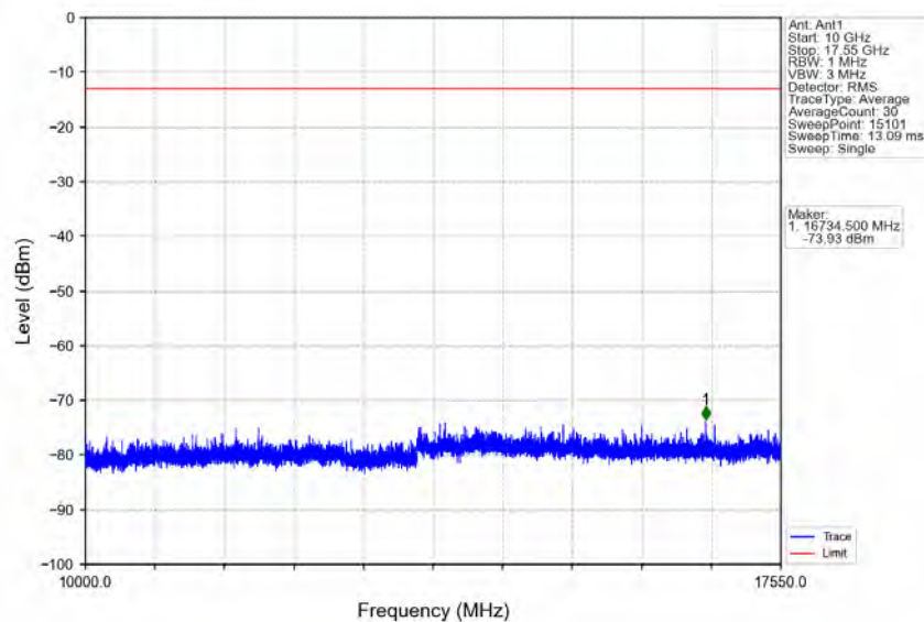
Band4_3MHz_16QAM_LCH_1711.5MHz_RB_15_0_NTNV
