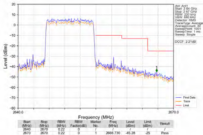
Band41_10MHz_16QAM_HCH_2650MHz_RB_50_0_NTNV
