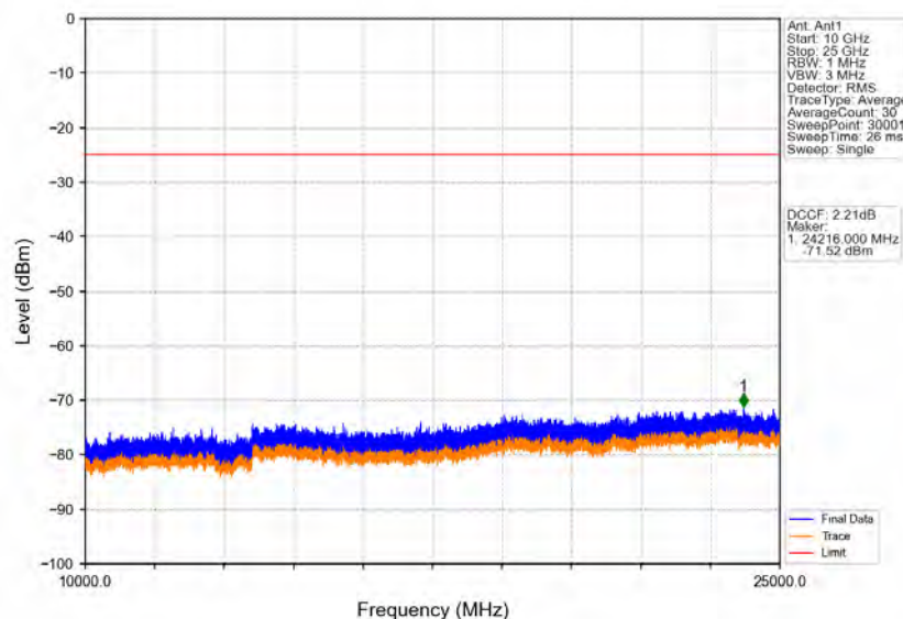
Band41_15MHz_16QAM_LCH_2542.5MHz_RB_1_0_NTNV
