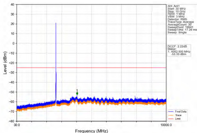
Band41_15MHz_16QAM_HCH_2647.5MHz_RB_1_0_NTNV
