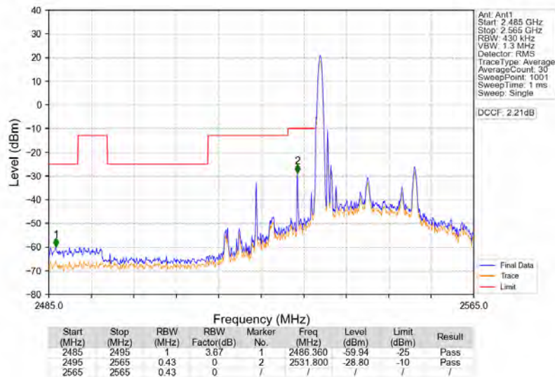
Band41_20MHz_16QAM_LCH_2545MHz_RB_1_0_NTNV
