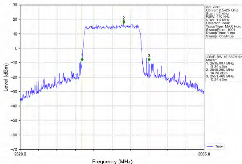
Band41_15MHz_16QAM_LCH_2542.5MHz_RB_75_0_NTNV
