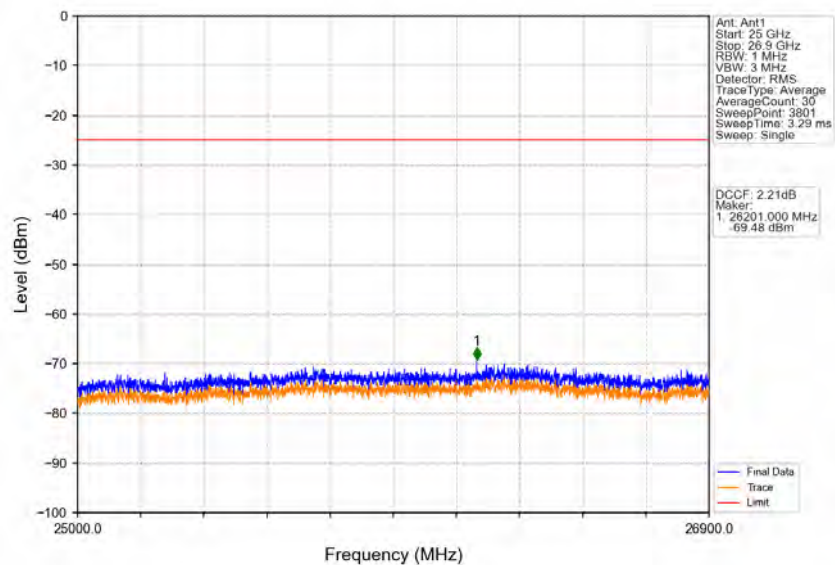
Band41_20MHz_16QAM_HCH_2645MHz_RB_1_0_NTNV
