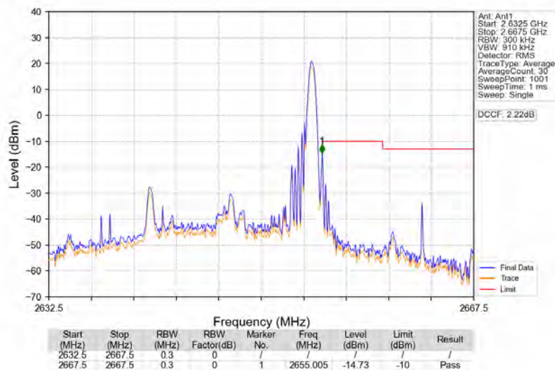
Band41_15MHz_16QAM_HCH_2647.5MHz_RB_1_74_NTNV
