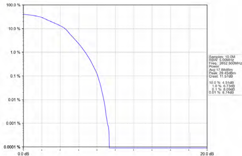
Band41_5MHz_16QAM_HCH_2652.5MHz_RB_25_0_NTNV
