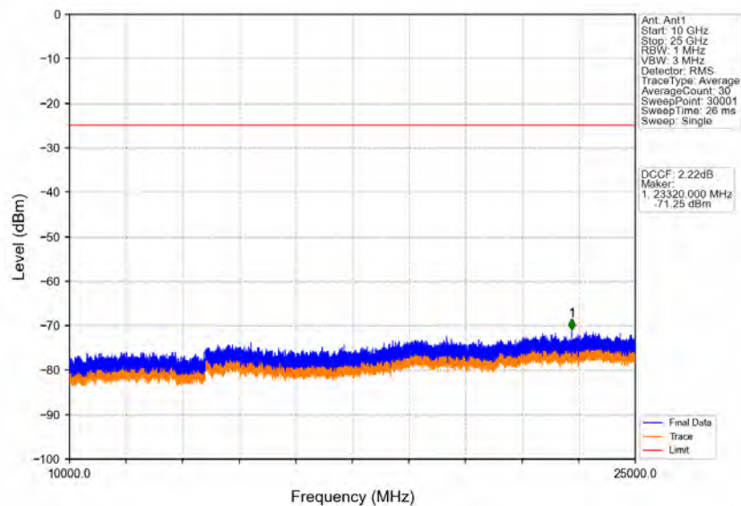
Band41_15MHz_16QAM_HCH_2647.5MHz_RB_1_0_NTNV
