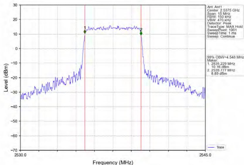
Band41_5MHz_16QAM_LCH_2537.5MHz_RB_25_0_NTNV
