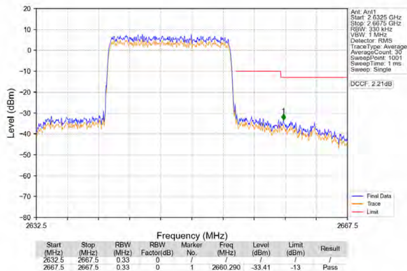
Band41_15MHz_QPSK_HCH_2647.5MHz_RB_75_0_NTNV
