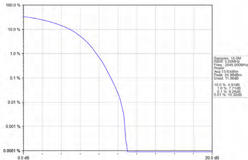
Band41_20MHz_16QAM_LCH_2545MHz_RB_100_0_NTNV
