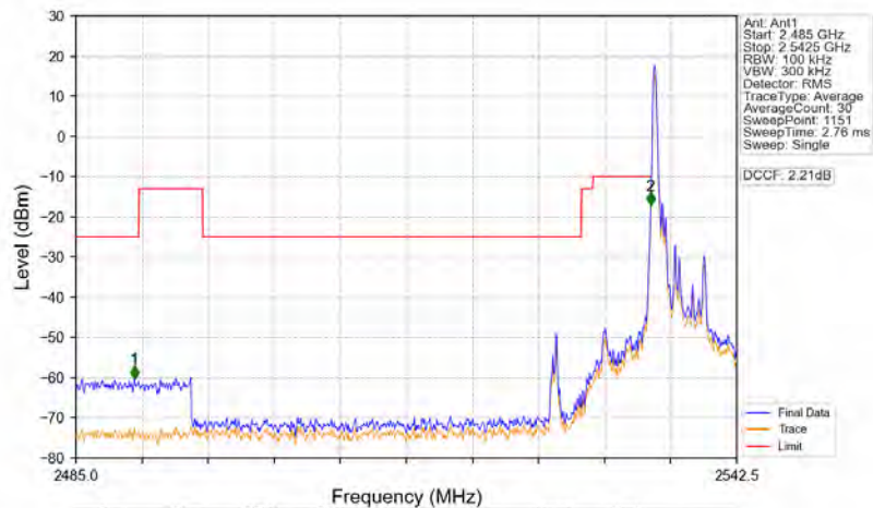
Band41_5MHz_16QAM_LCH_2537.5MHz_RB_1_0_NTNV
