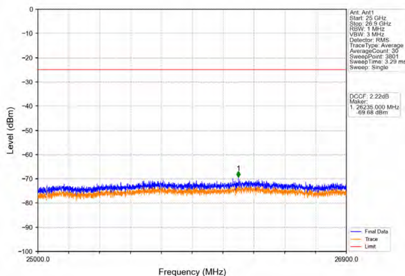
Band41_10MHz_16QAM_HCH_2650MHz_RB_1_0_NTNV
