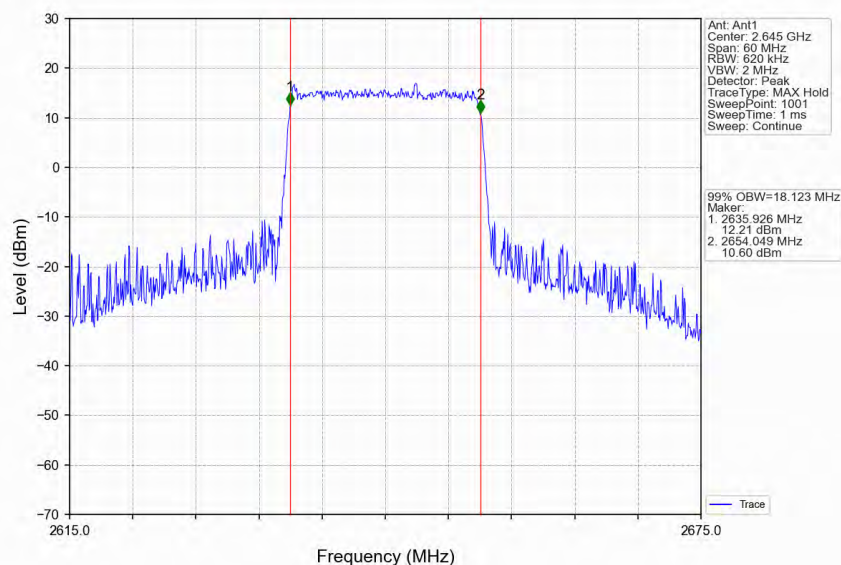
Band41_20MHz_16QAM_HCH_2645MHz_RB_100_0_NTNV
