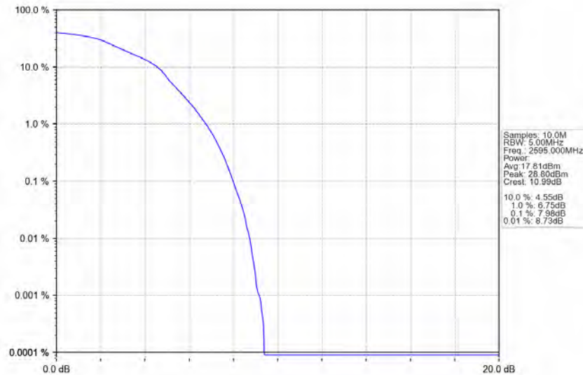
Band41_5MHz_16QAM_MCH_2595MHz_RB_25_0_NTNV
