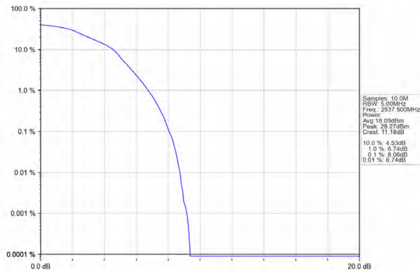
Band41_5MHz_16QAM_LCH_2537.5MHz_RB_25_0_NTNV
