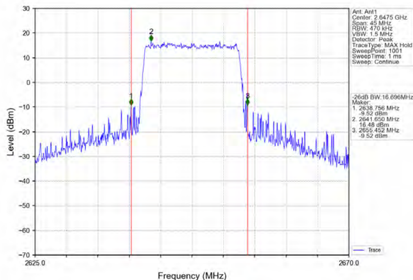
Band41_15MHz_16QAM_HCH_2647.5MHz_RB_75_0_NTNV
