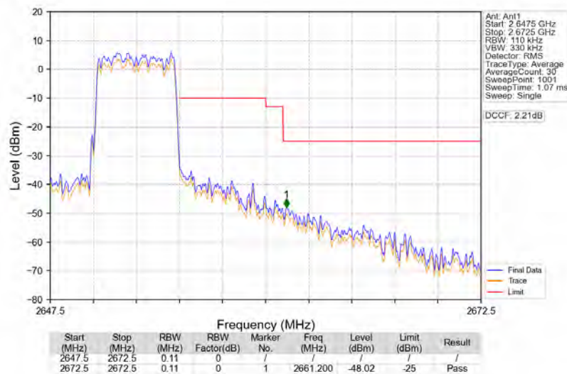
Band41_5MHz_16QAM_HCH_2652.5MHz_RB_25_0_NTNV
