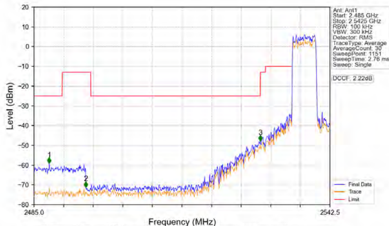
Band41_5MHz_16QAM_LCH_2537.5MHz_RB_25_0_NTNV
