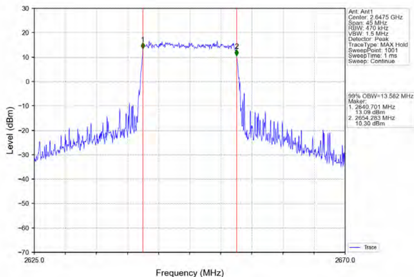
Band41_15MHz_16QAM_HCH_2647.5MHz_RB_75_0_NTNV
