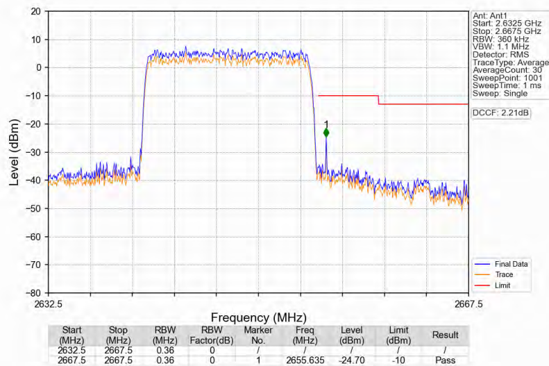
Band41_15MHz_16QAM_HCH_2647.5MHz_RB_75_0_NTNV
