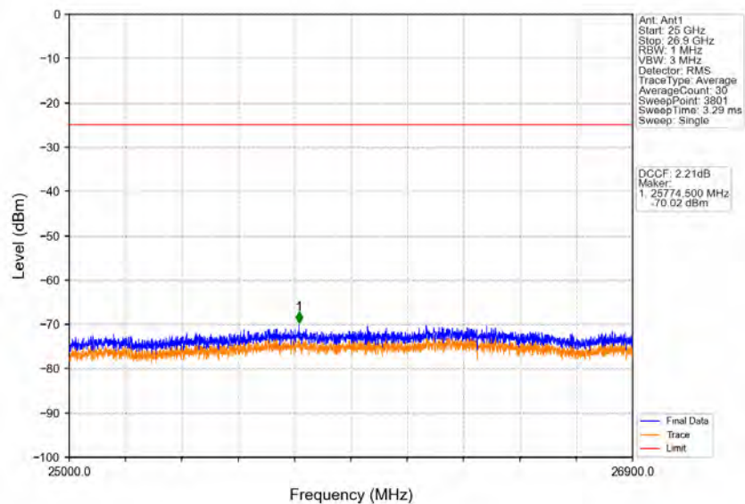
Band41_20MHz_16QAM_LCH_2545MHz_RB_100_0_NTNV
