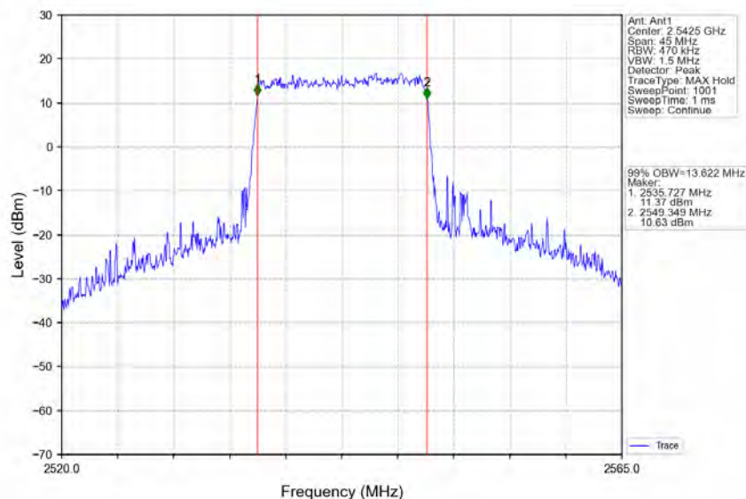
Band41_15MHz_16QAM_LCH_2542.5MHz_RB_75_0_NTNV
