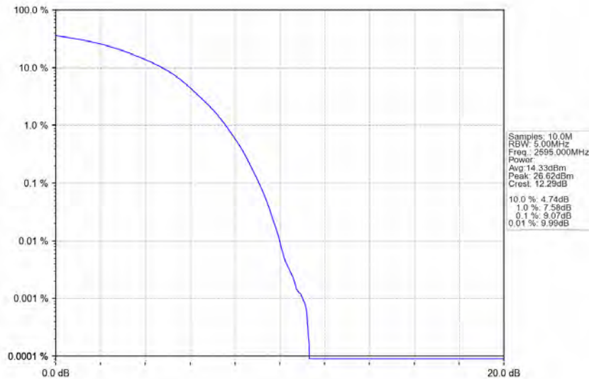
Band41_15MHz_16QAM_MCH_2595MHz_RB_75_0_NTNV
