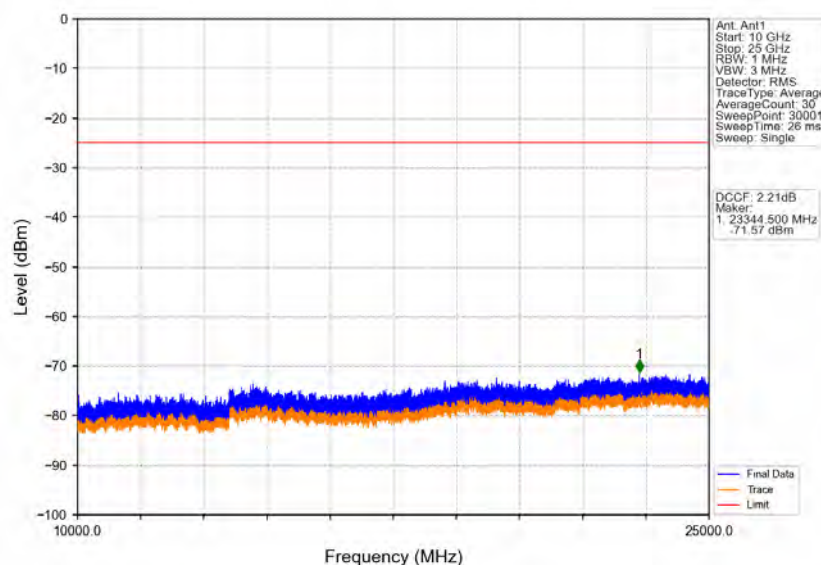
Band41_15MHz_16QAM_MCH_2595MHz_RB_1_0_NTNV
