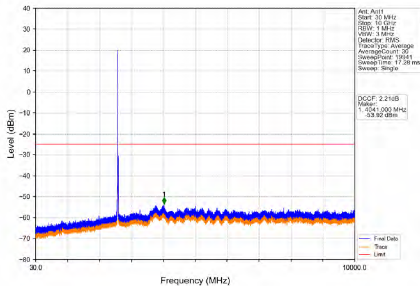
Band41_15MHz_16QAM_MCH_2595MHz_RB_1_0_NTNV
