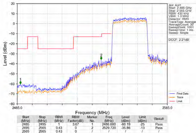
Band41_20MHz_16QAM_LCH_2545MHz_RB_100_0_NTNV
