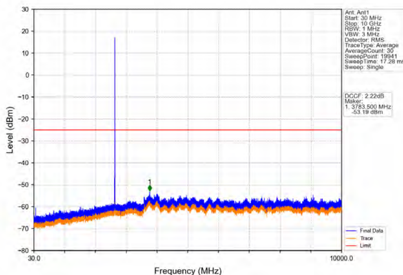
Band41_5MHz_16QAM_HCH_2652.5MHz_RB_1_0_NTNV
