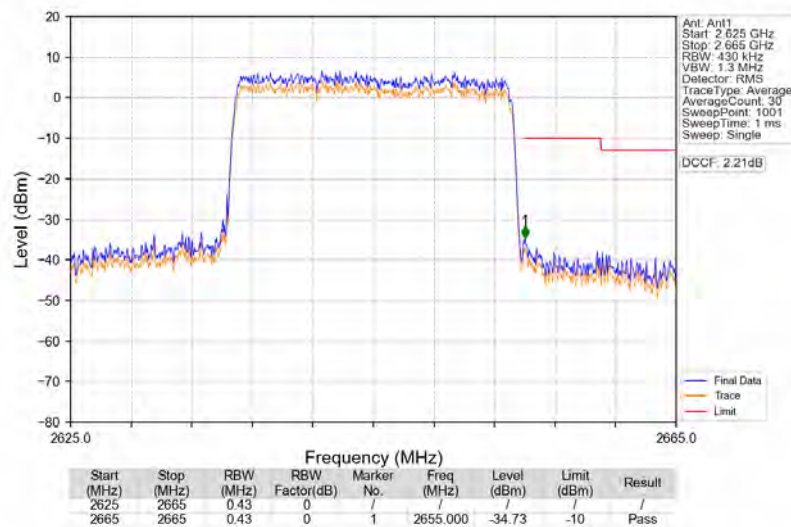
Band41_20MHz_16QAM_HCH_2645MHz_RB_100_0_NTNV
