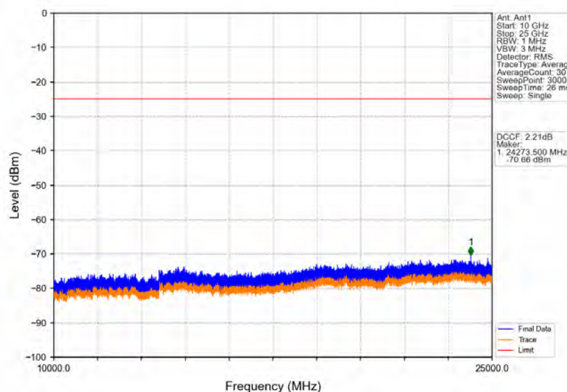
Band41_5MHz_16QAM_MCH_2595MHz_RB_1_0_NTNV
