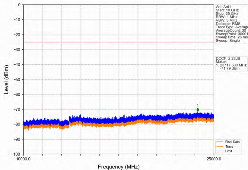
Band41_15MHz_QPSK_LCH_2542.5MHz_RB_1_0_NTNV
