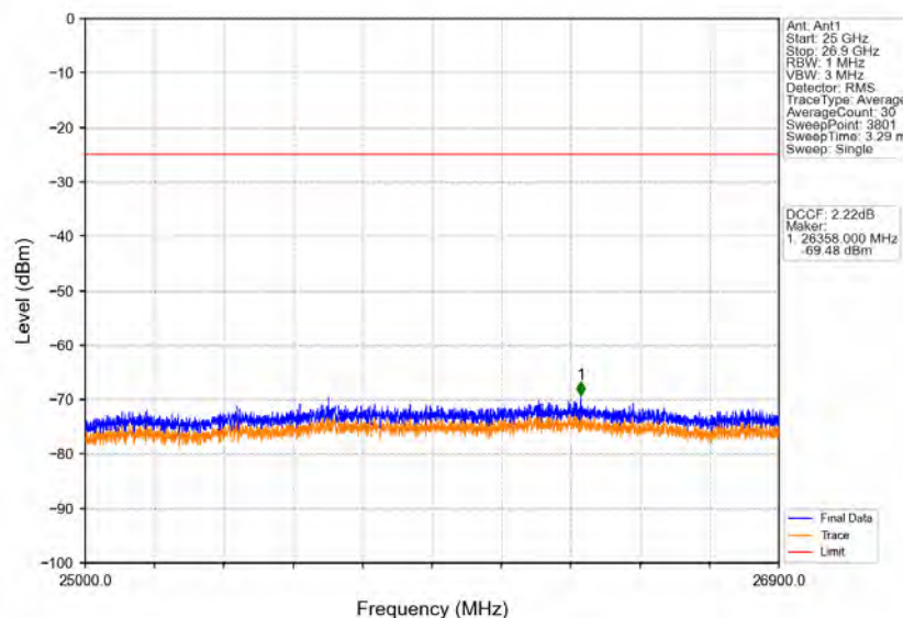
Band41_5MHz_16QAM_HCH_2652.5MHz_RB_1_0_NTNV
