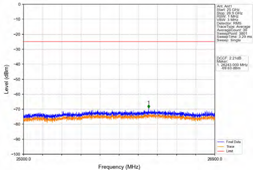
Band41_15MHz_16QAM_HCH_2647.5MHz_RB_1_0_NTNV
