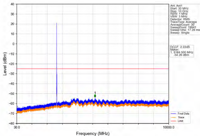
Band41_10MHz_16QAM_HCH_2650MHz_RB_1_0_NTNV
