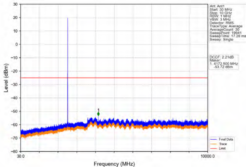
Band41_5MHz_16QAM_LCH_2537.5MHz_RB_1_0_NTNV
