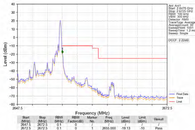
Band41_5MHz_16QAM_HCH_2652.5MHz_RB_1_24_NTNV
