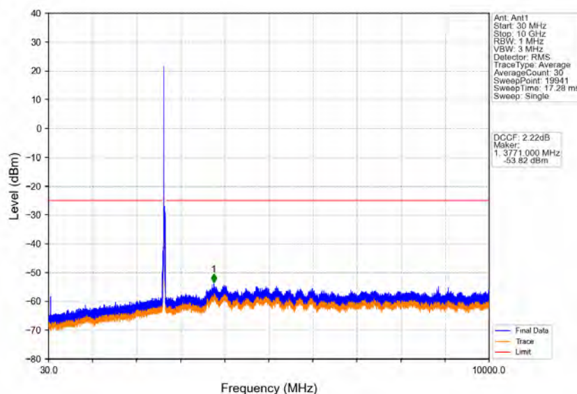
Band41_20MHz_16QAM_HCH_2645MHz_RB_1_0_NTNV
