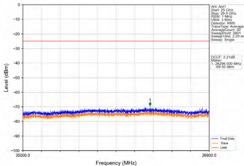
Band41_5MHz_16QAM_LCH_2537.5MHz_RB_25_0_NTNV
