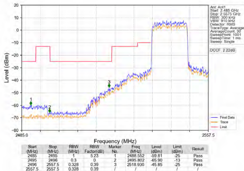
Band41_15MHz_QPSK_LCH_2542.5MHz_RB_75_0_NTNV
