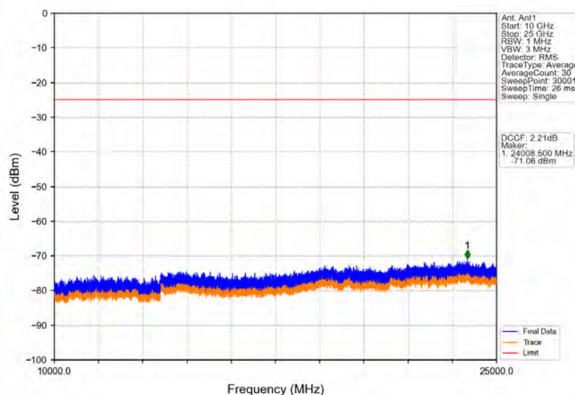
Band41_20MHz_16QAM_LCH_2545MHz_RB_1_0_NTNV
