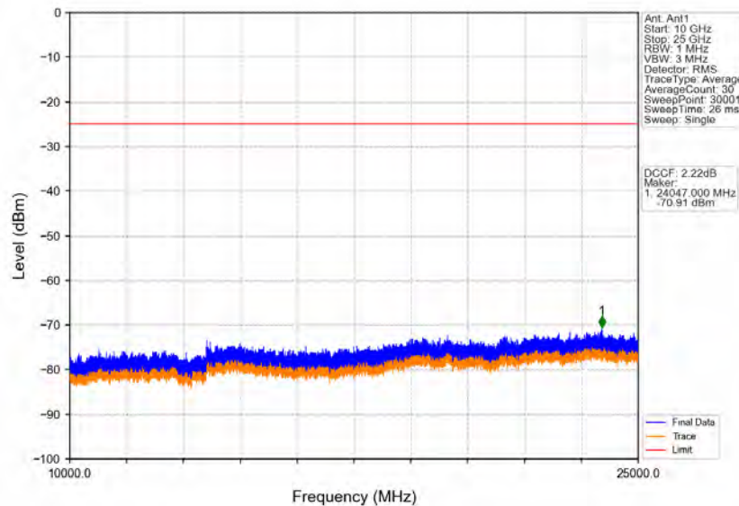
Band41_20MHz_16QAM_HCH_2645MHz_RB_1_0_NTNV
