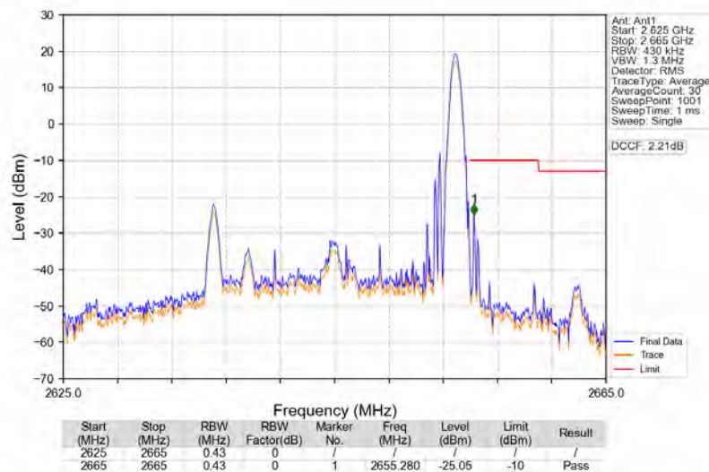
Band41_20MHz_16QAM_HCH_2645MHz_RB_1_99_NTNV
