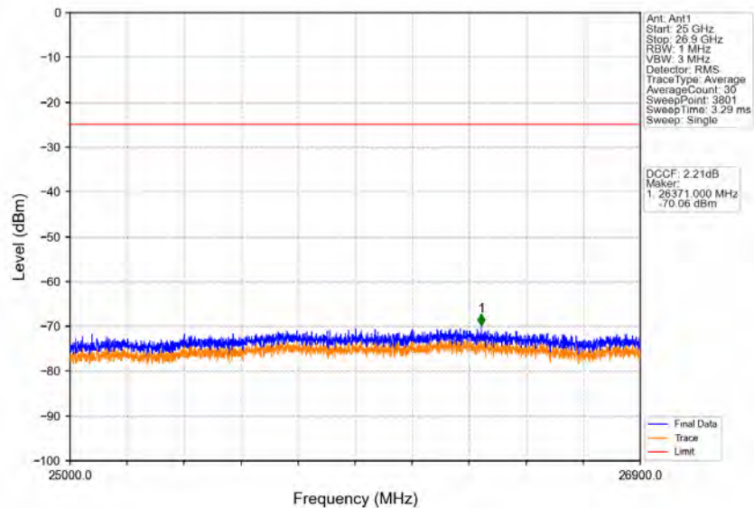
Band41_10MHz_16QAM_HCH_2650MHz_RB_1_0_NTNV
