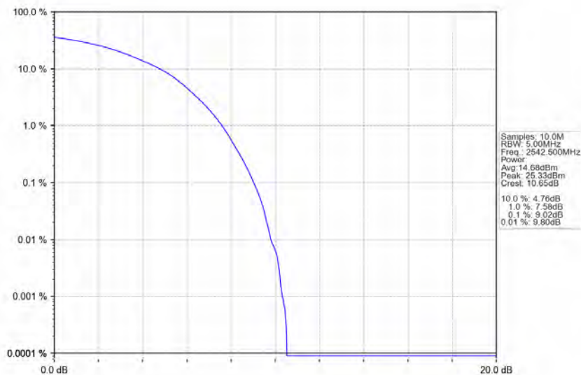
Band41_15MHz_16QAM_LCH_2542.5MHz_RB_75_0_NTNV
