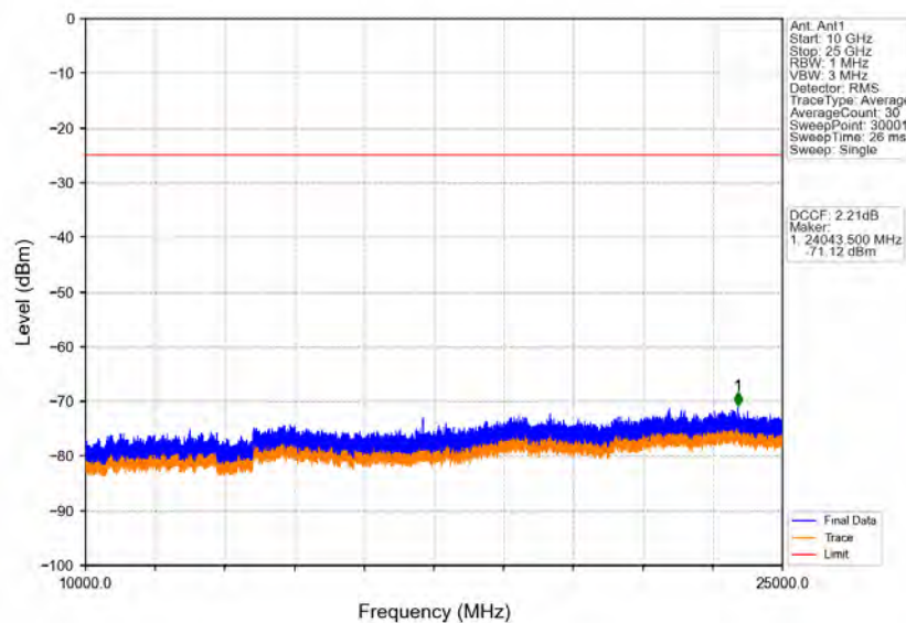
Band41_5MHz_16QAM_LCH_2537.5MHz_RB_1_0_NTNV
