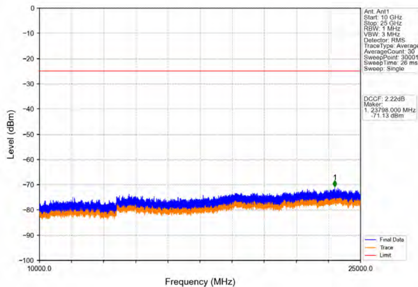
Band41_10MHz_16QAM_HCH_2650MHz_RB_1_0_NTNV
