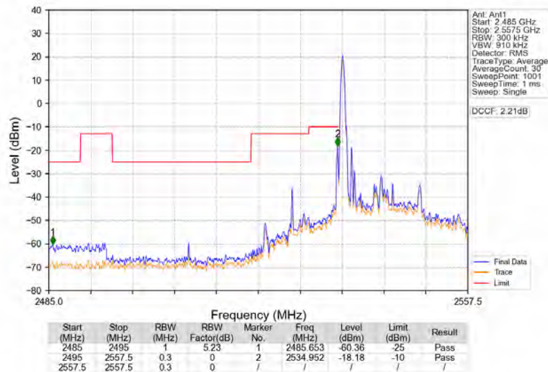
Band41_15MHz_16QAM_LCH_2542.5MHz_RB_1_0_NTNV
