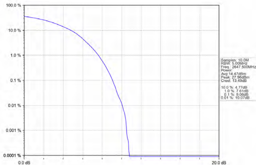
Band41_15MHz_16QAM_HCH_2647.5MHz_RB_75_0_NTNV
