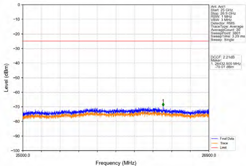
Band41_5MHz_16QAM_HCH_2652.5MHz_RB_1_0_NTNV
