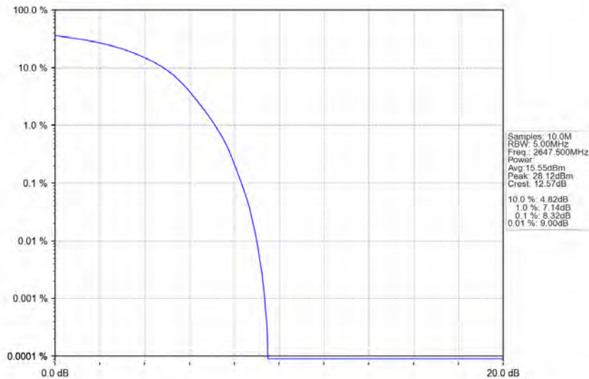
Band41_15MHz_QPSK_HCH_2647.5MHz_RB_75_0_NTNV
