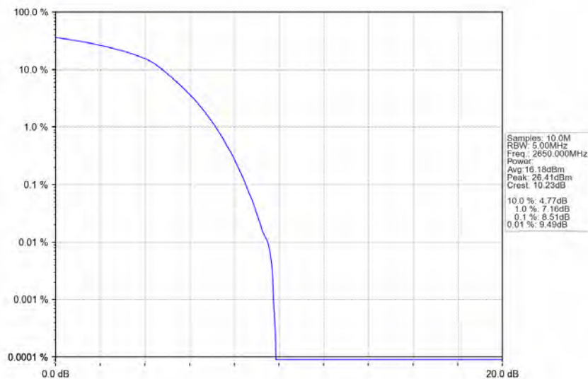
Band41_10MHz_16QAM_HCH_2650MHz_RB_50_0_NTNV
