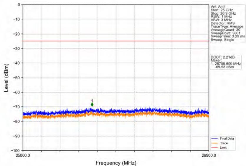
Band41_15MHz_16QAM_LCH_2542.5MHz_RB_75_0_NTNV
