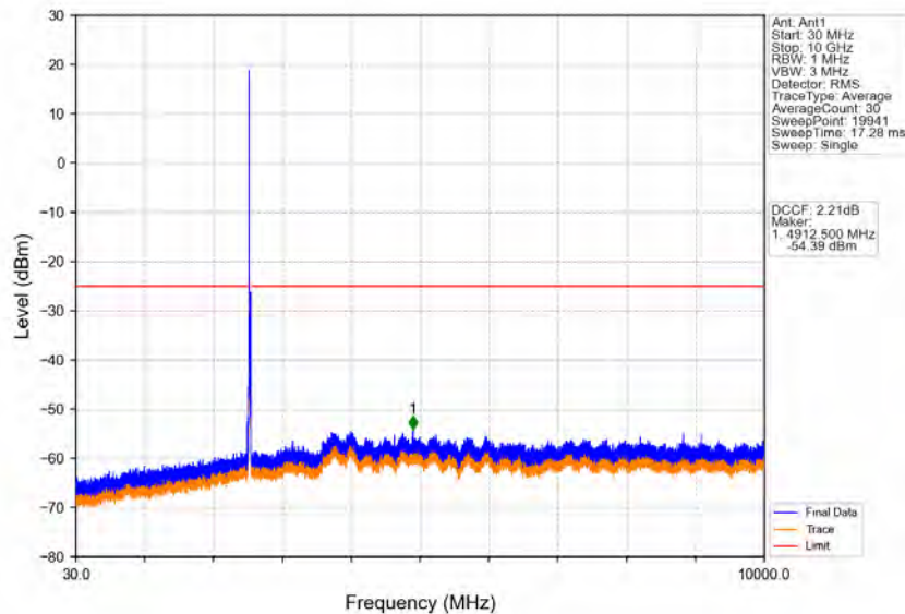
Band41_15MHz_16QAM_LCH_2542.5MHz_RB_1_0_NTNV
