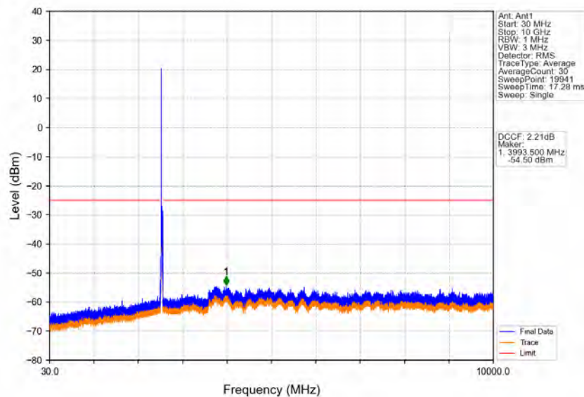
Band41_20MHz_16QAM_LCH_2545MHz_RB_1_0_NTNV
