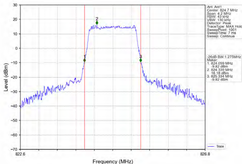
Band5_1.4MHz_16QAM_LCH_824.7MHz_RB_6_0_NTNV
