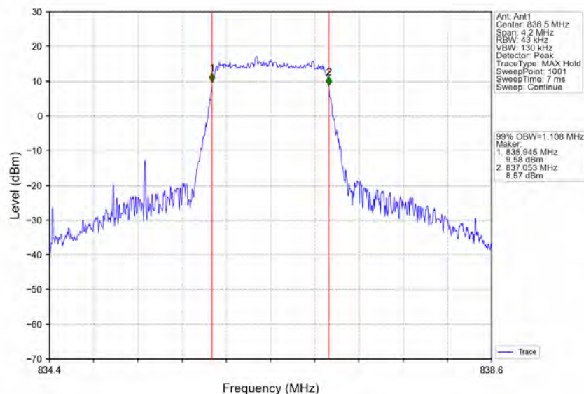
Band5_1.4MHz_16QAM_MCH_836.5MHz_RB_6_0_NTNV
