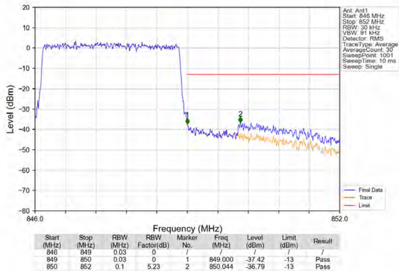
Band5_3MHz_16QAM_HCH_847.5MHz_RB_15_0_NTNV
