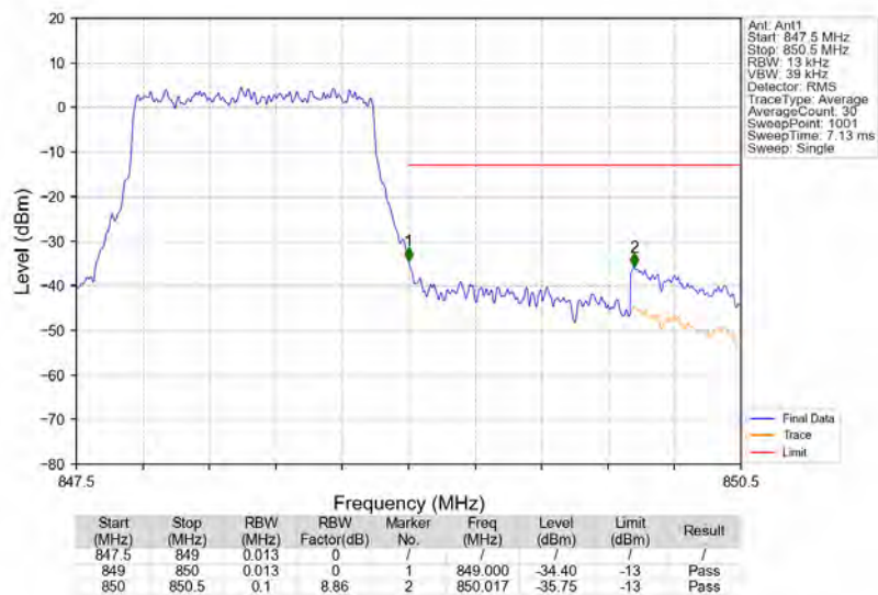
Band5_1.4MHz_QPSK_HCH_848.3MHz_RB_6_0_NTNV
