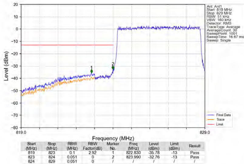
Band5_5MHz_16QAM_LCH_826.5MHz_RB_25_0_NTNV
