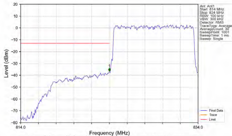
Band5_10MHz_16QAM_LCH_829MHz_RB_50_0_NTNV
