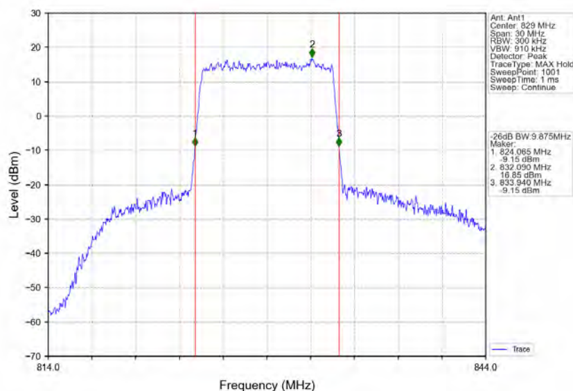
Band5_10MHz_16QAM_LCH_829MHz_RB_50_0_NTNV
