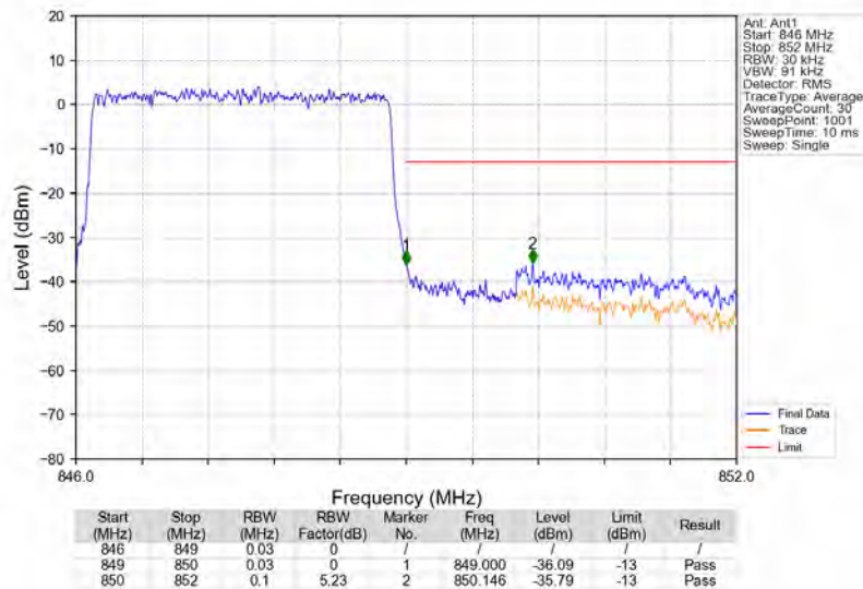
Band5_3MHz_QPSK_HCH_847.5MHz_RB_15_0_NTNV
