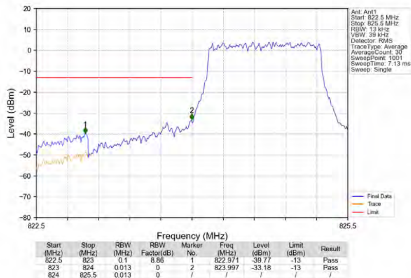
Band5_1.4MHz_QPSK_LCH_824.7MHz_RB_6_0_NTNV
