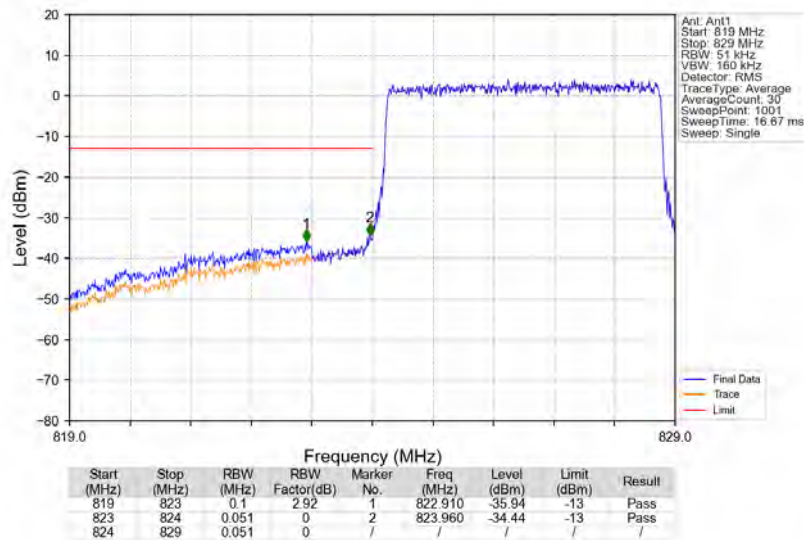
Band5_5MHz_QPSK_LCH_826.5MHz_RB_25_0_NTNV
