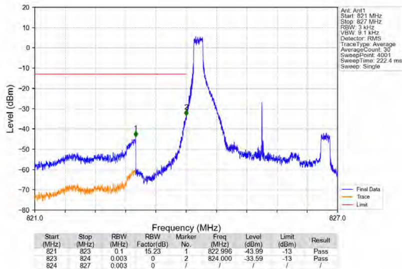
Band5_3MHz_16QAM_LCH_825.5MHz_RB_1_0_NTNV
