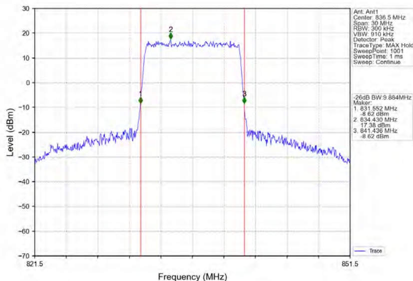
Band5_10MHz_QPSK_MCH_836.5MHz_RB_50_0_NTNV
