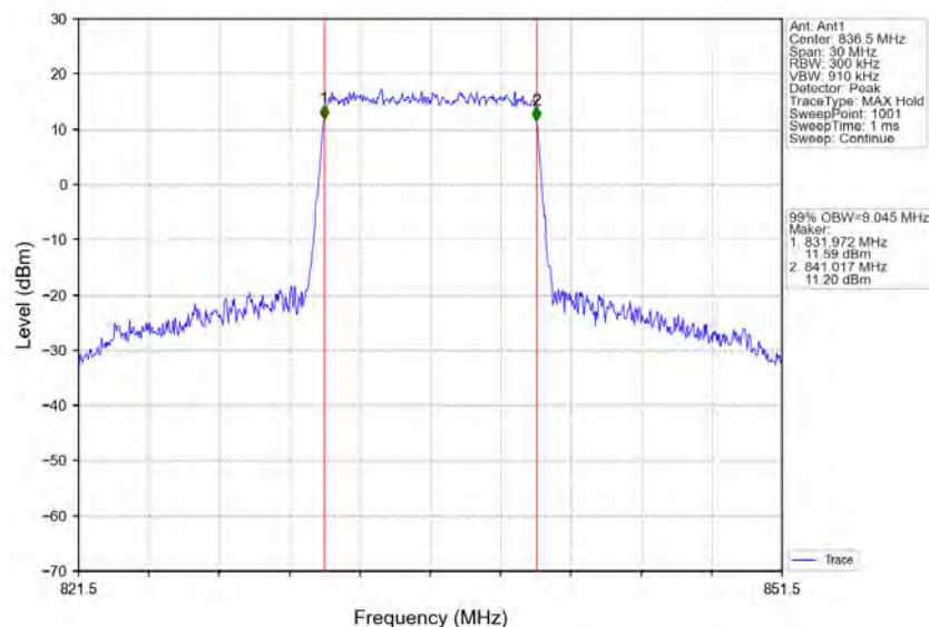
Band5_10MHz_QPSK_MCH_836.5MHz_RB_50_0_NTNV
