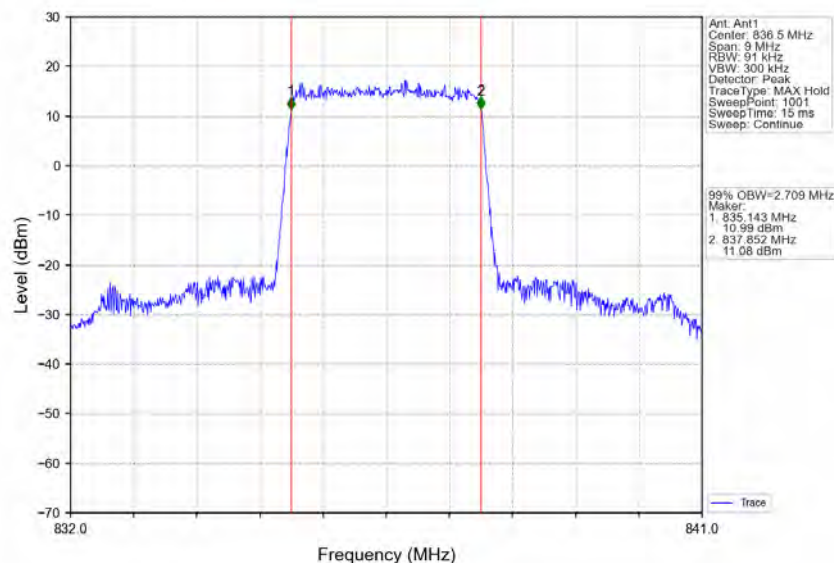
Band5_3MHz_QPSK_MCH_836.5MHz_RB_15_0_NTNV
