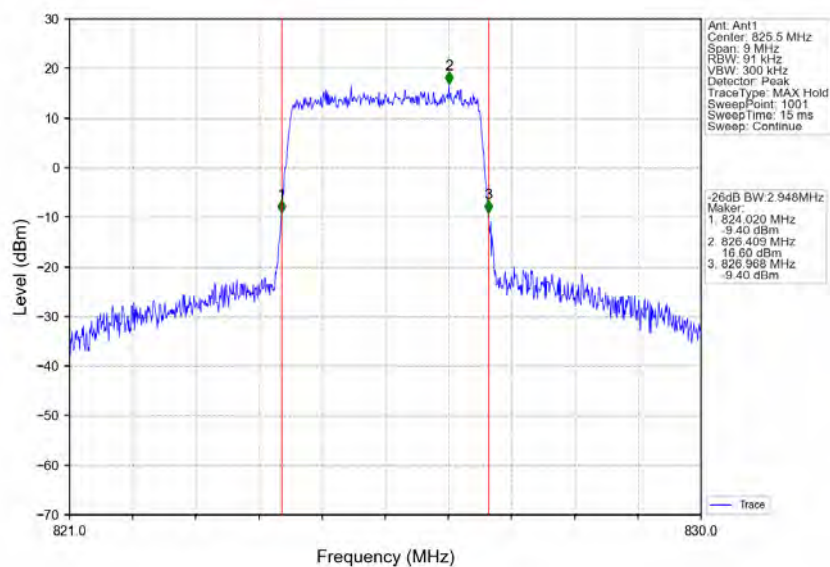
Band5_3MHz_16QAM_LCH_825.5MHz_RB_15_0_NTNV
