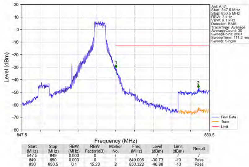
Band5_1.4MHz_QPSK_HCH_848.3MHz_RB_1_5_NTNV
