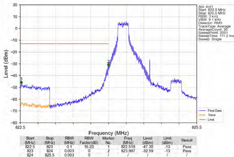
Band5_1.4MHz_16QAM_LCH_824.7MHz_RB_1_0_NTNV
