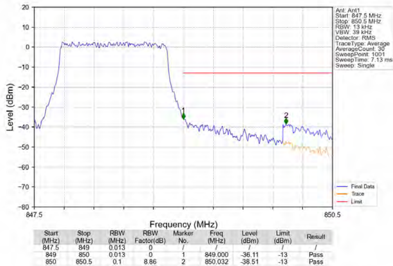
Band5_1.4MHz_16QAM_HCH_848.3MHz_RB_6_0_NTNV
