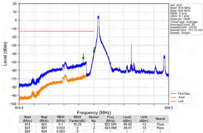
Band5_10MHz_16QAM_LCH_829MHz_RB_1_0_NTNV
