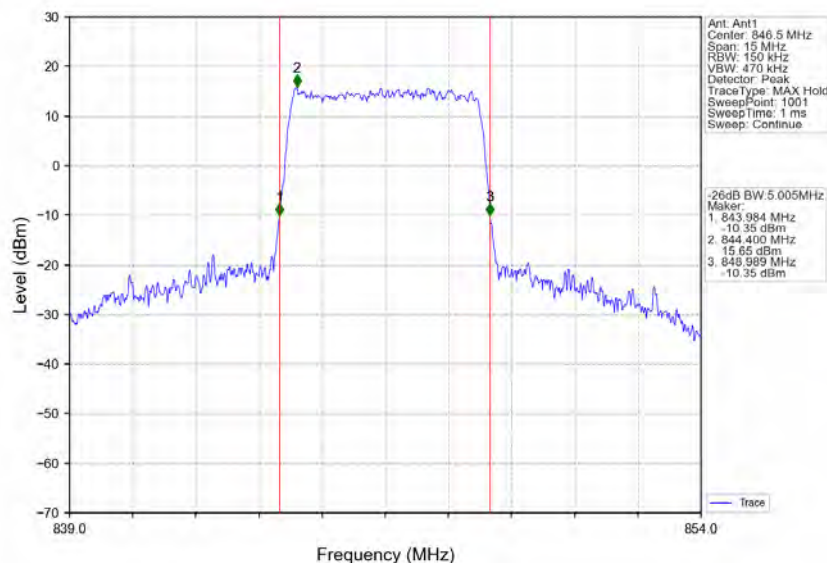
Band5_5MHz_16QAM_HCH_846.5MHz_RB_25_0_NTNV
