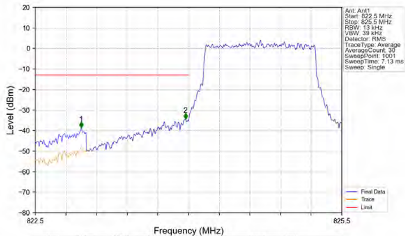
Band5_1.4MHz_16QAM_LCH_824.7MHz_RB_6_0_NTNV
