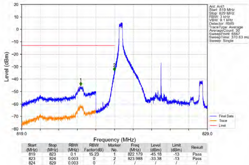
Band5_5MHz_16QAM_LCH_826.5MHz_RB_1_0_NTNV
