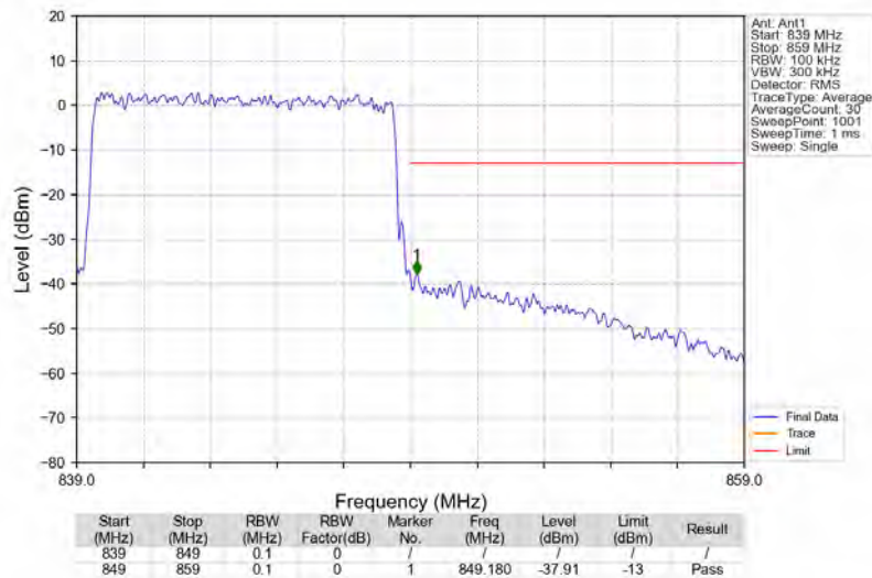
Band5_10MHz_16QAM_HCH_844MHz_RB_50_0_NTNV
