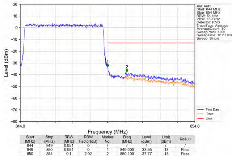
Band5_5MHz_QPSK_HCH_846.5MHz_RB_25_0_NTNV
