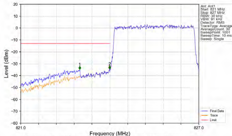
Band5_3MHz_16QAM_LCH_825.5MHz_RB_15_0_NTNV
