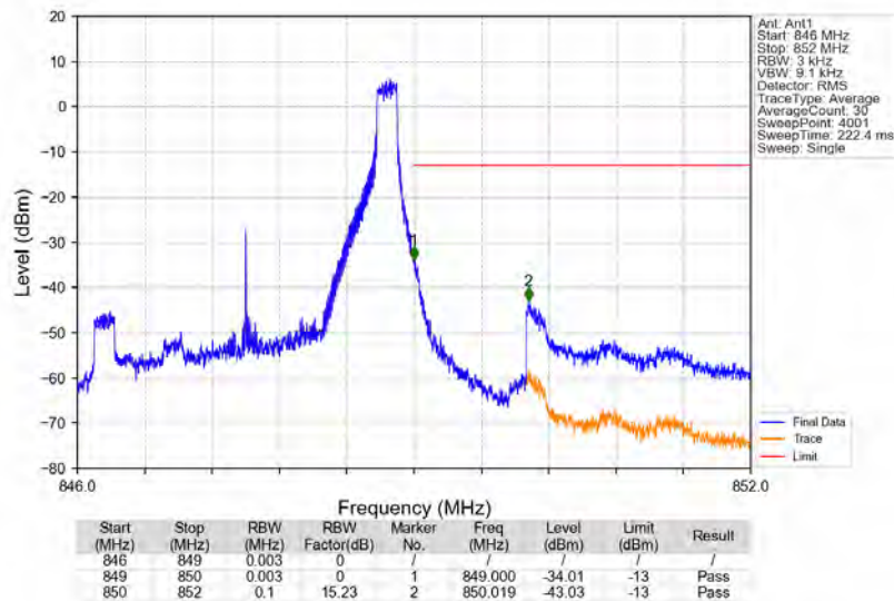
Band5_3MHz_16QAM_HCH_847.5MHz_RB_1_14_NTNV
