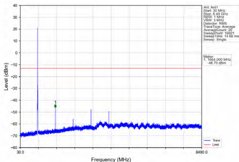
Band5_10MHz_QPSK_MCH_836.5MHz_RB_1_0_NTNV
