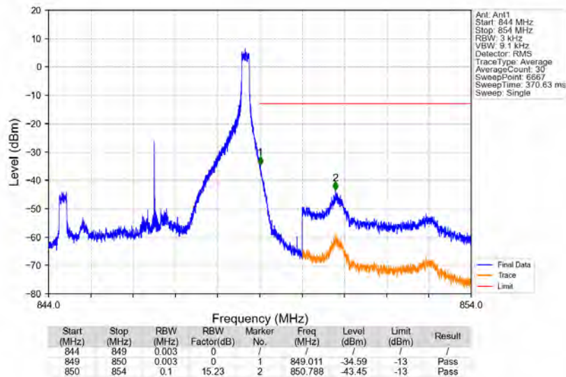
Band5_5MHz_16QAM_HCH_846.5MHz_RB_1_24_NTNV
