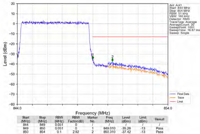
Band5_5MHz_16QAM_HCH_846.5MHz_RB_25_0_NTNV
