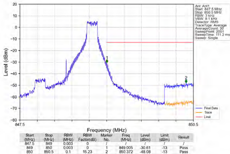
Band5_1.4MHz_16QAM_HCH_848.3MHz_RB_1_5_NTNV
