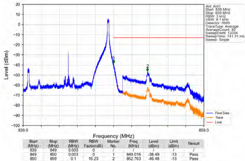
Band5_10MHz_16QAM_HCH_844MHz_RB_1_49_NTNV
