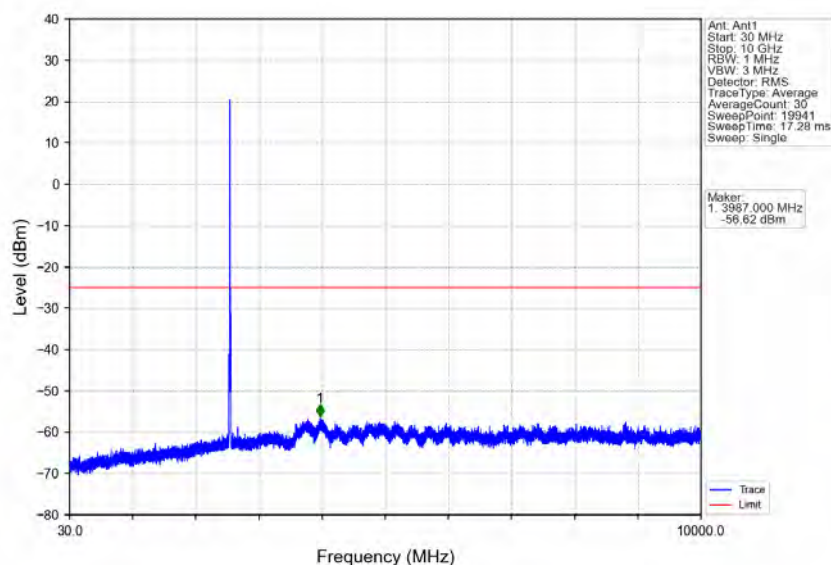
Band7_10MHz_16QAM_HCH_2565MHz_RB_1_0_NTNV
