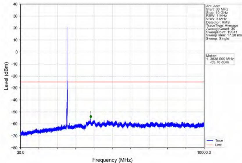
Band7_15MHz_QPSK_HCH_2562.5MHz_RB_1_0_NTNV
