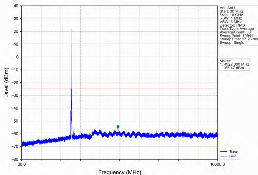
Band7_15MHz_16QAM_HCH_2562.5MHz_RB_1_0_NTNV
