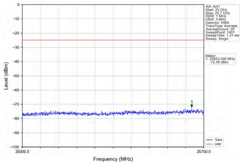
Band7_15MHz_16QAM_HCH_2562.5MHz_RB_1_0_NTNV
