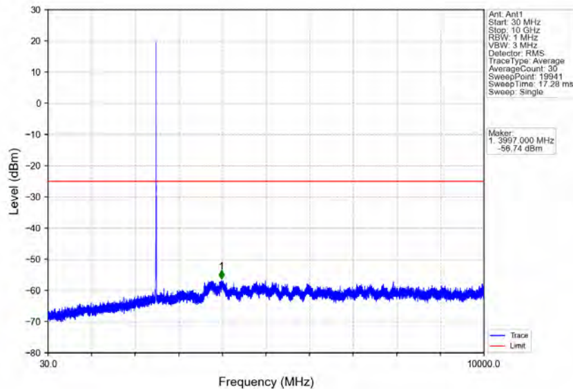
Band7_5MHz_16QAM_LCH_2502.5MHz_RB_1_0_NTNV
