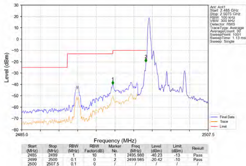
Band7_5MHz_16QAM_LCH_2502.5MHz_RB_1_0_NTNV
