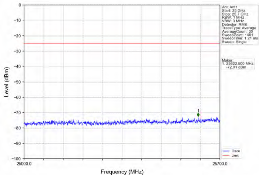
Band7_5MHz_16QAM_HCH_2567.5MHz_RB_1_0_NTNV
