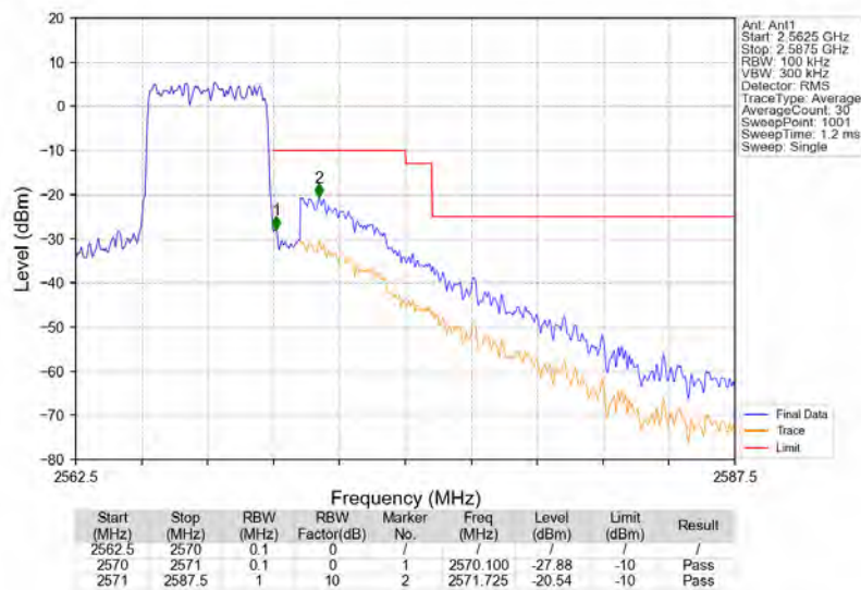
Band7_5MHz_16QAM_HCH_2567.5MHz_RB_25_0_NTNV
