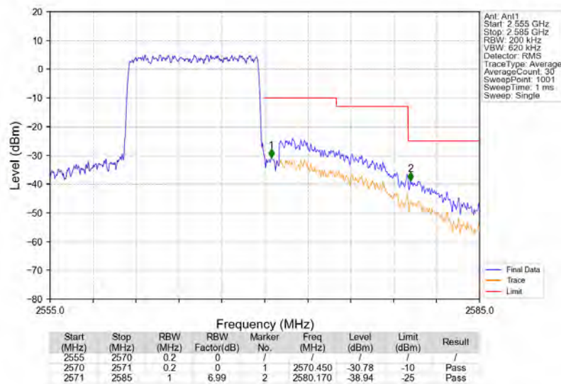
Band7_10MHz_16QAM_HCH_2565MHz_RB_50_0_NTNV
