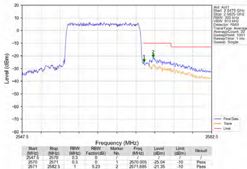
Band7_15MHz_QPSK_HCH_2562.5MHz_RB_75_0_NTNV
