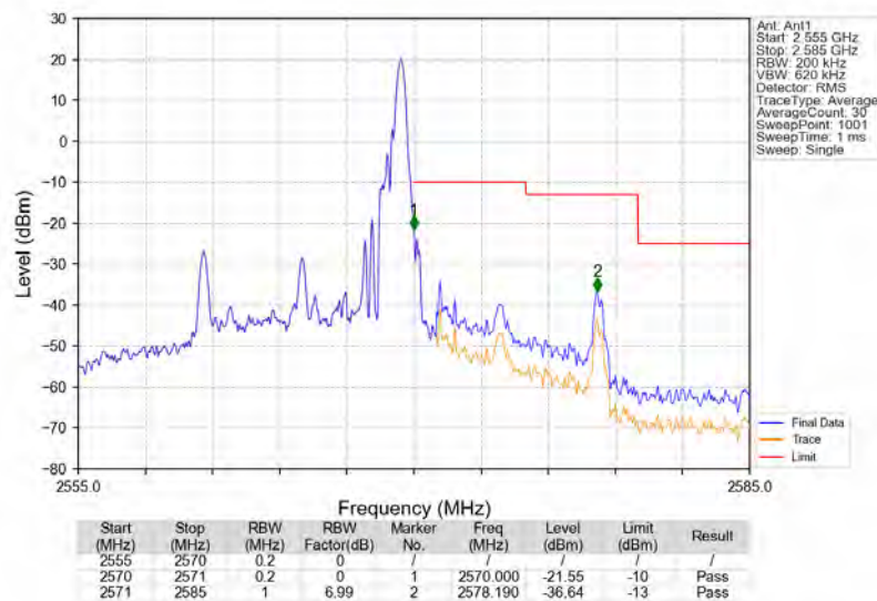
Band7_10MHz_16QAM_HCH_2565MHz_RB_1_49_NTNV
