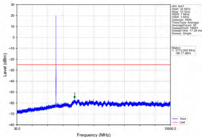
Band7_5MHz_16QAM_HCH_2567.5MHz_RB_1_0_NTNV
