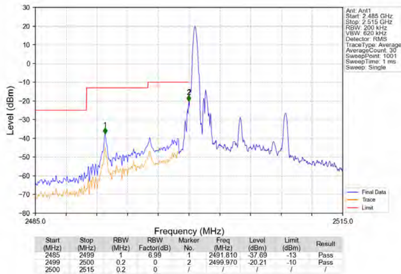
Band7_10MHz_16QAM_LCH_2505MHz_RB_1_0_NTNV
