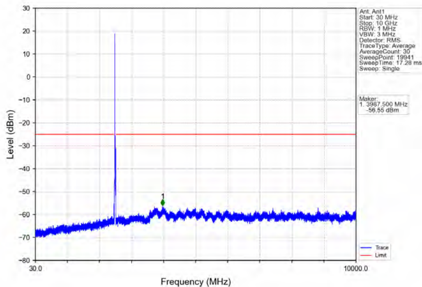
Band7_15MHz_16QAM_LCH_2507.5MHz_RB_1_0_NTNV
