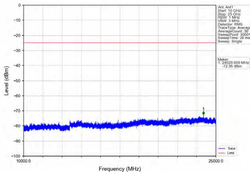
Band7_5MHz_16QAM_LCH_2502.5MHz_RB_1_0_NTNV
