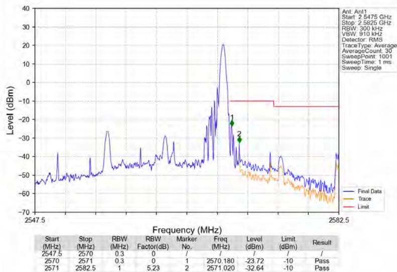
Band7_15MHz_16QAM_HCH_2562.5MHz_RB_1_74_NTNV
