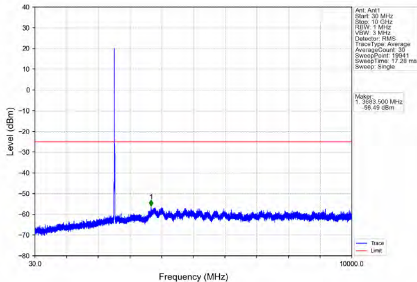
Band7_10MHz_16QAM_MCH_2535MHz_RB_1_0_NTNV
