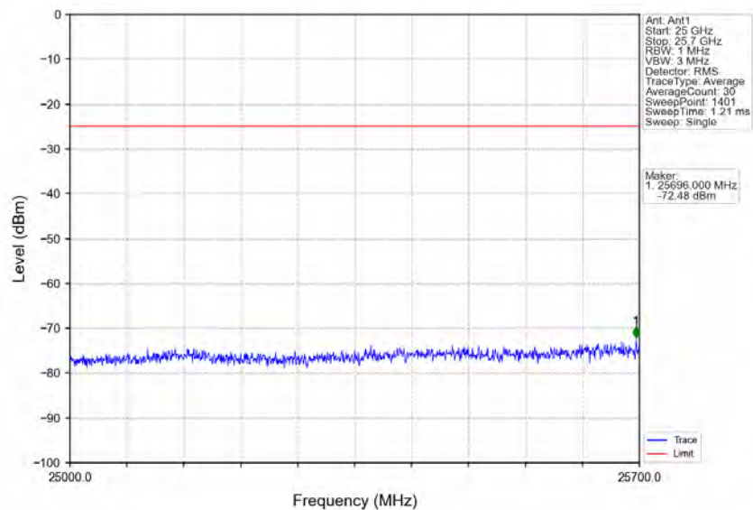
Band7_10MHz_16QAM_HCH_2565MHz_RB_1_0_NTNV
