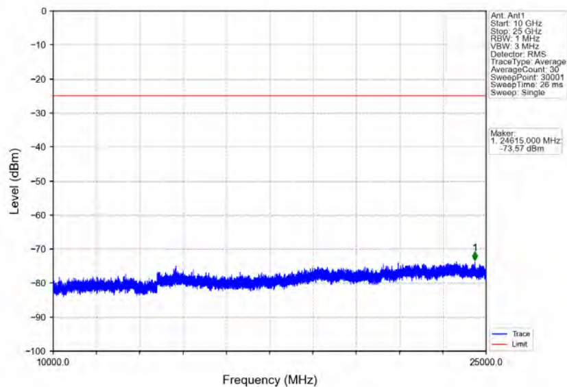
Band7_10MHz_16QAM_HCH_2565MHz_RB_1_0_NTNV
