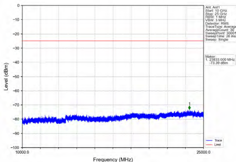
Band7 20MHz 16QAM MCH 2535MHz RB 1 0 NTV
