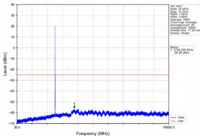
Band7 5MHz QPSK MCH 2535MHz RB 1_0 NTNV
