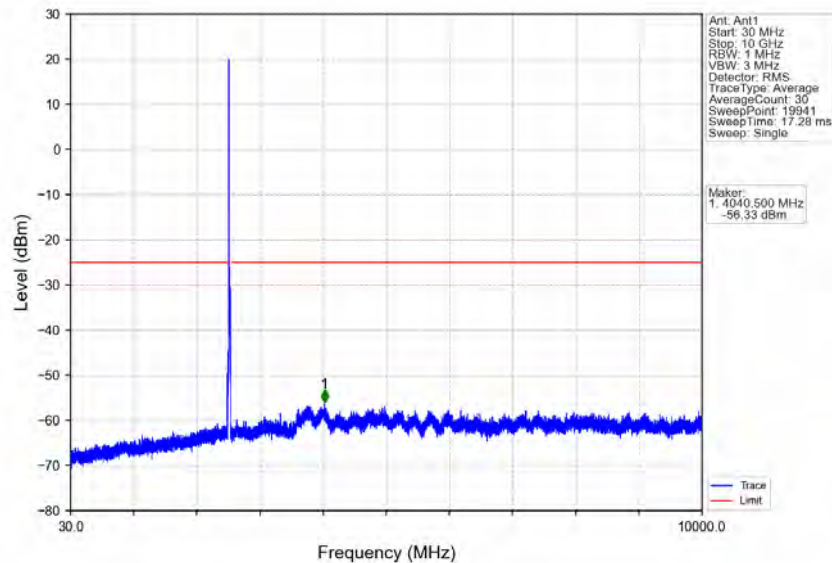
Band7_15MHz_16QAM_MCH_2535MHz_RB_1_0_NTNV
