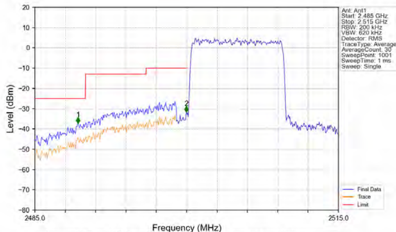
Band7_10MHz_16QAM_LCH_2505MHz_RB_50_0_NTNV
