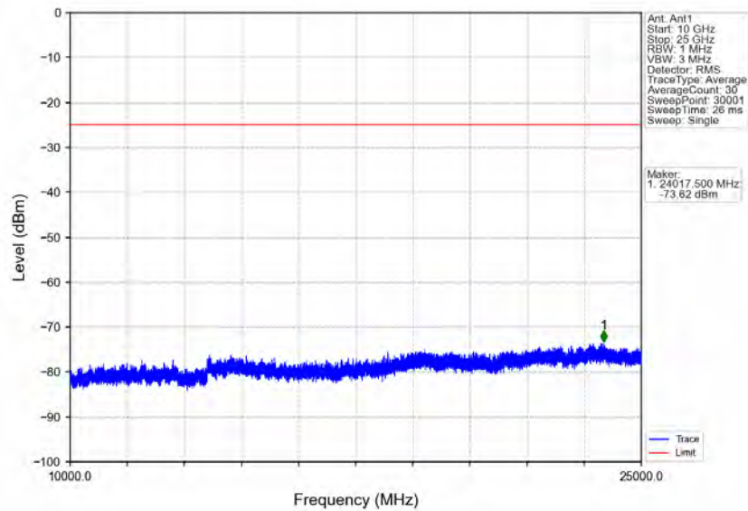
Band7_15MHz_16QAM_HCH_2562.5MHz_RB_1_0_NTNV
