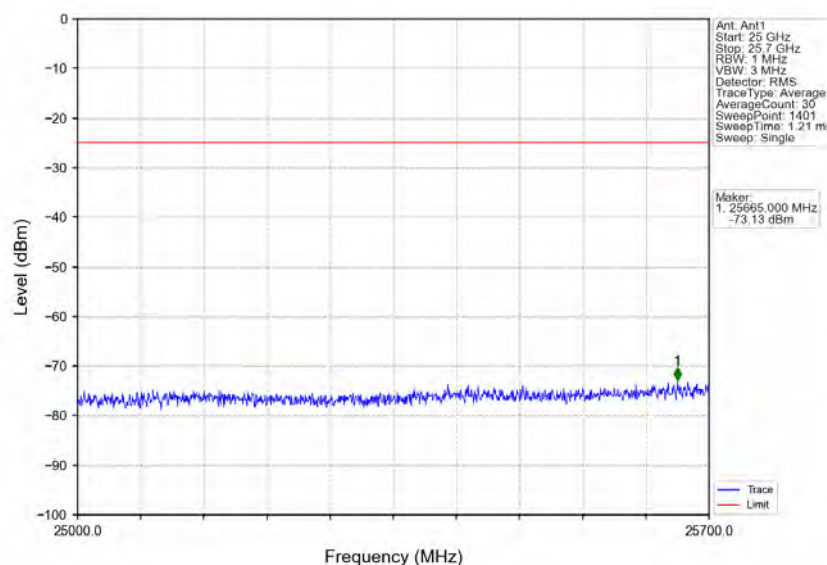
Band7_15MHz_QPSK_MCH_2535MHz_RB_1_0_NTNV
