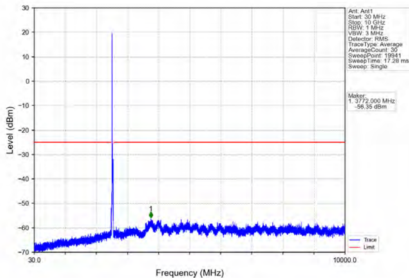
Band7 20MHz 16QAM MCH 2535MHz RB 1 0 NTV
