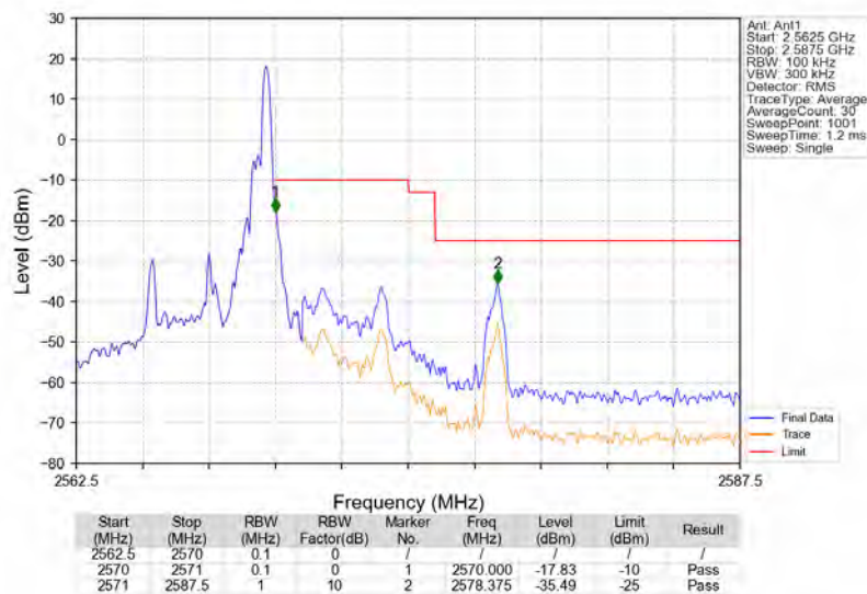
Band7_5MHz_16QAM_HCH_2567.5MHz_RB_1_24_NTNV
