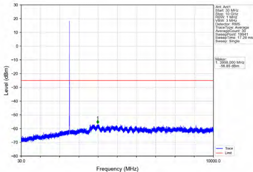
Band7_5MHz_16QAM_MCH_2535MHz_RB_1_0_NTNV
