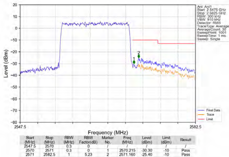
Band7_15MHz_16QAM_HCH_2562.5MHz_RB_75_0_NTNV
