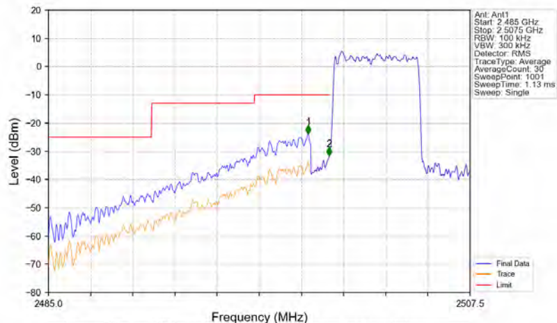
Band7_5MHz_16QAM_LCH_2502.5MHz_RB_25_0_NTNV
