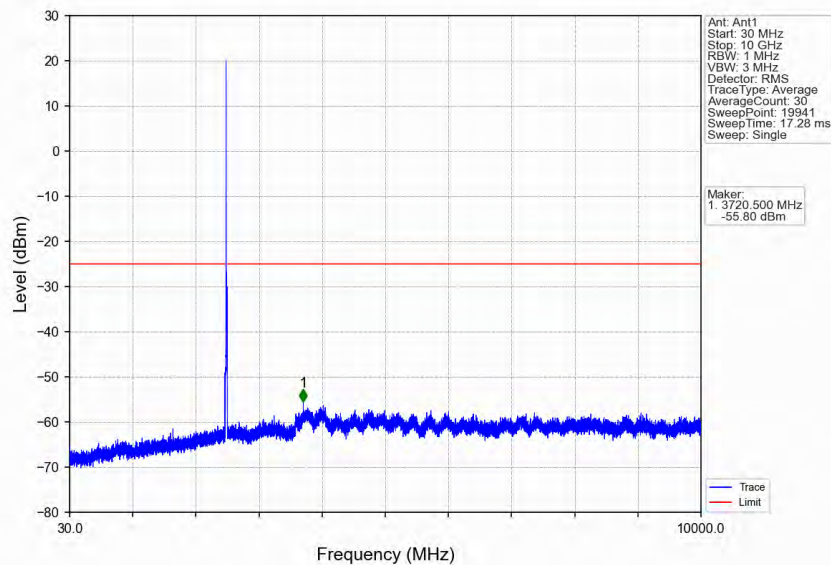
Band7_10MHz_16QAM_LCH_2505MHz_RB_1_0_NTNV
