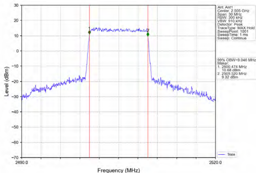
Band7_10MHz_16QAM_LCH_2505MHz_RB_50_0_NTNV
