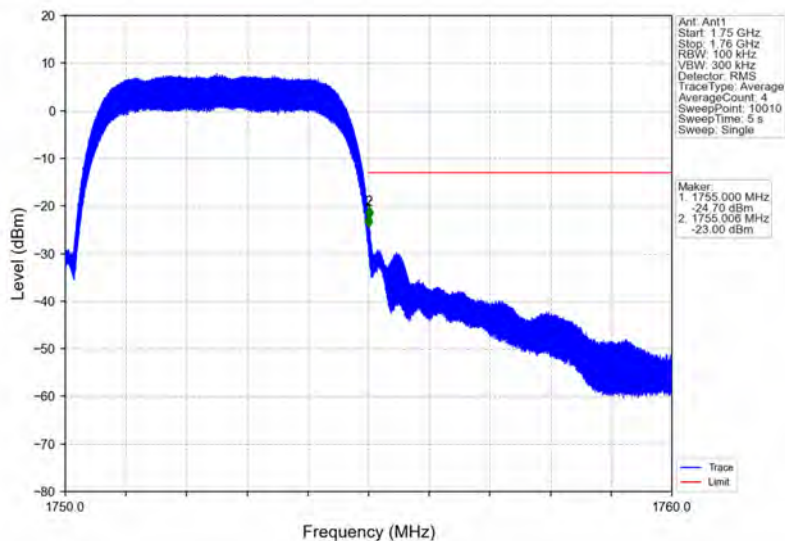
Band4_HSDPA_HCH_1752.6MHz_Subtest 1_NTNV
