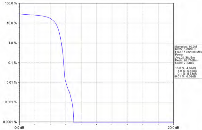
Band4_HSDPA_MCH_1732.6MHz_Subtest 1_NTNV
