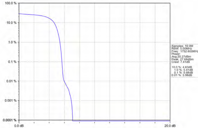
Band4_HSUPA_HCH_1752.6MHz_Subtest 1_NTNV
