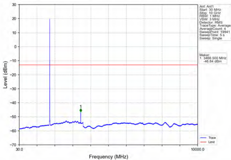
Band4_RMC_MCH_1732.6MHz_12.2kbps RMC_NTNV
