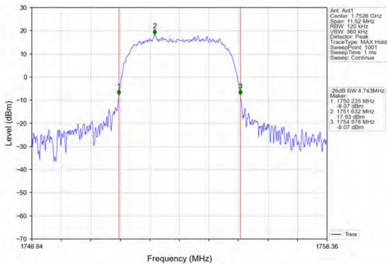
Band4_HSDPA_HCH_1752.6MHz_Subtest 1_NTNV
