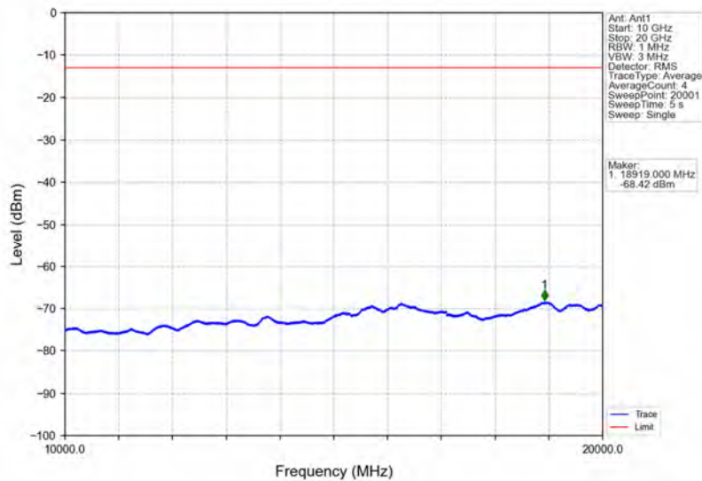
Band4_HSUPA_MCH_1732.6MHz_Subtest 1_NTNV
