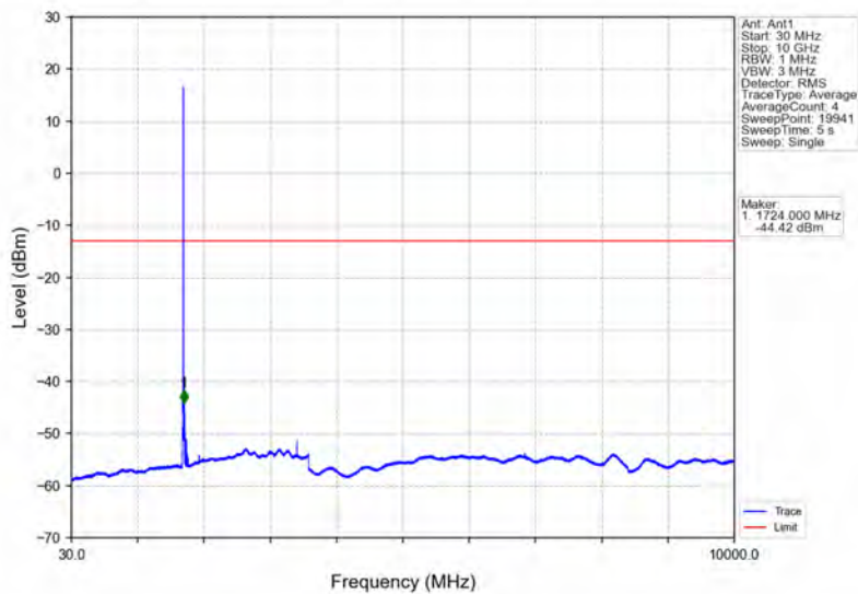
Band4_HSDPA_LCH_1712.4MHz_Subtest 1_NTNV
