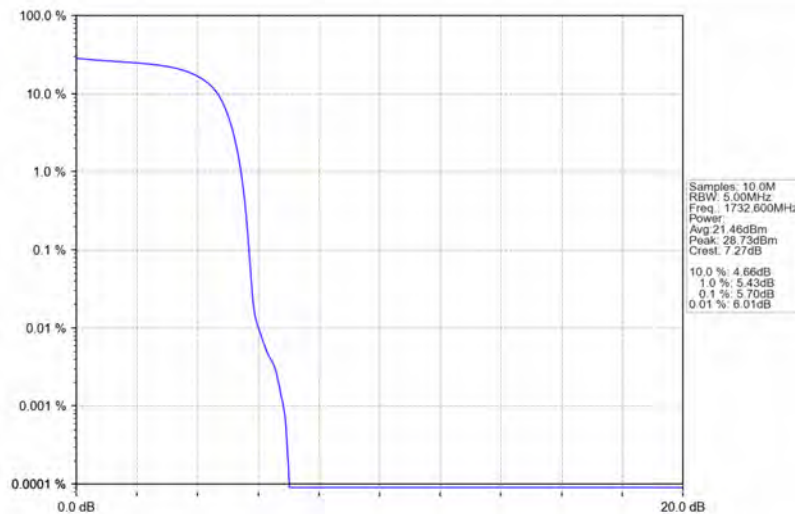
Band4_HSUPA_MCH_1732.6MHz_Subtest 1_NTNV
