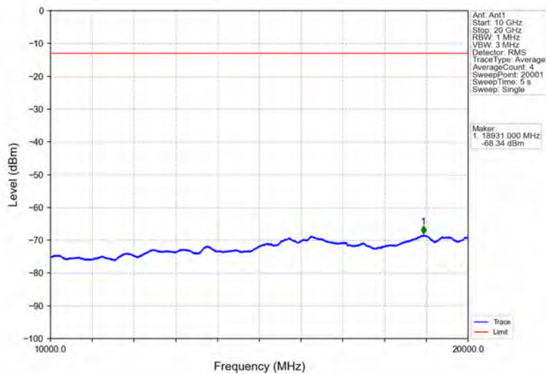
Band4_RMC_HCH_1752.6MHz_12.2kbps RMC_NTNV
