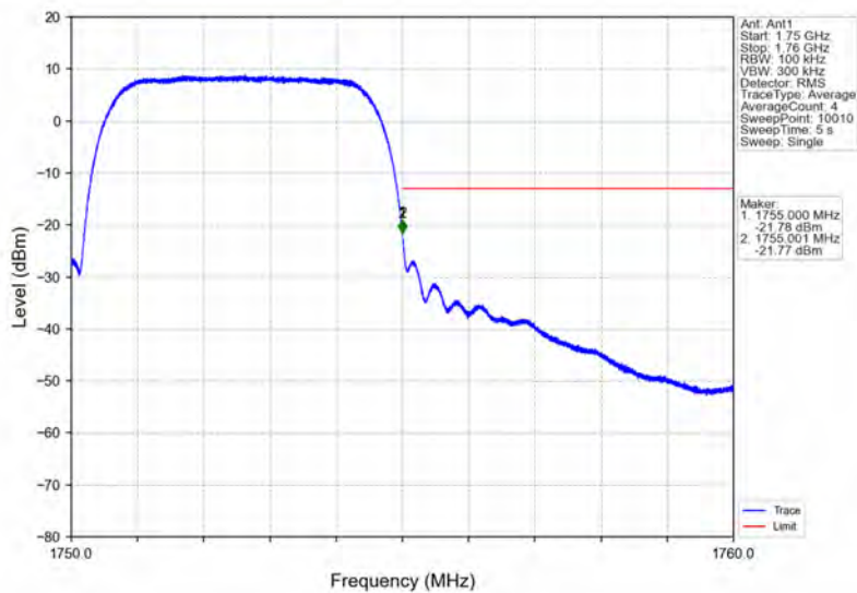
Band4_RMC_HCH_1752.6MHz_12.2kbps RMC_NTNV
