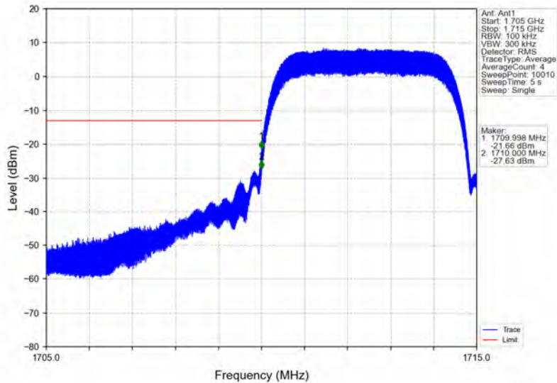
Band4_HSDPA_LCH_1712.4MHz_Subtest 1_NTNV
