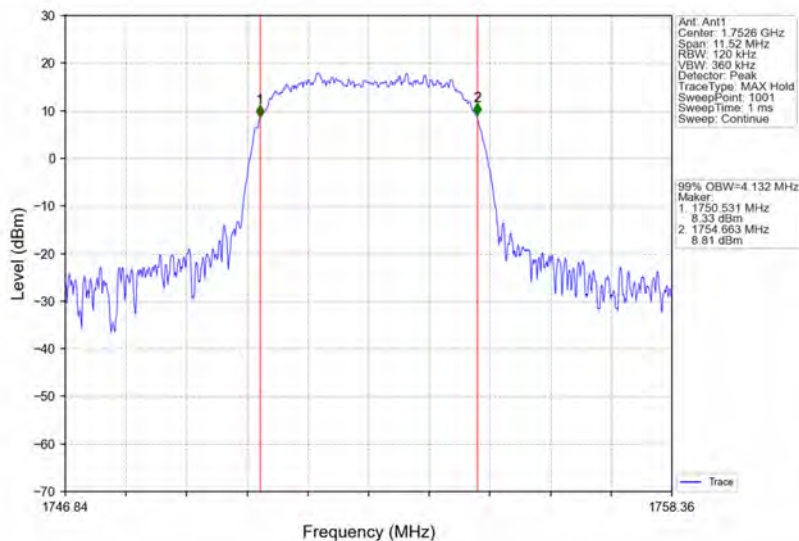
Band4_HSDPA_HCH_1752.6MHz_Subtest 1_NTNV
