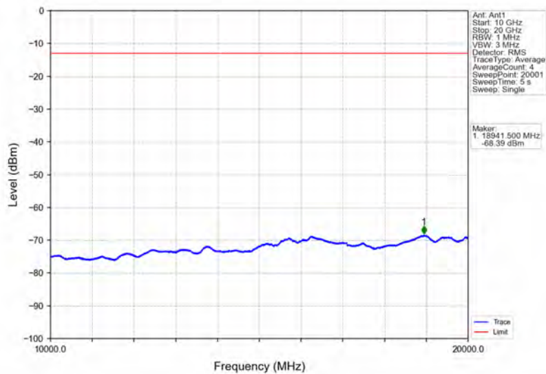
Band4_HSUPA_HCH_1752.6MHz_Subtest 1_NTNV
