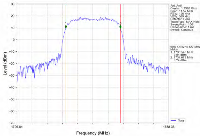
Band4_HSUPA_MCH_1732.6MHz_Subtest 1_NTNV
