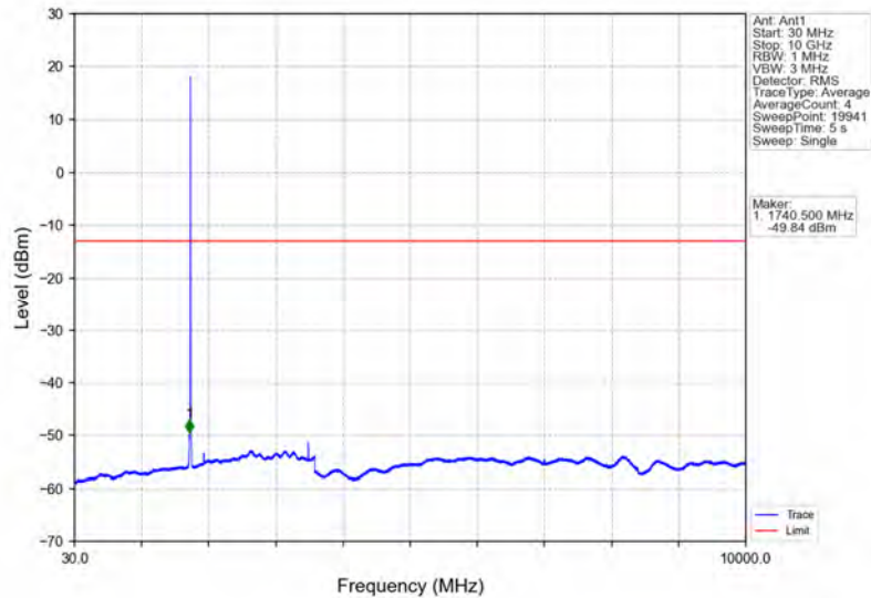
Band4_RMC_HCH_1752.6MHz_12.2kbps RMC_NTNV
