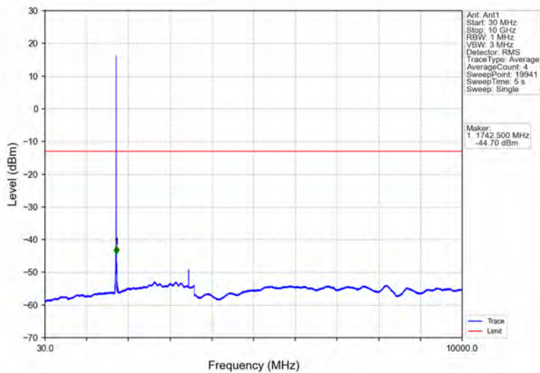
Band4_HSDPA_MCH_1732.6MHz_Subtest 1_NTNV
