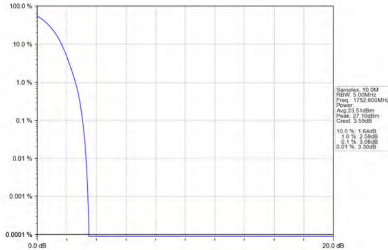
Band4_RMC_HCH_1752.6MHz_12.2kbps RMC_NTNV
