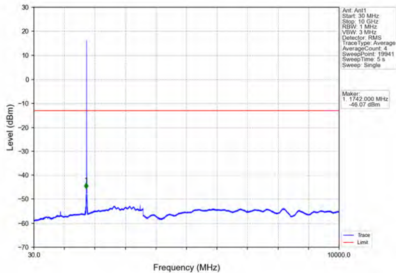
Band4_HSUPA_HCH_1752.6MHz_Subtest 1_NTNV
