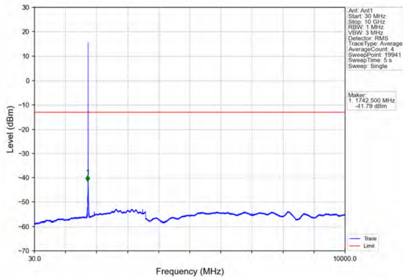
Band4_HSDPA_HCH_1752.6MHz_Subtest 1_NTNV
