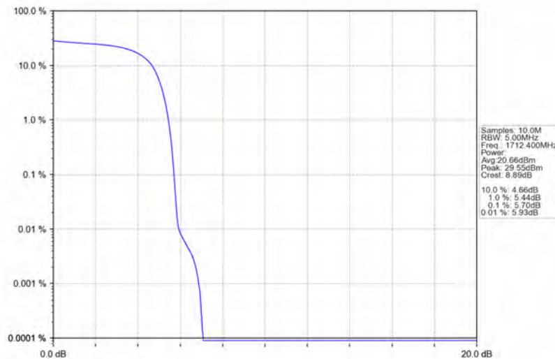
Band4_HSDPA_LCH_1712.4MHz_Subtest 1_NTNV
