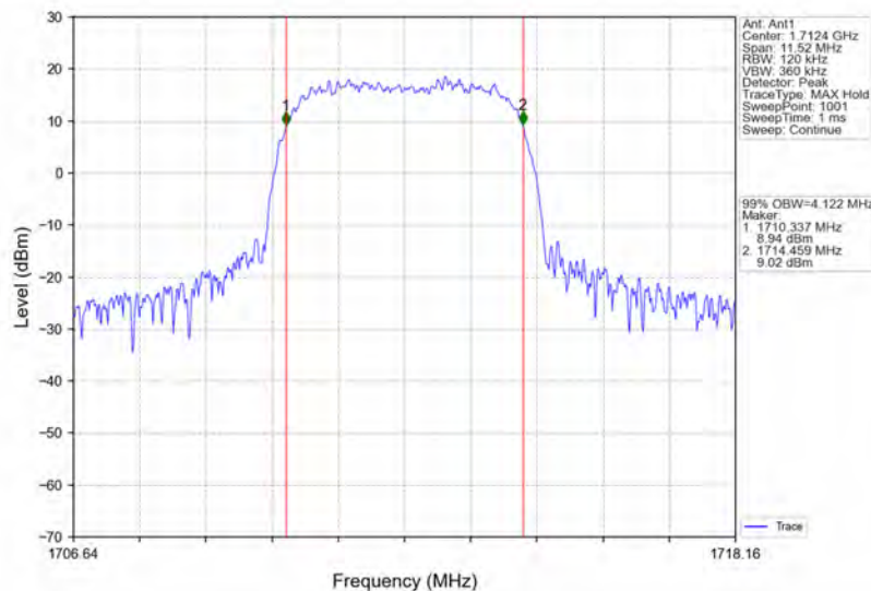
Band4_HSDPA_LCH_1712.4MHz_Subtest 1_NTNV
