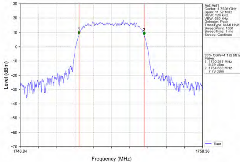
Band4_HSUPA_HCH_1752.6MHz_Subtest 1_NTNV
