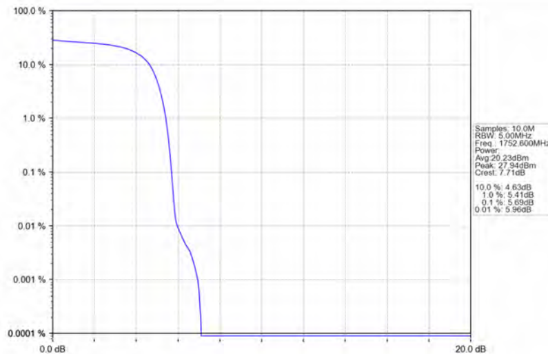
Band4_HSDPA_HCH_1752.6MHz_Subtest 1_NTNV
