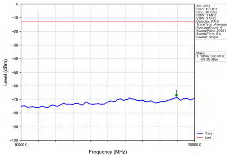
Band4_RMC_MCH_1732.6MHz_12.2kbps RMC_NTNV
