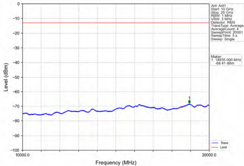
Band4_HSDPA_MCH_1732.6MHz_Subtest 1_NTNV
