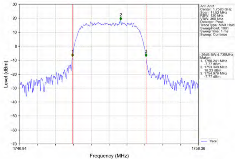
Band4_HSUPA_HCH_1752.6MHz_Subtest 1_NTNV
