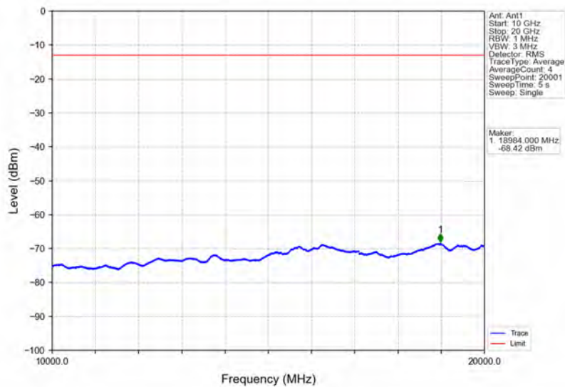
Band4_HSDPA_HCH_1752.6MHz_Subtest 1_NTNV
