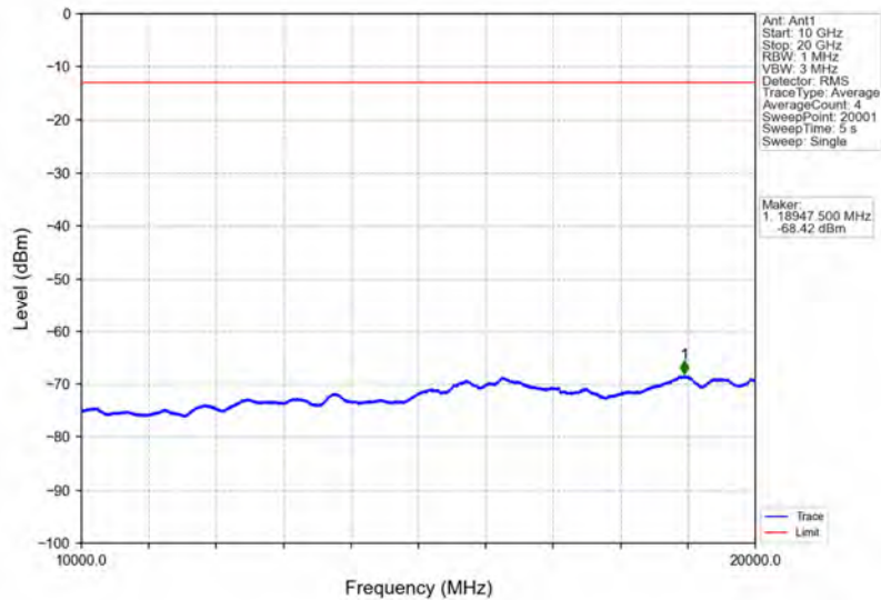
Band4_RMC_HCH_1752.6MHz_12.2kbps RMC_NTNV
