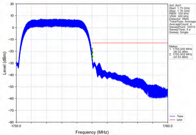
Band4_HSUPA_HCH_1752.6MHz_Subtest 1_NTNV
