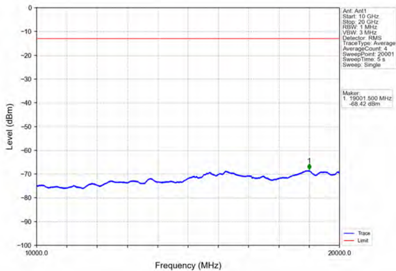
Band2_3MHz_16QAM_HCH_1908.5MHz_RB_1_0_NTNV
