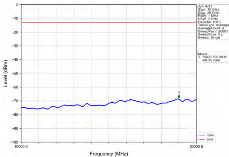
Band2_10MHz_64QAM_HCH_1905MHz_RB_1_0_NTNV
