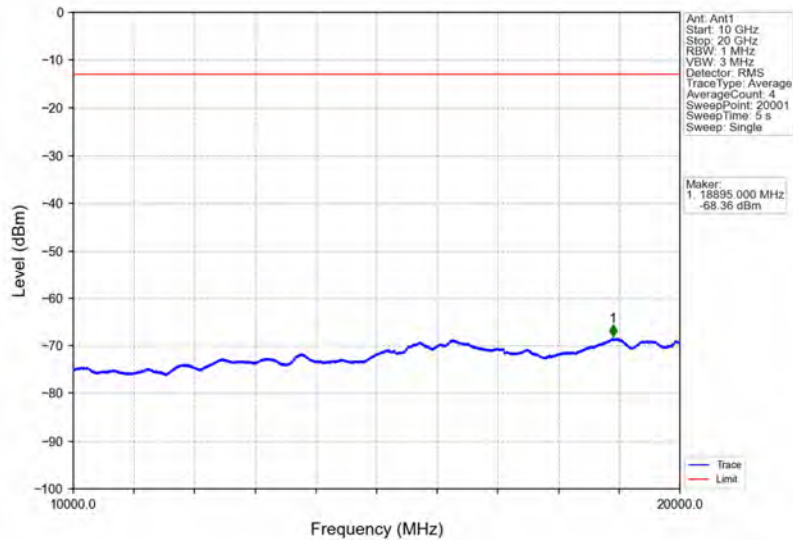
Band2_1.4MHz_QPSK_LCH_1850.7MHz_RB_6_0_NTNV
