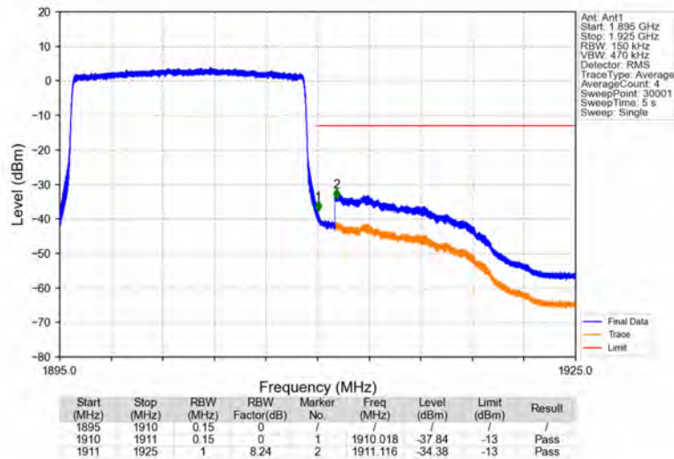
Band2_15MHz_16QAM_HCH_1902.5MHz_RB_75_0_NTNV
