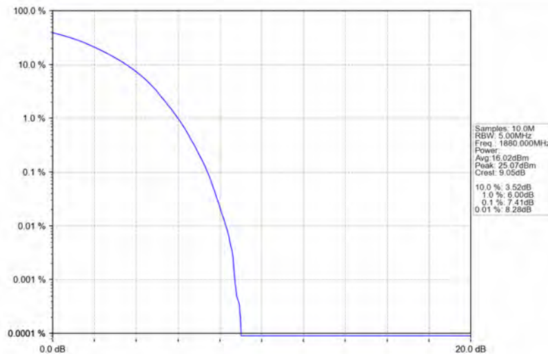
Band2_15MHz_64QAM_MCH_1880MHz_RB_75_0_NTNV
