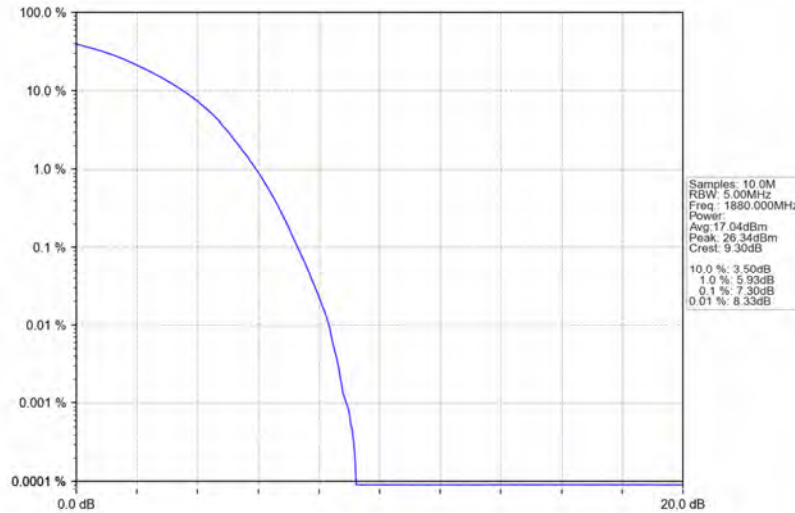
Band2_15MHz_16QAM_MCH_1880MHz_RB_75_0_NTNV
