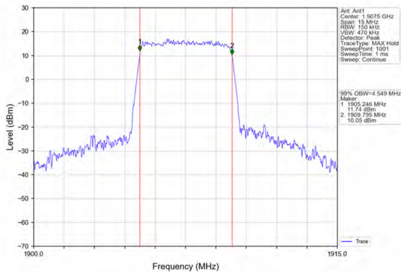
Band2_5MHz_16QAM_HCH_1907.5MHz_RB_25_0_NTNV
