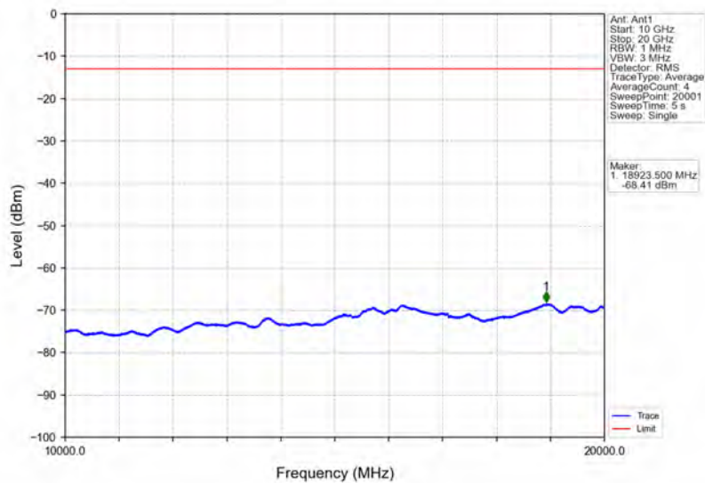
Band2_1.4MHz_16QAM_HCH_1909.3MHz_RB_1_0_NTNV
