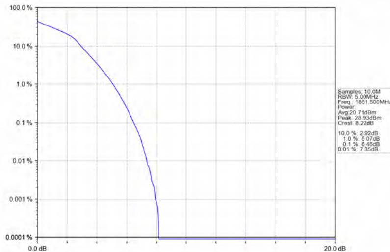
Band2_3MHz_16QAM_LCH_1851.5MHz_RB_15_0_NTNV
