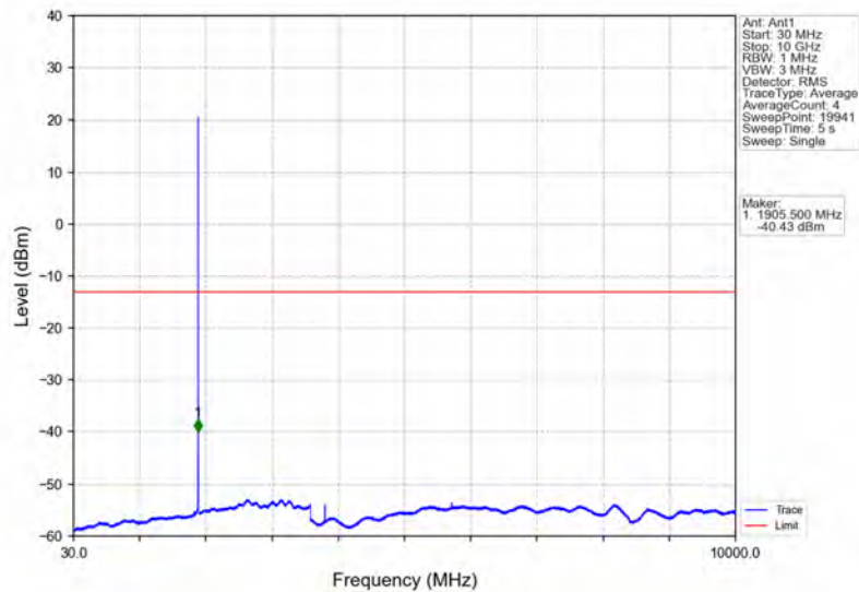
Band2_1.4MHz_64QAM_HCH_1909.3MHz_RB_1_0_NTNV
