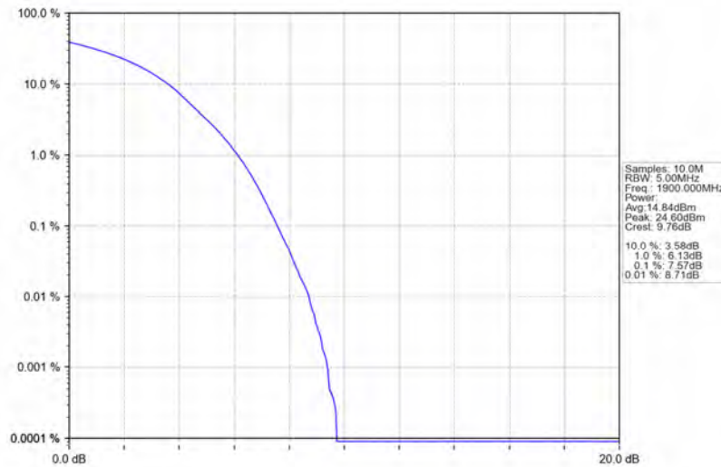
Band2_20MHz_64QAM_HCH_1900MHz_RB_100_0_NTNV
