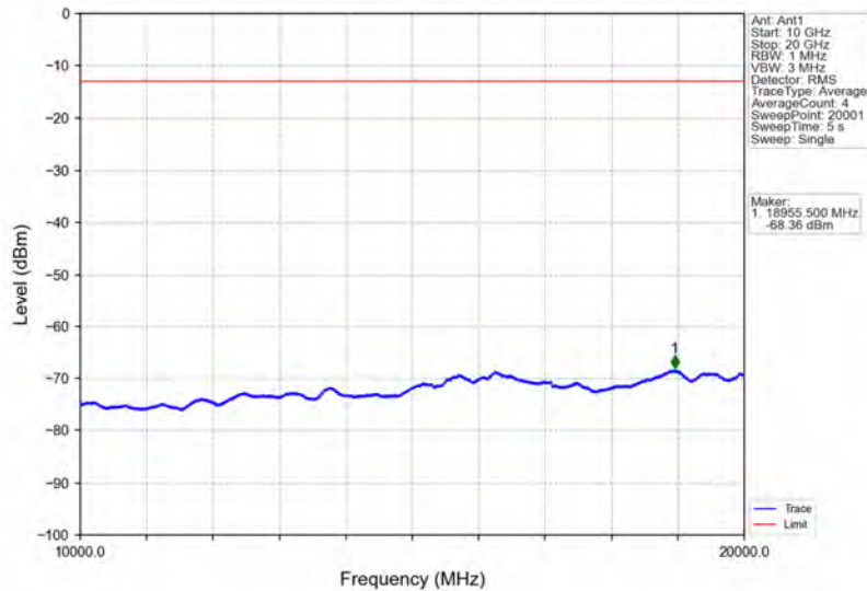
Band2_3MHz_QPSK_LCH_1851.5MHz_RB_15_0_NTNV
