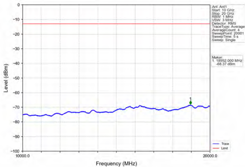
Band2_3MHz_64QAM_MCH_1880MHz_RB_1_0_NTNV
