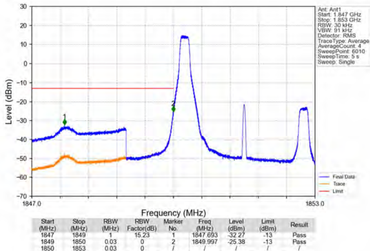
Band2_3MHz_64QAM_LCH_1851.5MHz_RB_1_0_NTNV
