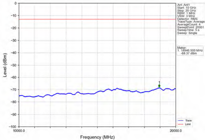
Band2_5MHz_64QAM_LCH_1852.5MHz_RB_25_0_NTNV
