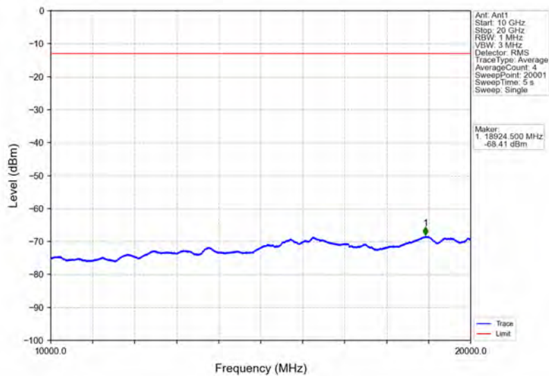
Band2_15MHz_16QAM_MCH_1880MHz_RB_1_0_NTNV
