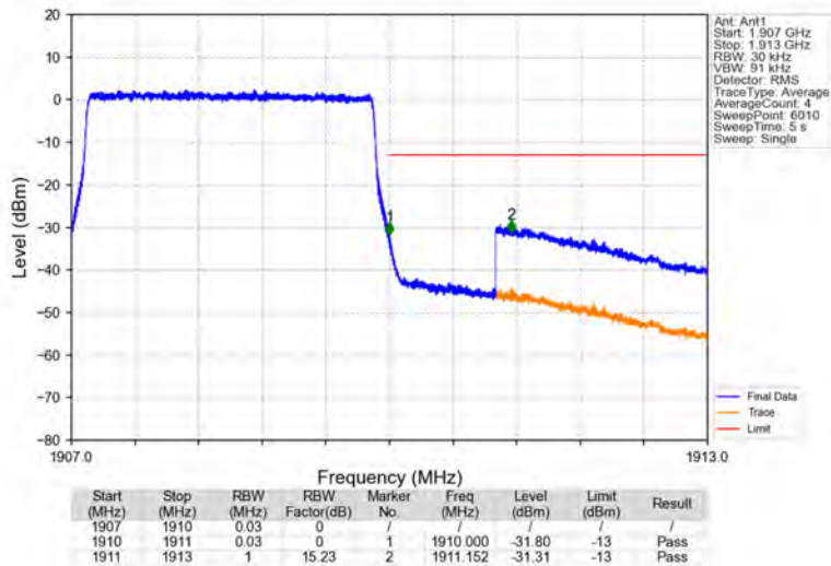
Band2_3MHz_64QAM_HCH_1908.5MHz_RB_15_0_NTNV
