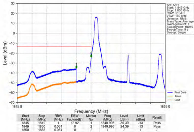
Band2_5MHz_64QAM_LCH_1852.5MHz_RB_1_0_NTNV
