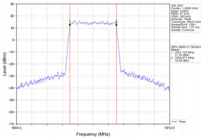
Band2_3MHz_64QAM_HCH_1908.5MHz_RB_15_0_NTNV
