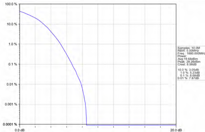
Band2_3MHz_64QAM_MCH_1880MHz_RB_15_0_NTNV
