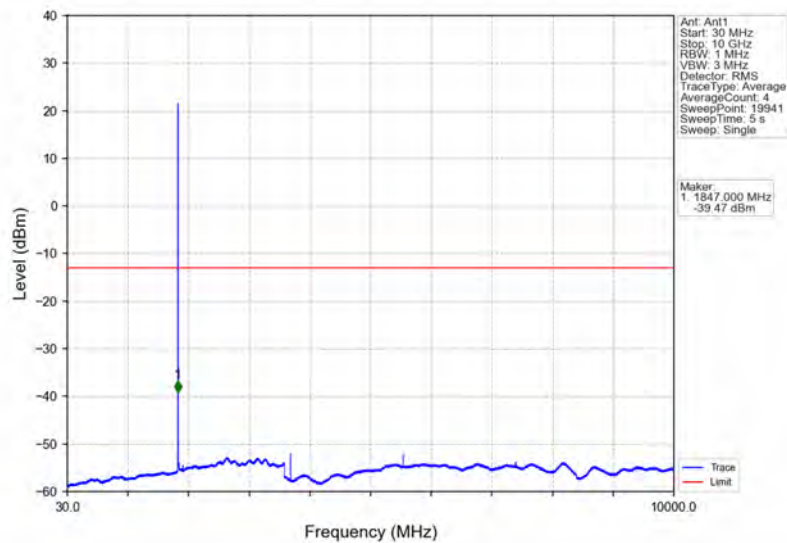
Band2_1.4MHz_16QAM_LCH_1850.7MHz_RB_1_0_NTNV
