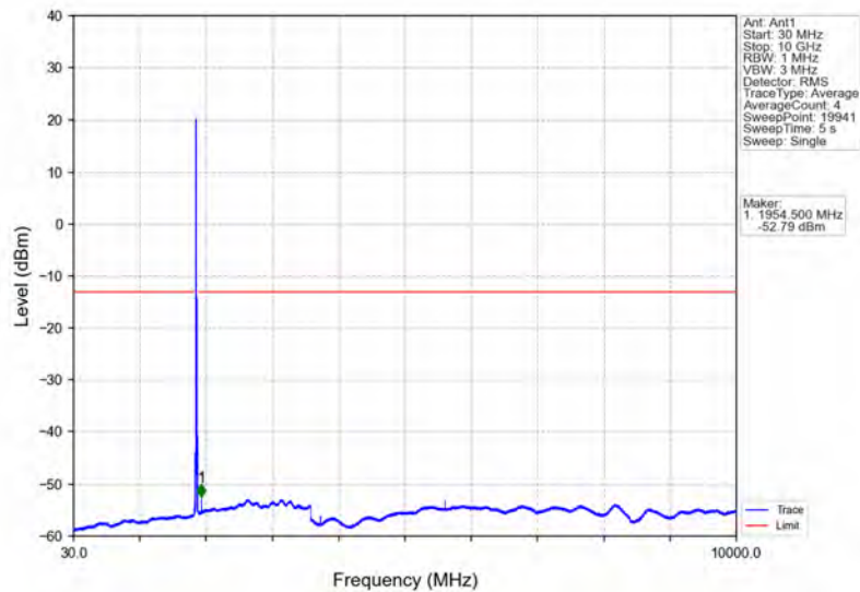
Band2_15MHz_64QAM_MCH_1880MHz_RB_1_0_NTNV
