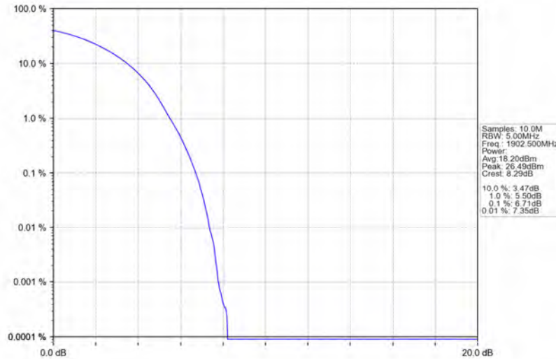
Band2_15MHz_QPSK_HCH_1902.5MHz_RB_75_0_NTNV
