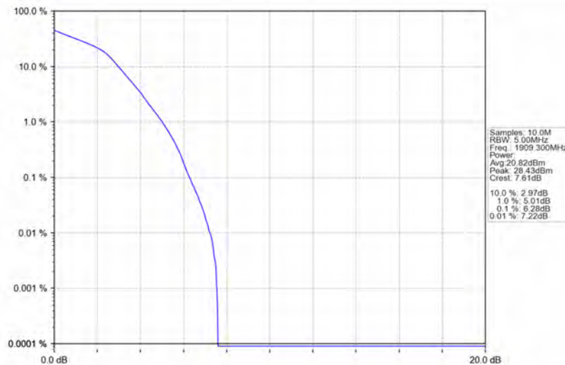
Band2_1.4MHz_16QAM_HCH_1909.3MHz_RB_6_0_NTNV
