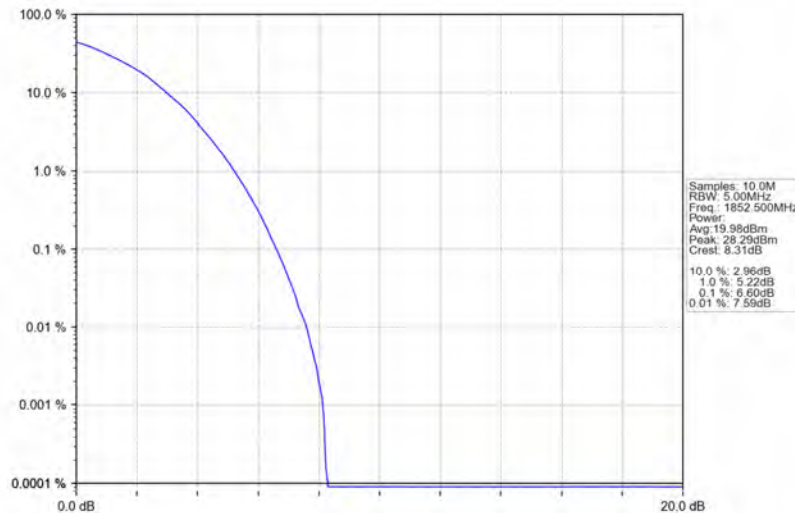
Band2_5MHz_64QAM_LCH_1852.5MHz_RB_25_0_NTNV
