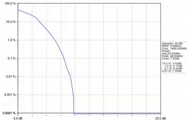
Band2_1.4MHz_16QAM_MCH_1880MHz_RB_6_0_NTNV
