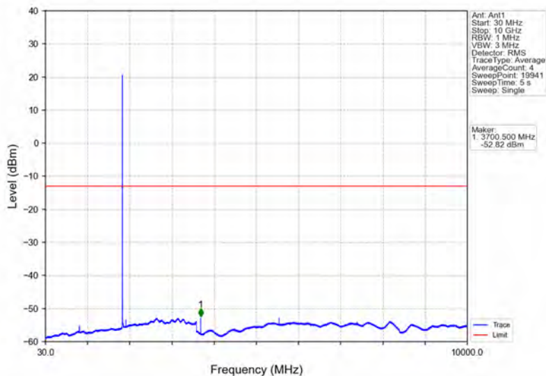
Band2_3MHz_64QAM_LCH_1851.5MHz_RB_1_0_NTNV
