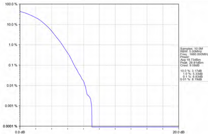
Band2_1.4MHz_64QAM_MCH_1880MHz_RB_6_0_NTNV
