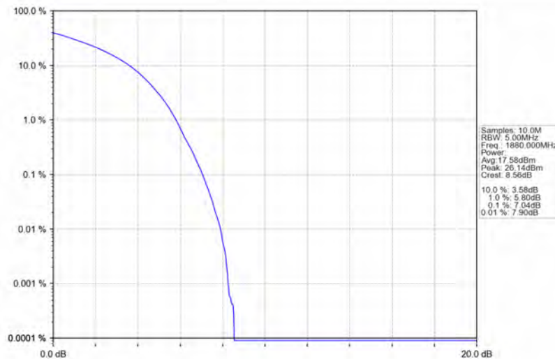
Band2_10MHz_64QAM_MCH_1880MHz_RB_50_0_NTNV
