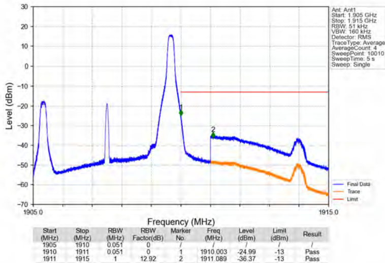
Band2_5MHz_64QAM_HCH_1907.5MHz_RB_1_24_NTNV
