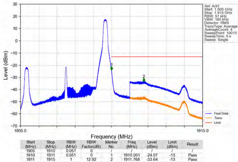
Band2_5MHz_16QAM_HCH_1907.5MHz_RB_1_24_NTNV
