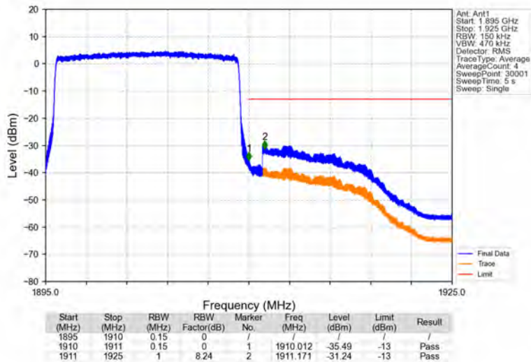
Band2_15MHz_QPSK_HCH_1902.5MHz_RB_75_0_NTNV
