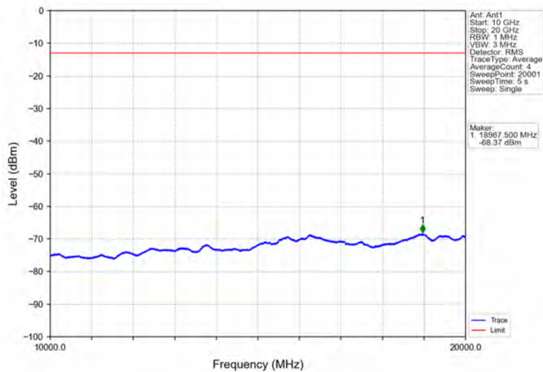
Band2_10MHz_64QAM_MCH_1880MHz_RB_1_0_NTNV
