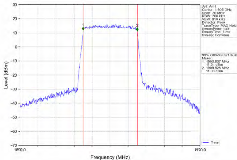
Band2_10MHz_64QAM_HCH_1905MHz_RB_50_0_NTNV
