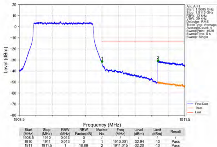
Band2_1.4MHz_QPSK_HCH_1909.3MHz_RB_6_0_NTNV
