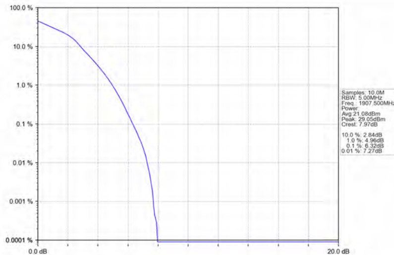
Band2_5MHz_16QAM_HCH_1907.5MHz_RB_25_0_NTNV
