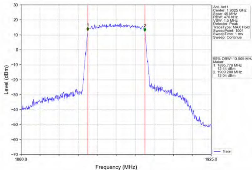
Band2_15MHz_16QAM_HCH_1902.5MHz_RB_75_0_NTNV
