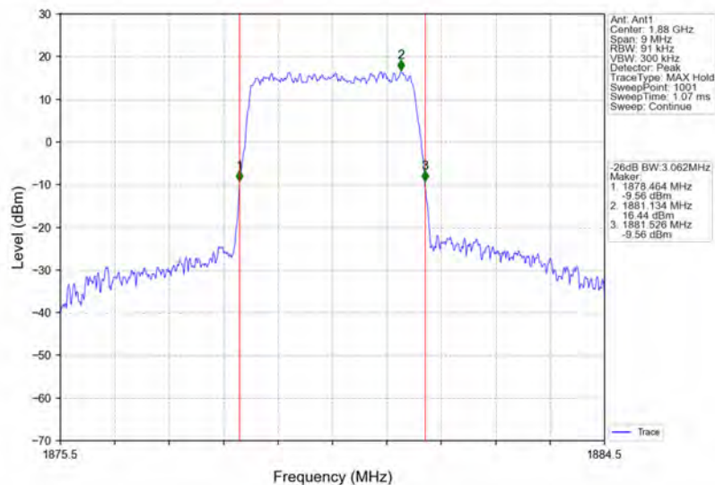
Band2_3MHz_16QAM_MCH_1880MHz_RB_15_0_NTNV
