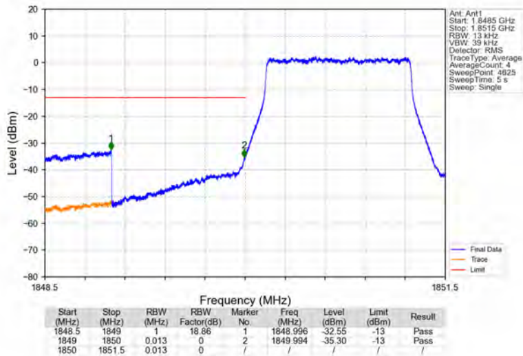
Band2_1.4MHz_64QAM_LCH_1850.7MHz_RB_6_0_NTNV
