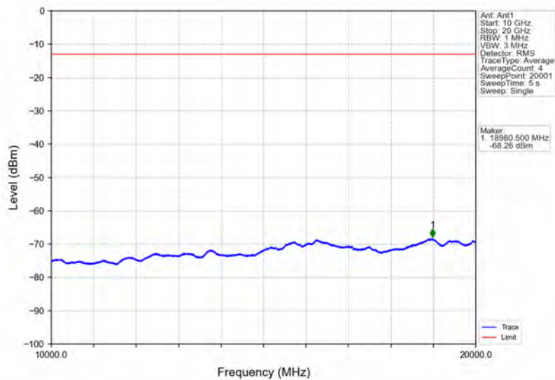
Band2_3MHz_64QAM_HCH_1908.5MHz_RB_1_0_NTNV
