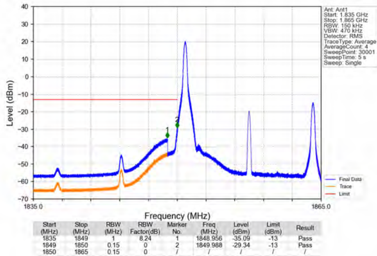
Band2_15MHz_64QAM_LCH_1857.5MHz_RB_1_0_NTNV
