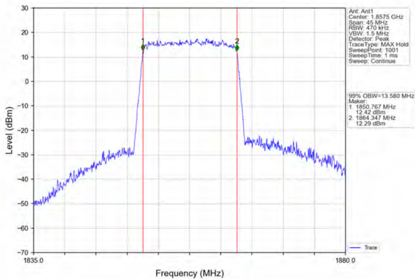
Band2_15MHz_16QAM_LCH_1857.5MHz_RB_75_0_NTNV
