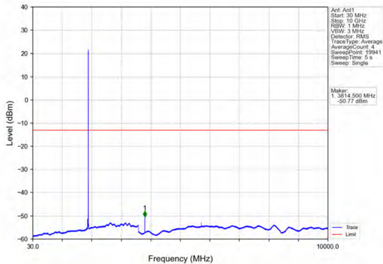
Band2_3MHz_16QAM_HCH_1908.5MHz_RB_1_0_NTNV
