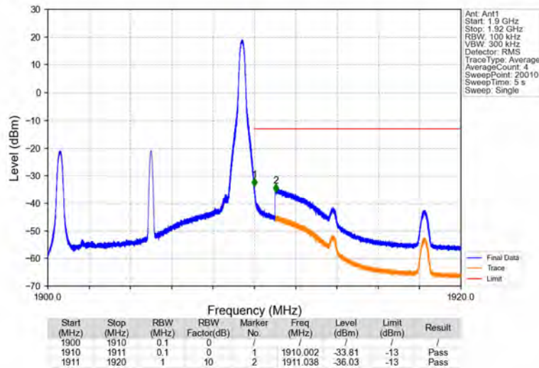
Band2_10MHz_64QAM_HCH_1905MHz_RB_1_49_NTNV
