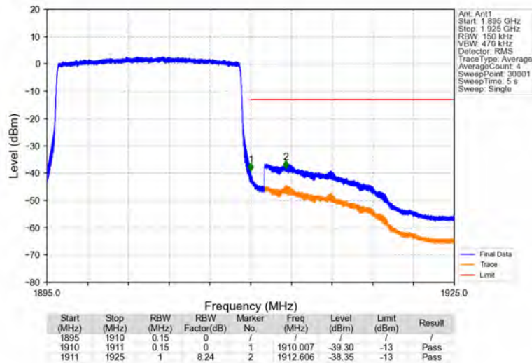
Band2_15MHz_64QAM_HCH_1902.5MHz_RB_75_0_NTNV
