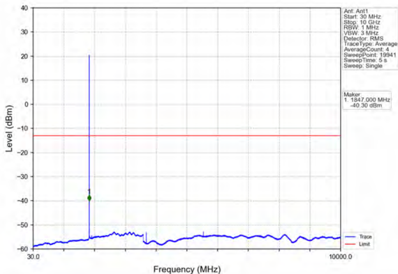
Band2_1.4MHz_64QAM_LCH_1850.7MHz_RB_1_0_NTNV
