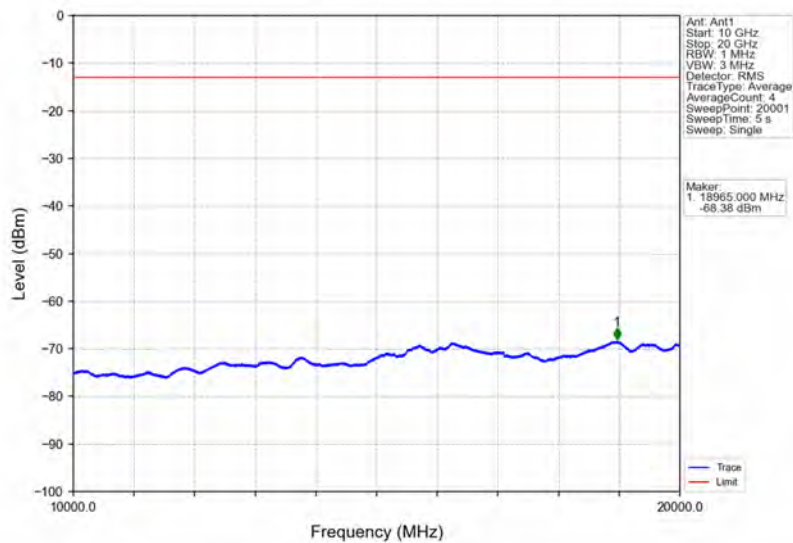
Band2_1.4MHz_64QAM_HCH_1909.3MHz_RB_1_0_NTNV
