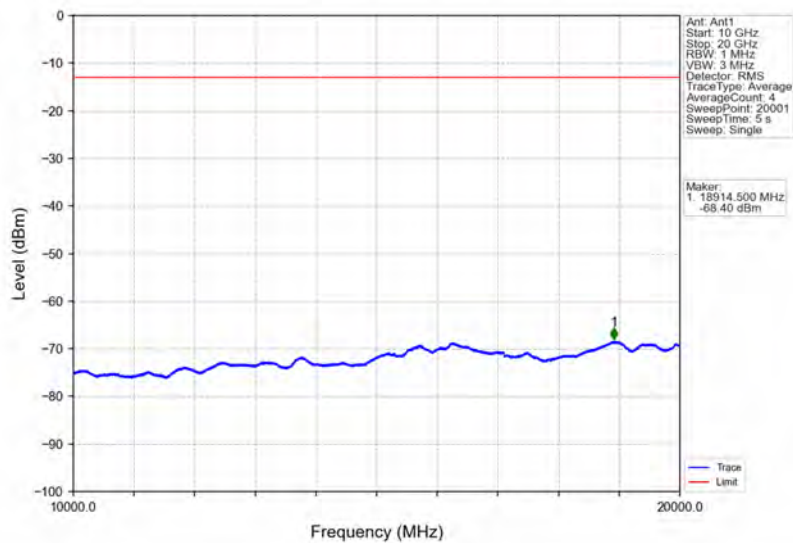
Band2_15MHz_64QAM_MCH_1880MHz_RB_1_0_NTNV
