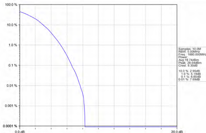
Band2_5MHz_64QAM_MCH_1880MHz_RB_25_0_NTNV
