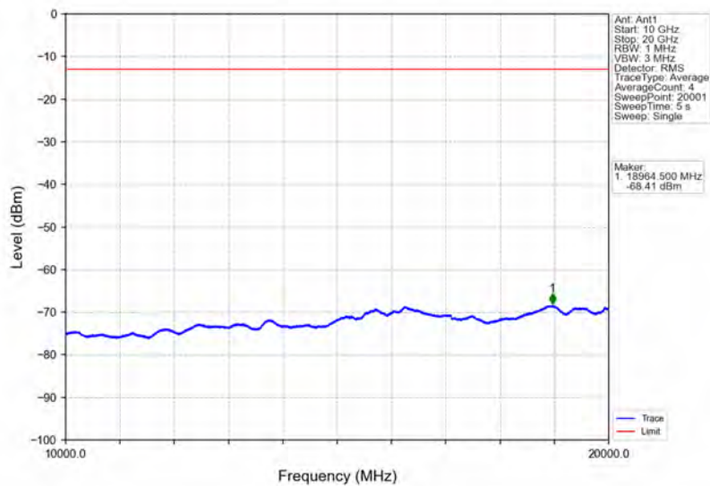
Band2_15MHz_16QAM_HCH_1902.5MHz_RB_1_0_NTNV
