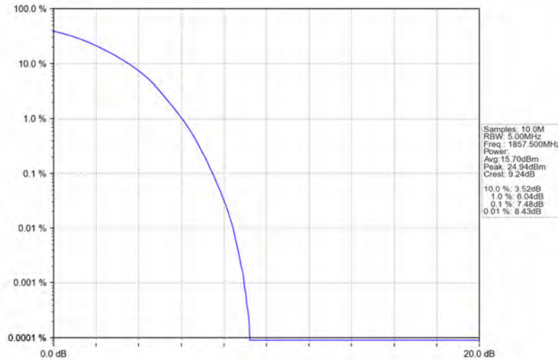
Band2_15MHz_64QAM_LCH_1857.5MHz_RB_75_0_NTNV
