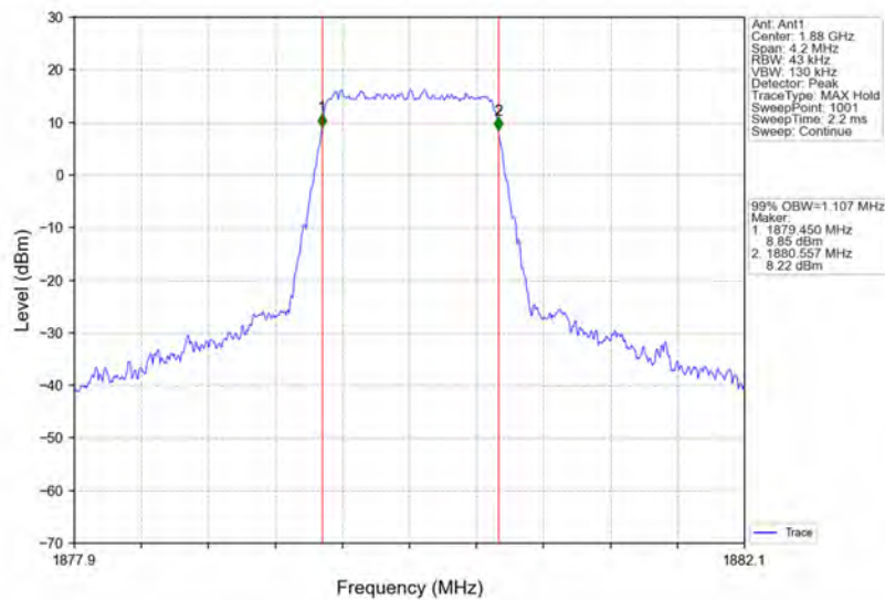
Band2_1.4MHz_64QAM_MCH_1880MHz_RB_6_0_NTNV
