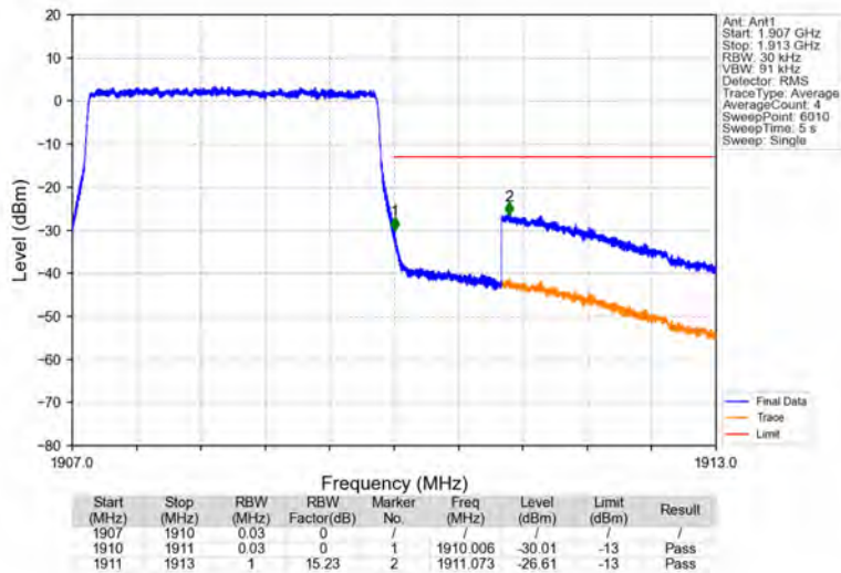
Band2_3MHz_16QAM_HCH_1908.5MHz_RB_15_0_NTNV
