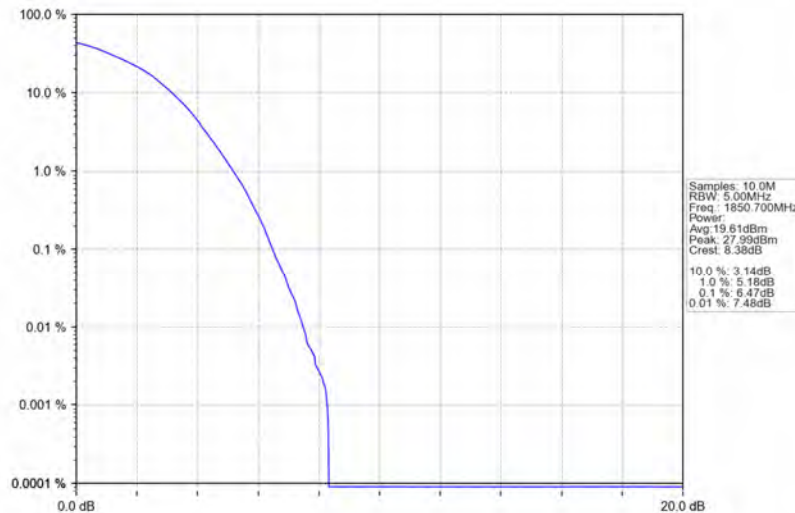
Band2_1.4MHz_64QAM_LCH_1850.7MHz_RB_6_0_NTNV
