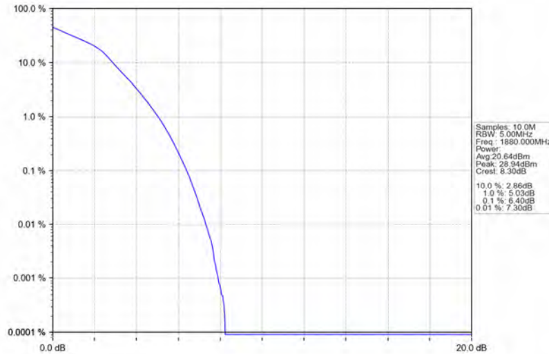
Band2_5MHz_16QAM_MCH_1880MHz_RB_25_0_NTNV
