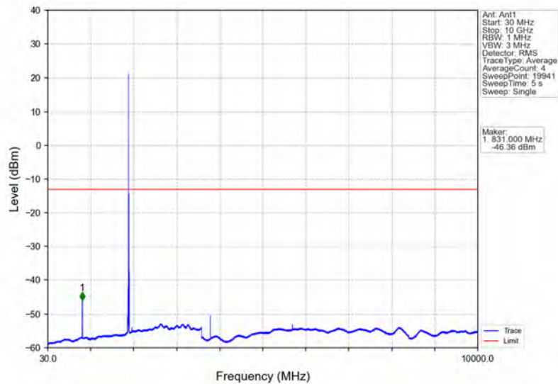
Band2_10MHz_64QAM_HCH_1905MHz_RB_1_0_NTNV
