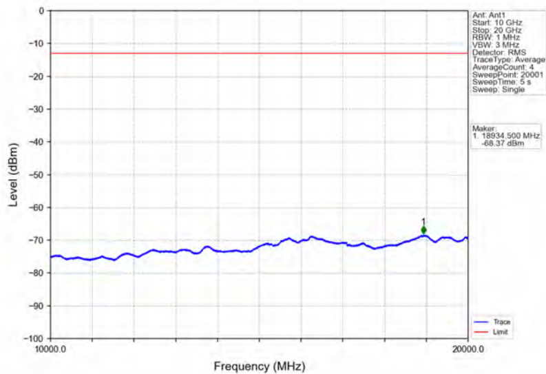
Band2_5MHz_16QAM_MCH_1880MHz_RB_1_0_NTNV
