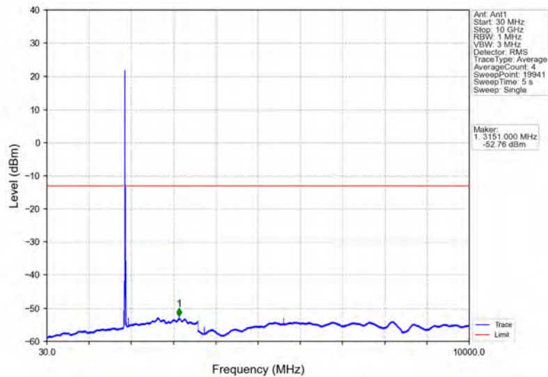
Band2_15MHz_16QAM_MCH_1880MHz_RB_1_0_NTNV
