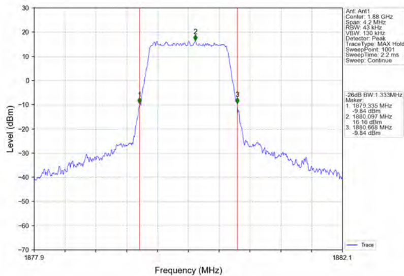
Band2_1.4MHz_64QAM_MCH_1880MHz_RB_6_0_NTNV
