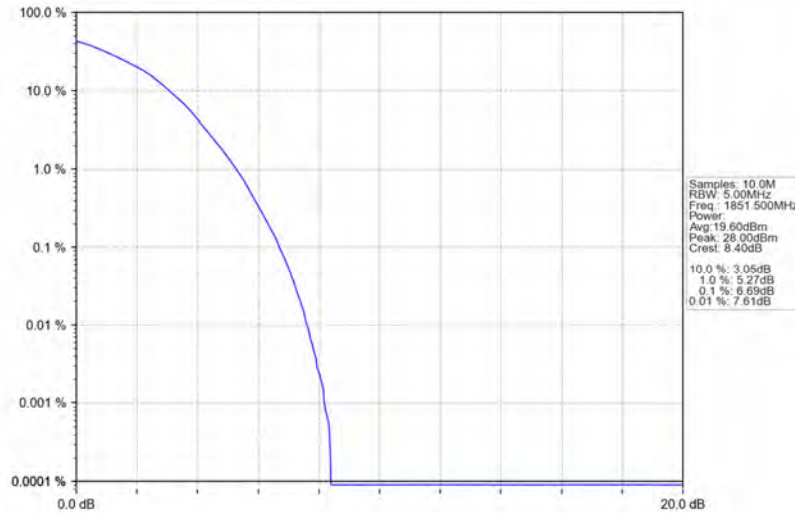
Band2_3MHz_64QAM_LCH_1851.5MHz_RB_15_0_NTNV
