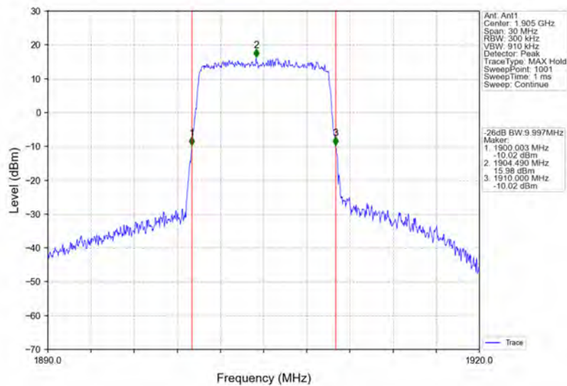
Band2_10MHz_64QAM_HCH_1905MHz_RB_50_0_NTNV
