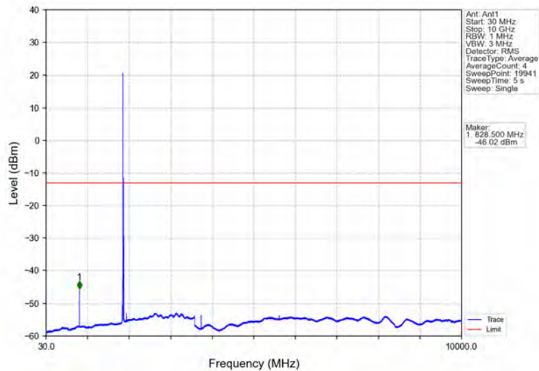
Band2_10MHz_64QAM_MCH_1880MHz_RB_1_0_NTNV
