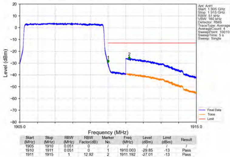
Band2_5MHz_QPSK_HCH_1907.5MHz_RB_25_0_NTNV
