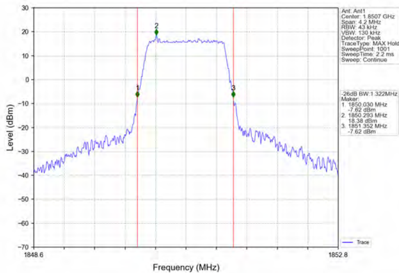
Band2_1.4MHz_16QAM_LCH_1850.7MHz_RB_6_0_NTNV
