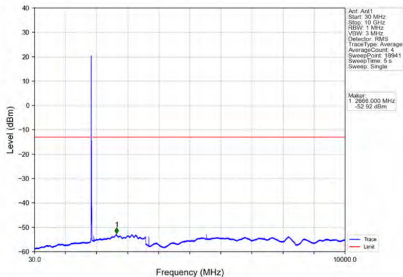
Band2_15MHz_64QAM_LCH_1857.5MHz_RB_1_0_NTNV
