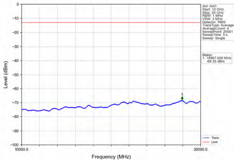
Band2_15MHz_64QAM_LCH_1857.5MHz_RB_75_0_NTNV
