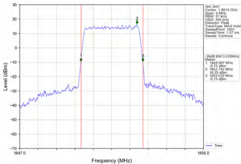
Band2_3MHz_64QAM_LCH_1851.5MHz_RB_15_0_NTNV
