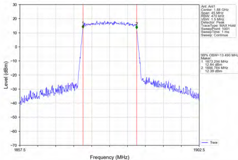
Band2_15MHz_QPSK_MCH_1880MHz_RB_75_0_NTNV
