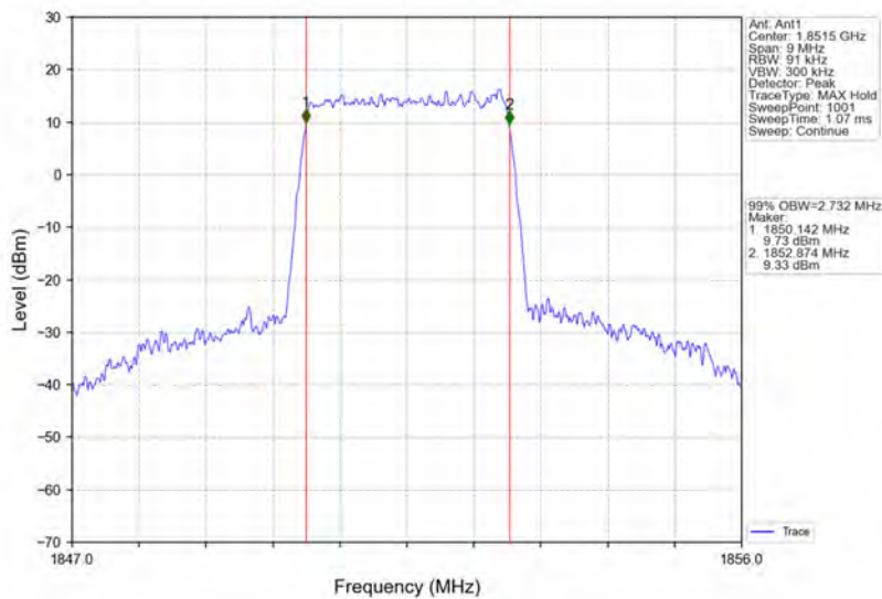
Band2_3MHz_64QAM_LCH_1851.5MHz_RB_15_0_NTNV
