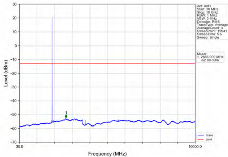
Band2_3MHz_64QAM_MCH_1880MHz_RB_1_0_NTNV
