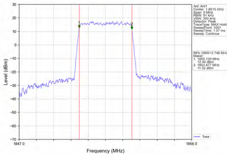
Band2_3MHz_QPSK_LCH_1851.5MHz_RB_15_0_NTNV
