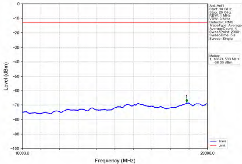
Band2_3MHz_64QAM_LCH_1851.5MHz_RB_15_0_NTNV
