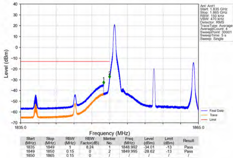
Band2_15MHz_16QAM_LCH_1857.5MHz_RB_1_0_NTNV
