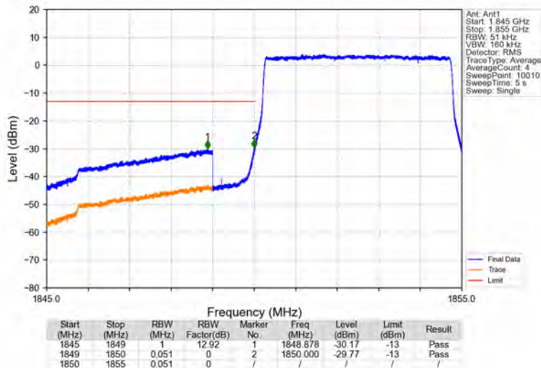
Band2_5MHz_QPSK_LCH_1852.5MHz_RB_25_0_NTNV
