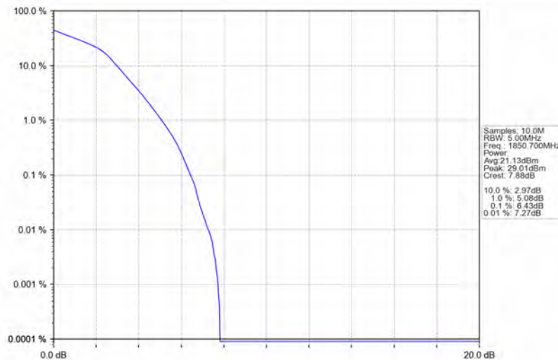
Band2_1.4MHz_16QAM_LCH_1850.7MHz_RB_6_0_NTNV
