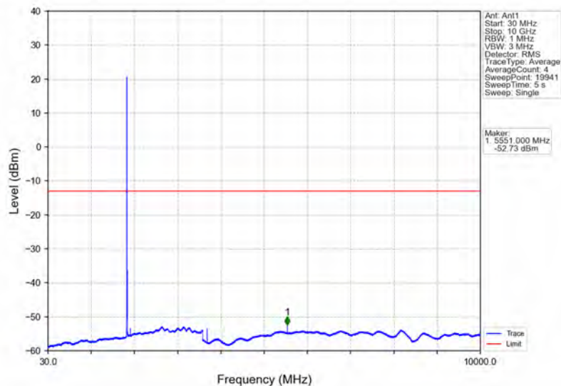
Band2_5MHz_64QAM_LCH_1852.5MHz_RB_1_0_NTNV
