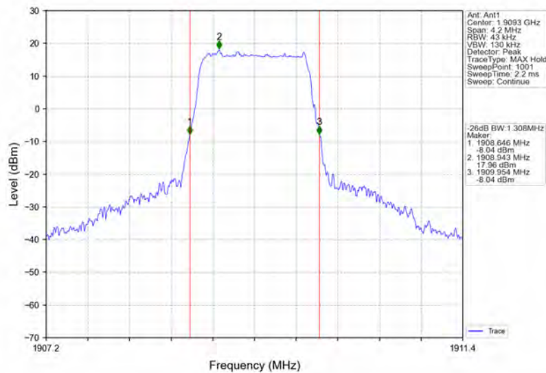
Band2_1.4MHz_16QAM_HCH_1909.3MHz_RB_6_0_NTNV
