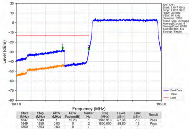
Band2_3MHz_QPSK_LCH_1851.5MHz_RB_15_0_NTNV
