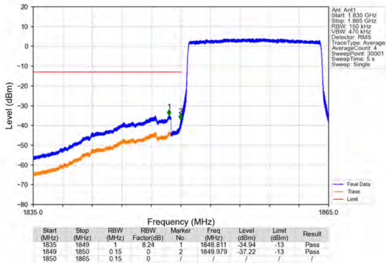
Band2_15MHz_QPSK_LCH_1857.5MHz_RB_75_0_NTNV
