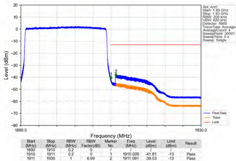
Band2_20MHz_64QAM_HCH_1900MHz_RB_100_0_NTNV
