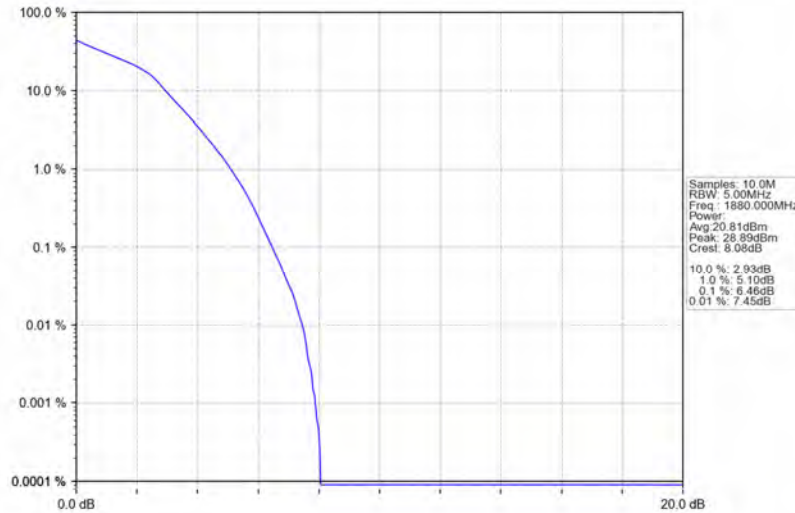
Band2_3MHz_16QAM_MCH_1880MHz_RB_15_0_NTNV
