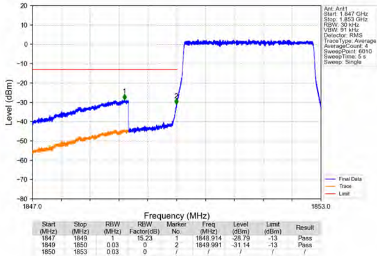
Band2_3MHz_64QAM_LCH_1851.5MHz_RB_15_0_NTNV
