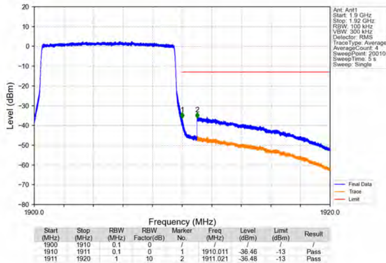
Band2_10MHz_64QAM_HCH_1905MHz_RB_50_0_NTNV
