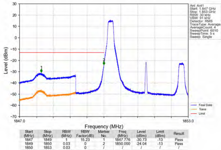
Band2_3MHz_16QAM_LCH_1851.5MHz_RB_1_0_NTNV
