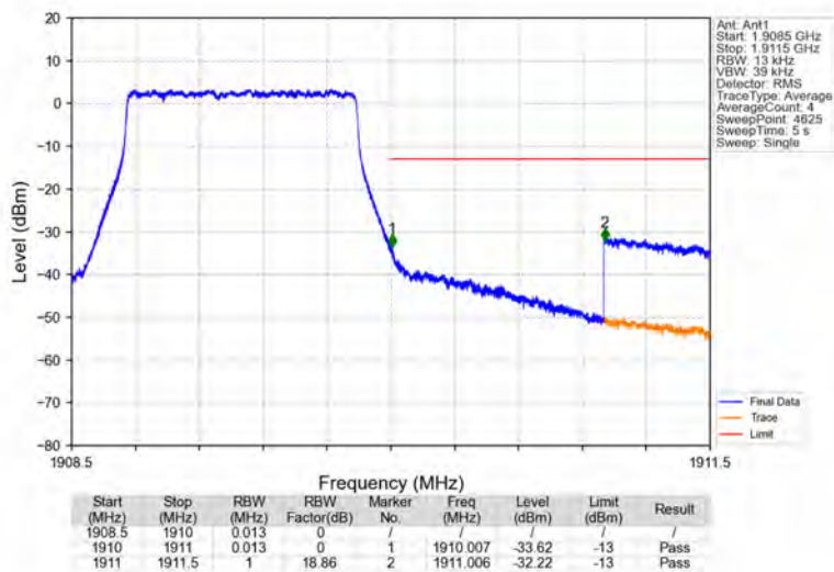
Band2_1.4MHz_16QAM_HCH_1909.3MHz_RB_6_0_NTNV
