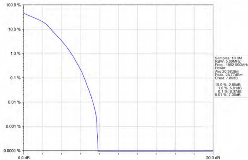
Band2_5MHz_16QAM_LCH_1852.5MHz_RB_25_0_NTNV
