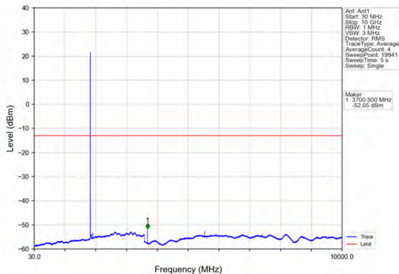
Band2_3MHz_16QAM_LCH_1851.5MHz_RB_1_0_NTNV
