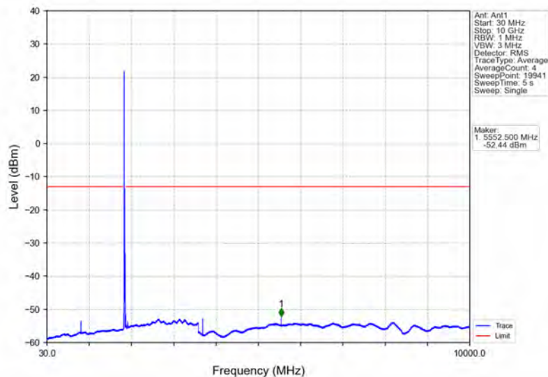
Band2_15MHz_16QAM_LCH_1857.5MHz_RB_1_0_NTNV
