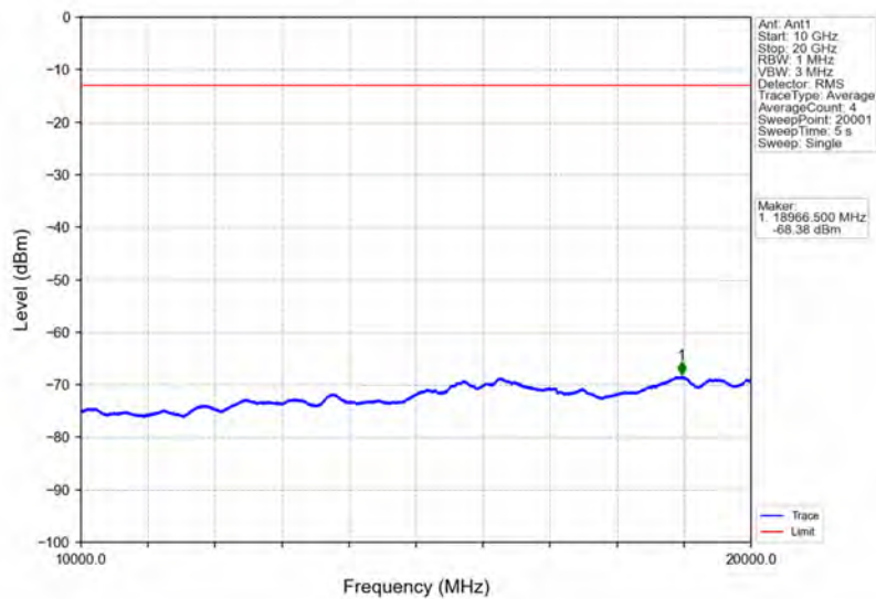
Band2_20MHz_64QAM_HCH_1900MHz_RB_1_0_NTNV
