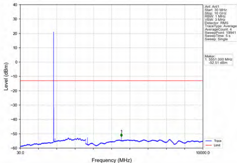
Band2_5MHz_16QAM_LCH_1852.5MHz_RB_1_0_NTNV
