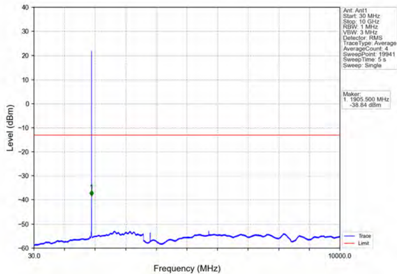
Band2_1.4MHz_16QAM_HCH_1909.3MHz_RB_1_0_NTNV
