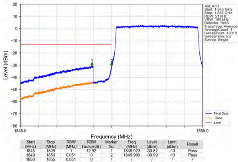
Band2_5MHz_16QAM_LCH_1852.5MHz_RB_25_0_NTNV
