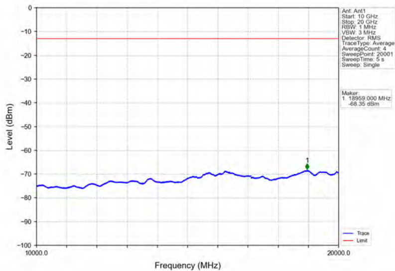
Band2_5MHz_16QAM_HCH_1907.5MHz_RB_1_0_NTNV
