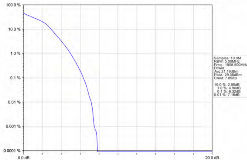
Band2_3MHz_16QAM_HCH_1908.5MHz_RB_15_0_NTNV
