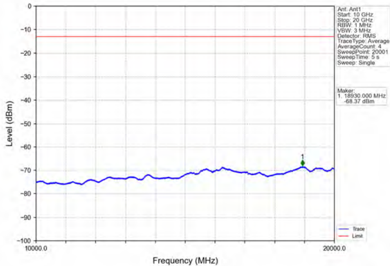
Band2_15MHz_16QAM_LCH_1857.5MHz_RB_75_0_NTNV
