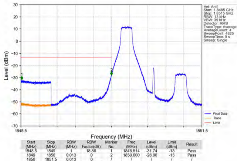
Band2_1.4MHz_16QAM_LCH_1850.7MHz_RB_1_0_NTNV
