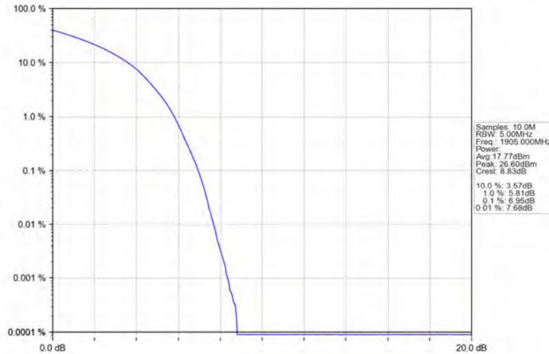
Band2_10MHz_64QAM_HCH_1905MHz_RB_50_0_NTNV
