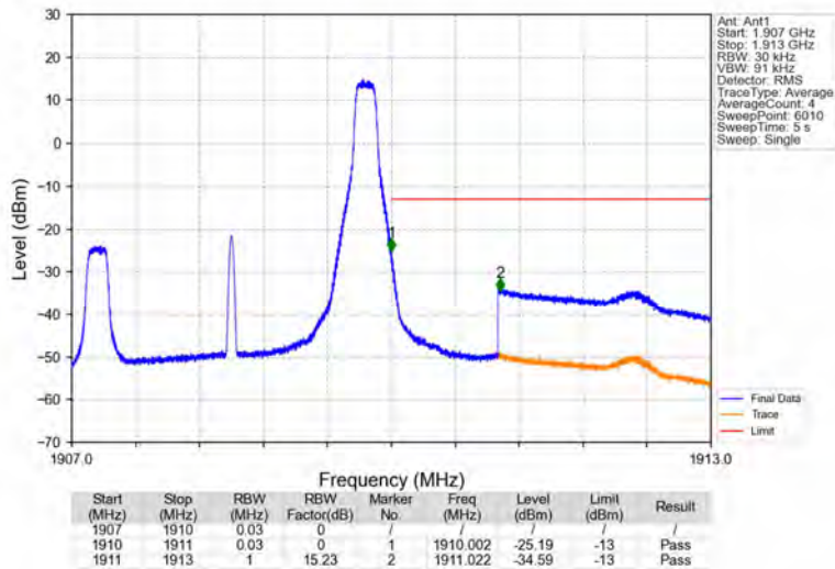
Band2_3MHz_64QAM_HCH_1908.5MHz_RB_1_14_NTNV
