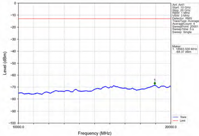
Band2_5MHz_QPSK_LCH_1852.5MHz_RB_25_0_NTNV
