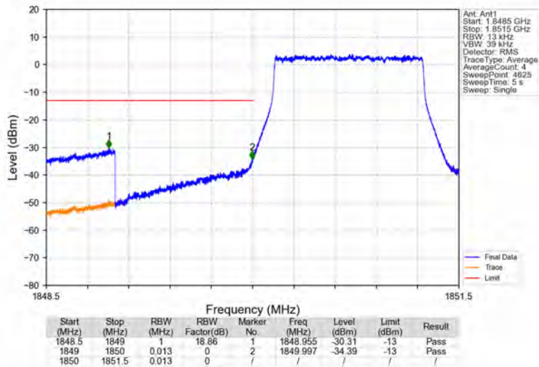
Band2_1.4MHz_16QAM_LCH_1850.7MHz_RB_6_0_NTNV
