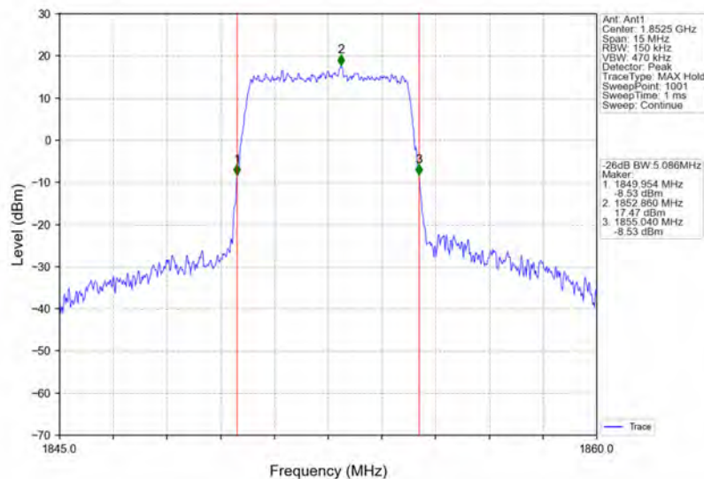
Band2_5MHz_16QAM_LCH_1852.5MHz_RB_25_0_NTNV
