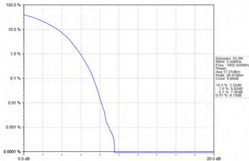
Band2_15MHz_16QAM_HCH_1902.5MHz_RB_75_0_NTNV
