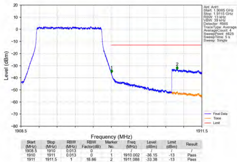
Band2_1.4MHz_64QAM_HCH_1909.3MHz_RB_6_0_NTNV
