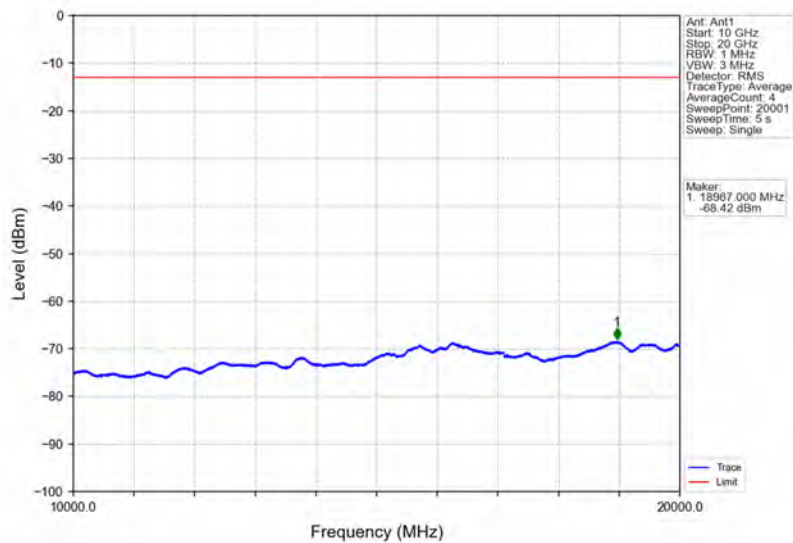
Band2_1.4MHz_64QAM_MCH_1880MHz_RB_1_0_NTNV
