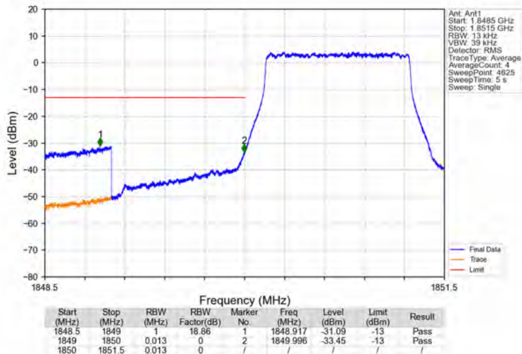
Band2_1.4MHz_QPSK_LCH_1850.7MHz_RB_6_0_NTNV
