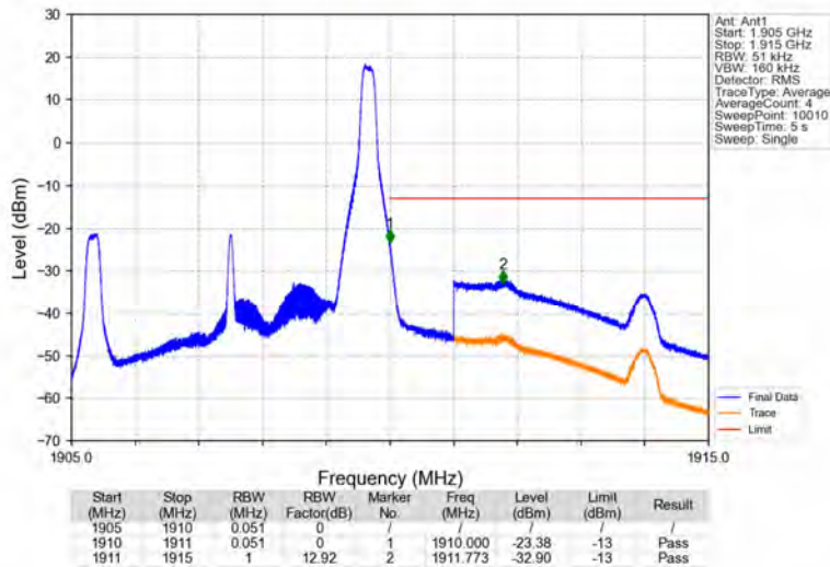
Band2_5MHz_QPSK_HCH_1907.5MHz_RB_1_24_NTNV
