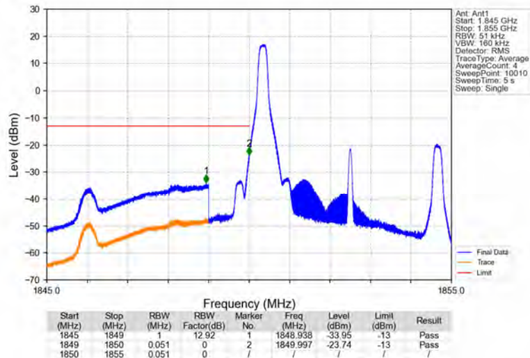
Band2_5MHz_16QAM_LCH_1852.5MHz_RB_1_0_NTNV
