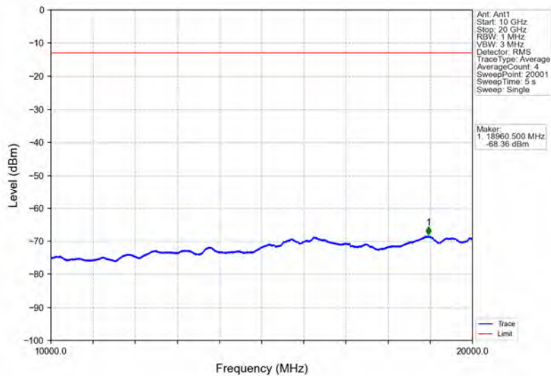
Band2_1.4MHz_16QAM_LCH_1850.7MHz_RB_6_0_NTNV
