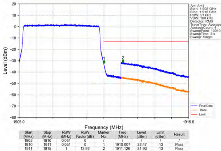
Band2_5MHz_64QAM_HCH_1907.5MHz_RB_25_0_NTNV
