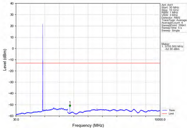
Band2_5MHz_16QAM_MCH_1880MHz_RB_1_0_NTNV
