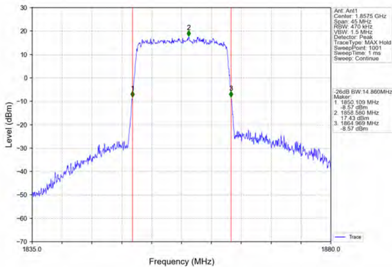
Band2_15MHz_16QAM_LCH_1857.5MHz_RB_75_0_NTNV
