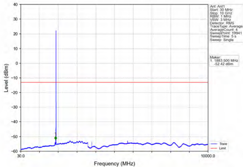
Band2_5MHz_QPSK_HCH_1907.5MHz_RB_1_0_NTNV
