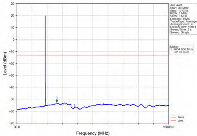
Band2_5MHz_64QAM_HCH_1907.5MHz_RB_1_0_NTNV
