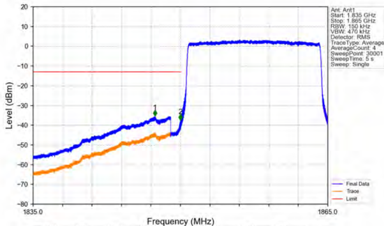
Band2_15MHz_16QAM_LCH_1857.5MHz_RB_75_0_NTNV
