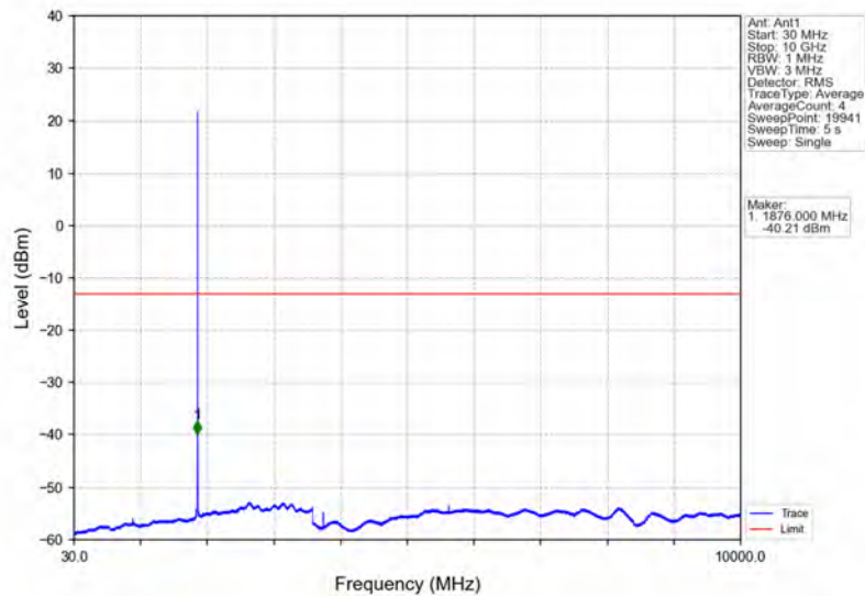
Band2_1.4MHz_16QAM_MCH_1880MHz_RB_1_0_NTNV
