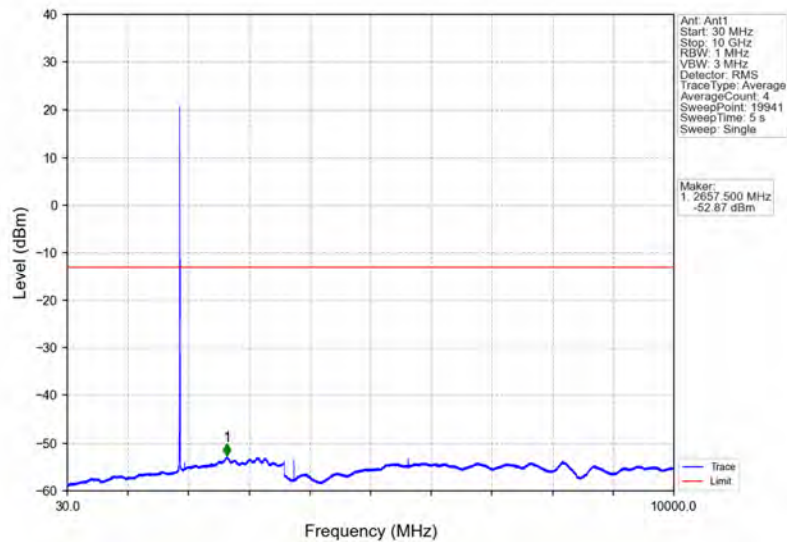
Band2_5MHz_64QAM_MCH_1880MHz_RB_1_0_NTNV
