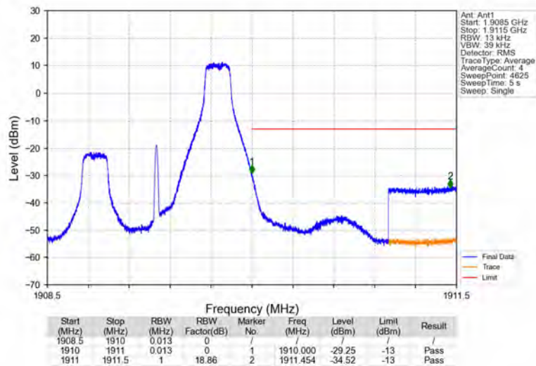
Band2_1.4MHz_64QAM_HCH_1909.3MHz_RB_1_5_NTNV
