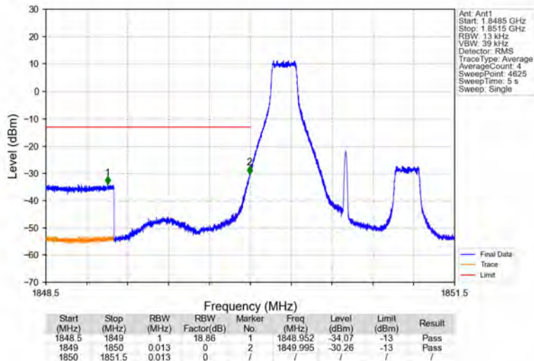
Band2_1.4MHz_64QAM_LCH_1850.7MHz_RB_1_0_NTNV
