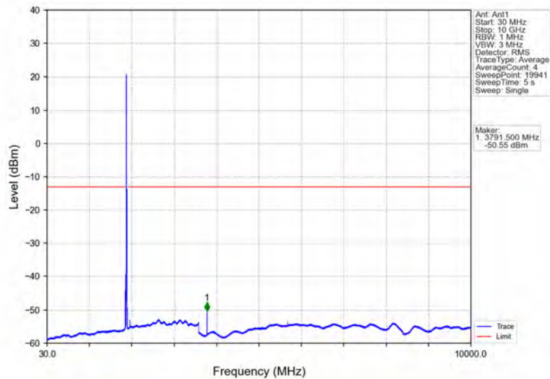
Band2_15MHz_64QAM_HCH_1902.5MHz_RB_1_0_NTNV
