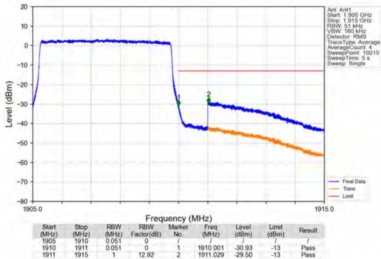
Band2_5MHz_16QAM_HCH_1907.5MHz_RB_25_0_NTNV
