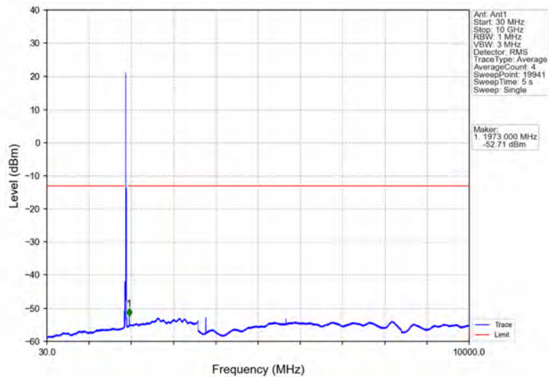
Band2_20MHz_64QAM_HCH_1900MHz_RB_1_0_NTNV
