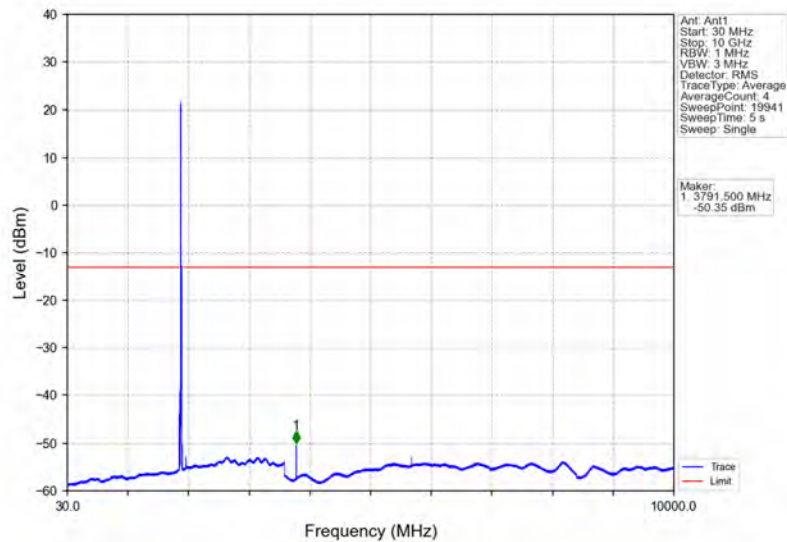
Band2_15MHz_16QAM_HCH_1902.5MHz_RB_1_0_NTNV
