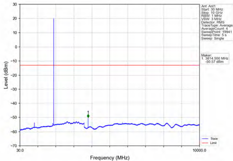
Band2_3MHz_64QAM_HCH_1908.5MHz_RB_1_0_NTNV
