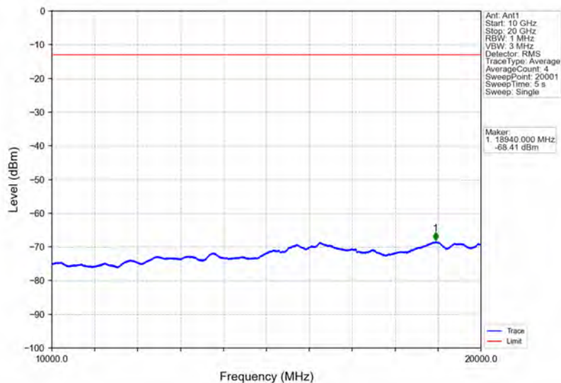
Band2_1.4MHz_16QAM_MCH_1880MHz_RB_1_0_NTNV
