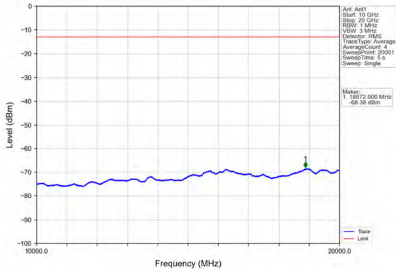
Band2_3MHz_16QAM_LCH_1851.5MHz_RB_15_0_NTNV
