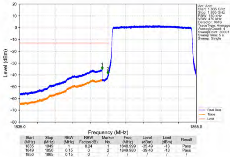
Band2_15MHz_64QAM_LCH_1857.5MHz_RB_75_0_NTNV
