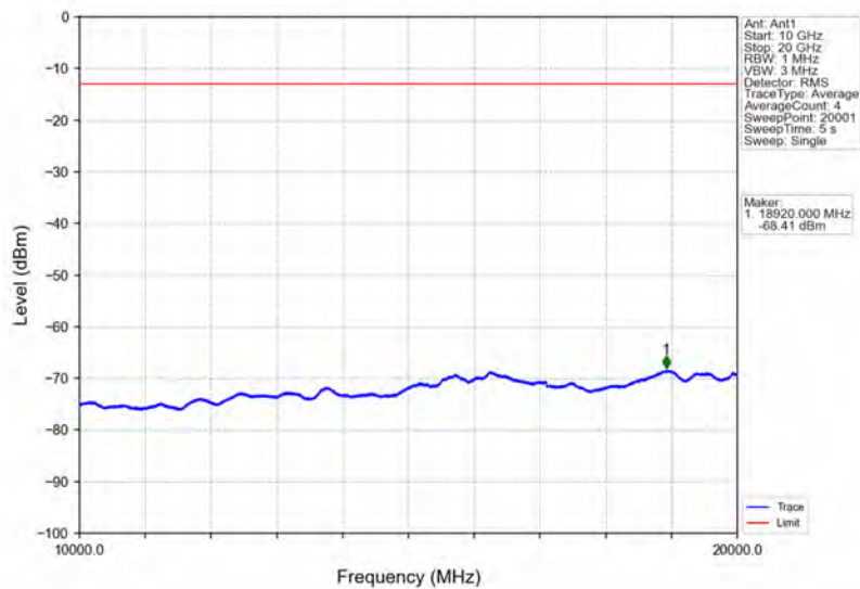
Band2_5MHz_64QAM_HCH_1907.5MHz_RB_1_0_NTNV
