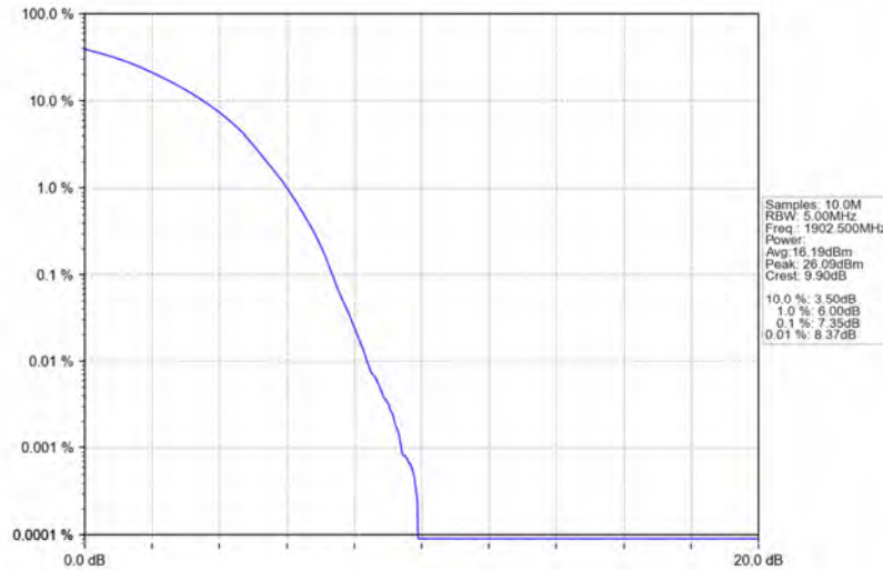
Band2_15MHz_64QAM_HCH_1902.5MHz_RB_75_0_NTNV
