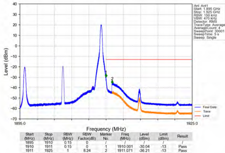
Band2_15MHz_64QAM_HCH_1902.5MHz_RB_1_74_NTNV
