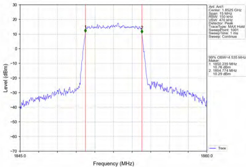
Band2_5MHz_16QAM_LCH_1852.5MHz_RB_25_0_NTNV
