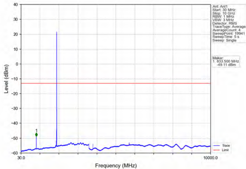
Band2_5MHz_16QAM_HCH_1907.5MHz_RB_1_0_NTNV
