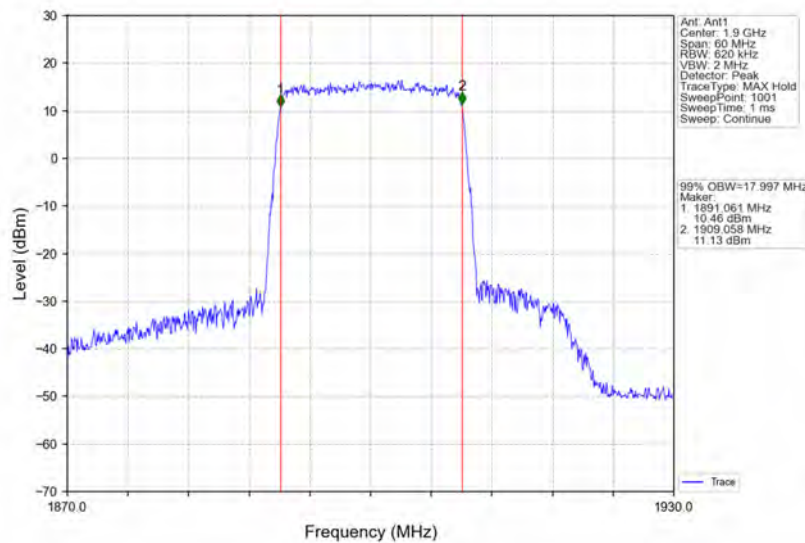
Band2_20MHz_64QAM_HCH_1900MHz_RB_100_0_NTNV
