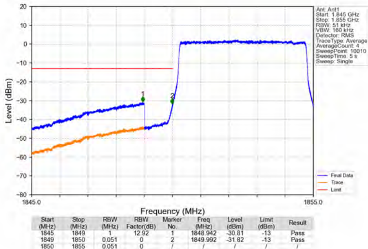
Band2_5MHz_64QAM_LCH_1852.5MHz_RB_25_0_NTNV
