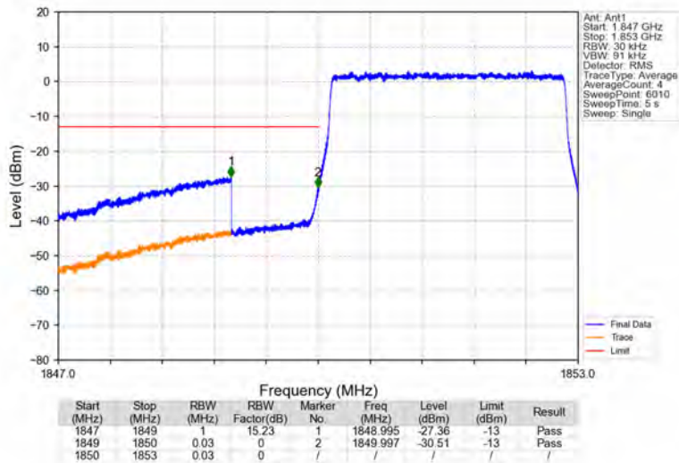
Band2_3MHz_16QAM_LCH_1851.5MHz_RB_15_0_NTNV
