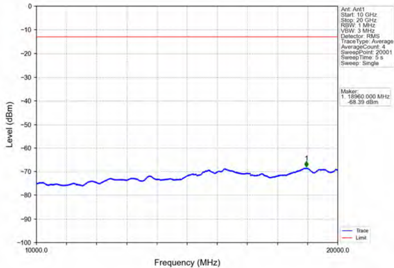
Band2_1.4MHz_64QAM_LCH_1850.7MHz_RB_6_0_NTNV
