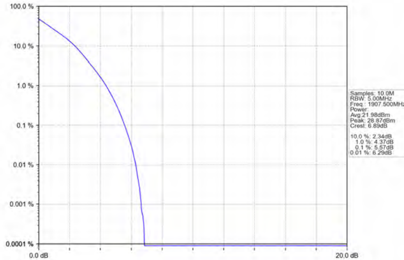
Band2_5MHz_QPSK_HCH_1907.5MHz_RB_25_0_NTNV
