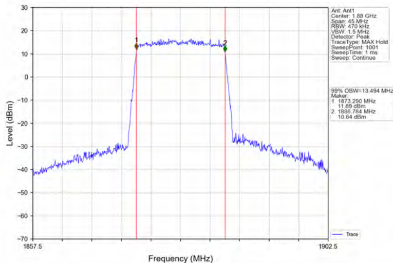
Band2_15MHz_64QAM_MCH_1880MHz_RB_75_0_NTNV
