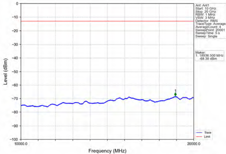
Band2_15MHz_QPSK_LCH_1857.5MHz_RB_75_0_NTNV
