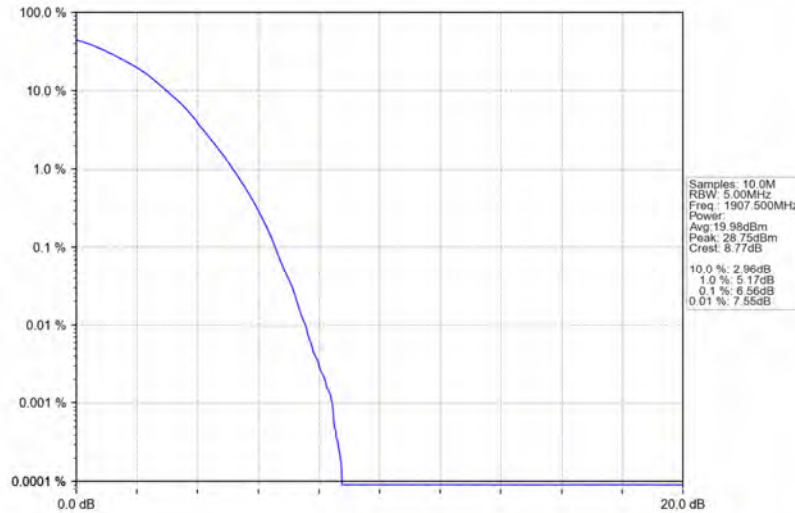
Band2_5MHz_64QAM_HCH_1907.5MHz_RB_25_0_NTNV
