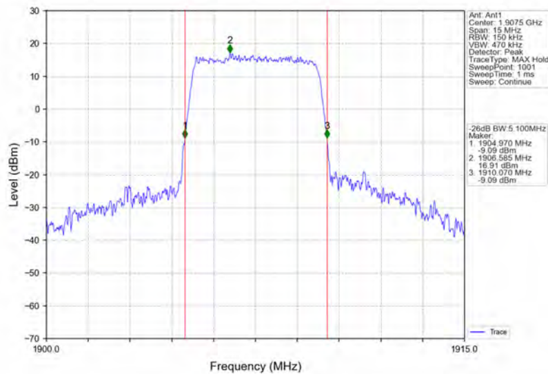
Band2_5MHz_16QAM_HCH_1907.5MHz_RB_25_0_NTNV
