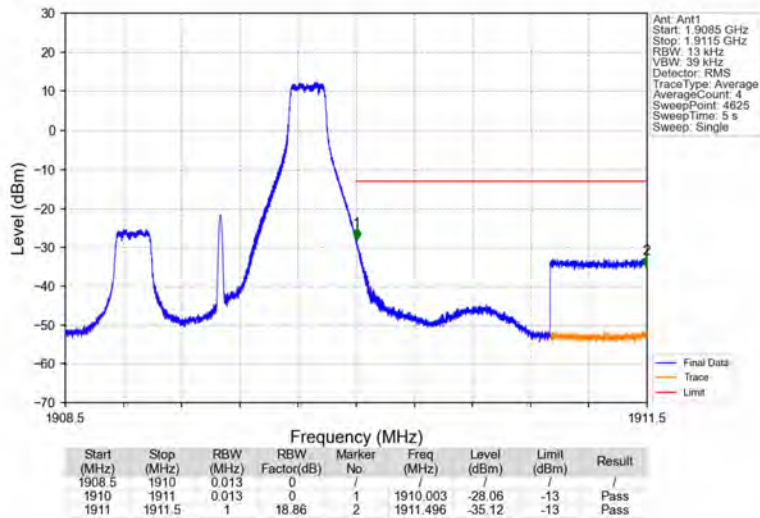
Band2_1.4MHz_16QAM_HCH_1909.3MHz_RB_1_5_NTNV
