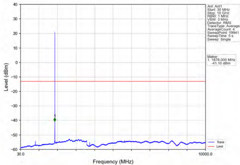
Band2_1.4MHz_64QAM_MCH_1880MHz_RB_1_0_NTNV
