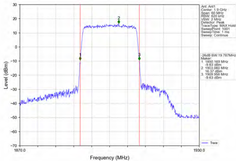
Band2_20MHz_64QAM_HCH_1900MHz_RB_100_0_NTNV
