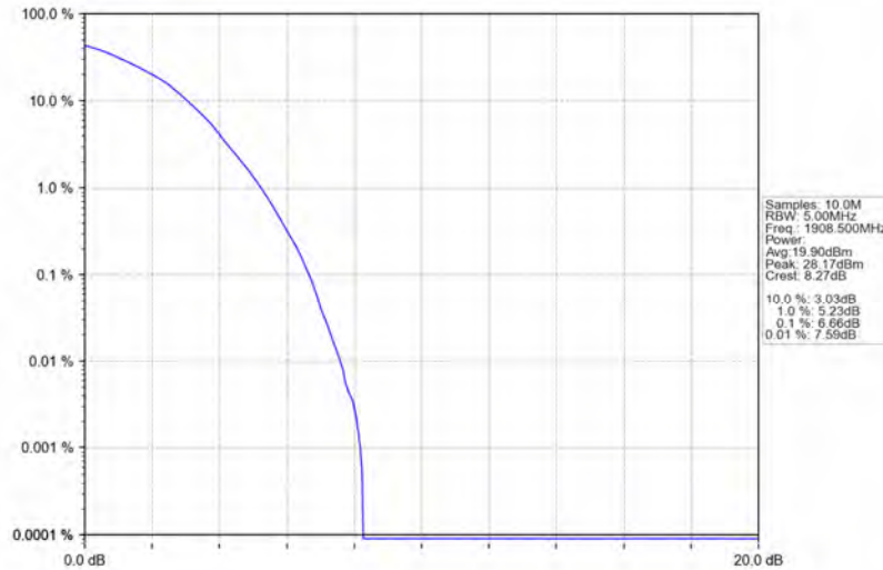
Band2_3MHz_64QAM_HCH_1908.5MHz_RB_15_0_NTNV
