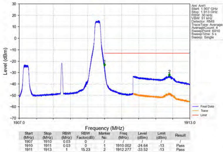
Band2_3MHz_16QAM_HCH_1908.5MHz_RB_1_14_NTNV
