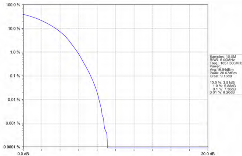
Band2_15MHz_16QAM_LCH_1857.5MHz_RB_75_0_NTNV
