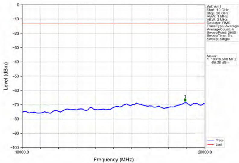
Band2_5MHz_64QAM_MCH_1880MHz_RB_1_0_NTNV
