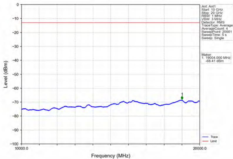
Band2_15MHz_64QAM_HCH_1902.5MHz_RB_1_0_NTNV
