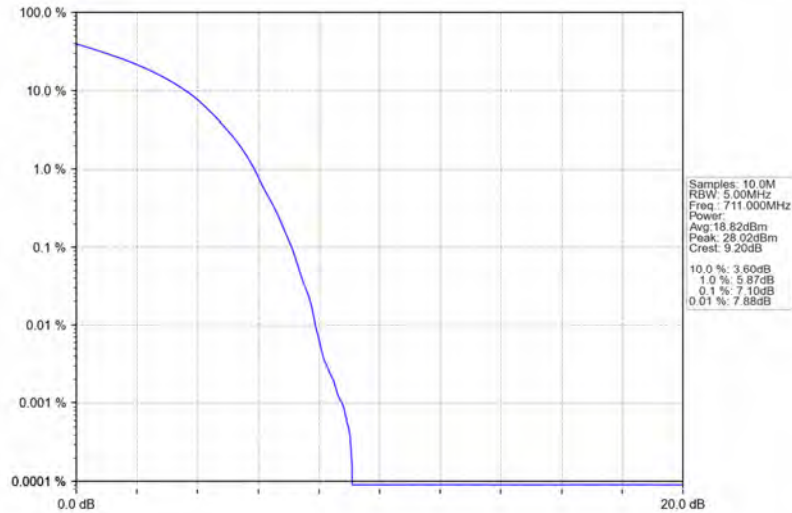
Band17_10MHz_64QAM_HCH_711MHz_RB_50_0_NTNV
