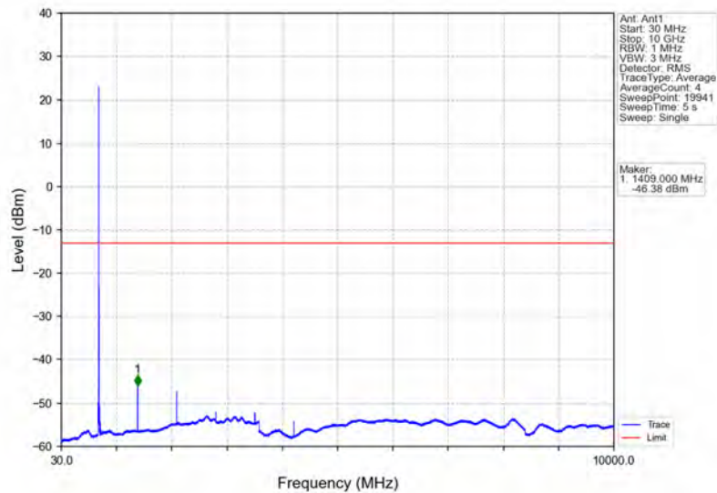
Band17_10MHz_16QAM_LCH_709MHz_RB_50_0_NTNV
