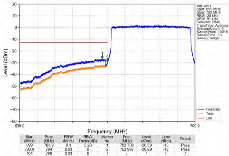
Band17_5MHz_16QAM_LCH_706.5MHz_RB_25_0_NTNV
