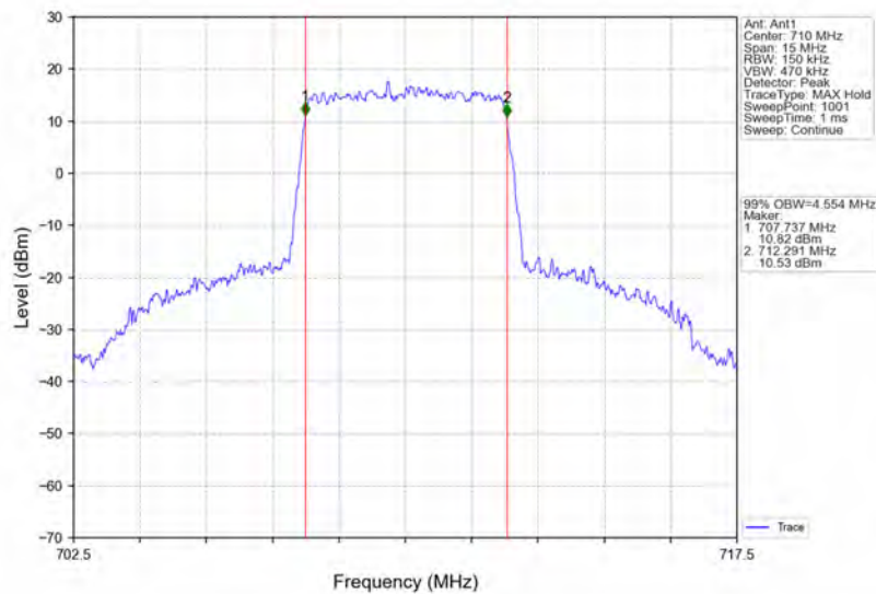
Band17_5MHz_64QAM_MCH_710MHz_RB_25_0_NTNV
