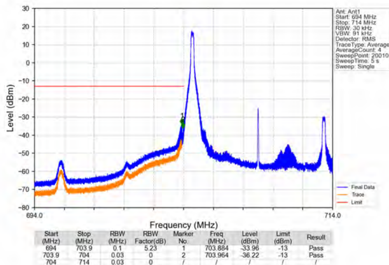
Band17_10MHz_16QAM_LCH_709MHz_RB_1_0_NTNV
