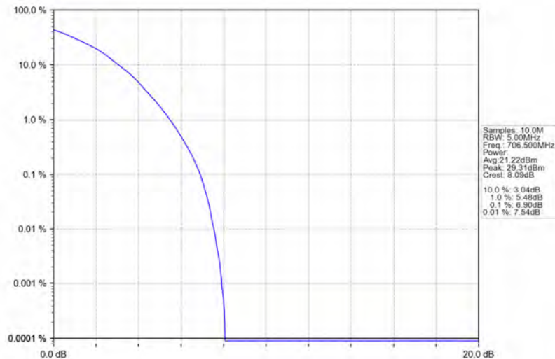
Band17_5MHz_64QAM_LCH_706.5MHz_RB_25_0_NTNV
