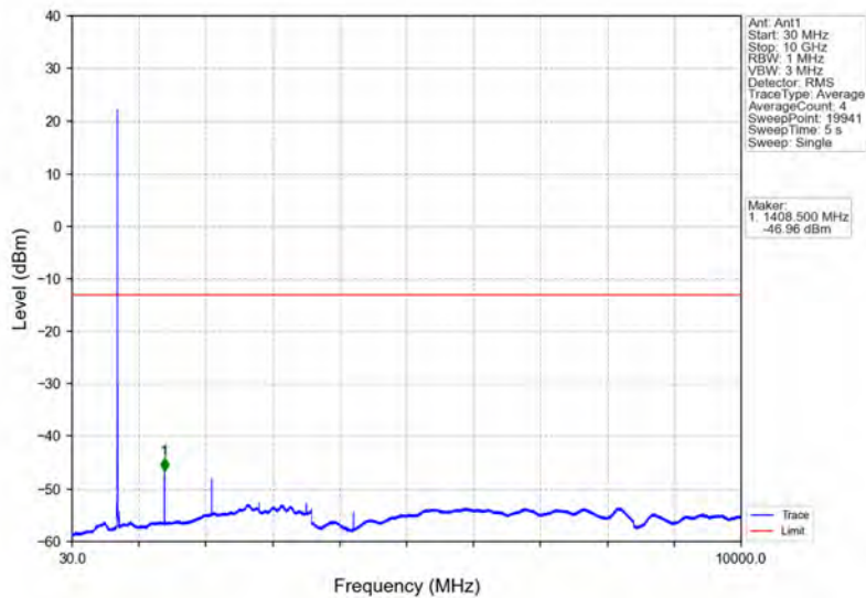
Band17_5MHz_16QAM_LCH_706.5MHz_RB_25_0_NTNV
