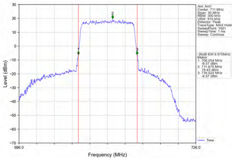
Band17_10MHz_QPSK_HCH_711MHz_RB_50_0_NTNV
