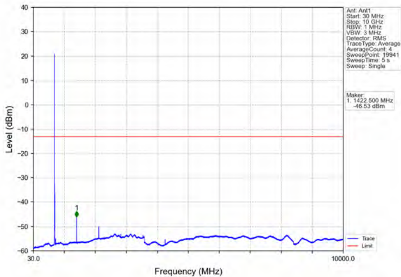
Band17_5MHz_64QAM_HCH_713.5MHz_RB_1_24_NTNV
