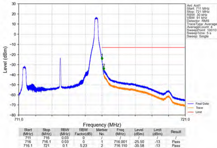
Band17_5MHz_16QAM_HCH_713.5MHz_RB_1_24_NTNV
