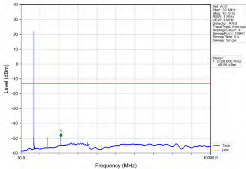
Band17_10MHz_64QAM_HCH_711MHz_RB_1_49_NTNV
