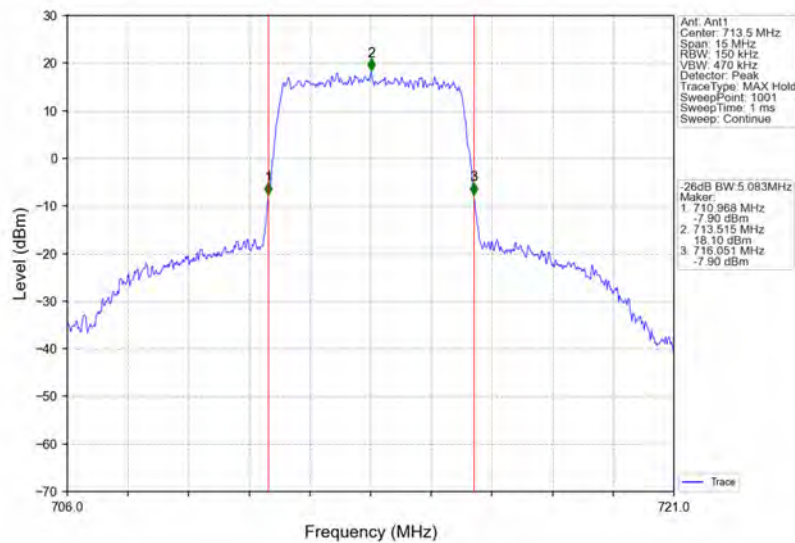
Band17_5MHz_16QAM_HCH_713.5MHz_RB_25_0_NTNV
