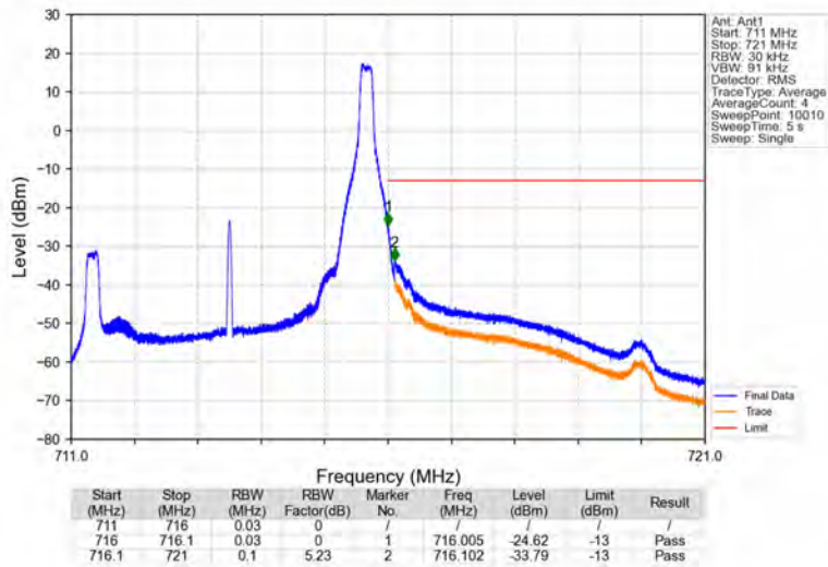
Band17_5MHz_QPSK_HCH_713.5MHz_RB_1_24_NTNV
