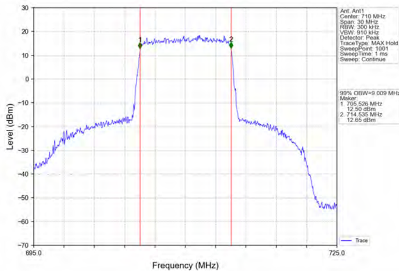
Band17_10MHz_16QAM_MCH_710MHz_RB_50_0_NTNV
