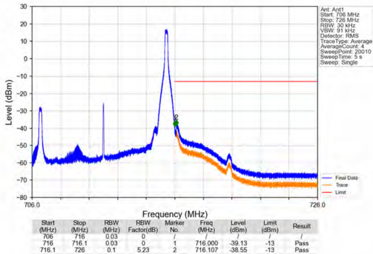
Band17_10MHz_16QAM_HCH_711MHz_RB_1_49_NTNV
