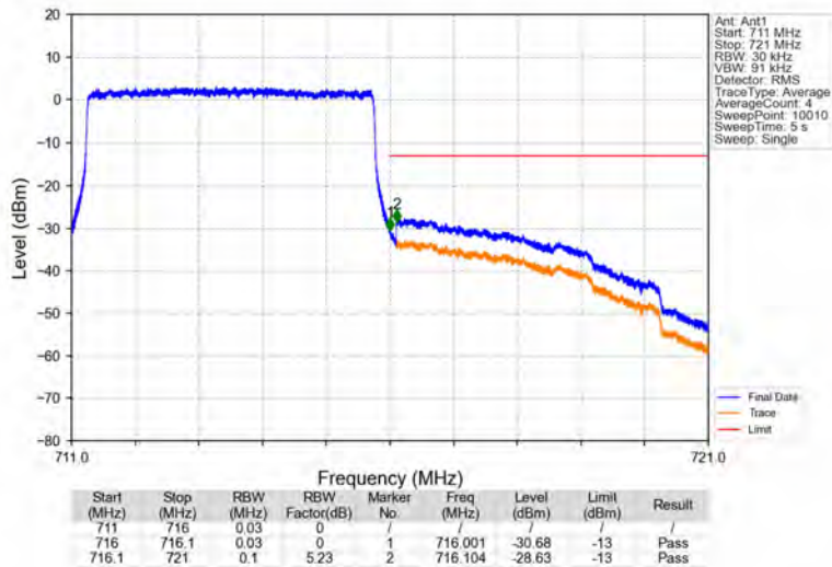
Band17_5MHz_QPSK_HCH_713.5MHz_RB_25_0_NTNV
