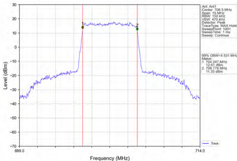
Band17_5MHz_16QAM_LCH_706.5MHz_RB_25_0_NTNV
