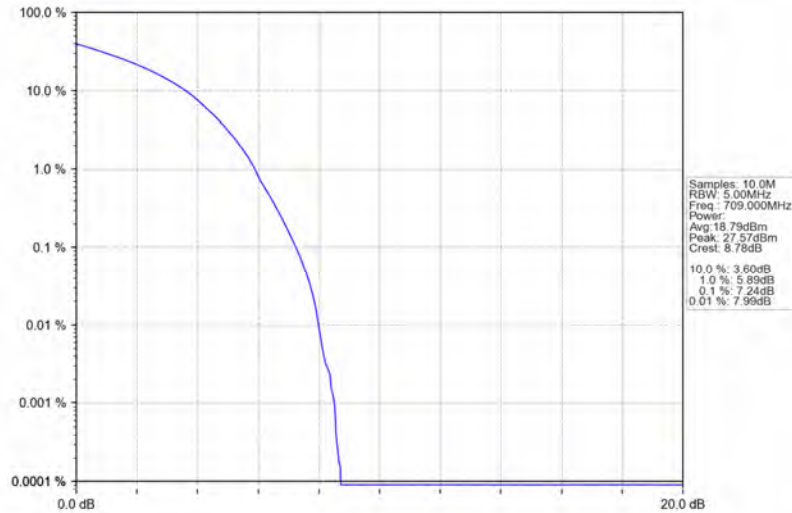
Band17_10MHz_64QAM_LCH_709MHz_RB_50_0_NTNV
