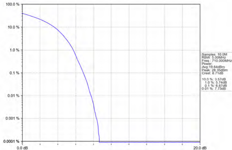
Band17_10MHz_16QAM_MCH_710MHz_RB_50_0_NTNV
