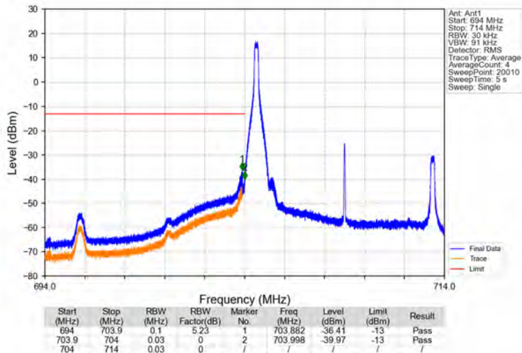
Band17_10MHz_64QAM_LCH_709MHz_RB_1_0_NTNV
