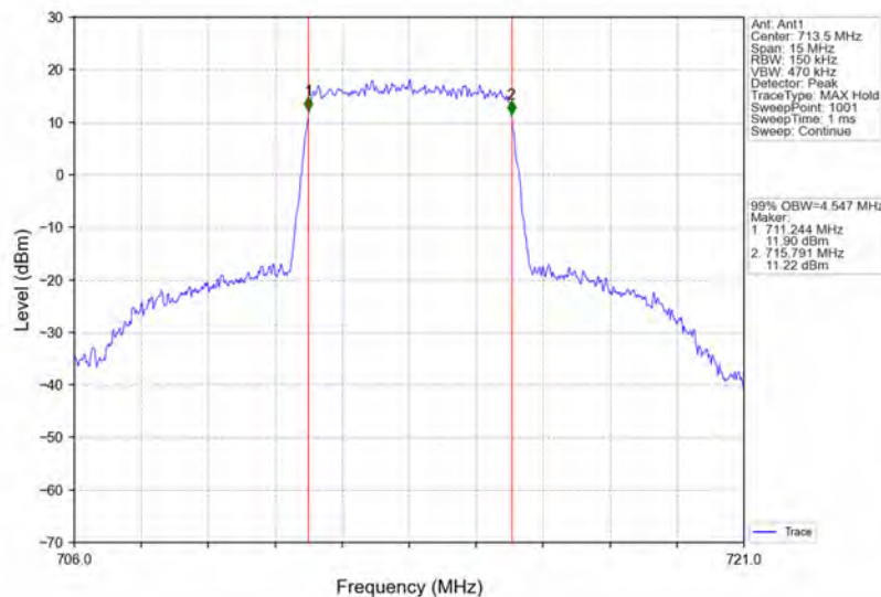
Band17_5MHz_16QAM_HCH_713.5MHz_RB_25_0_NTNV
