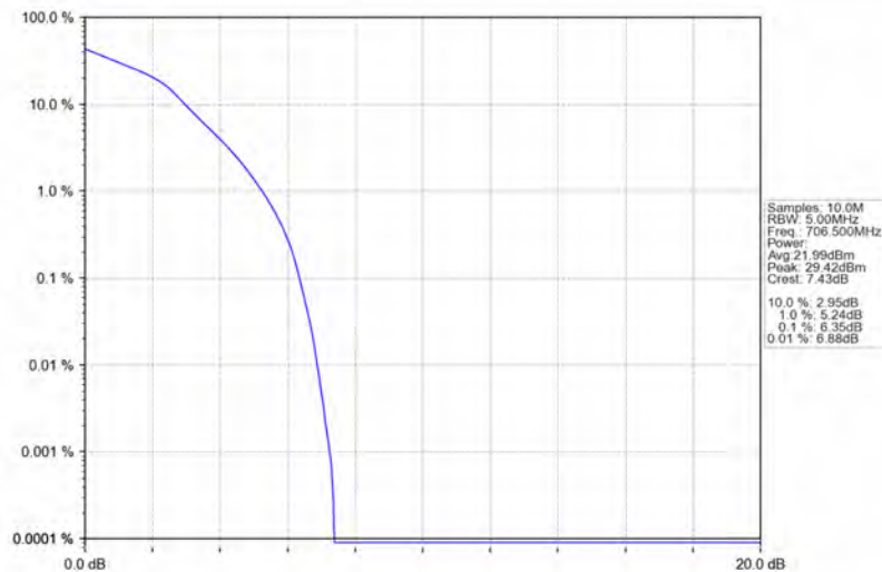
Band17_5MHz_16QAM_LCH_706.5MHz_RB_25_0_NTNV
