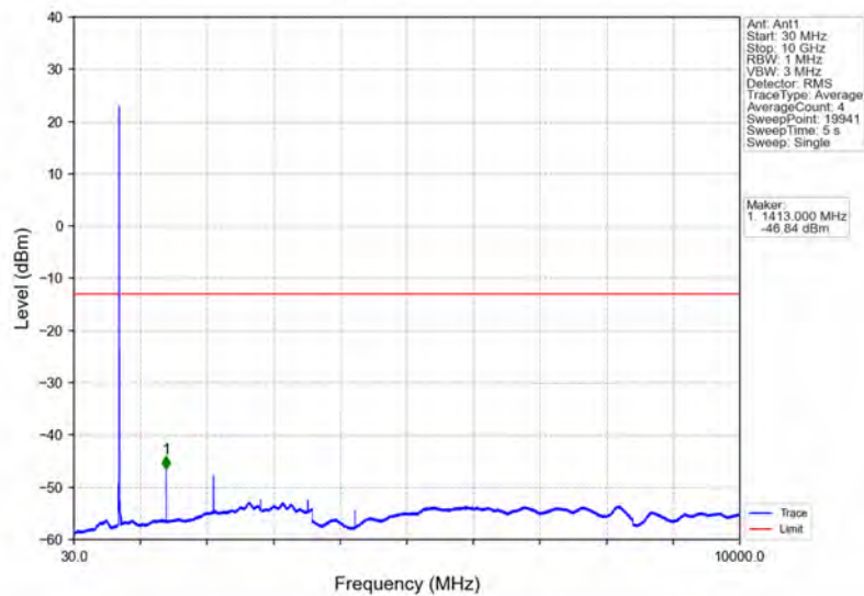
Band17_10MHz_16QAM_HCH_711MHz_RB_1_0_NTNV
