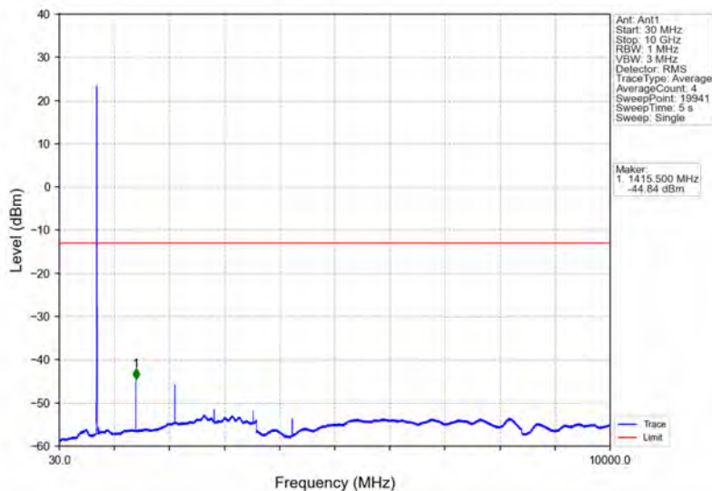
Band17_5MHz_QPSK_MCH_710MHz_RB_1_0_NTNV
