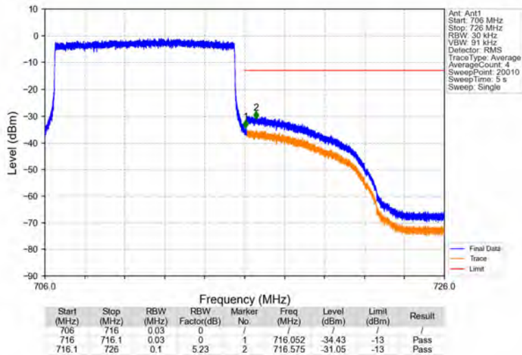
Band17_10MHz_64QAM_HCH_711MHz_RB_50_0_NTNV
