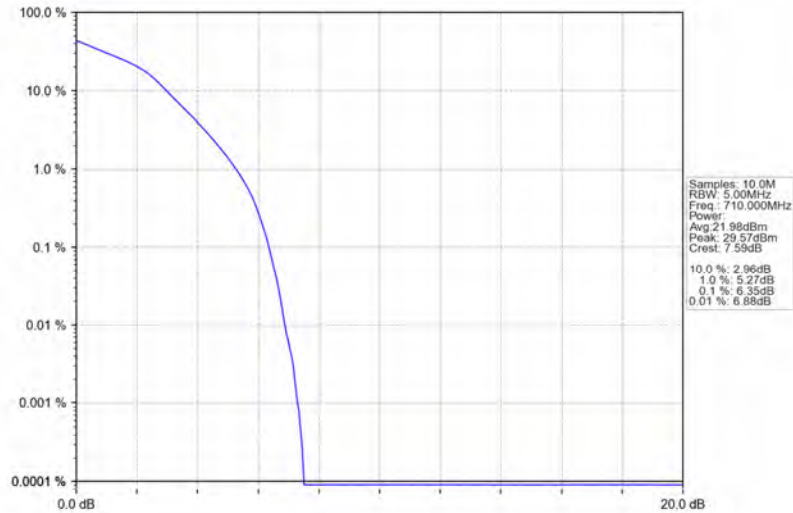
Band17_5MHz_16QAM_MCH_710MHz_RB_25_0_NTNV
