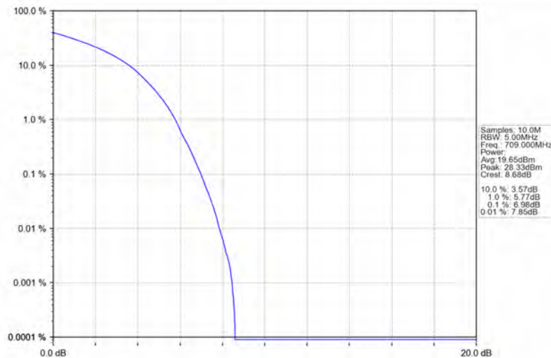
Band17_10MHz_16QAM_LCH_709MHz_RB_50_0_NTNV
