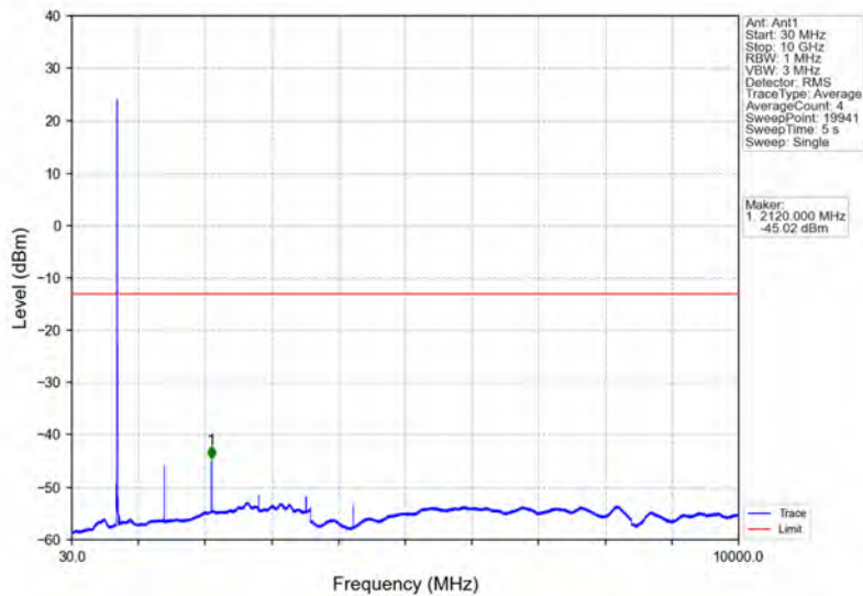
Band17_10MHz_QPSK_HCH_711MHz_RB_1_49_NTNV
