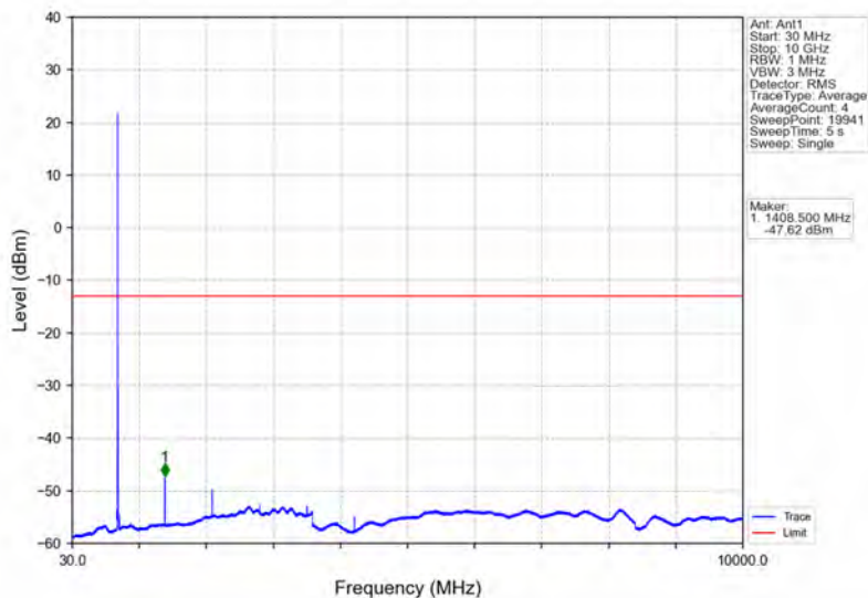
Band17_5MHz_64QAM_LCH_706.5MHz_RB_1_0_NTNV
