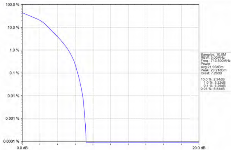
Band17_5MHz_16QAM_HCH_713.5MHz_RB_25_0_NTNV
