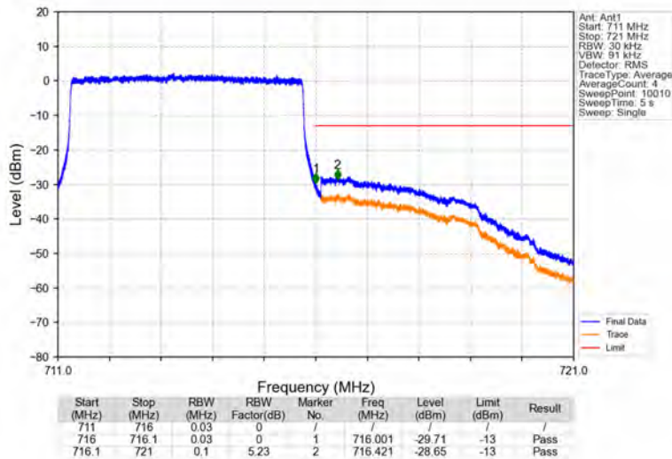
Band17_5MHz_16QAM_HCH_713.5MHz_RB_25_0_NTNV
