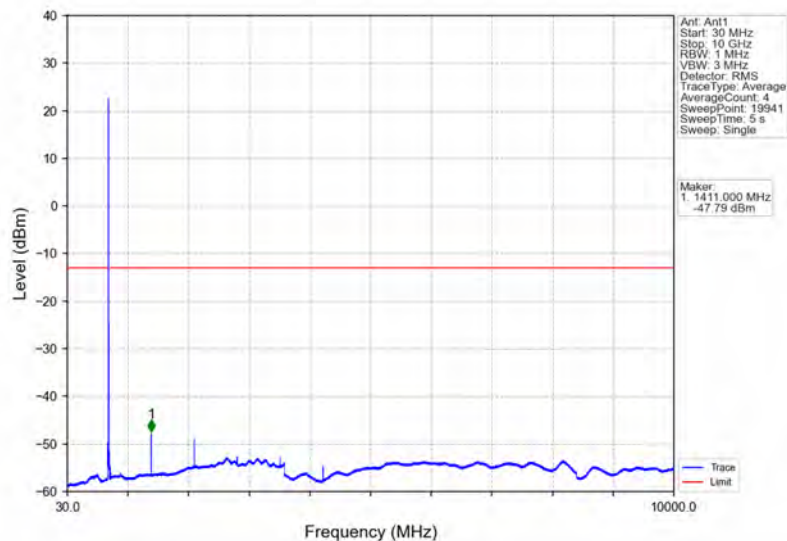
Band17_10MHz_64QAM_MCH_710MHz_RB_1_0_NTNV
