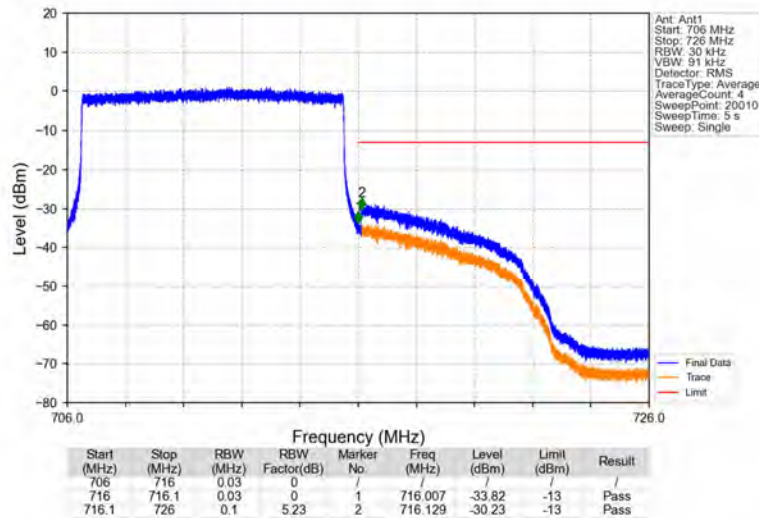
Band17_10MHz_QPSK_HCH_711MHz_RB_50_0_NTNV
