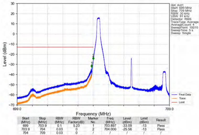
Band17_5MHz_16QAM_LCH_706.5MHz_RB_1_0_NTNV
