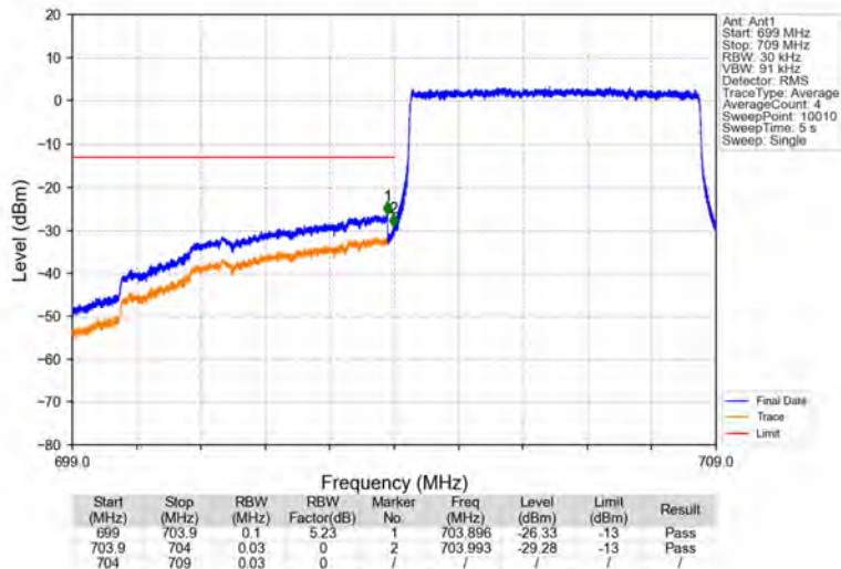
Band17_5MHz_QPSK_LCH_706.5MHz_RB_25_0_NTNV
