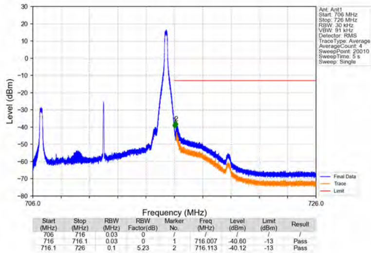
Band17_10MHz_64QAM_HCH_711MHz_RB_1_49_NTNV
