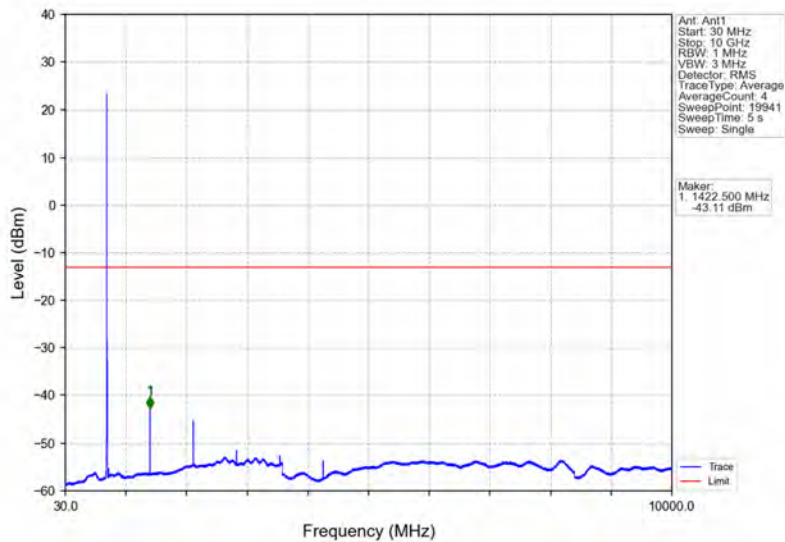
Band17_5MHz_QPSK_HCH_713.5MHz_RB_1_24_NTNV
