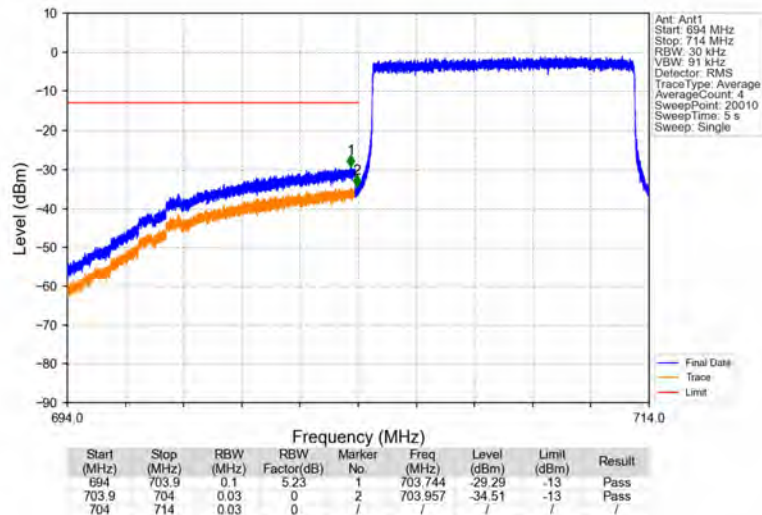
Band17_10MHz_64QAM_LCH_709MHz_RB_50_0_NTNV
