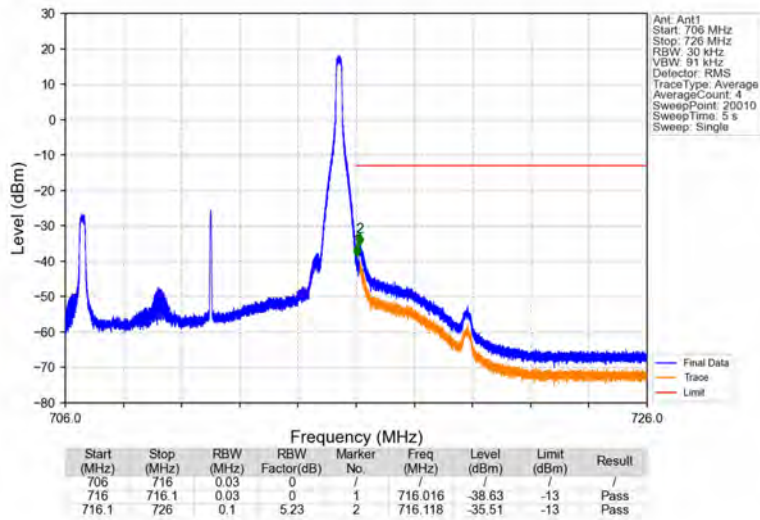
Band17_10MHz_QPSK_HCH_711MHz_RB_1_49_NTNV
