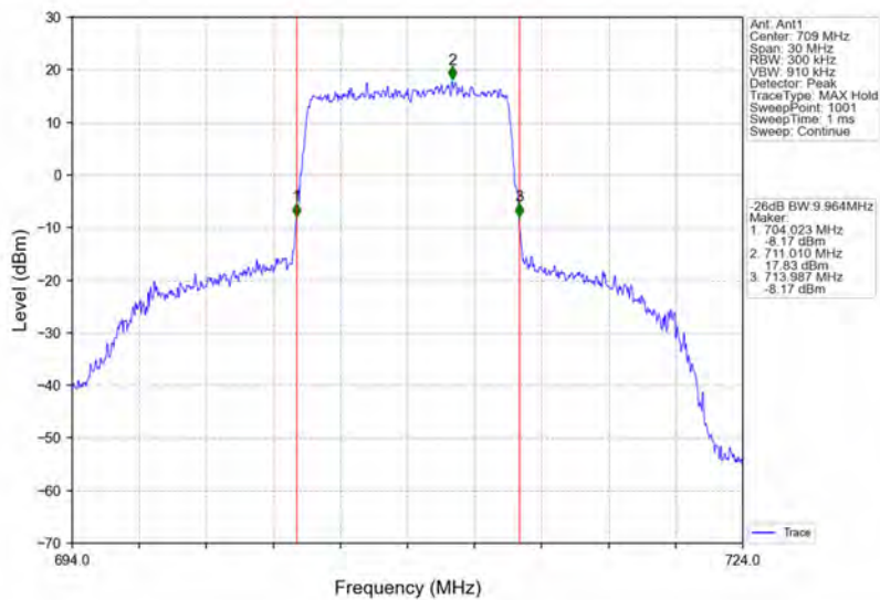
Band17_10MHz_64QAM_LCH_709MHz_RB_50_0_NTNV
