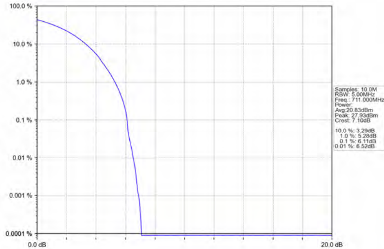
Band17_10MHz_QPSK_HCH_711MHz_RB_50_0_NTNV
