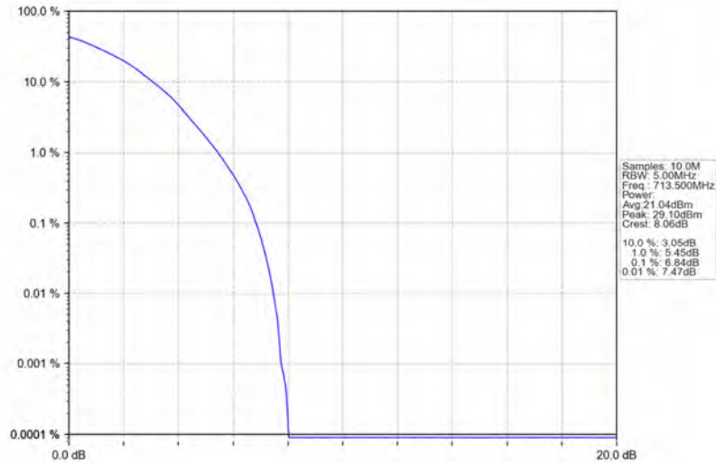
Band17_5MHz_64QAM_HCH_713.5MHz_RB_25_0_NTNV
