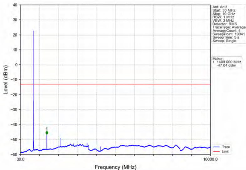
Band17_10MHz_64QAM_LCH_709MHz_RB_1_0_NTNV
