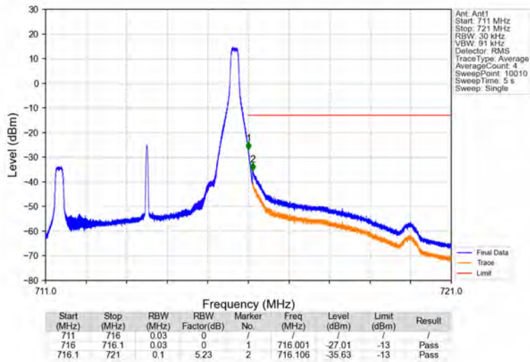
Band17_5MHz_64QAM_HCH_713.5MHz_RB_1_24_NTNV
