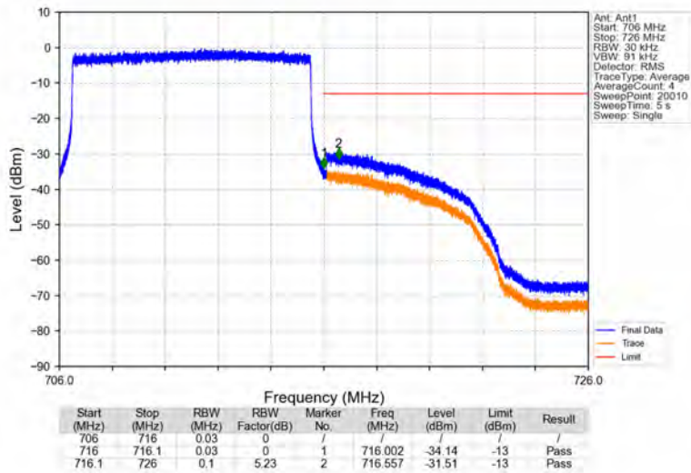
Band17_10MHz_16QAM_HCH_711MHz_RB_50_0_NTNV
