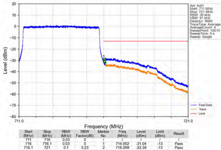
Band17_5MHz_64QAM_HCH_713.5MHz_RB_25_0_NTNV
