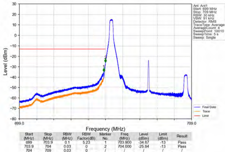
Band17_5MHz_64QAM_LCH_706.5MHz_RB_1_0_NTNV
