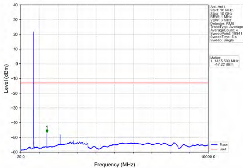
Band17_5MHz_64QAM_MCH_710MHz_RB_1_0_NTNV
