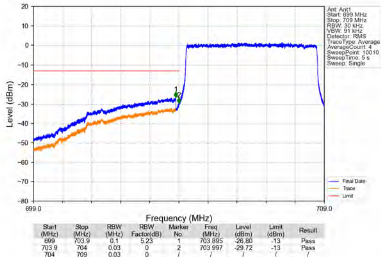
Band17_5MHz_64QAM_LCH_706.5MHz_RB_25_0_NTNV
