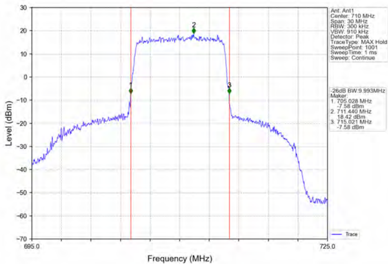
Band17_10MHz_16QAM_MCH_710MHz_RB_50_0_NTNV
