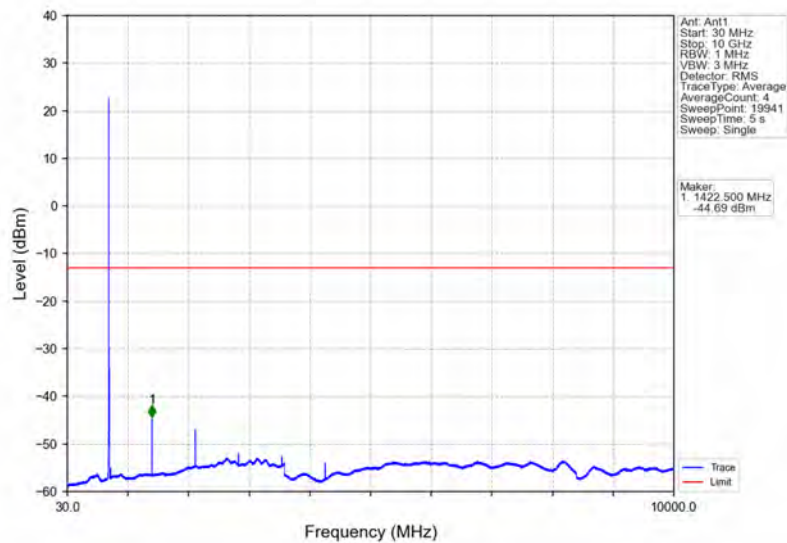
Band17_5MHz_16QAM_HCH_713.5MHz_RB_1_0_NTNV
