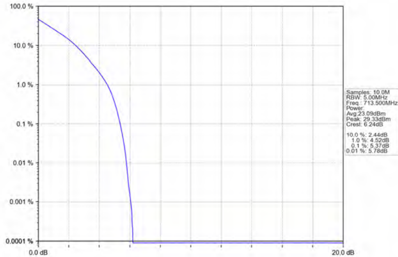
Band17_5MHz_QPSK_HCH_713.5MHz_RB_25_0_NTNV
