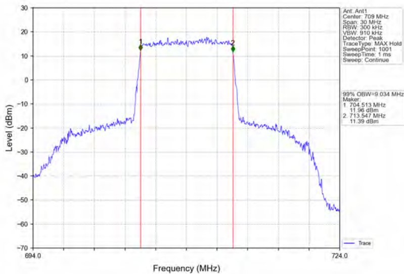
Band17_10MHz_64QAM_LCH_709MHz_RB_50_0_NTNV
