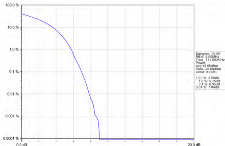
Band17_10MHz_16QAM_HCH_711MHz_RB_50_0_NTNV
