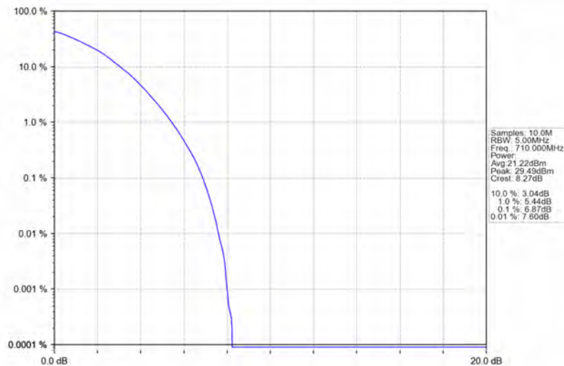
Band17_5MHz_64QAM_MCH_710MHz_RB_25_0_NTNV
