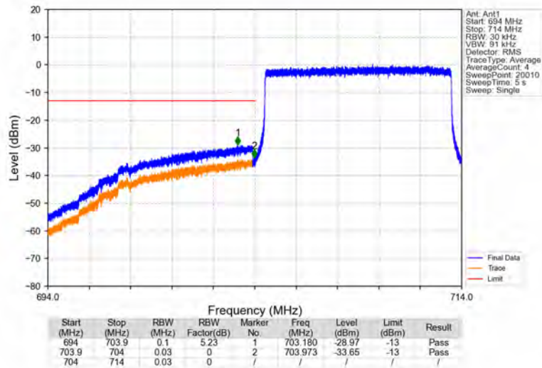
Band17_10MHz_16QAM_LCH_709MHz_RB_50_0_NTNV
