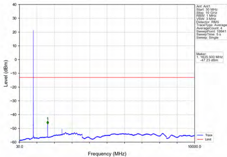
Band26a_3MHz_64QAM_MCH_819MHz_RB_1_0_NTNV
