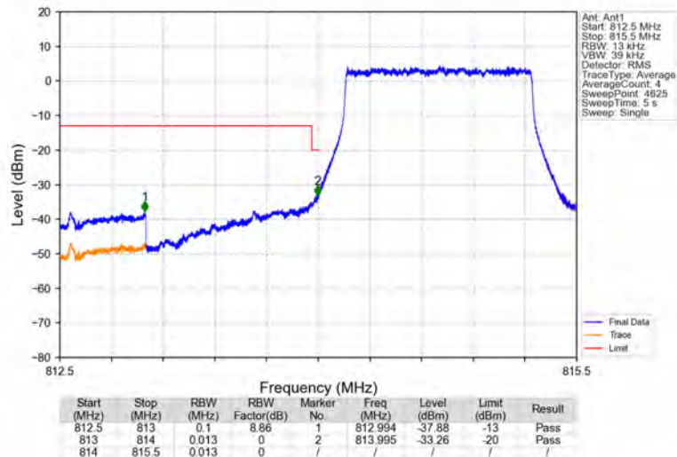
Band26a_1.4MHz_16QAM_LCH_814.7MHz_RB_6_0_NTNV
