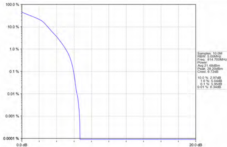
Band26a_1.4MHz_16QAM_LCH_814.7MHz_RB_6_0_NTNV
