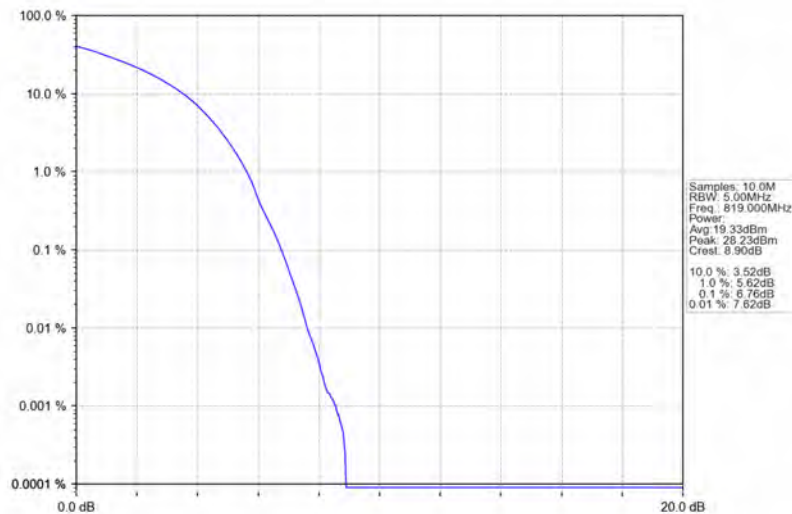
Band26a_10MHz_16QAM_LCH_819MHz_RB_50_0_NTNV
