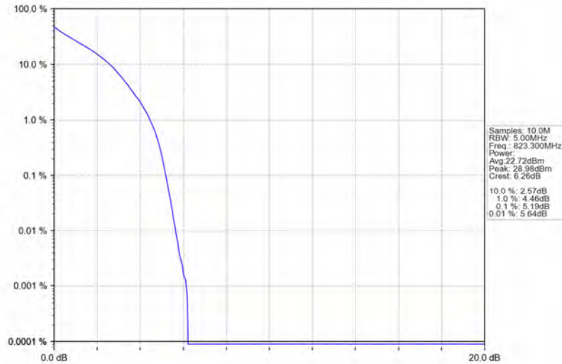
Band26a_1.4MHz_QPSK_HCH_823.3MHz_RB_6_0_NTNV
