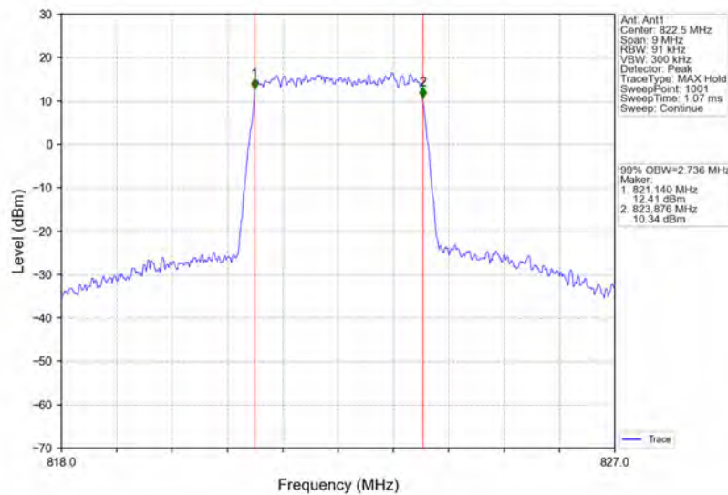
Band26a_3MHz_64QAM_HCH_822.5MHz_RB_15_0_NTNV
