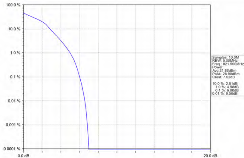
Band26a_5MHz_16QAM_HCH_821.5MHz_RB_25_0_NTNV
