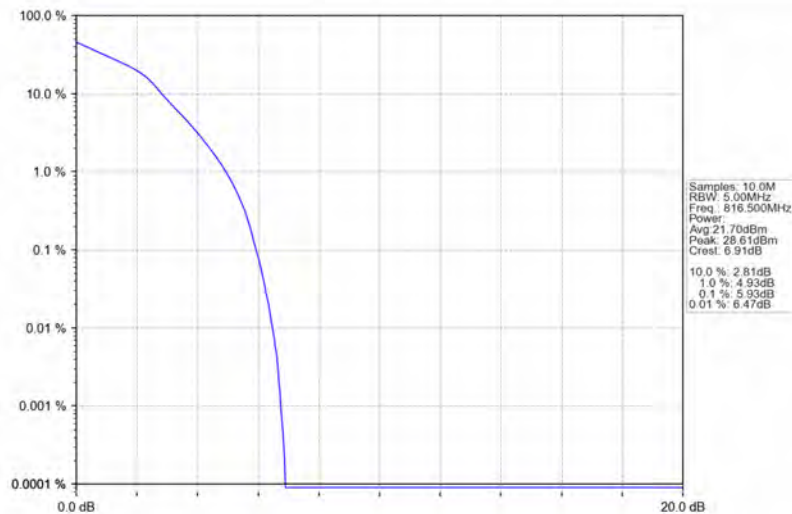
Band26a_5MHz_16QAM_LCH_816.5MHz_RB_25_0_NTNV
