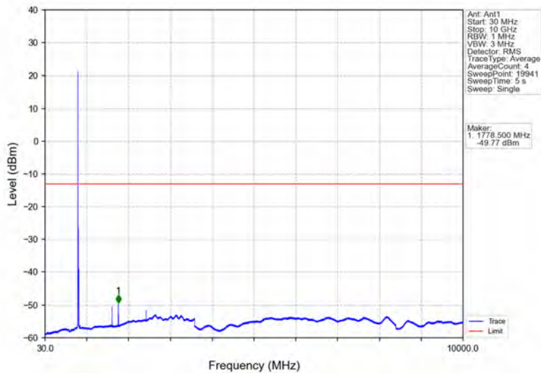
Band26a_10MHz_64QAM_HCH_819MHz_RB_1_49_NTNV
