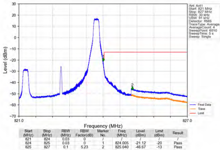
Band26a_3MHz_QPSK_HCH_822.5MHz_RB_1_14_NTNV
