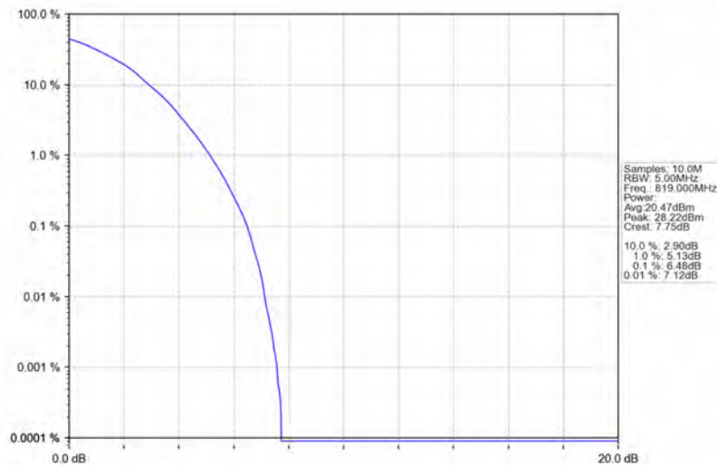
Band26a_5MHz_64QAM_MCH_819MHz_RB_25_0_NTNV
