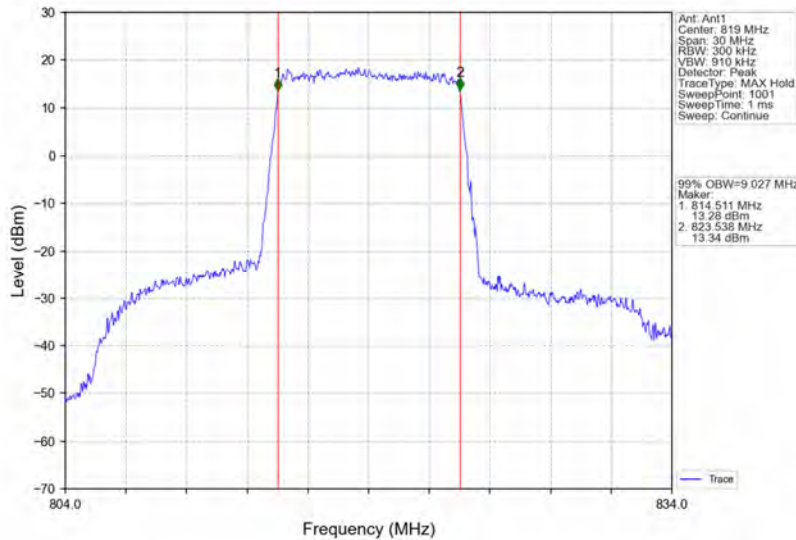
Band26a_10MHz_QPSK_HCH_819MHz_RB_50_0_NTNV
