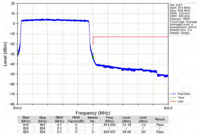
Band26a_10MHz_QPSK_HCH_819MHz_RB_50_0_NTNV
