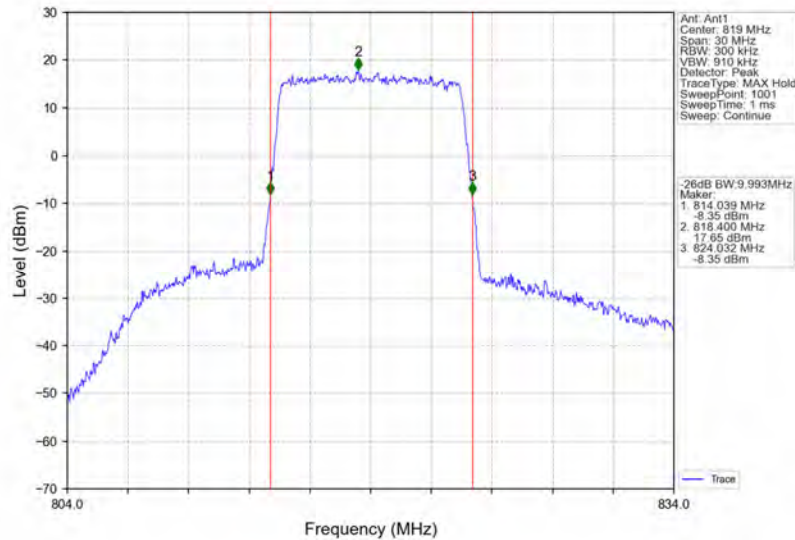
Band26a_10MHz_16QAM_MCH_819MHz_RB_50_0_NTNV
