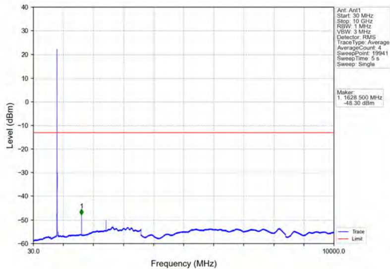
Band26a_3MHz_16QAM_LCH_815.5MHz_RB_15_0_NTNV
