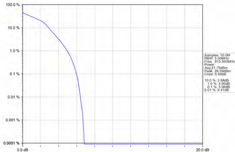
Band26a_3MHz_16QAM_LCH_815.5MHz_RB_15_0_NTNV
