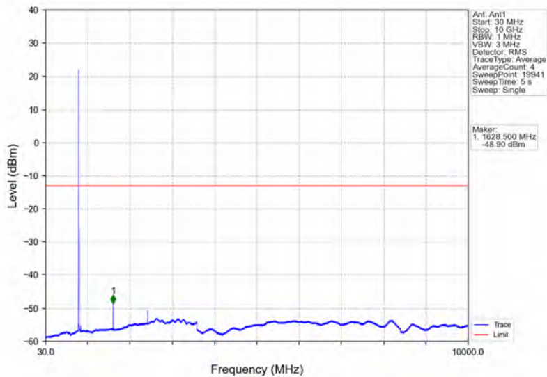
Band26a_5MHz_16QAM_LCH_816.5MHz_RB_25_0_NTNV
