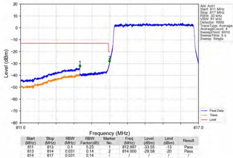
Band26a_3MHz_16QAM_LCH_815.5MHz_RB_15_0_NTNV
