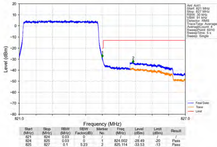
Band26a_3MHz_QPSK_HCH_822.5MHz_RB_15_0_NTNV
