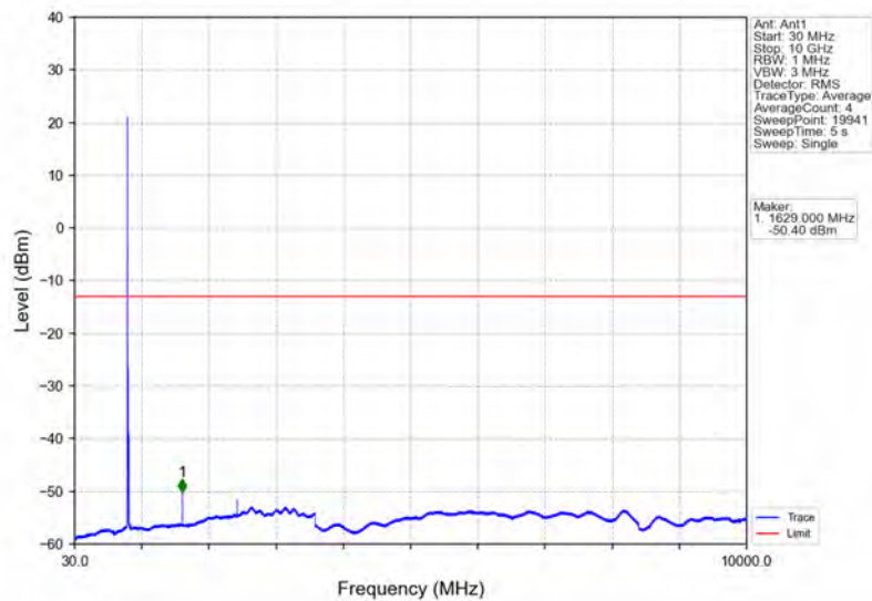
Band26a_10MHz_64QAM_LCH_819MHz_RB_1_0_NTNV
