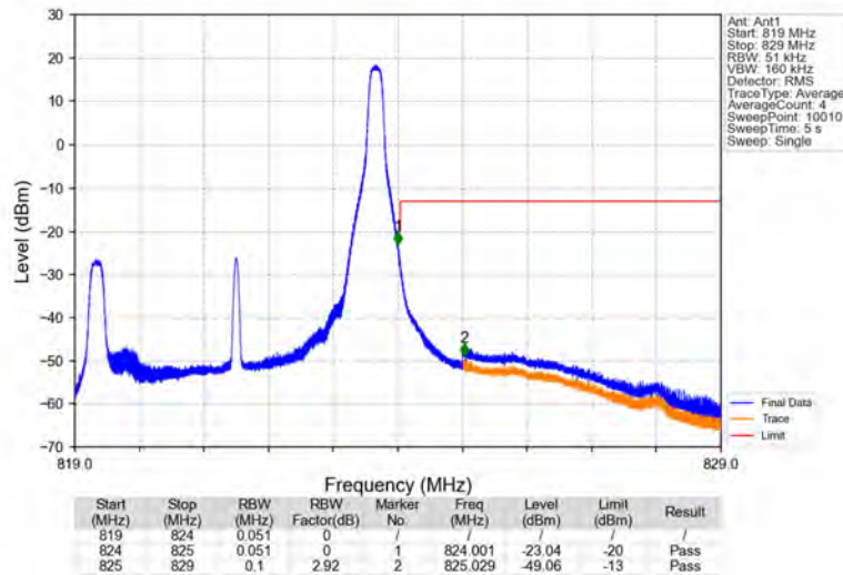
Band26a_5MHz_16QAM_HCH_821.5MHz_RB_1_24_NTNV
