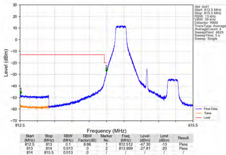
Band26a_1.4MHz_16QAM_LCH_814.7MHz_RB_1_0_NTNV
