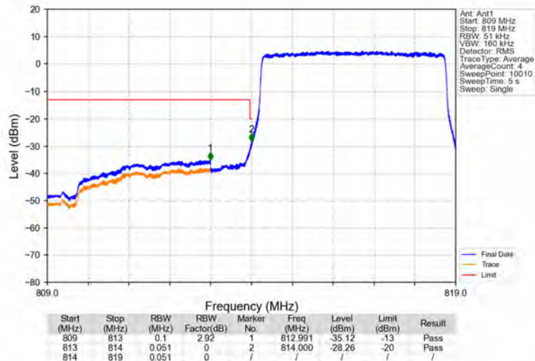
Band26a_5MHz_QPSK_LCH_816.5MHz_RB_25_0_NTNV
