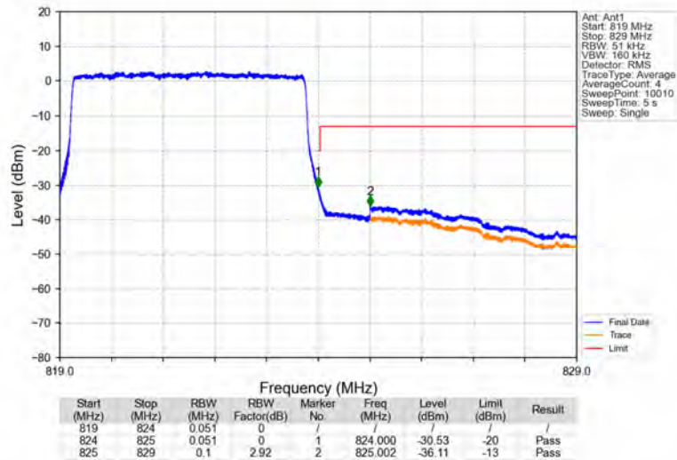
Band26a_5MHz_64QAM_HCH_821.5MHz_RB_25_0_NTNV
