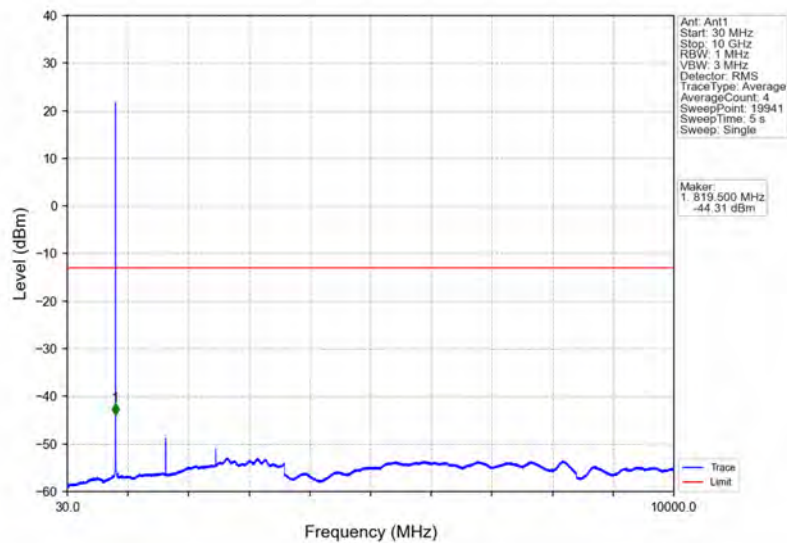
Band26a_1.4MHz_16QAM_HCH_823.3MHz_RB_1_0_NTNV
