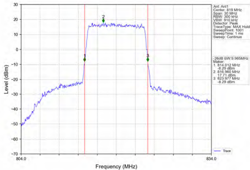
Band26a_10MHz_64QAM_LCH_819MHz_RB_50_0_NTNV
