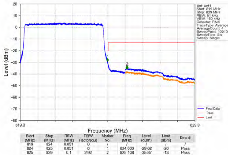
Band26a_5MHz_16QAM_HCH_821.5MHz_RB_25_0_NTNV
