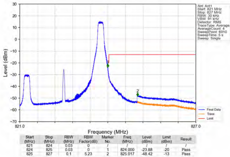
Band26a_3MHz_64QAM_HCH_822.5MHz_RB_1_14_NTNV
