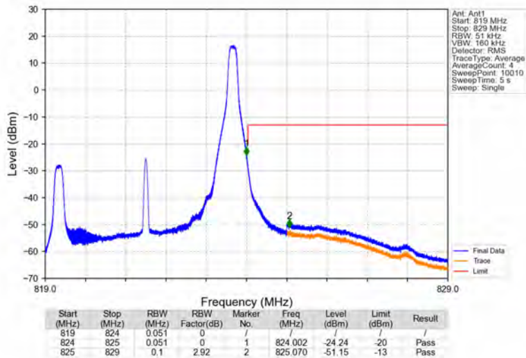
Band26a_5MHz_64QAM_HCH_821.5MHz_RB_1_24_NTNV
