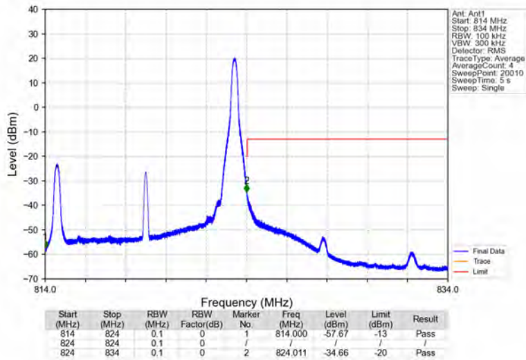
Band26a_10MHz_64QAM_HCH_819MHz_RB_1_49_NTNV
