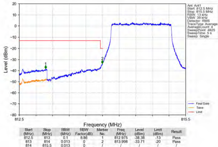
Band26a_1.4MHz_64QAM_LCH_814.7MHz_RB_6_0_NTNV
