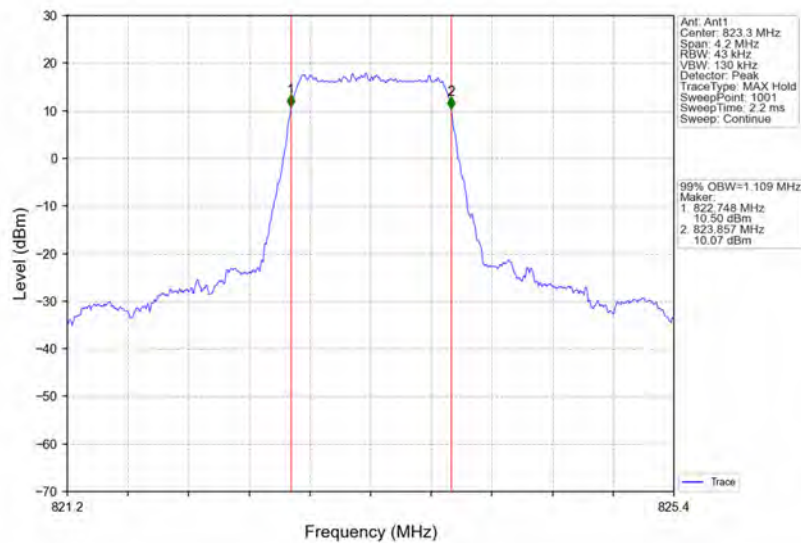
Band26a_1.4MHz_16QAM_HCH_823.3MHz_RB_6_0_NTNV
