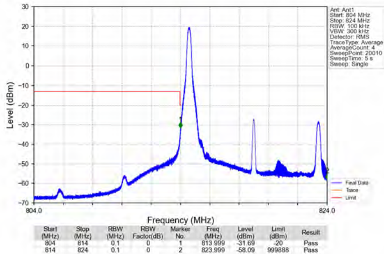
Band26a_10MHz_64QAM_LCH_819MHz_RB_1_0_NTNV
