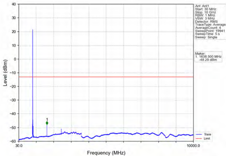
Band26a_5MHz_64QAM_HCH_821.5MHz_RB_1_24_NTNV
