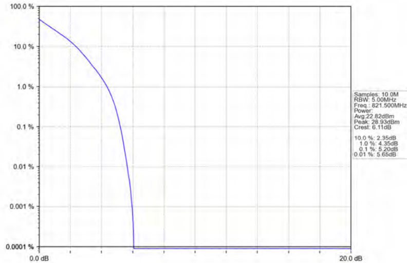
Band26a_5MHz_QPSK_HCH_821.5MHz_RB_25_0_NTNV
