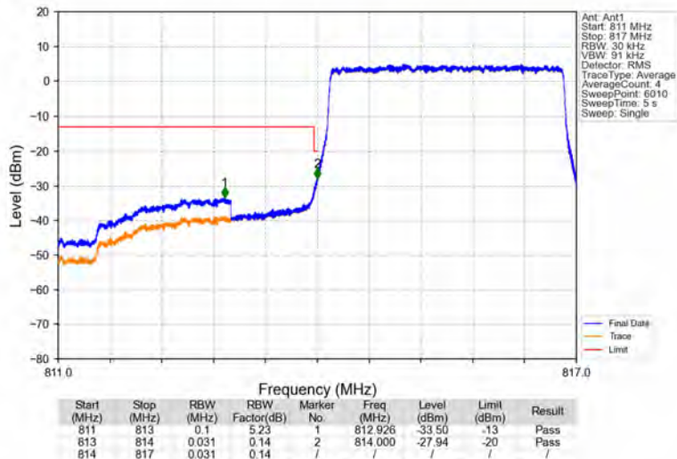
Band26a_3MHz_QPSK_LCH_815.5MHz_RB_15_0_NTNV
