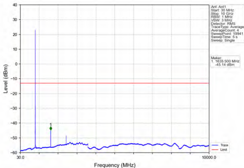
Band26a_3MHz_QPSK_MCH_819MHz_RB_1_0_NTNV
