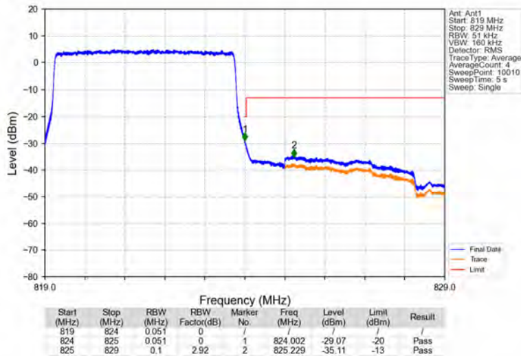
Band26a_5MHz_QPSK_HCH_821.5MHz_RB_25_0_NTNV
