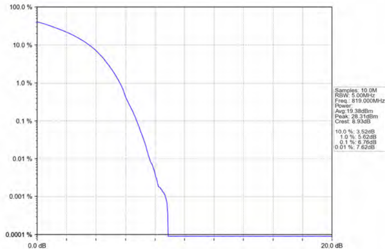
Band26a_10MHz_16QAM_MCH_819MHz_RB_50_0_NTNV
