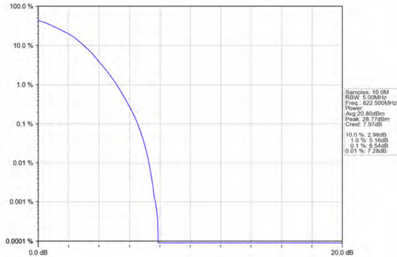
Band26a_3MHz_64QAM_HCH_822.5MHz_RB_15_0_NTNV
