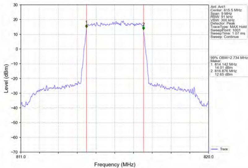
Band26a_3MHz_QPSK_LCH_815.5MHz_RB_15_0_NTNV
