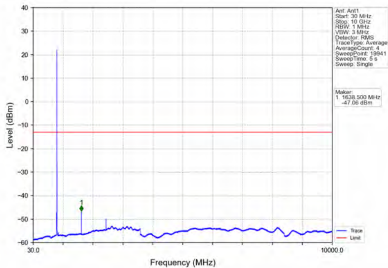
Band26a_5MHz_16QAM_HCH_821.5MHz_RB_1_0_NTNV
