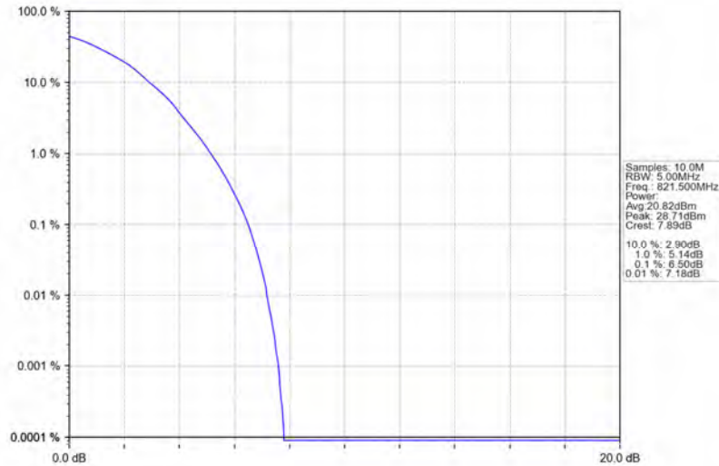
Band26a_5MHz_64QAM_HCH_821.5MHz_RB_25_0_NTNV
