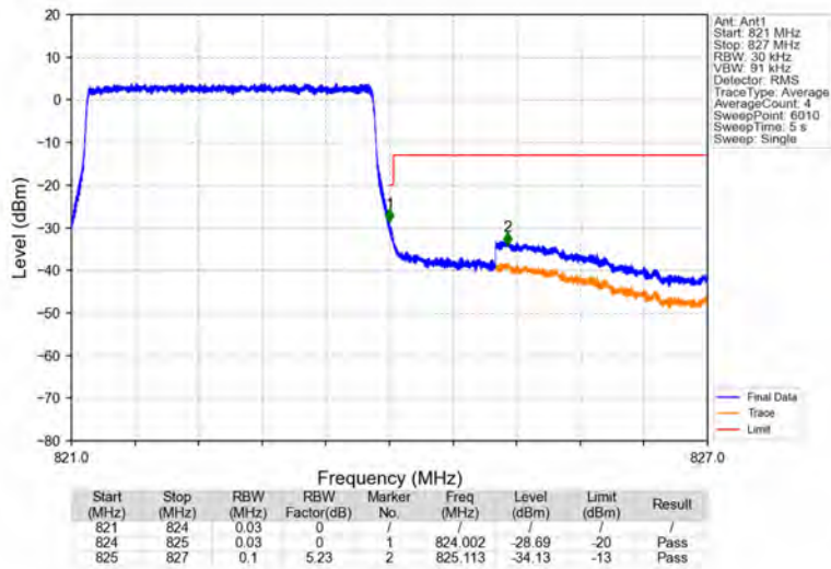
Band26a_3MHz_16QAM_HCH_822.5MHz_RB_15_0_NTNV
