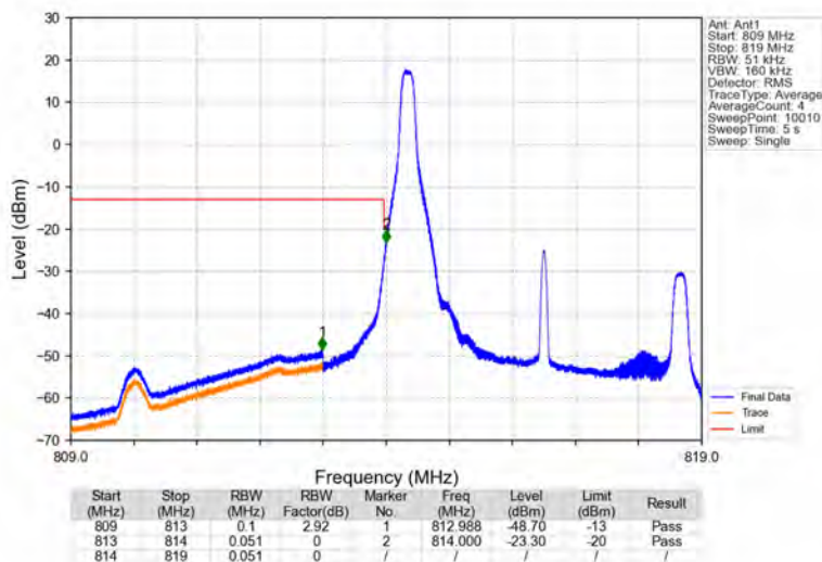
Band26a_5MHz_16QAM_LCH_816.5MHz_RB_1_0_NTNV
