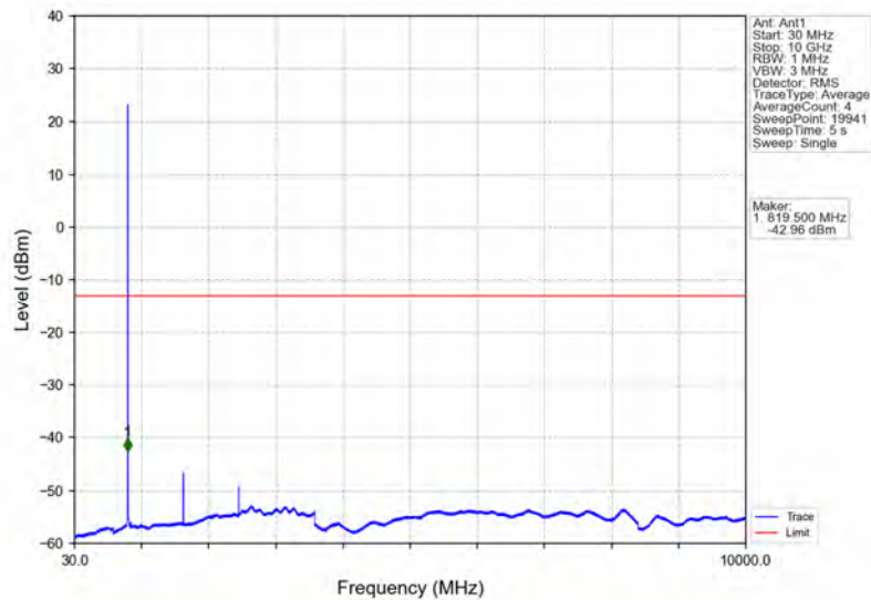
Band26a_1.4MHz_QPSK_HCH_823.3MHz_RB_1_5_NTNV
