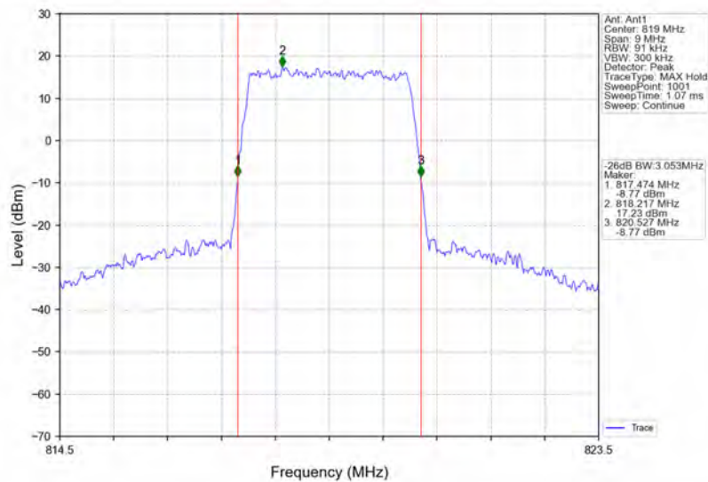
Band26a_3MHz_16QAM_MCH_819MHz_RB_15_0_NTNV
