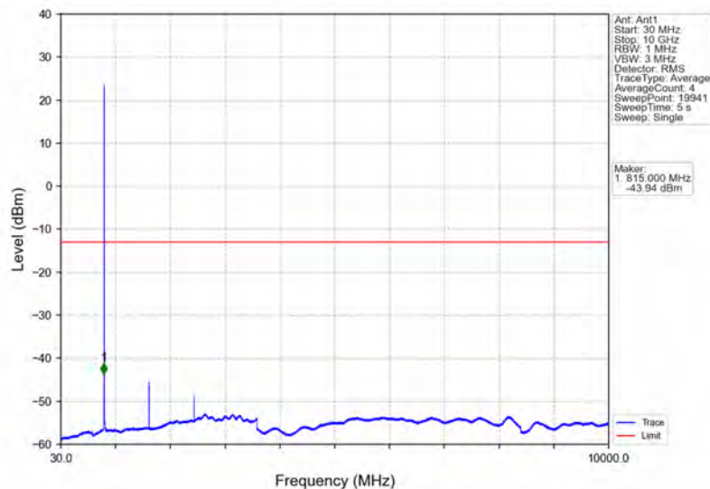
Band26a_1.4MHz_QPSK_MCH_819MHz_RB_1_0_NTNV
