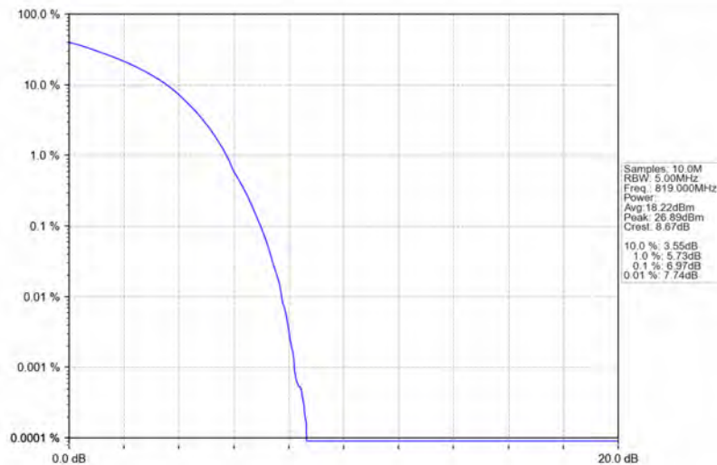
Band26a_10MHz_64QAM_MCH_819MHz_RB_50_0_NTNV
