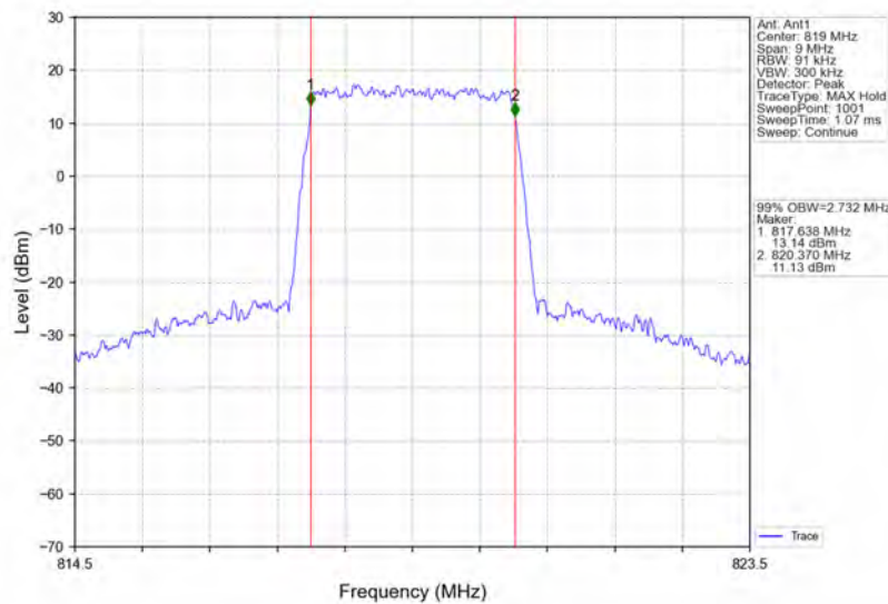
Band26a_3MHz_16QAM_MCH_819MHz_RB_15_0_NTNV
