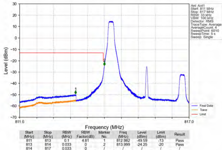
Band26a_3MHz_64QAM_LCH_815.5MHz_RB_1_0_NTNV
