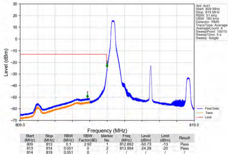
Band26a_5MHz_64QAM_LCH_816.5MHz_RB_1_0_NTNV
