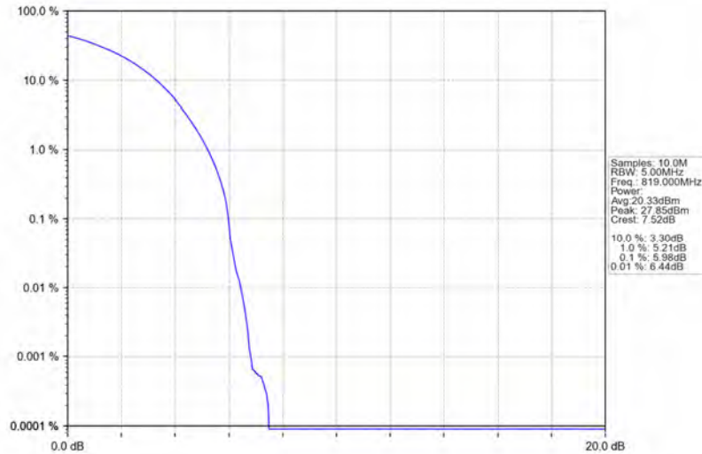
Band26a_10MHz_QPSK_HCH_819MHz_RB_50_0_NTNV
