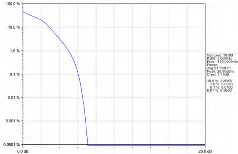
Band26a_3MHz_16QAM_MCH_819MHz_RB_15_0_NTNV
