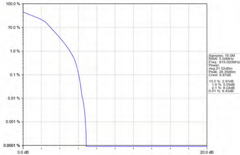
Band26a_1.4MHz_16QAM_MCH_819MHz_RB_6_0_NTNV
