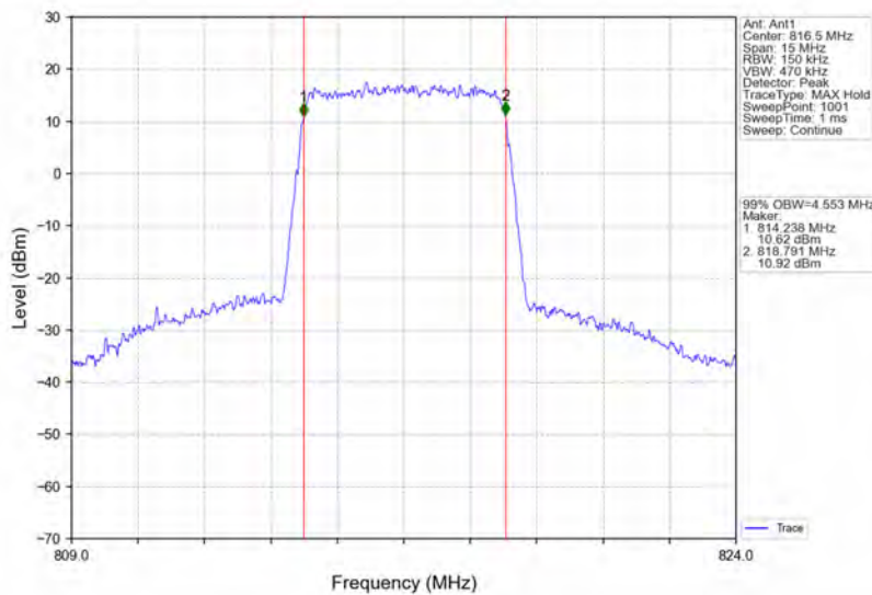
Band26a_5MHz_16QAM_LCH_816.5MHz_RB_25_0_NTNV
