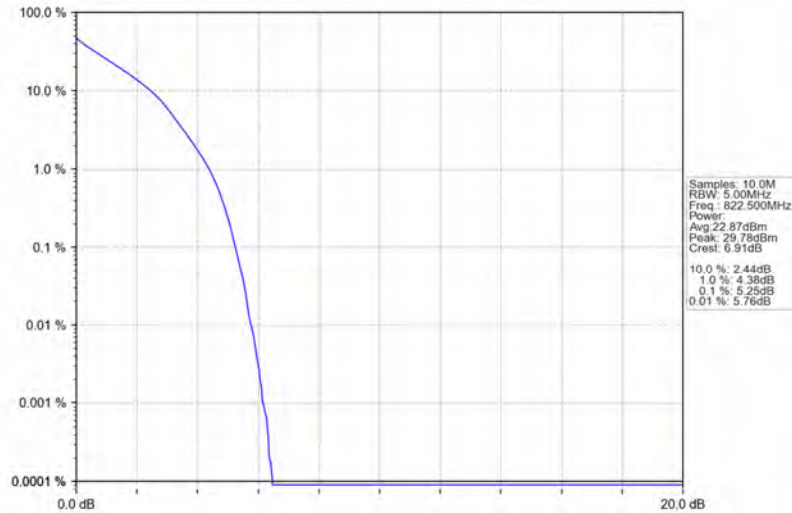
Band26a_3MHz_QPSK_HCH_822.5MHz_RB_15_0_NTNV
