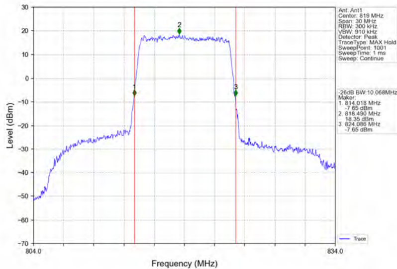
Band26a_10MHz_QPSK_HCH_819MHz_RB_50_0_NTNV
