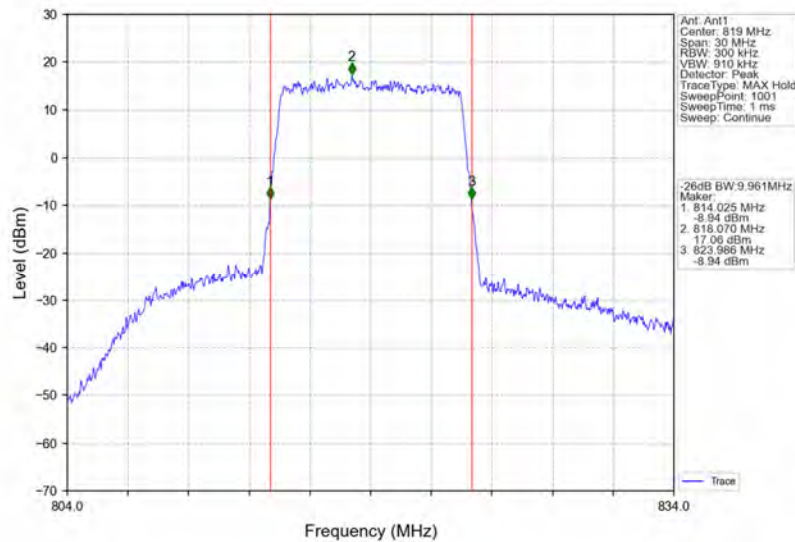
Band26a_10MHz_64QAM_HCH_819MHz_RB_50_0_NTNV
