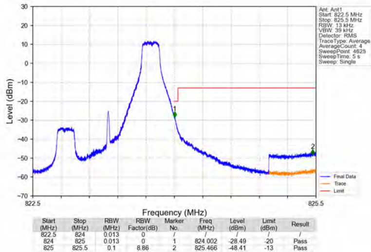
Band26a_1.4MHz_64QAM_HCH_823.3MHz_RB_1_5_NTNV
