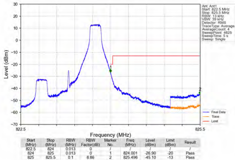
Band26a_1.4MHz_QPSK_HCH_823.3MHz_RB_1_5_NTNV
