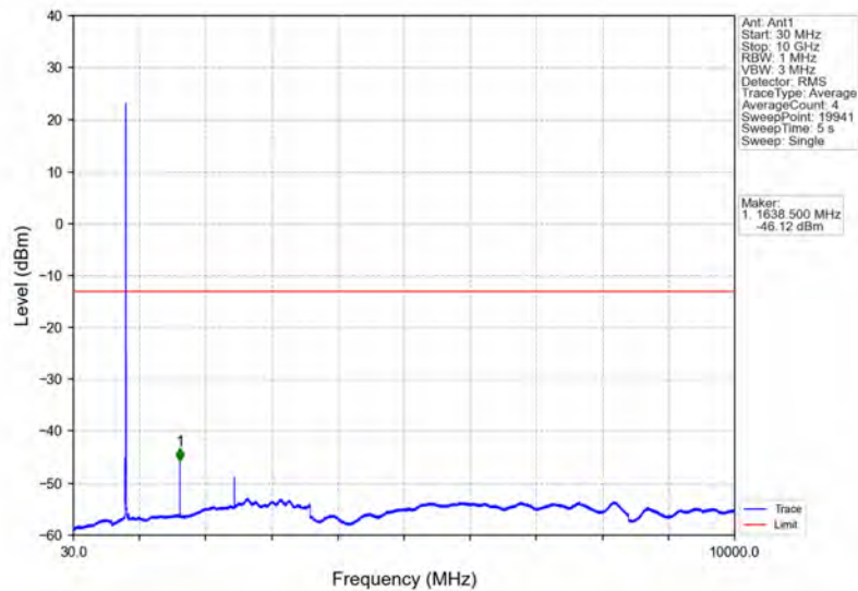
Band26a_5MHz_QPSK_HCH_821.5MHz_RB_1_24_NTNV
