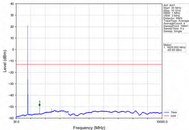
Band26a_10MHz_64QAM_MCH_819MHz_RB_1_0_NTNV
