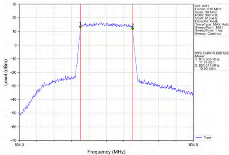
Band26a_10MHz_64QAM_HCH_819MHz_RB_50_0_NTNV
