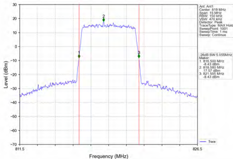
Band26a_5MHz_64QAM_MCH_819MHz_RB_25_0_NTNV
