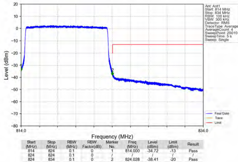
Band26a_10MHz_64QAM_HCH_819MHz_RB_50_0_NTNV
