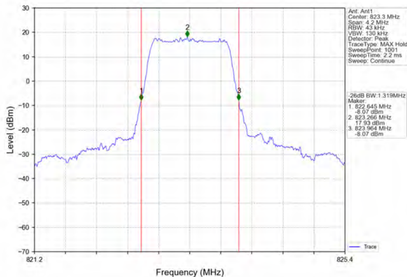
Band26a_1.4MHz_16QAM_HCH_823.3MHz_RB_6_0_NTNV
