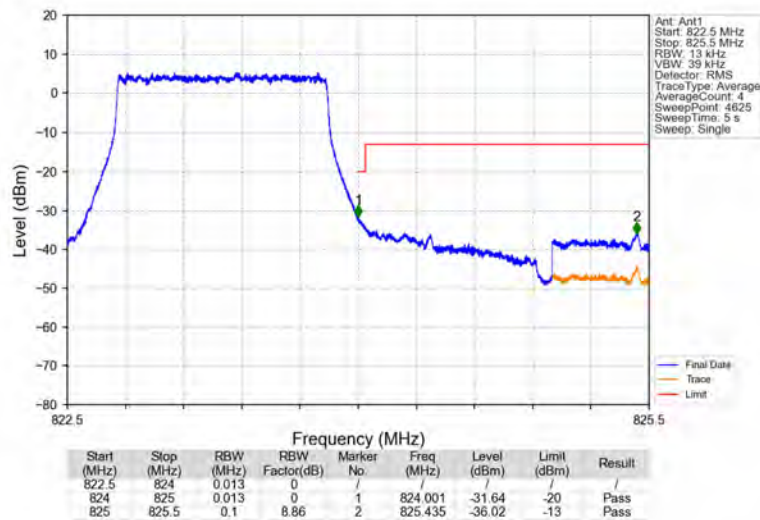
Band26a_1.4MHz_QPSK_HCH_823.3MHz_RB_6_0_NTNV
