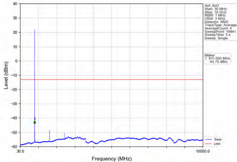
Band26a_1.4MHz_16QAM_LCH_814.7MHz_RB_6_0_NTNV
