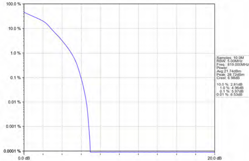
Band26a_5MHz_16QAM_MCH_819MHz_RB_25_0_NTNV
