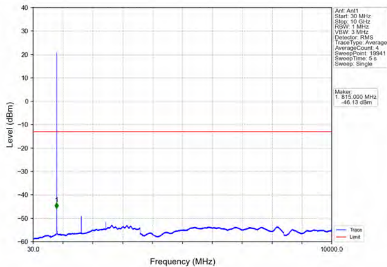
Band26a_1.4MHz_64QAM_MCH_819MHz_RB_1_0_NTNV
