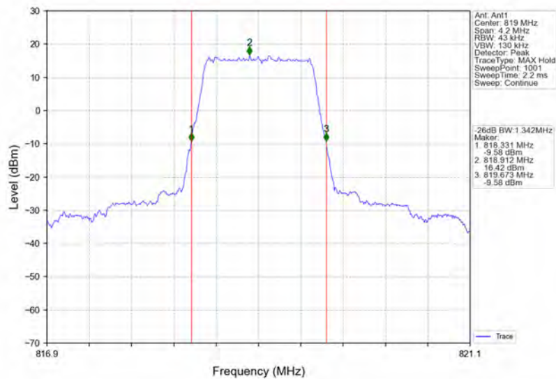
Band26a_1.4MHz_64QAM_MCH_819MHz_RB_6_0_NTNV
