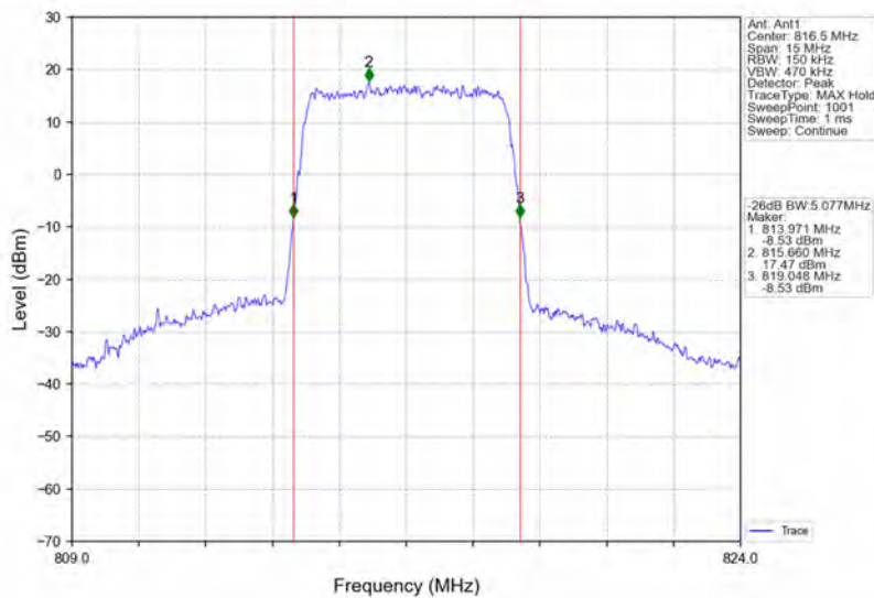
Band26a_5MHz_16QAM_LCH_816.5MHz_RB_25_0_NTNV
