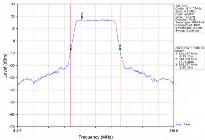
Band26a_1.4MHz_16QAM_LCH_814.7MHz_RB_6_0_NTNV
