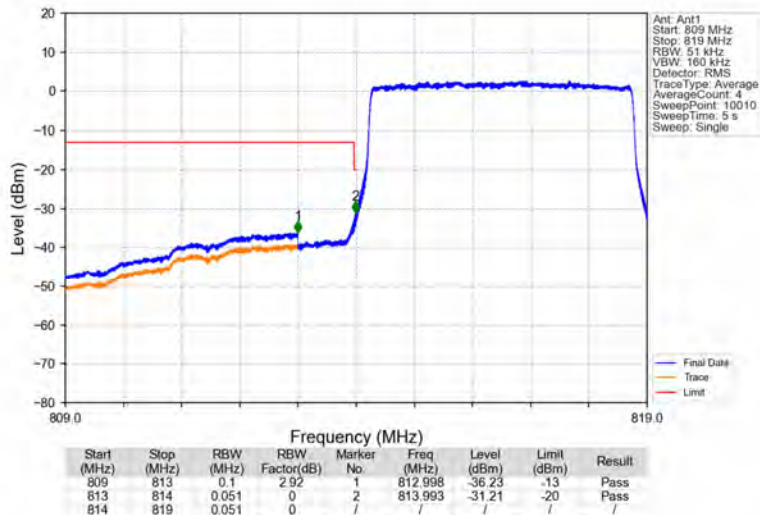
Band26a_5MHz_64QAM_LCH_816.5MHz_RB_25_0_NTNV
