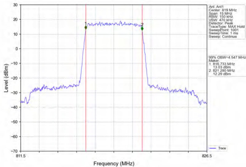
Band26a_5MHz_QPSK_MCH_819MHz_RB_25_0_NTNV
