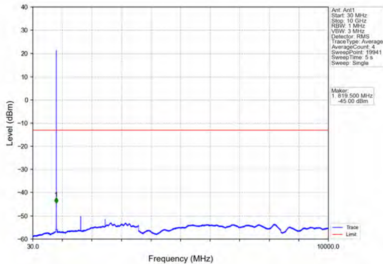
Band26a_1.4MHz_64QAM_HCH_823.3MHz_RB_1_5_NTNV
