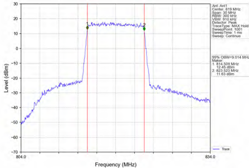
Band26a_10MHz_64QAM_LCH_819MHz_RB_50_0_NTNV
