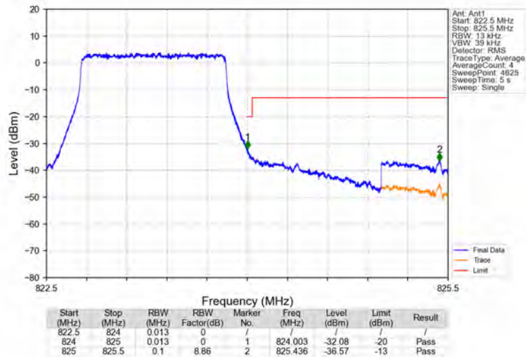
Band26a_1.4MHz_16QAM_HCH_823.3MHz_RB_6_0_NTNV
