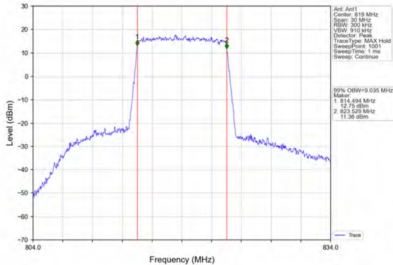
Band26a_10MHz_16QAM_MCH_819MHz_RB_50_0_NTNV
