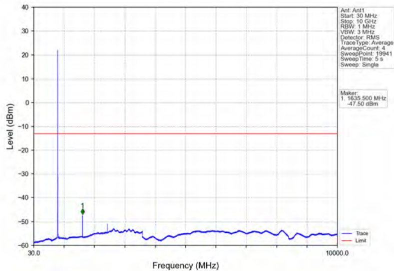
Band26a_3MHz_16QAM_HCH_822.5MHz_RB_1_0_NTNV
