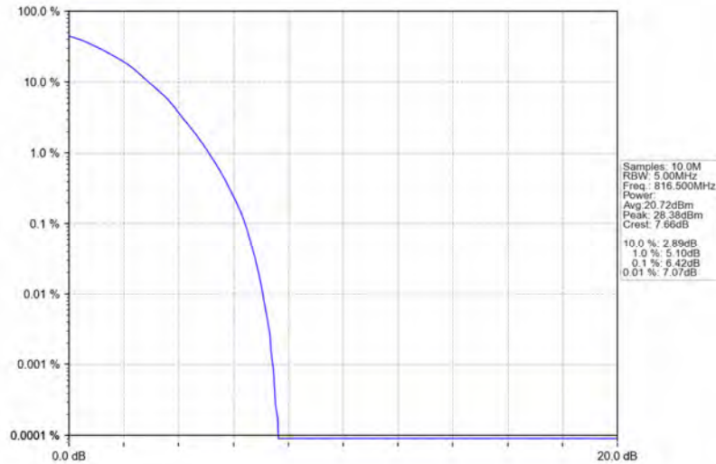
Band26a_5MHz_64QAM_LCH_816.5MHz_RB_25_0_NTNV
