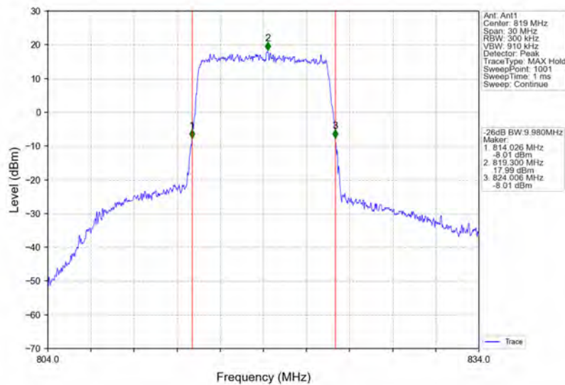
Band26a_10MHz_16QAM_MCH_819MHz_RB_50_0_NTNV
