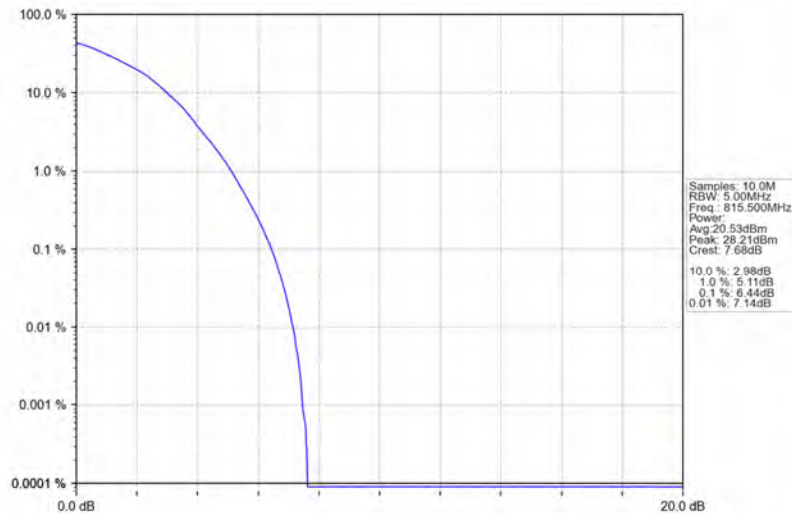
Band26a_3MHz_64QAM_LCH_815.5MHz_RB_15_0_NTNV
