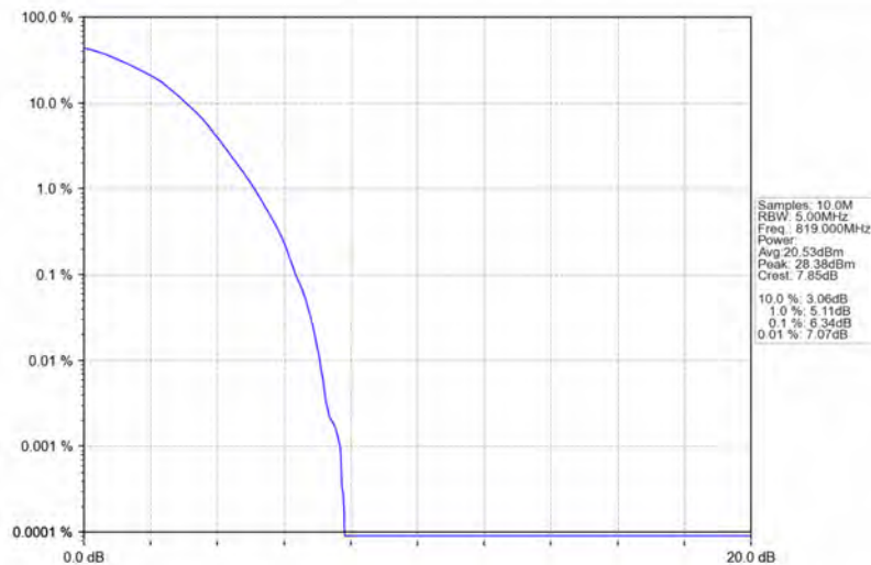
Band26a_1.4MHz_64QAM_MCH_819MHz_RB_6_0_NTNV
