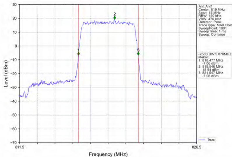
Band26a_5MHz_QPSK_MCH_819MHz_RB_25_0_NTNV
