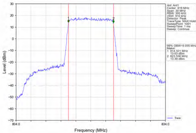
Band26a_10MHz_QPSK_HCH_819MHz_RB_50_0_NTNV
