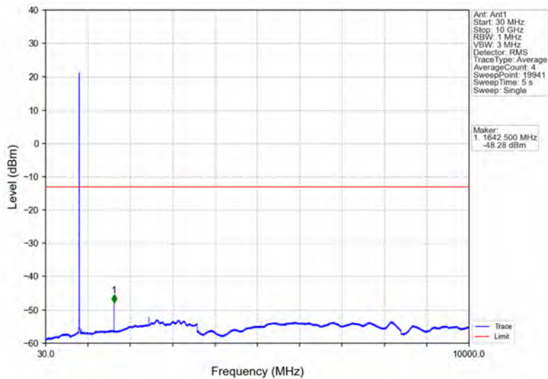
Band26a_3MHz_64QAM_HCH_822.5MHz_RB_1_14_NTNV
