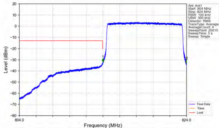
Band26a_10MHz_16QAM_LCH_819MHz_RB_50_0_NTNV
