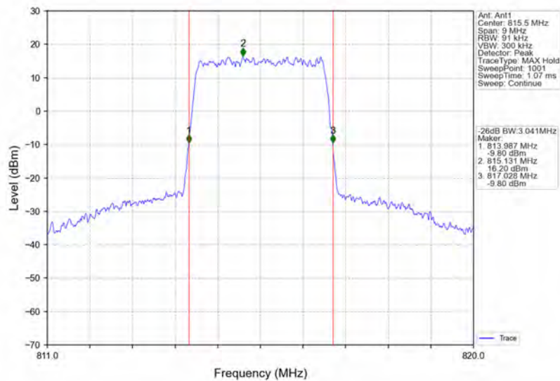
Band26a_3MHz_64QAM_LCH_815.5MHz_RB_15_0_NTNV
