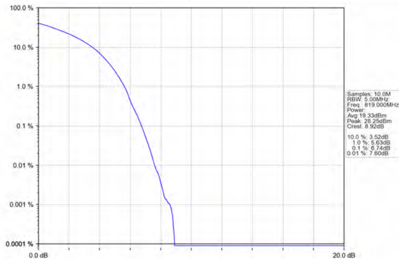
Band26a_10MHz_16QAM_HCH_819MHz_RB_50_0_NTNV
