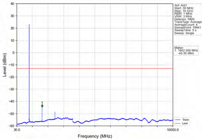
Band26a_3MHz_QPSK_HCH_822.5MHz_RB_1_14_NTNV
