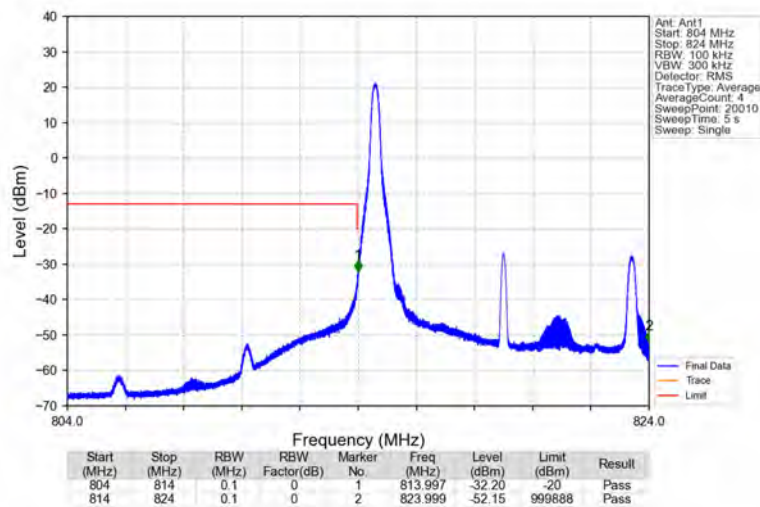
Band26a_10MHz_16QAM_LCH_819MHz_RB_1_0_NTNV
