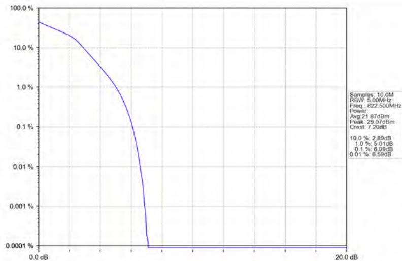
Band26a_3MHz_16QAM_HCH_822.5MHz_RB_15_0_NTNV
