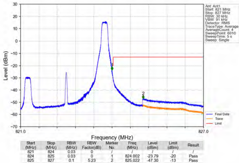
Band26a_3MHz_16QAM_HCH_822.5MHz_RB_1_14_NTNV
