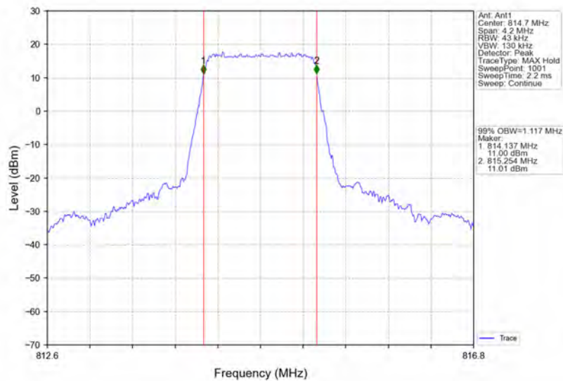
Band26a_1.4MHz_16QAM_LCH_814.7MHz_RB_6_0_NTNV
