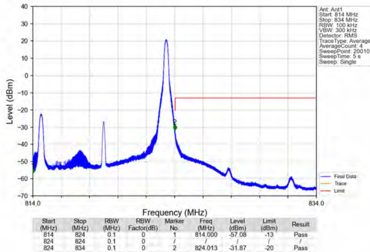
Band26a_10MHz_16QAM_HCH_819MHz_RB_1_49_NTNV
