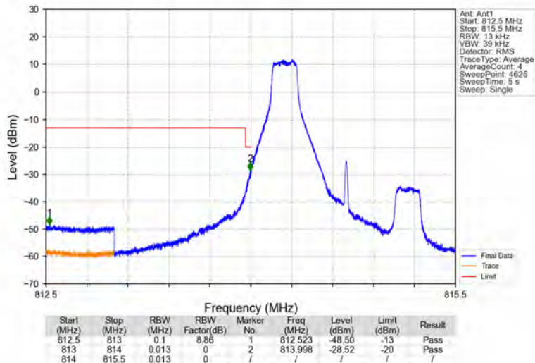
Band26a_1.4MHz_64QAM_LCH_814.7MHz_RB_1_0_NTNV
