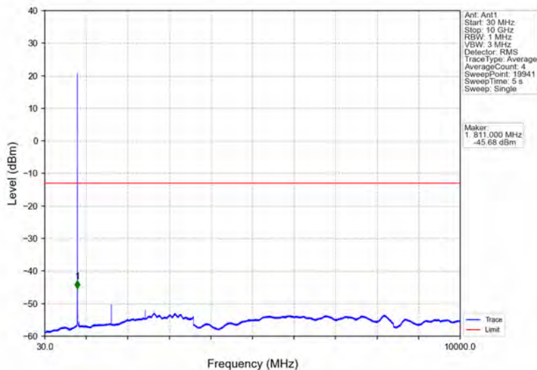
Band26a_1.4MHz_64QAM_LCH_814.7MHz_RB_1_0_NTNV
