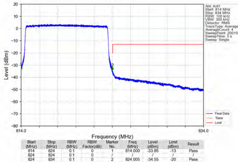
Band26a_10MHz_16QAM_HCH_819MHz_RB_50_0_NTNV
