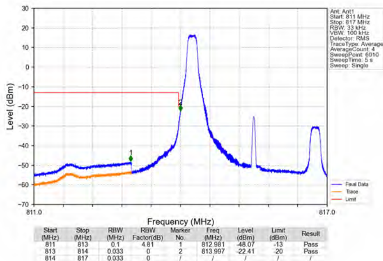
Band26a_3MHz_16QAM_LCH_815.5MHz_RB_1_0_NTNV
