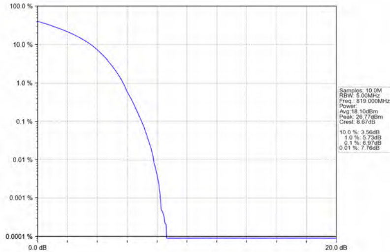
Band26a_10MHz_64QAM_HCH_819MHz_RB_50_0_NTNV
