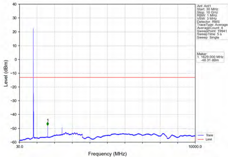
Band26a_10MHz_16QAM_HCH_819MHz_RB_1_0_NTNV
