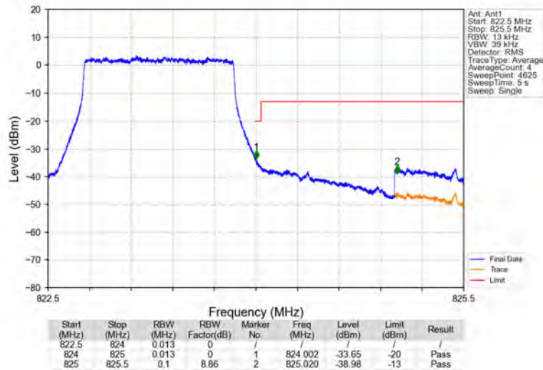
Band26a_1.4MHz_64QAM_HCH_823.3MHz_RB_6_0_NTNV
