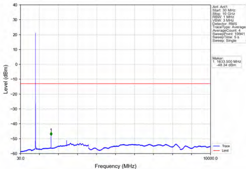
Band26a_5MHz_64QAM_MCH_819MHz_RB_1_0_NTNV
