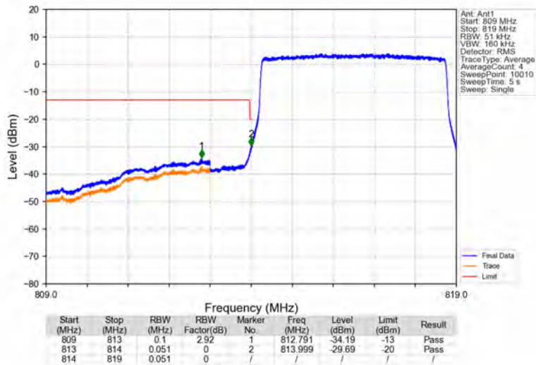
Band26a_5MHz_16QAM_LCH_816.5MHz_RB_25_0_NTNV
