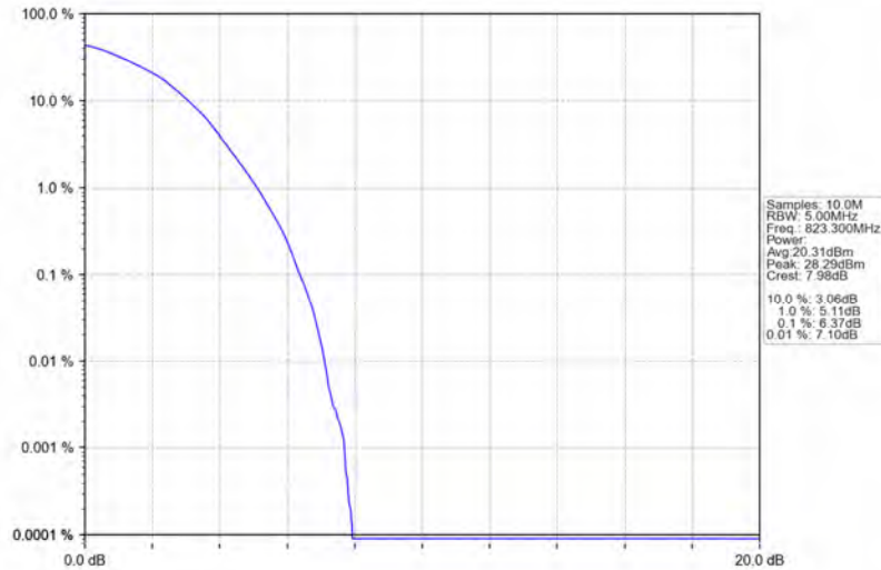
Band26a_1.4MHz_64QAM_HCH_823.3MHz_RB_6_0_NTNV
