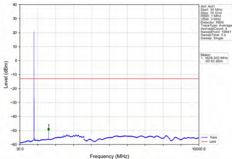
Band26a_5MHz_64QAM_LCH_816.5MHz_RB_1_0_NTNV
