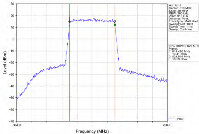
Band26a_10MHz_16QAM_MCH_819MHz_RB_50_0_NTNV
