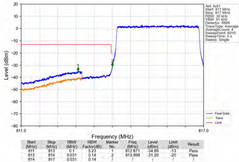
Band26a_3MHz_64QAM_LCH_815.5MHz_RB_15_0_NTNV
