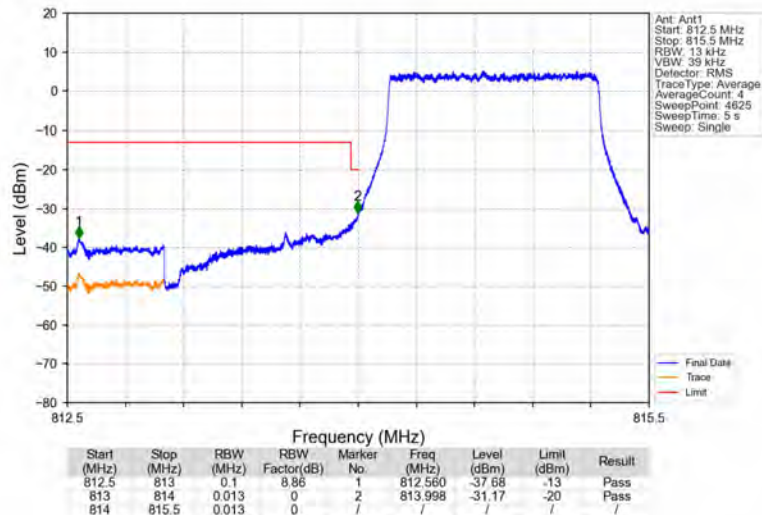
Band26a_1.4MHz_QPSK_LCH_814.7MHz_RB_6_0_NTNV
