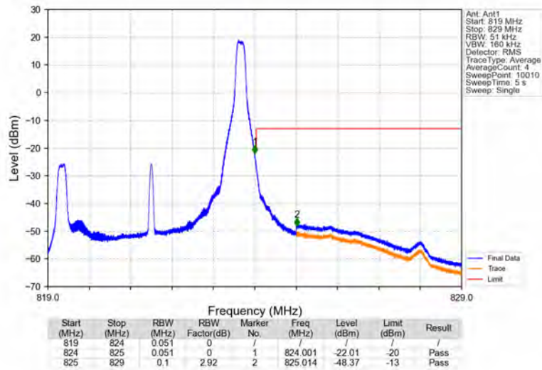
Band26a_5MHz_QPSK_HCH_821.5MHz_RB_1_24_NTNV
