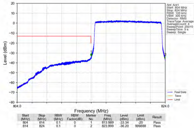
Band26a_10MHz_64QAM_LCH_819MHz_RB_50_0_NTNV
