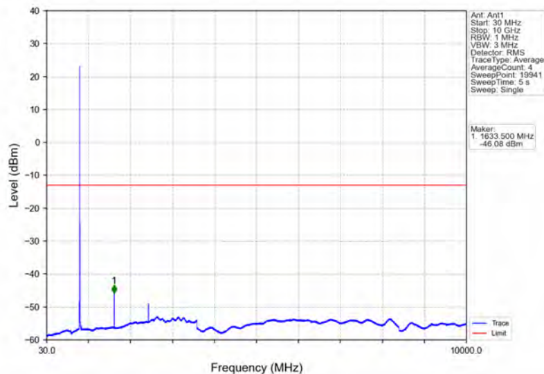
Band26a_5MHz_QPSK_MCH_819MHz_RB_1_0_NTNV
