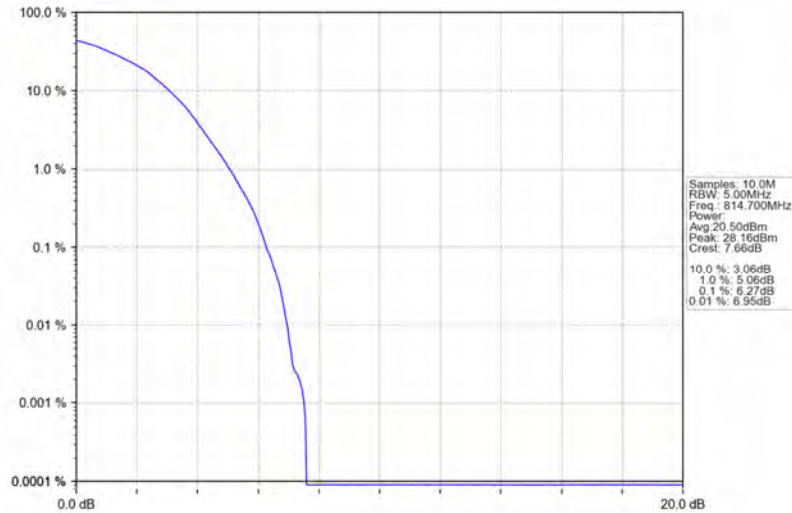
Band26a_1.4MHz_64QAM_LCH_814.7MHz_RB_6_0_NTNV
