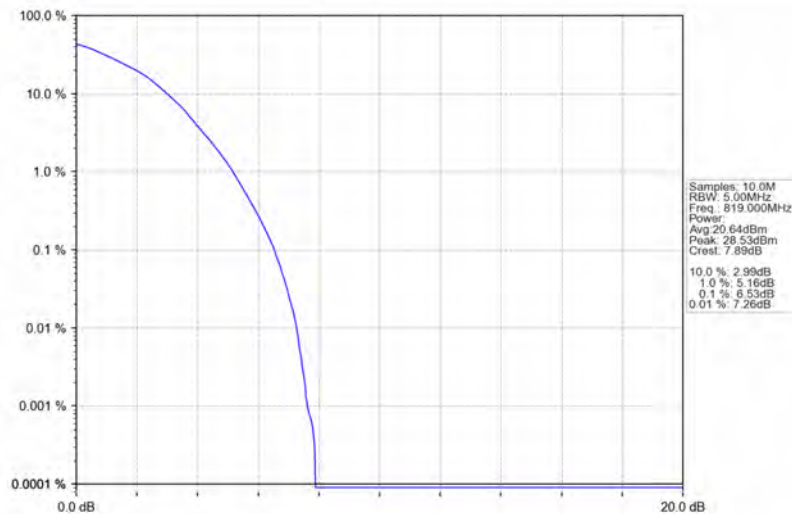
Band26a_3MHz_64QAM_MCH_819MHz_RB_15_0_NTNV
