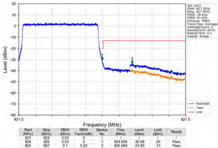
Band26a_3MHz_64QAM_HCH_822.5MHz_RB_15_0_NTNV
