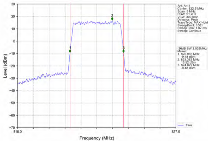
Band26a_3MHz_64QAM_HCH_822.5MHz_RB_15_0_NTNV
