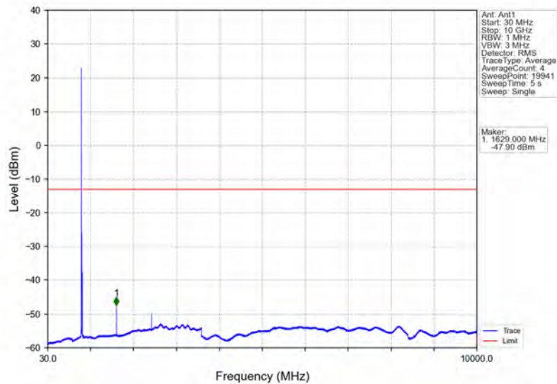
Band26a_10MHz_16QAM_LCH_819MHz_RB_50_0_NTNV
