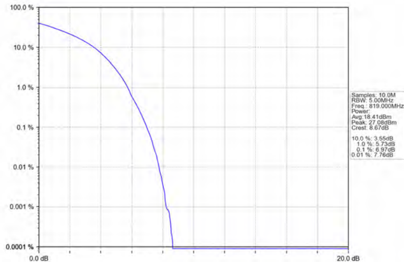
Band26a_10MHz_64QAM_LCH_819MHz_RB_50_0_NTNV
