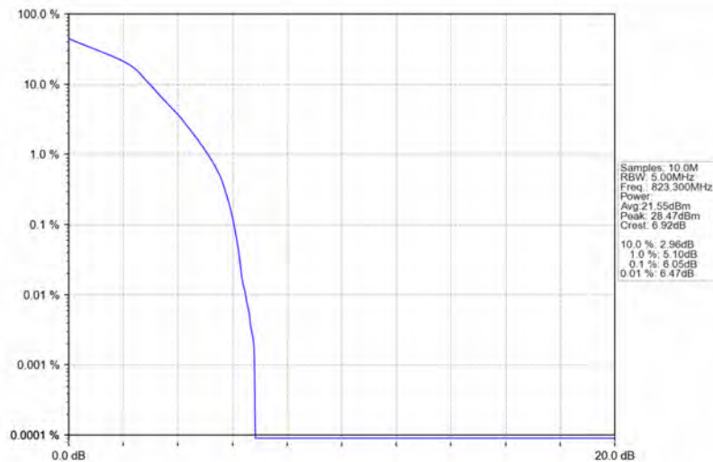
Band26a_1.4MHz_16QAM_HCH_823.3MHz_RB_6_0_NTNV
