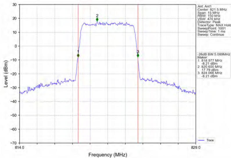
Band26a_5MHz_16QAM_HCH_821.5MHz_RB_25_0_NTNV
