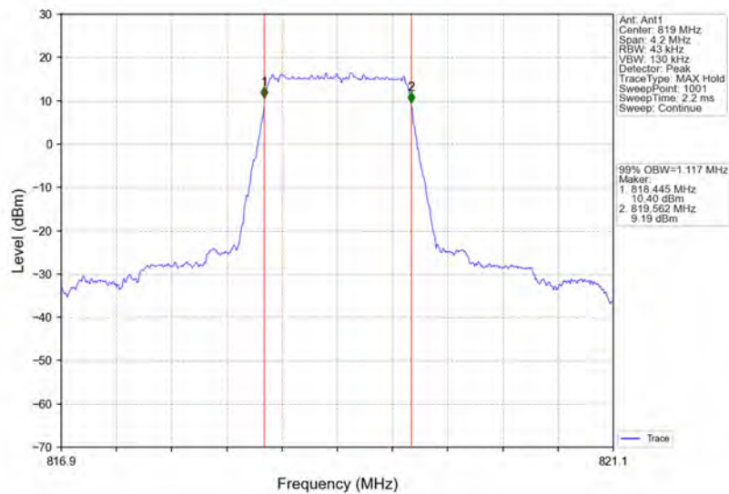
Band26a_1.4MHz_64QAM_MCH_819MHz_RB_6_0_NTNV
