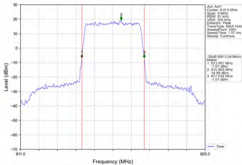
Band26a_3MHz_QPSK_LCH_815.5MHz_RB_15_0_NTNV
