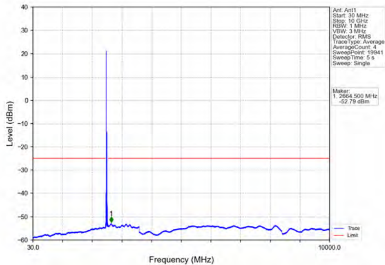
Band41_20MHz_16QAM_LCH_2506MHz_RB_1_0_NTNV
