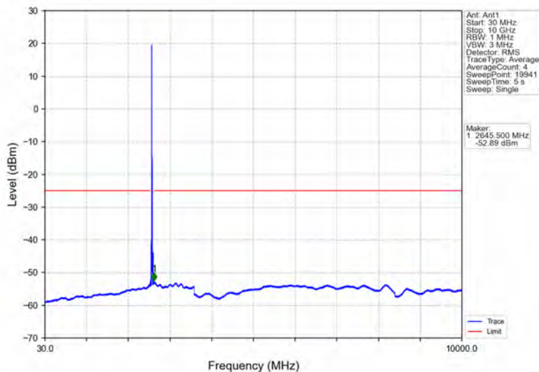
Band41_20MHz_64QAM_MCH_2593MHz_RB_1_0_NTNV
