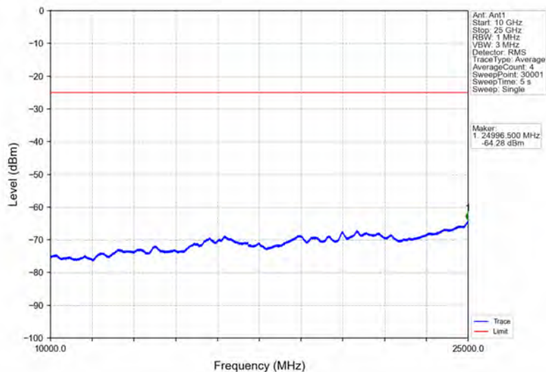
Band41_20MHz_64QAM_HCH_2680MHz_RB_1_0_NTNV
