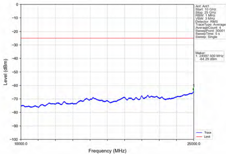
Band41_10MHz_64QAM_HCH_2685MHz_RB_1_0_NTNV
