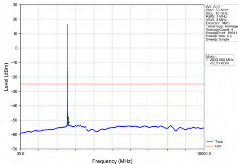
Band41_15MHz_64QAM_MCH_2593MHz_RB_1_0_NTNV
