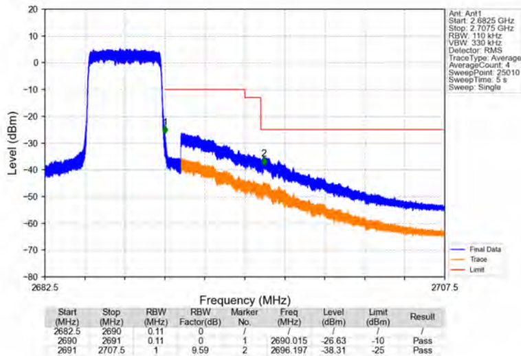
Band41_5MHz_16QAM_HCH_2687.5MHz_RB_25_0_NTNV
