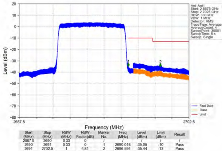
Band41_15MHz_64QAM_HCH_2682.5MHz_RB_75_0_NTNV
