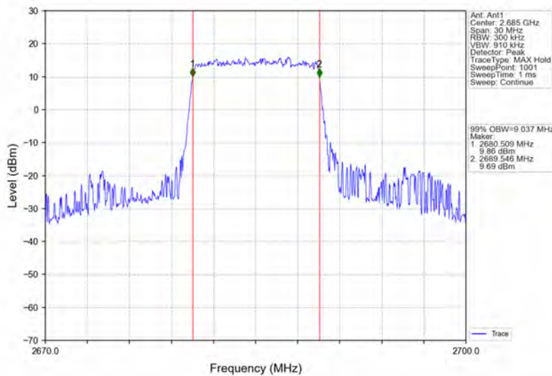
Band41_10MHz_64QAM_HCH_2685MHz_RB_50_0_NTNV
