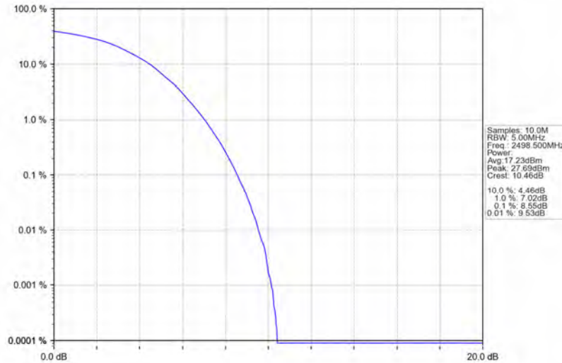
Band41_5MHz_64QAM_LCH_2498.5MHz_RB_25_0_NTNV
