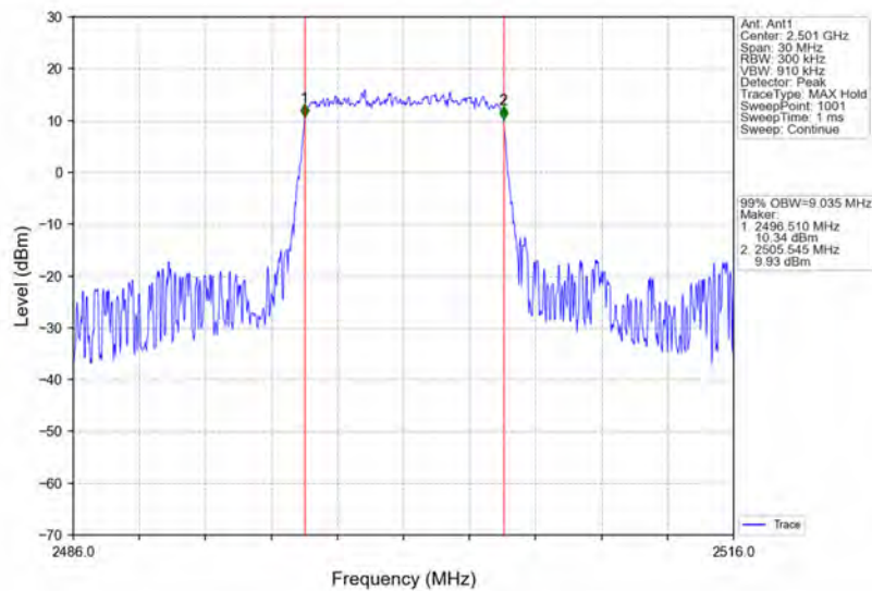
Band41_10MHz_64QAM_LCH_2501MHz_RB_50_0_NTNV
