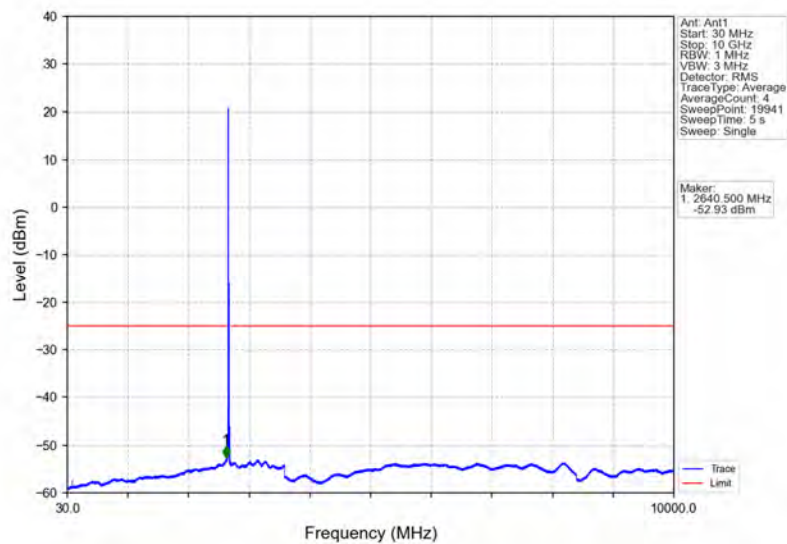
Band41_15MHz_64QAM_HCH_2682.5MHz_RB_1_0_NTNV
