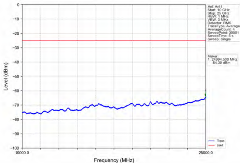
Band41_15MHz_16QAM_MCH_2593MHz_RB_1_0_NTNV
