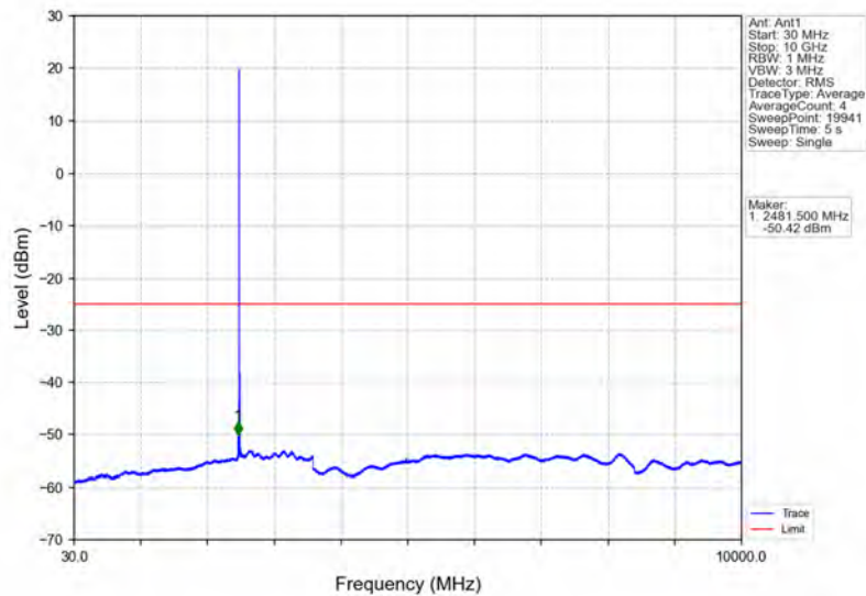
Band41_5MHz_16QAM_LCH_2498.5MHz_RB_1_0_NTNV
