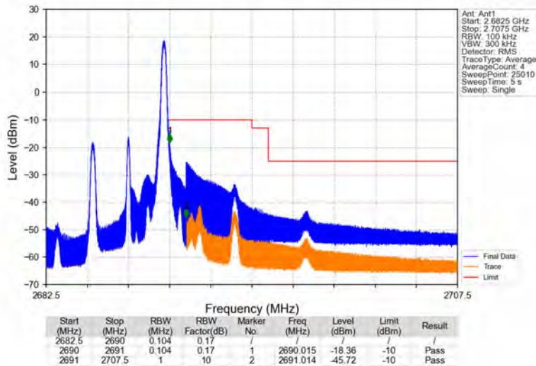
Band41_5MHz_16QAM_HCH_2687.5MHz_RB_1_24_NTNV
