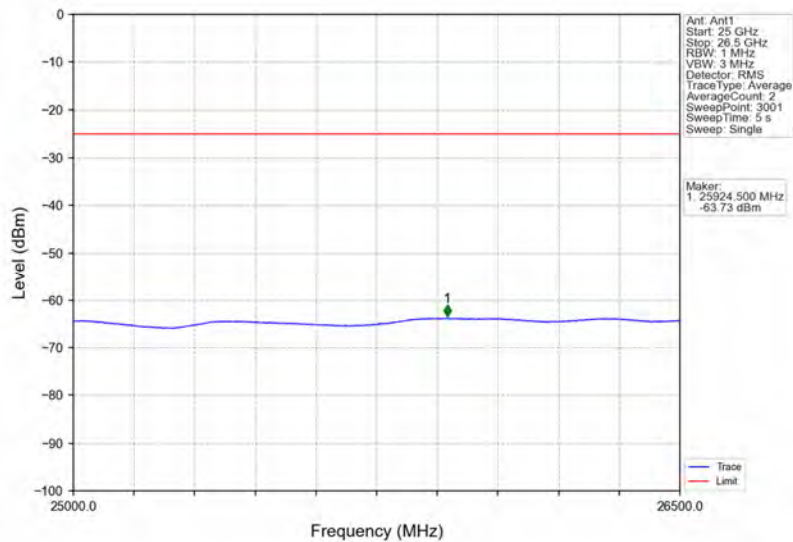
Band41_5MHz_16QAM_LCH_2498.5MHz_RB_25_0_NTNV
