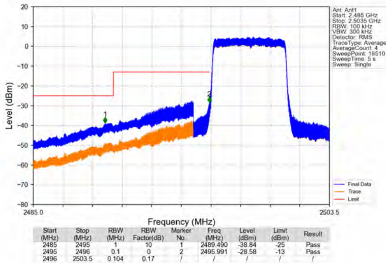
Band41_5MHz_16QAM_LCH_2498.5MHz_RB_25_0_NTNV
