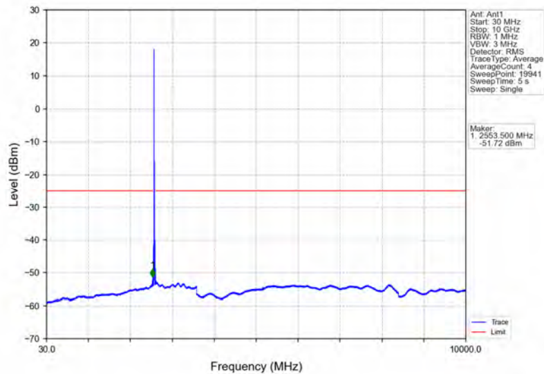
Band41_15MHz_16QAM_MCH_2593MHz_RB_1_0_NTNV
