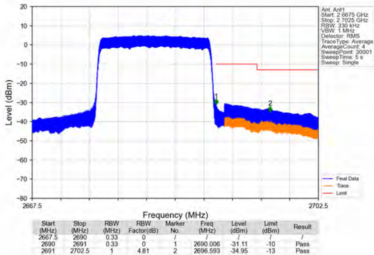
Band41_15MHz_16QAM_HCH_2682.5MHz_RB_75_0_NTNV
