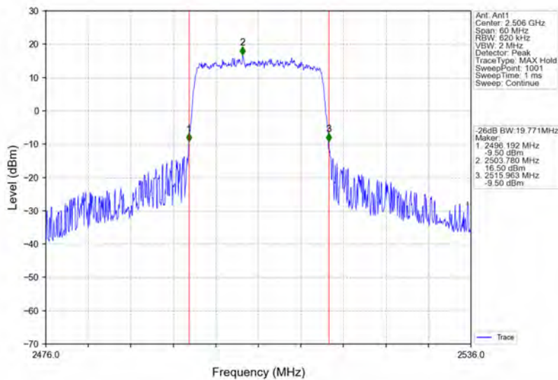
Band41_20MHz_64QAM_LCH_2506MHz_RB_100_0_NTNV
