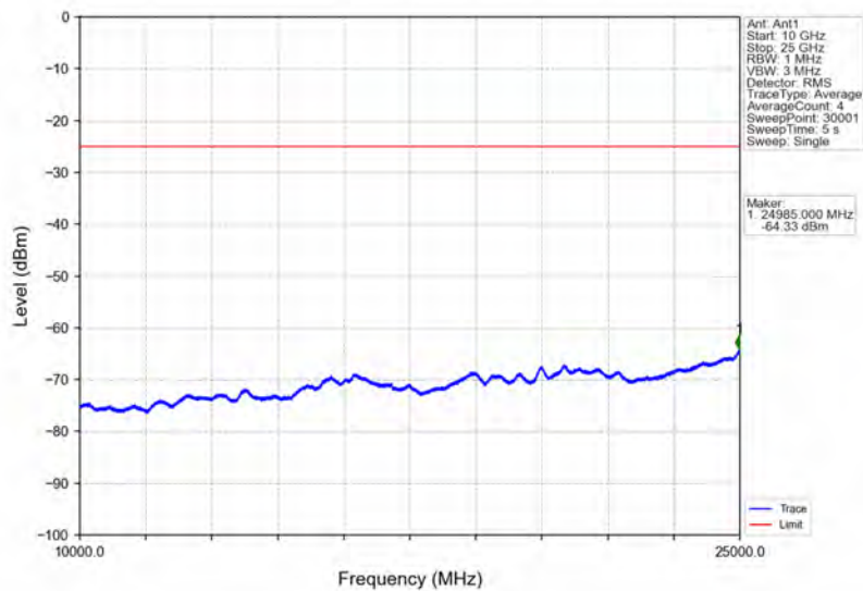
Band41_15MHz_16QAM_LCH_2503.5MHz_RB_1_0_NTNV
