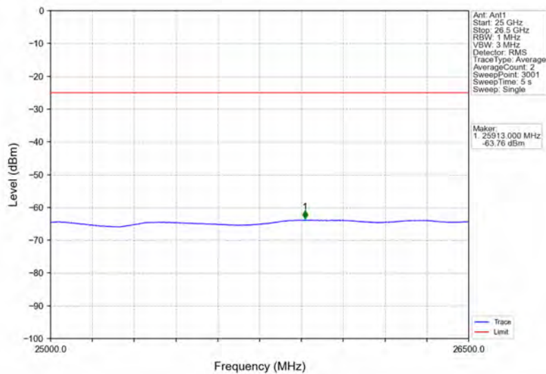
Band41_15MHz_64QAM_MCH_2593MHz_RB_1_0_NTNV
