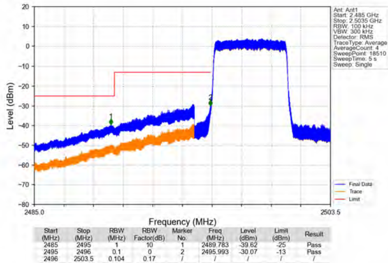
Band41_5MHz_64QAM_LCH_2498.5MHz_RB_25_0_NTNV
