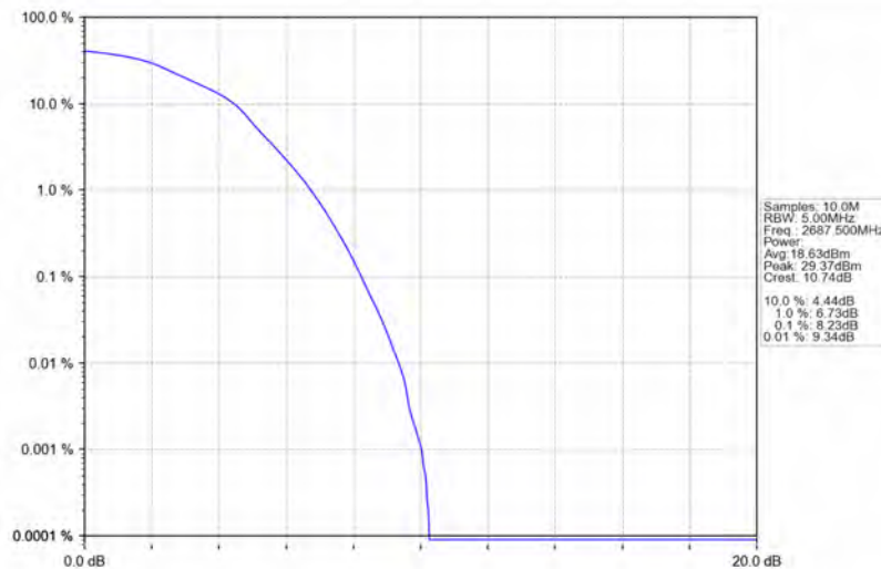
Band41_5MHz_16QAM_HCH_2687.5MHz_RB_25_0_NTNV
