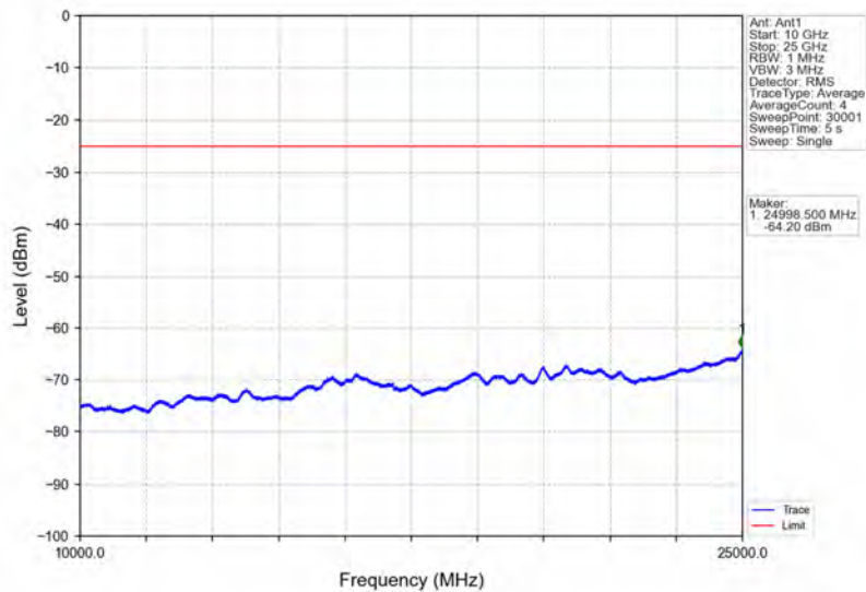
Band41_20MHz_64QAM_MCH_2593MHz_RB_1_0_NTNV
