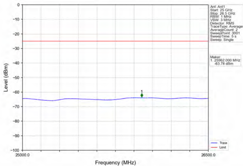
Band41_20MHz_64QAM_LCH_2506MHz_RB_1_0_NTNV
