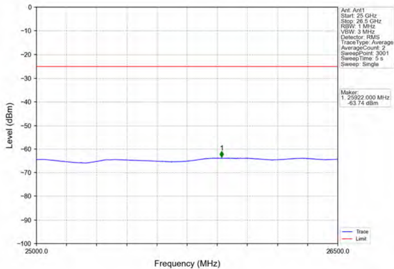
Band41_20MHz_16QAM_HCH_2680MHz_RB_1_0_NTNV
