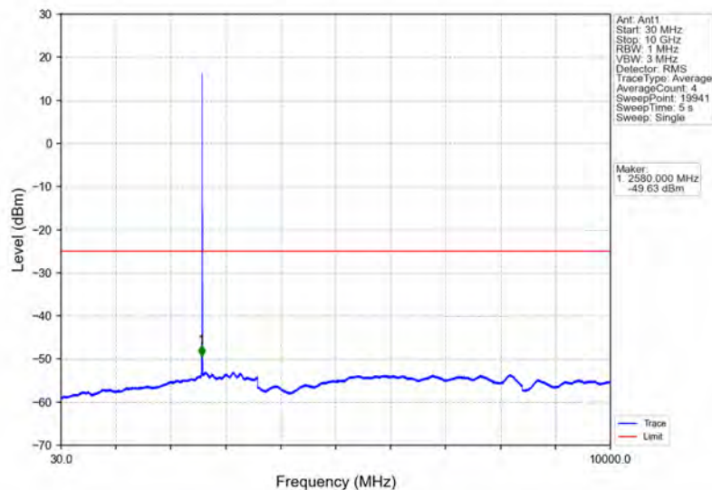
Band41_5MHz_64QAM_MCH_2593MHz_RB_1_0_NTNV
