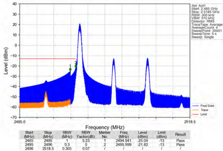
Band41_15MHz_64QAM_LCH_2503.5MHz_RB_1_0_NTNV
