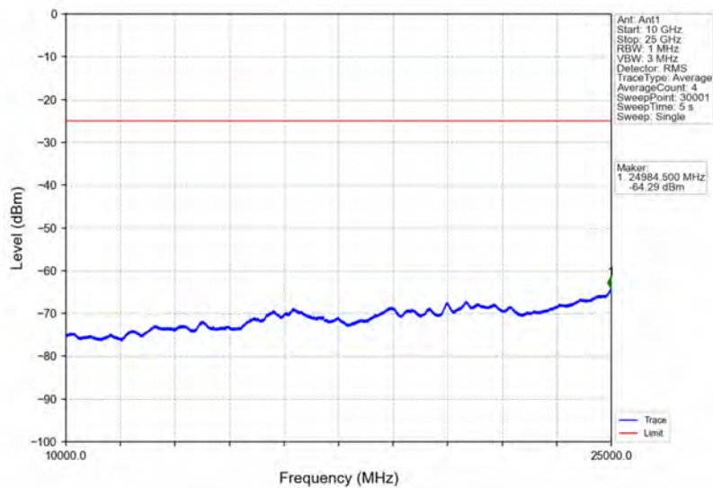
Band41_5MHz_64QAM_HCH_2687.5MHz_RB_1_0_NTNV
