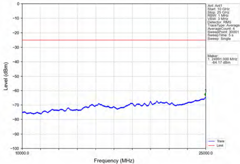
Band41_5MHz_64QAM_MCH_2593MHz_RB_1_0_NTNV
