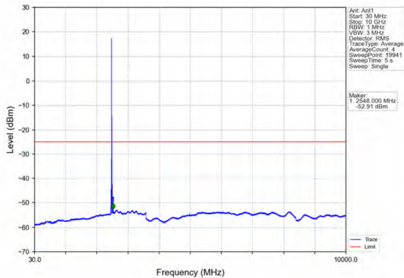
Band41_15MHz_16QAM_LCH_2503.5MHz_RB_1_0_NTNV
