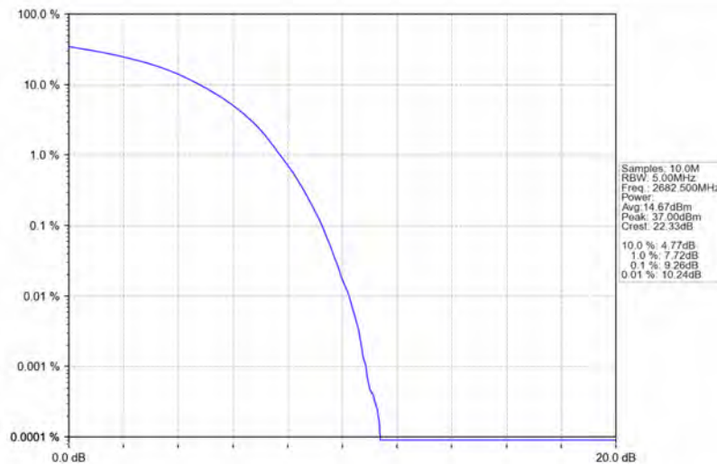
Band41_15MHz_16QAM_HCH_2682.5MHz_RB_75_0_NTNV
