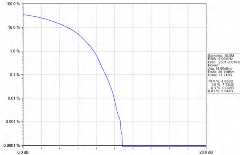
Band41_10MHz_64QAM_LCH_2501MHz_RB_50_0_NTNV
