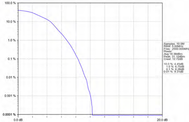
Band41_5MHz_16QAM_MCH_2593MHz_RB_25_0_NTNV
