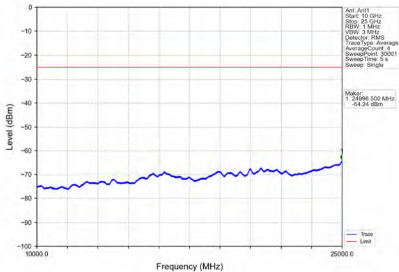
Band41_10MHz_64QAM_MCH_2593MHz_RB_1_0_NTNV
