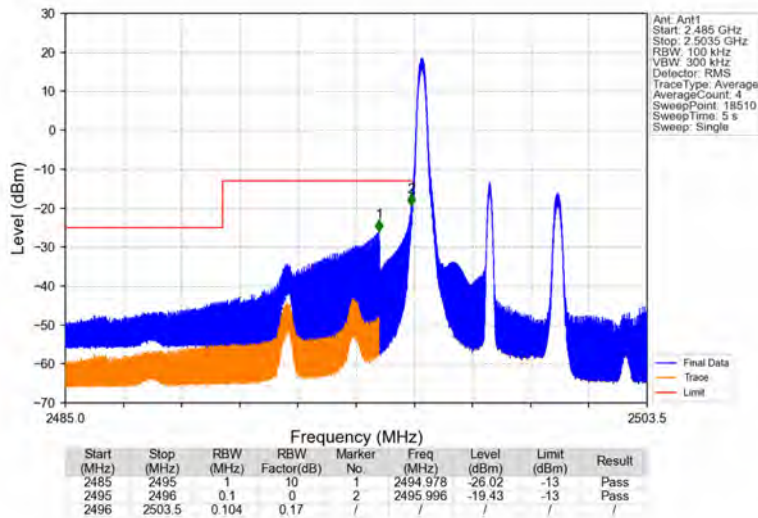
Band41_5MHz_16QAM_LCH_2498.5MHz_RB_1_0_NTNV
