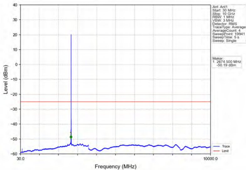
Band41_5MHz_16QAM_HCH_2687.5MHz_RB_1_0_NTNV
