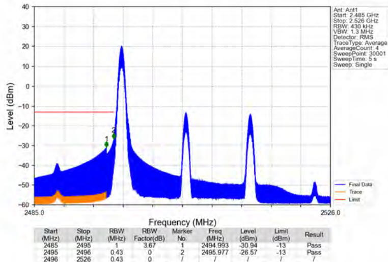
Band41_20MHz_64QAM_LCH_2506MHz_RB_1_0_NTNV
