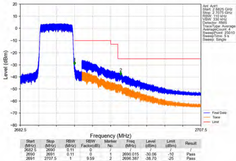
Band41_5MHz_64QAM_HCH_2687.5MHz_RB_25_0_NTNV
