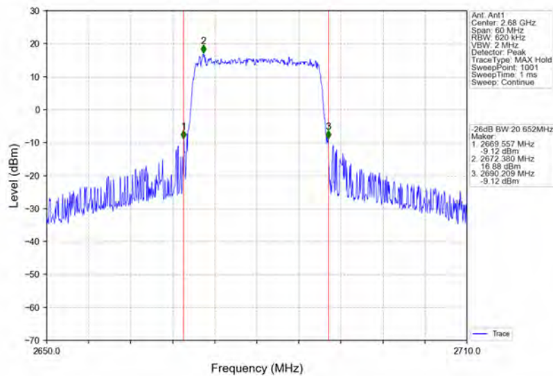
Band41_20MHz_64QAM_HCH_2680MHz_RB_100_0_NTNV
