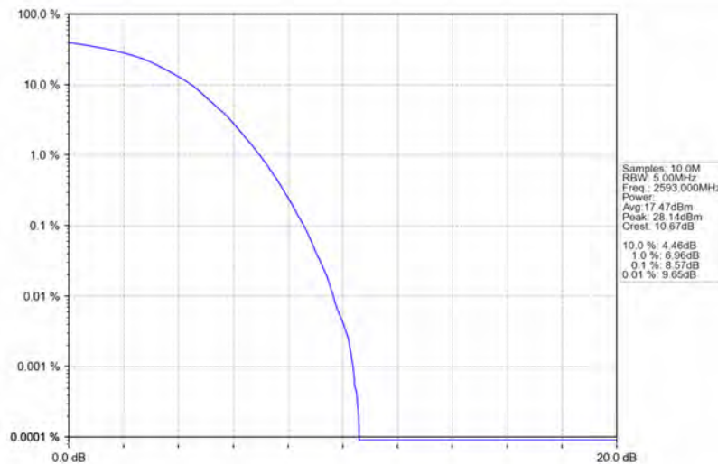
Band41_5MHz_64QAM_MCH_2593MHz_RB_25_0_NTNV
