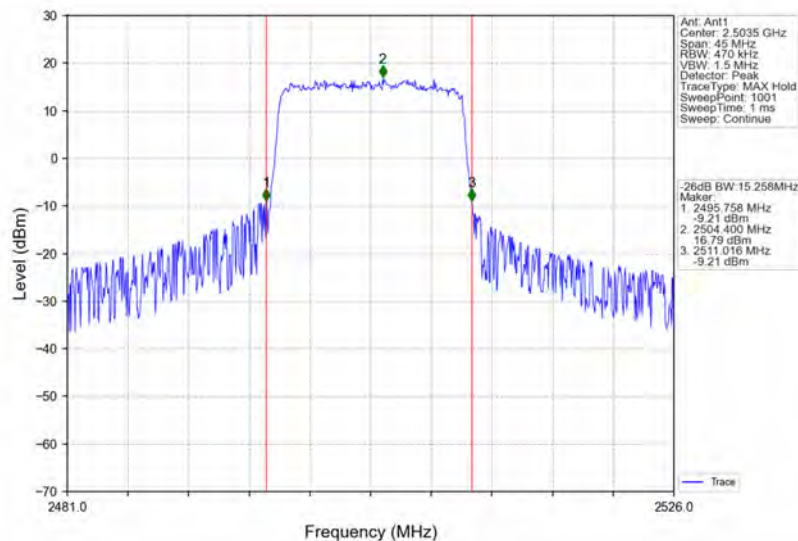
Band41_15MHz_16QAM_LCH_2503.5MHz_RB_75_0_NTNV
