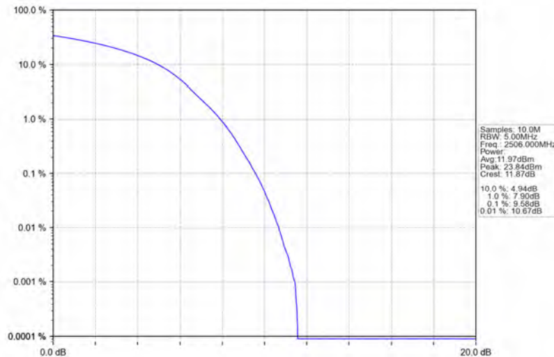
Band41_20MHz_64QAM_LCH_2506MHz_RB_100_0_NTNV
