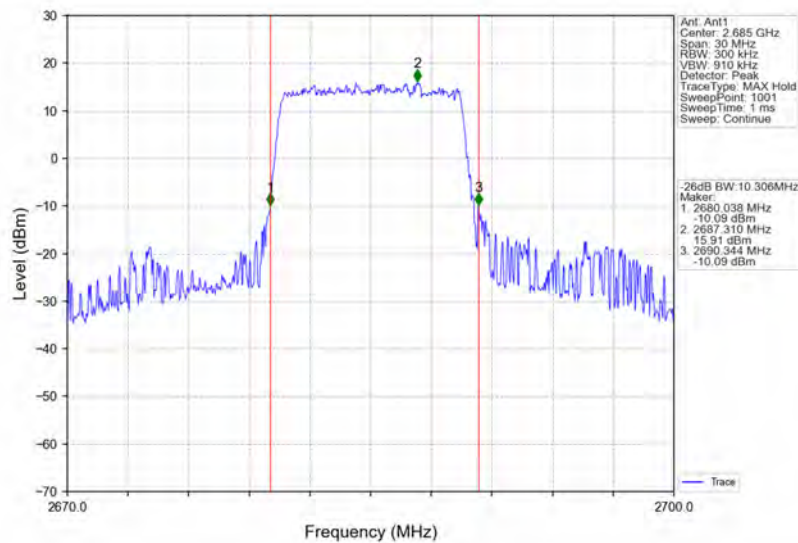
Band41_10MHz_64QAM_HCH_2685MHz_RB_50_0_NTNV
