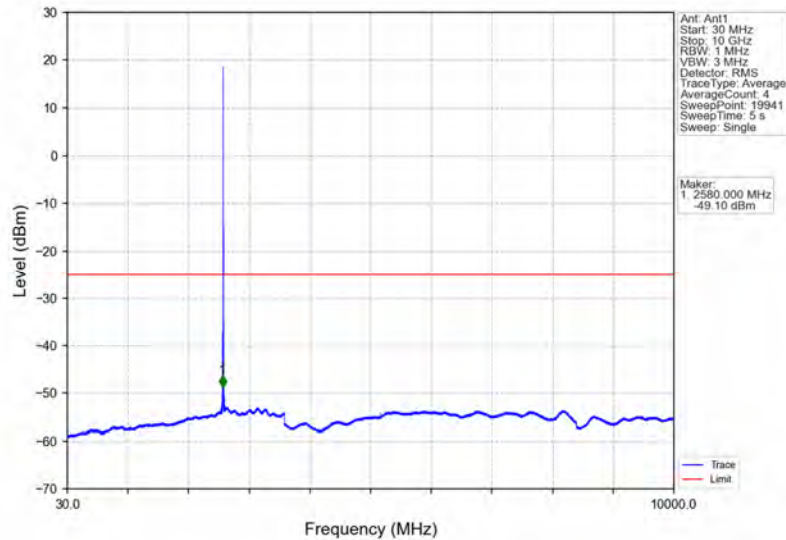
Band41_5MHz_16QAM_MCH_2593MHz_RB_1_0_NTNV
