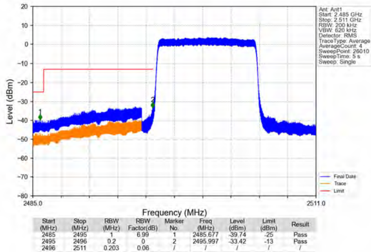
Band41_10MHz_64QAM_LCH_2501MHz_RB_50_0_NTNV
