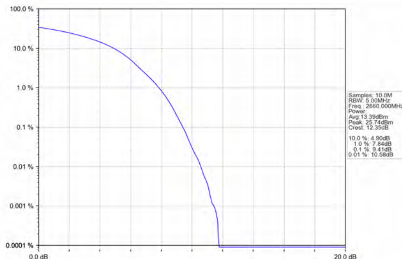
Band41_20MHz_16QAM_HCH_2680MHz_RB_100_0_NTNV
