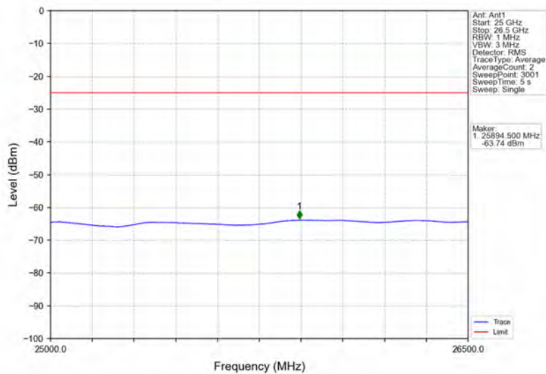
Band41_15MHz_64QAM_LCH_2503.5MHz_RB_1_0_NTNV
