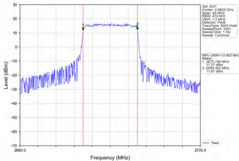
Band41_15MHz_16QAM_HCH_2682.5MHz_RB_75_0_NTNV
