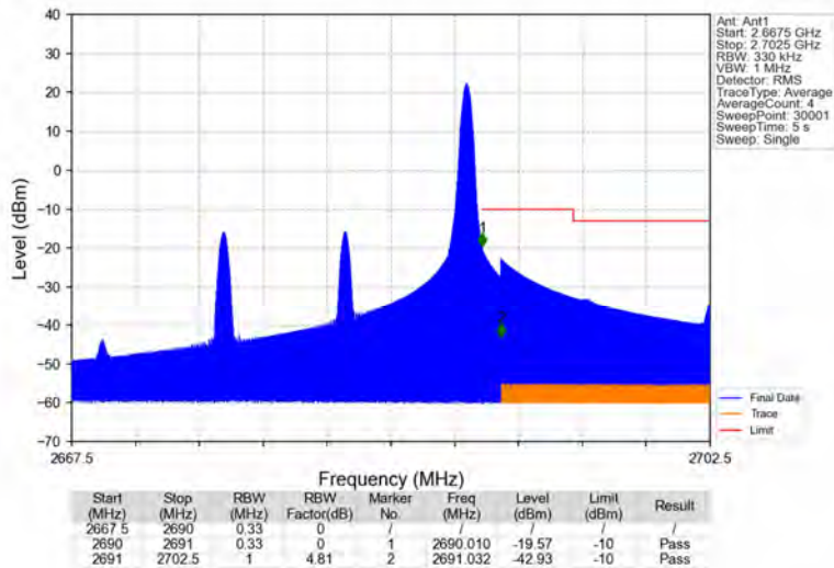
Band41_15MHz_16QAM_HCH_2682.5MHz_RB_1_74_NTNV
