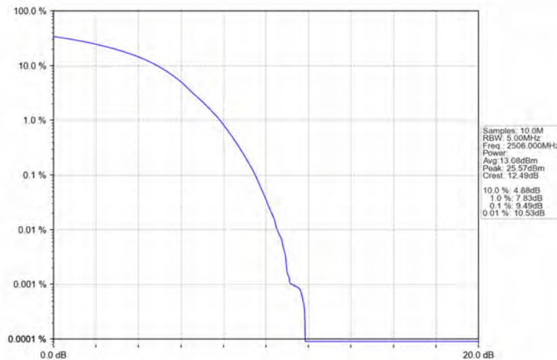
Band41_20MHz_16QAM_LCH_2506MHz_RB_100_0_NTNV
