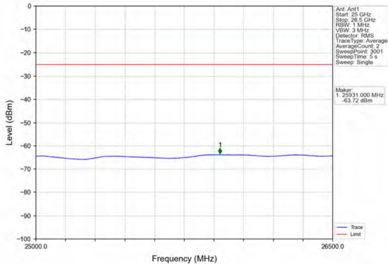
Band41_5MHz_16QAM_HCH_2687.5MHz_RB_1_0_NTNV
