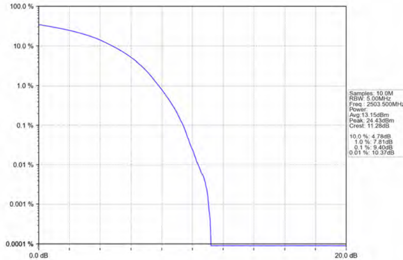
Band41_15MHz_64QAM_LCH_2503.5MHz_RB_75_0_NTNV
