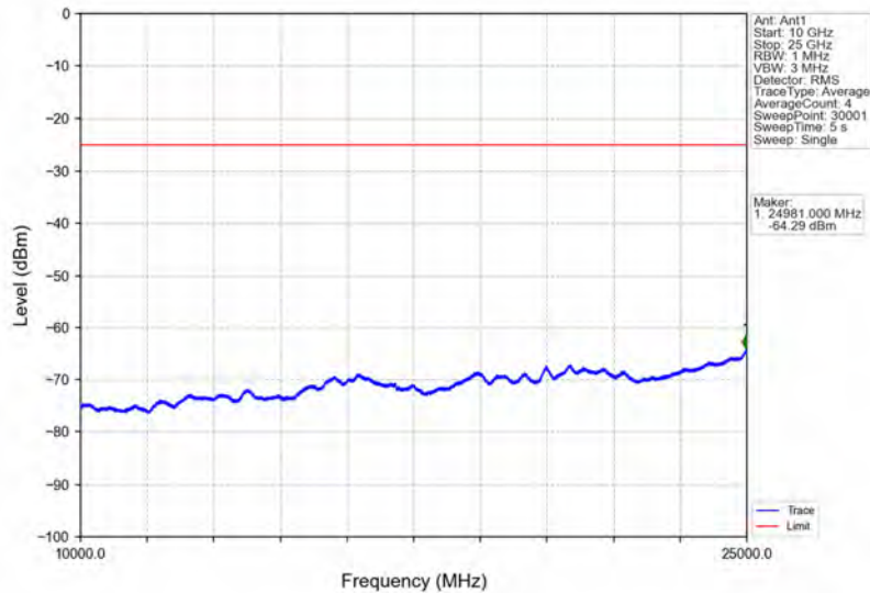
Band41_15MHz_64QAM_MCH_2593MHz_RB_1_0_NTNV
