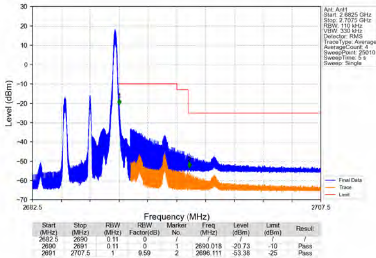
Band41_5MHz_64QAM_HCH_2687.5MHz_RB_1_24_NTNV
