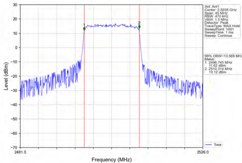
Band41_15MHz_16QAM_LCH_2503.5MHz_RB_75_0_NTNV
