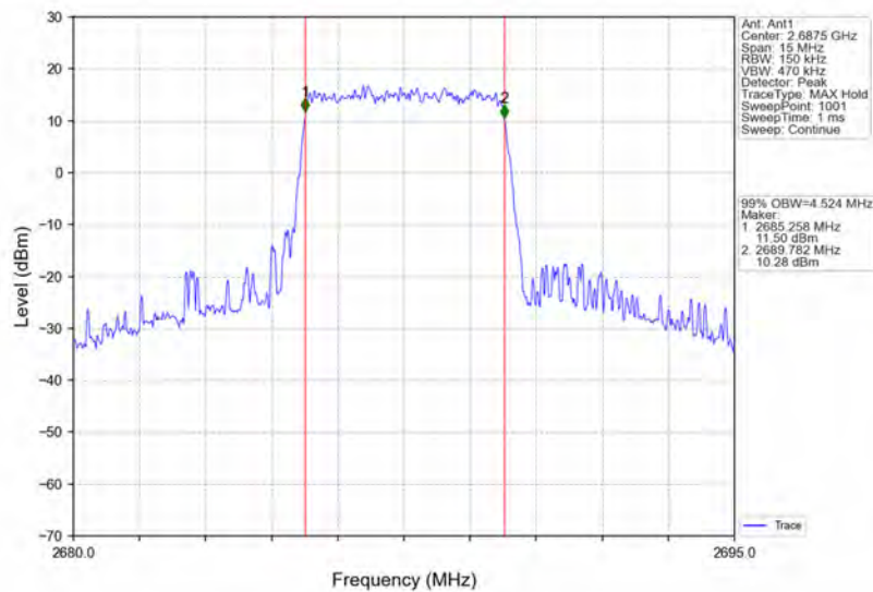
Band41_5MHz_16QAM_HCH_2687.5MHz_RB_25_0_NTNV
