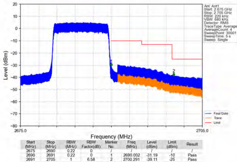
Band41_10MHz_64QAM_HCH_2685MHz_RB_50_0_NTNV
