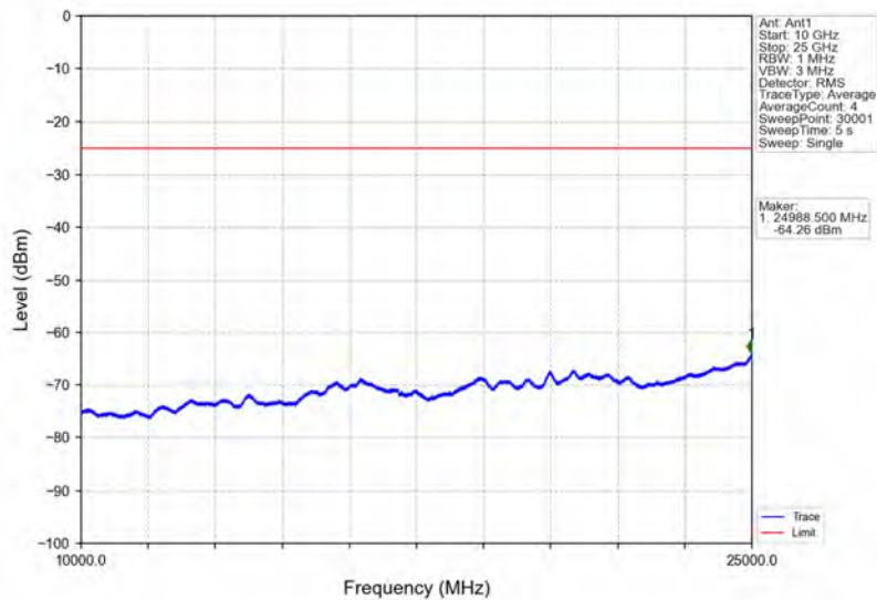
Band41_15MHz_16QAM_HCH_2682.5MHz_RB_1_0_NTNV
