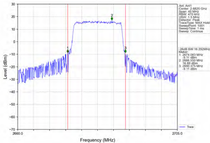
Band41_15MHz_16QAM_HCH_2682.5MHz_RB_75_0_NTNV
