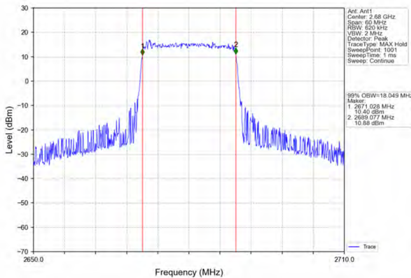
Band41_20MHz_64QAM_HCH_2680MHz_RB_100_0_NTNV
