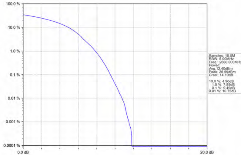
Band41_20MHz_64QAM_HCH_2680MHz_RB_100_0_NTNV
