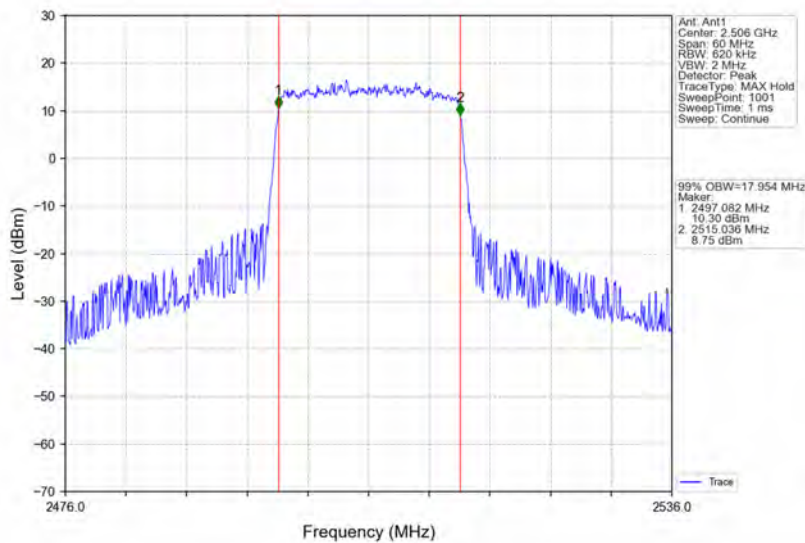
Band41_20MHz_64QAM_LCH_2506MHz_RB_100_0_NTNV
