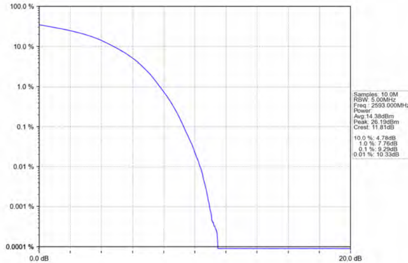
Band41_15MHz_16QAM_MCH_2593MHz_RB_75_0_NTNV
