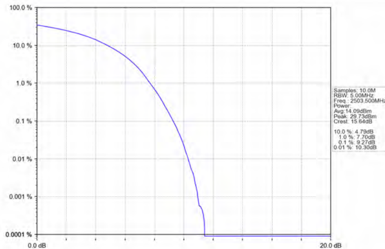
Band41_15MHz_16QAM_LCH_2503.5MHz_RB_75_0_NTNV
