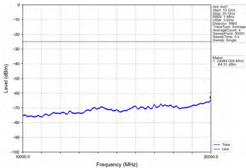
Band41_15MHz_64QAM_HCH_2682.5MHz_RB_1_0_NTNV
