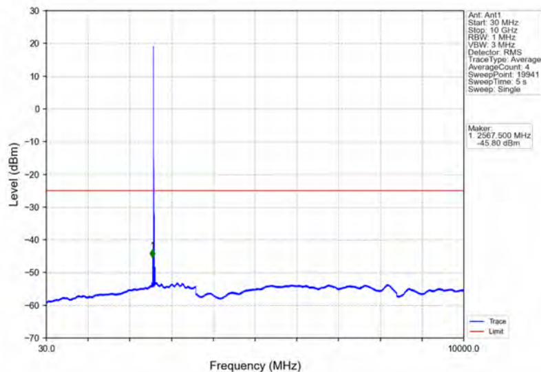
Band41_10MHz_64QAM_MCH_2593MHz_RB_1_0_NTNV
