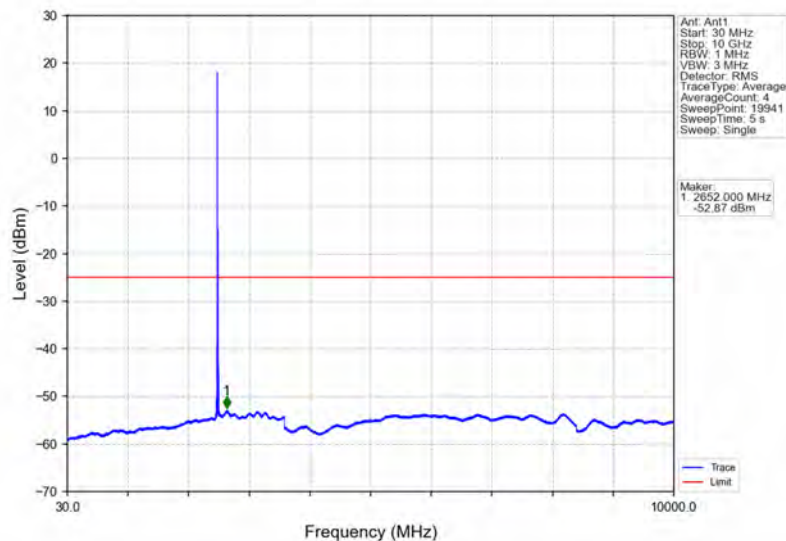
Band41_10MHz_64QAM_LCH_2501MHz_RB_1_0_NTNV
