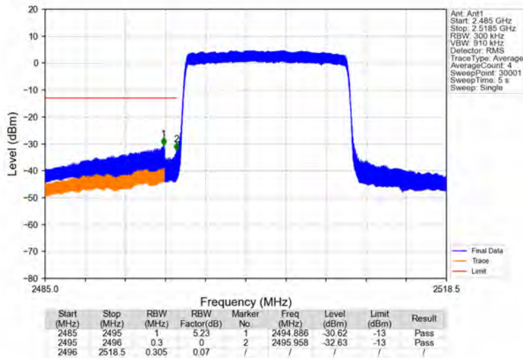
Band41_15MHz_16QAM_LCH_2503.5MHz_RB_75_0_NTNV
