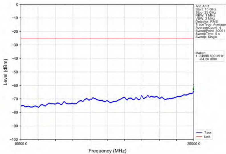
Band41_5MHz_16QAM_LCH_2498.5MHz_RB_1_0_NTNV
