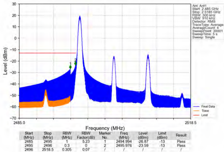
Band41_15MHz_16QAM_LCH_2503.5MHz_RB_1_0_NTNV
