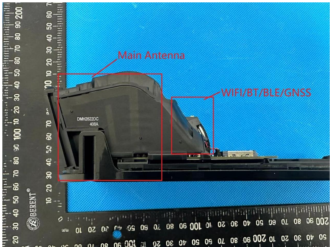
Antenna position
