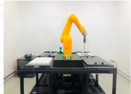
Figure 7.4.2-1: DASY6
