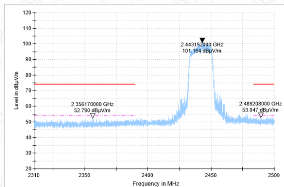
Bandedge-11N(20M)-CH7-PK
