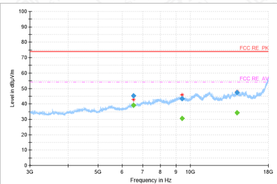
RSE-11N(40M)-CH9-3GHz-18GHz
