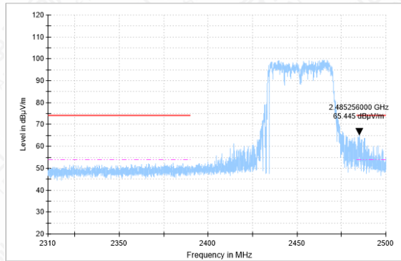
Bandedge-11N(40M)-CH9-PK
