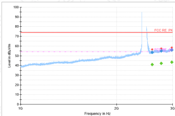
RSE-11N(40M)-CH9-1GHz-3GHz
