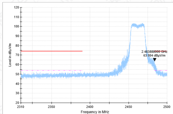
Bandedge-11N(20M)-CH11-PK
