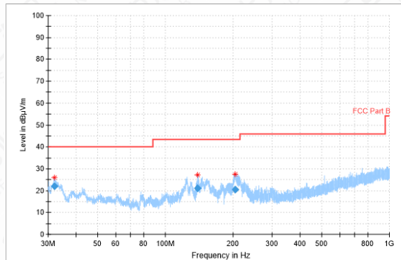
RSE-11B-CH7-30MHz-1GHz
