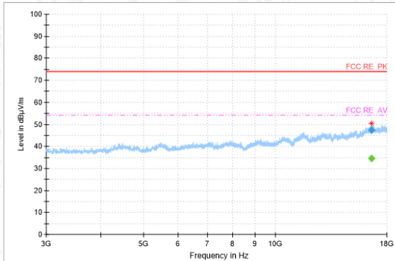
RSE-11N(40M)-CH7-3GHz-18GHz
