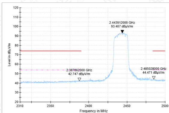
Bandedge -11N(20M)-CH7-AV
