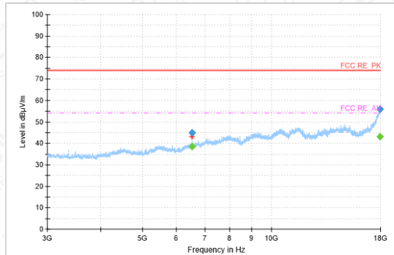
RSE-11N(40M)-CH9-3GHz-18GHz
