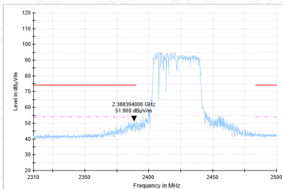
Bandedge-11N(40M)-CH3-AV
