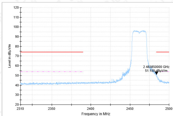
Bandedge-11N(20M)-CH11-AV
