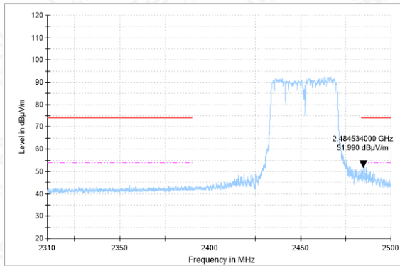
Bandedge-11N(40M)-CH9-AV
