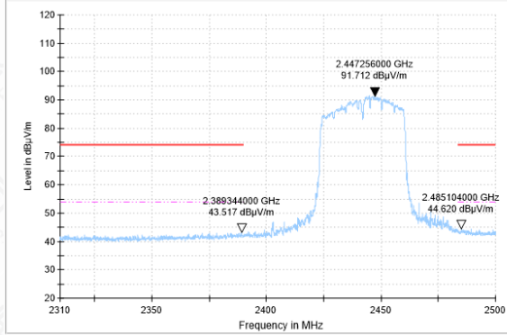
Bandedge-11N(40M)-CH9-AV
