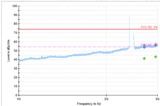
RSE-11N(40M)-CH9-1GHz-3GHz
