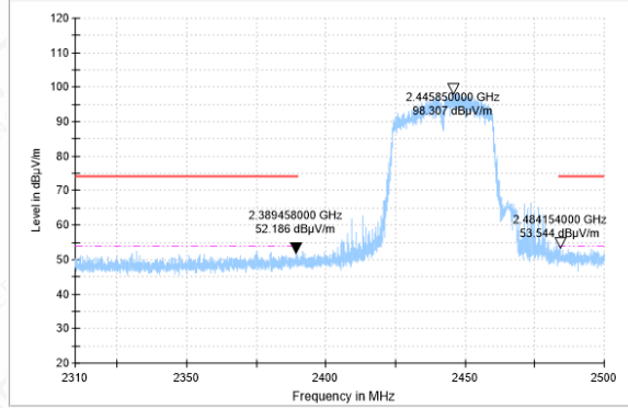
Bandedge-11N(40M)-CH9-PK
