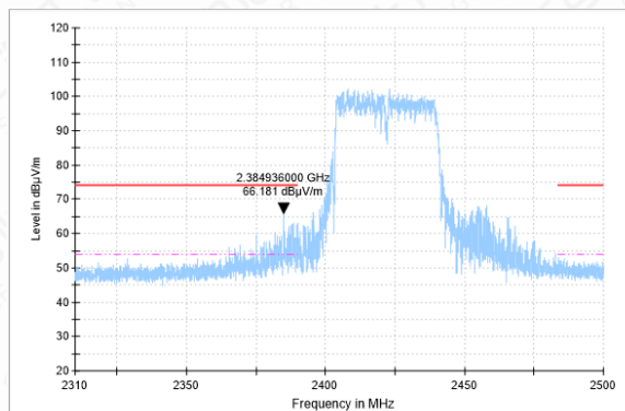
Bandedge-11N(40M)-CH3-PK
