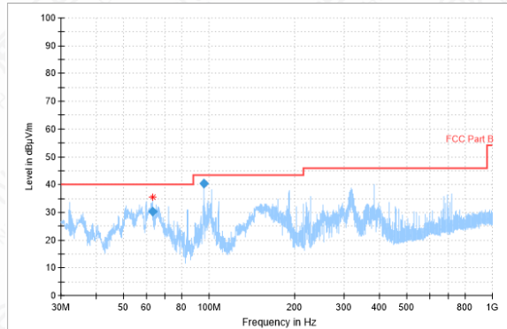
RSE-11N(40M)-CH9-30MHz-1GHz
