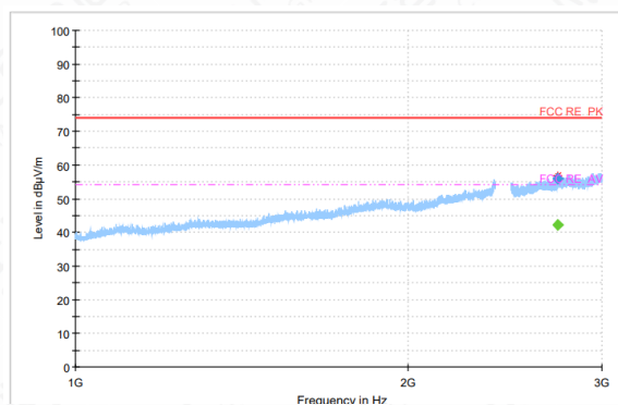
Bandedge: 2M Ch0
