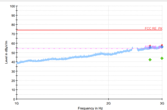
Radiated emission:2M Ch39, 1GHz~3GHz
