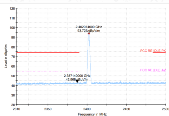
Bandedge: 2M Ch0
