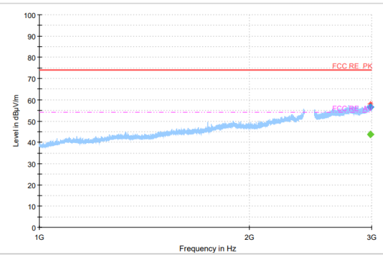
Bandedge:2M Ch0
