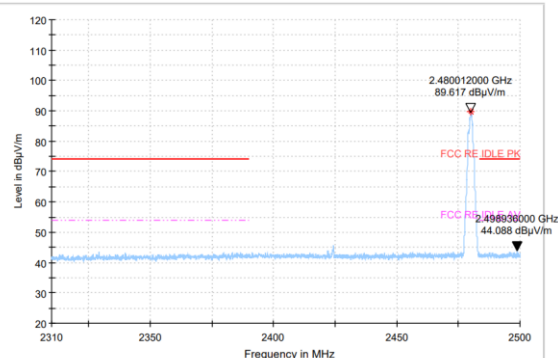
Bandedge: 2M Ch39
