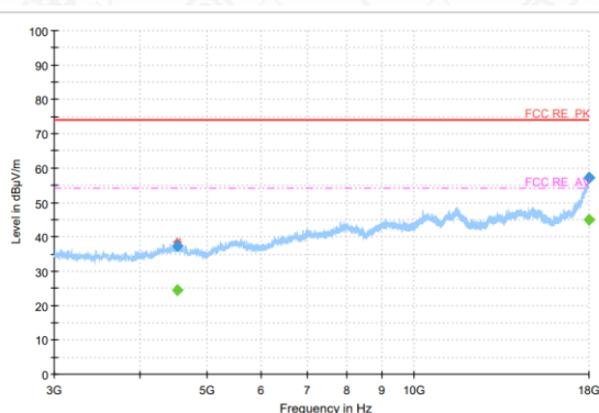
Radiated emission: 2M Ch0, 3GHz~18GHz
