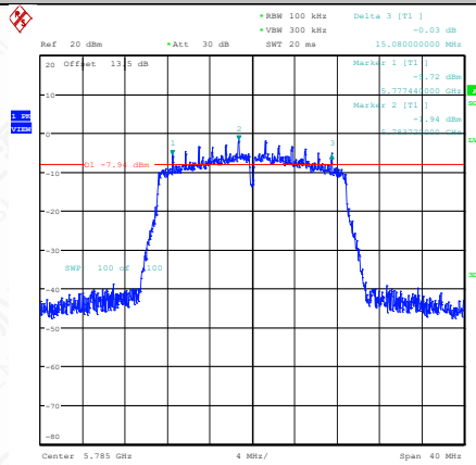
11N20SISO-Ant1-5785-PASS
