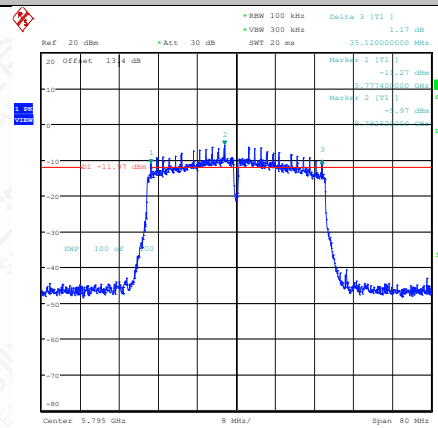
11N40SISO-Ant1-5795-PASS
