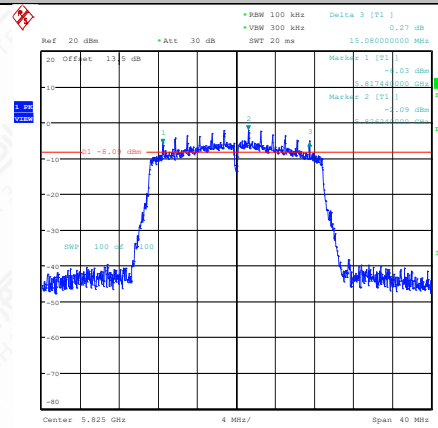
11N20SISO-Ant1-5825-PASS
