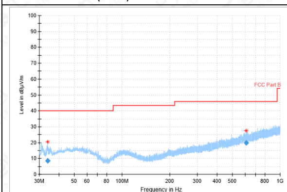
RSE-11N(40M)-CH134-30MHz-1GHz
