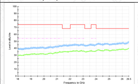
RSE-11N(40M)-CH134-18GHz-26.5GHz
