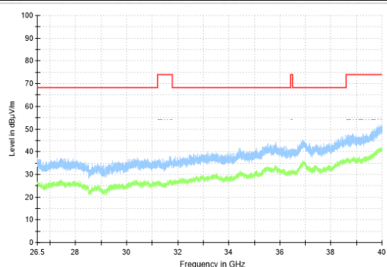
RSE-11N(20M)-CH140-26.5GHz-40GHz
