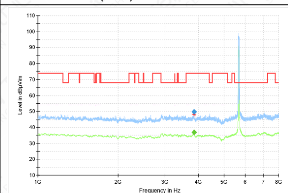
RSE-11N(40M)-CH134-1GHz-8GHz
