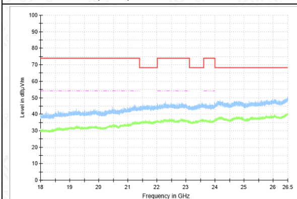
RSE-11N(40M)-CH54-18GHz-26.5GHz
