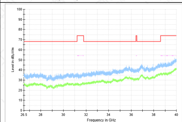
RSE-11N(40M)-CH54-26.5GHz-40GHz
