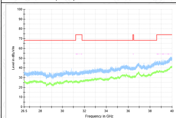
RSE-11N(40M)-CH134-26.5GHz-40GHz
