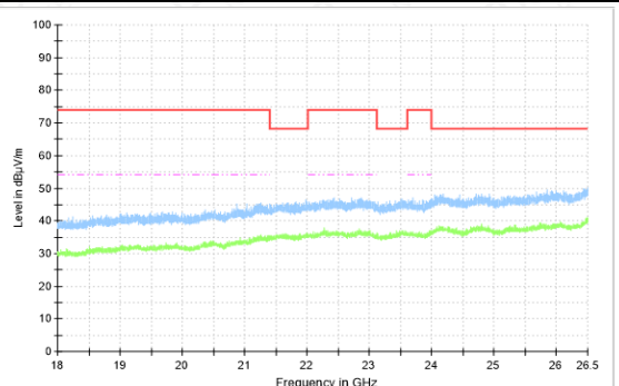
RSE-11N(20M)-CH140-18GHz-26.5GHz
