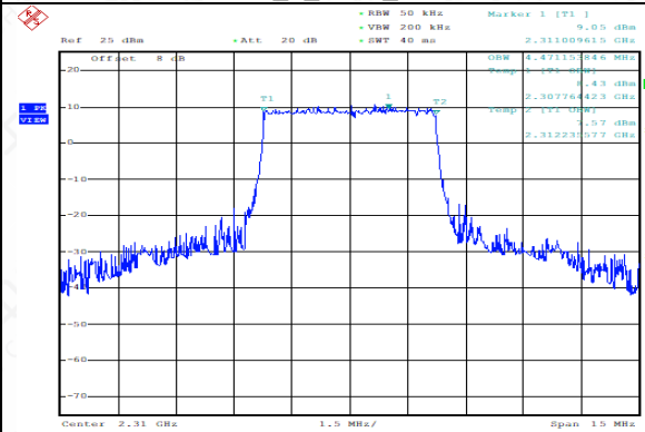
TDD40(2305-2315MHz)_Channel Mid_5_2310_Q16
