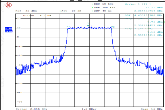
TDD40(2350-2360MHz)_Channel Mid_5_2355_Q16
