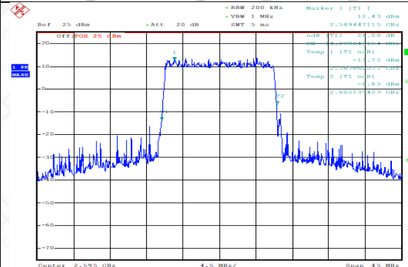
TDD38_Channel Mid_15MHz_2595MHz_Q16
