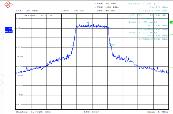
FDD04_Channel Mid_1.4MHz_1732.5MHz _Q16
