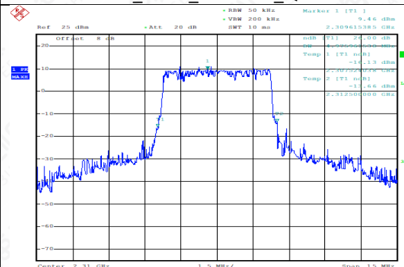
TDD40(2305-2315MHz)_Channel Mid_5MHz_2310MHz_Q16
