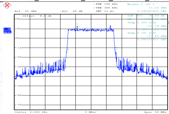
TDD41_Channel Mid_10MHz_2593MHz_Q16
