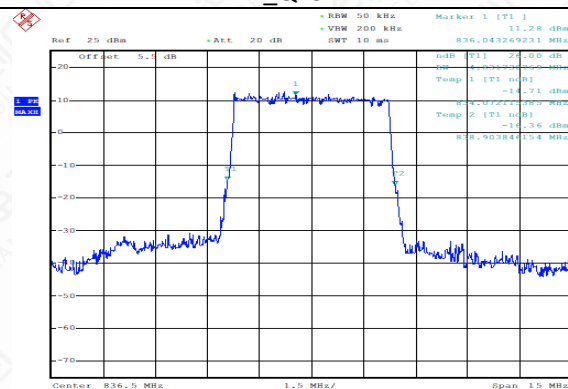
FDD26(PART 22)_Channel Mid_5MHz_836.5MHz _QPSK
