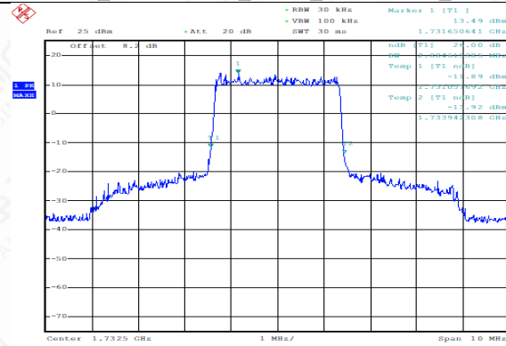
FDD04_Channel Mid_3MHz_1732.5MHz_QPSK
