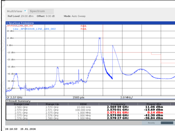
FDD07_Channel High_5MHz_QPSK_FullRB
