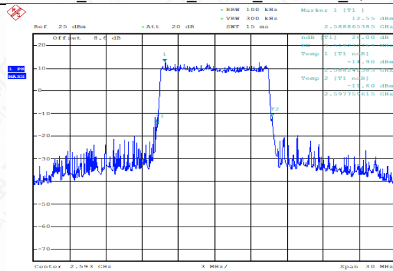
TDD41_Channel Mid_10MHz_2593MHz_QPSK
