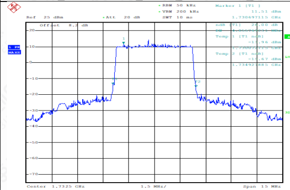
FDD04_Channel Mid_5MHz_1732.5MHz_Q16
