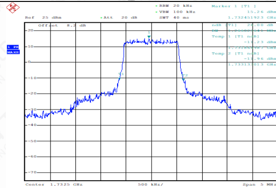
FDD04_Channel Mid_1.4MHz_1732.5MHz _QPSK
