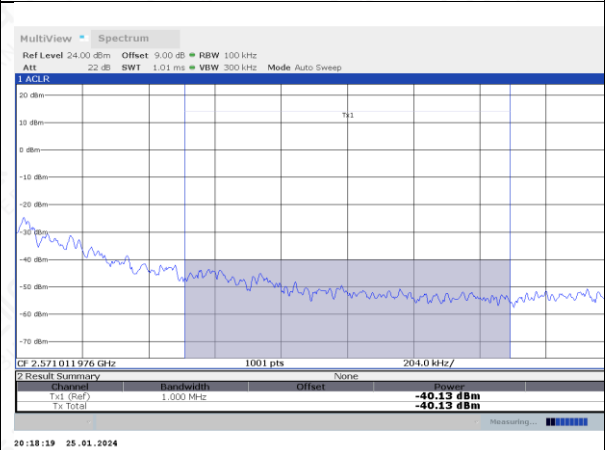
FDD07_Channel High_10MHz_QPSK_1RB_High
