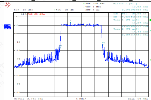
TDD38_Channel Mid_20MHz_2595MHz_Q16
