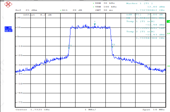
FDD04_Channel Mid_3MHz_1732.5MHz_Q16
