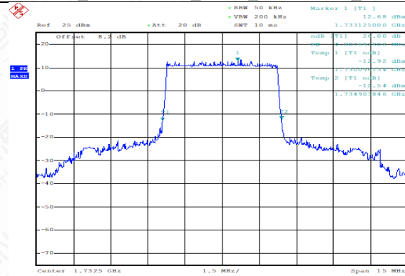
FDD04_Channel Mid_5MHz_1732.5MHz_QPSK
