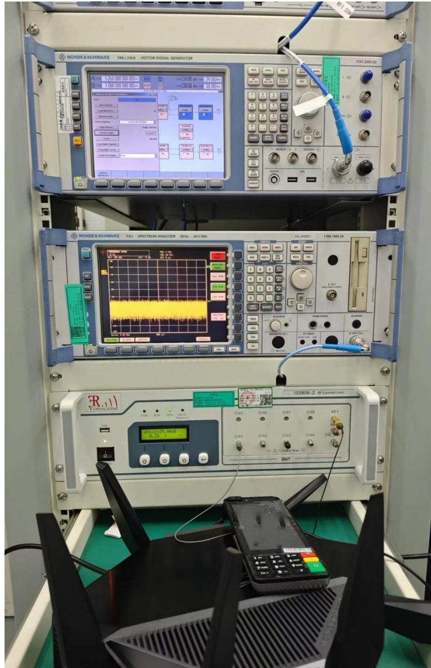
Figure: DFS Set-up Photo
