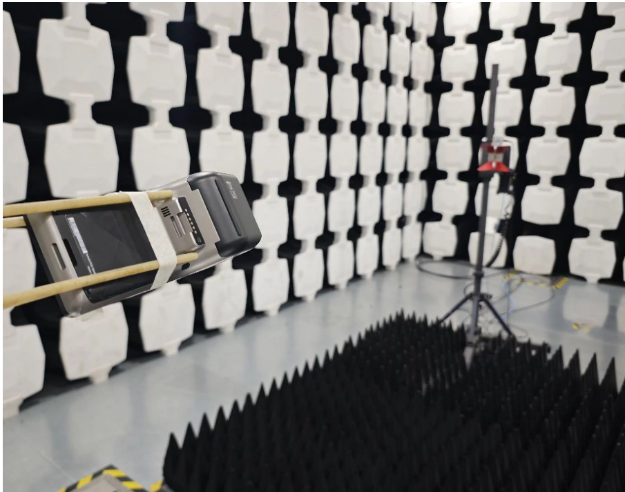
Description: Substitution Antenna for Radiated Emissions above 1GHz Test
