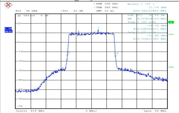
FDD26_90_MidRange_10MHz_819MHz 16QAM
