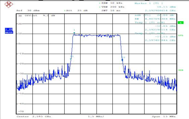
TDD38_MidRange_5MHz_2595MHz_16QAM
