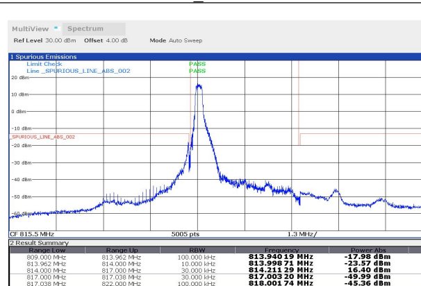
FDD26_90LowRange_3MHz_QPSK_1RB low
