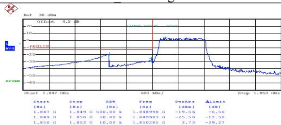
FDD02LowRange_1.4MHz_QPSK_FullRB_LowRange
