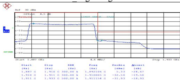
FDD02HighRange_20MHz_QPSK_FullRB_HighRange
