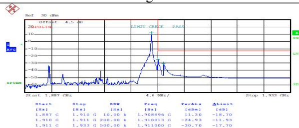
FDD02HighRange_20MHz_QPSK_1RB_HighRange
