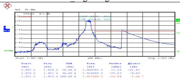
FDD02HighRange_1.4MHz_QPSK_1RB_HighRange
