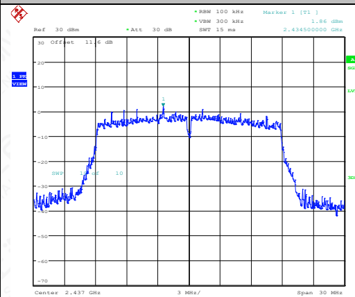
11N20ISO-Ant1-2437-0~Reference-PASS
