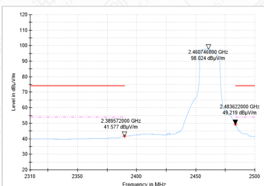
BANDEGE-11G-CH11-AV
