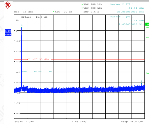
11G-Ant1-2462-1000~26500-PASS
