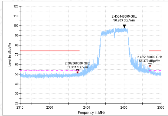
BANDEGE-11N(40M)-CH9-PK
