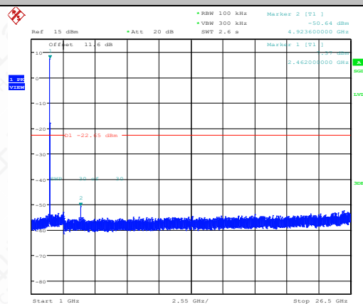
11B-Ant1-2462-1000~26500-PASS
