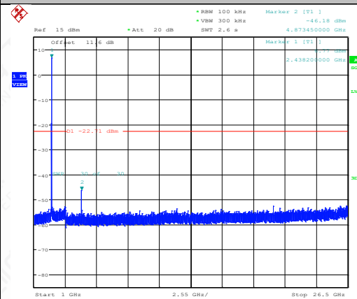
11B-Ant1-2437-1000~26500-PASS
