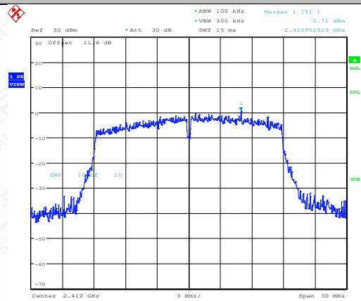
11N20ISO-Ant1-2412-0~Reference-PASS
