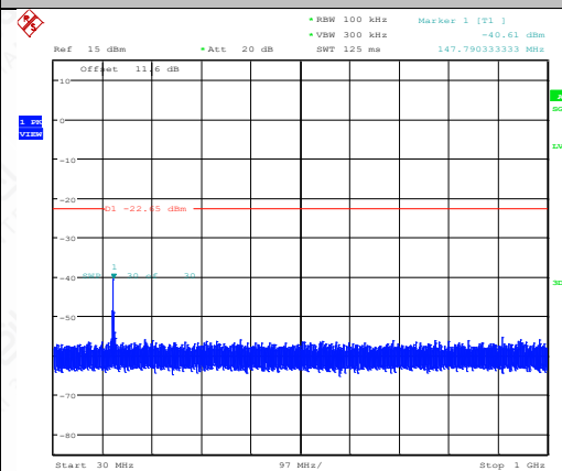
11B-Ant1-2462-30~1000-PASS
