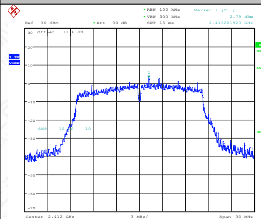
11G-Ant1-2412-0~Reference-PASS
