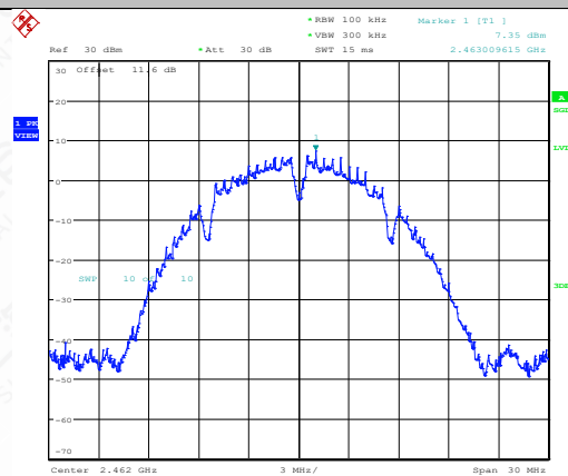
11B-Ant1-2462-0~Reference-PASS
