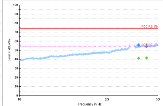
RSE-11G-CH6-1GHz-3GHz
