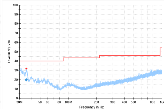
RSE-11G-CH6-30MHz-1GHz
