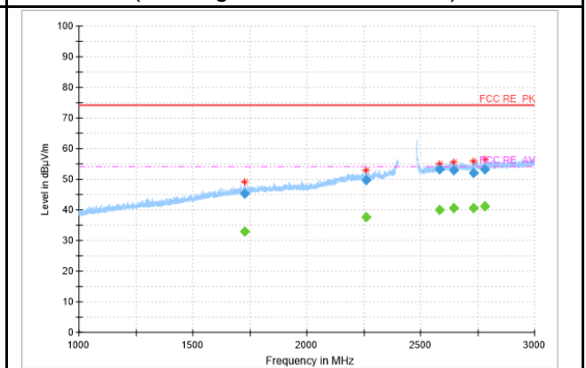
Radiated Spurious Emission (802.11g, Ch11, 1GHz~3GHz)
