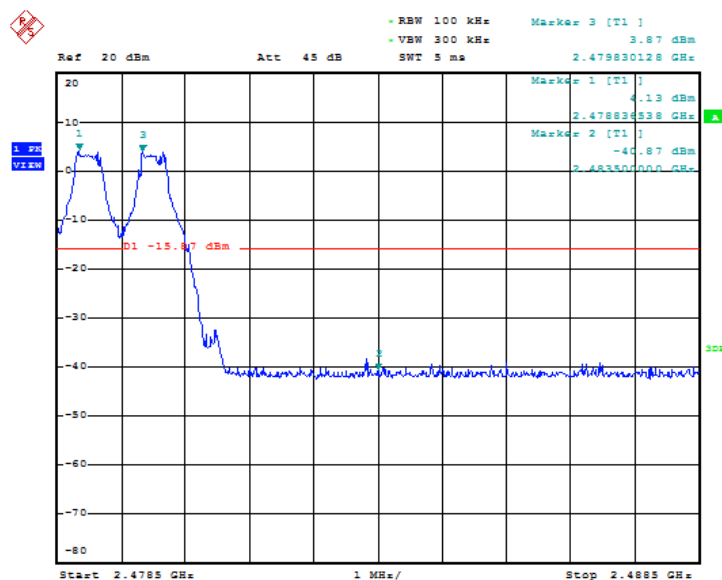
Fig.12 Frequency Band Edge: GFSK, Ch78, Hopping OFF
