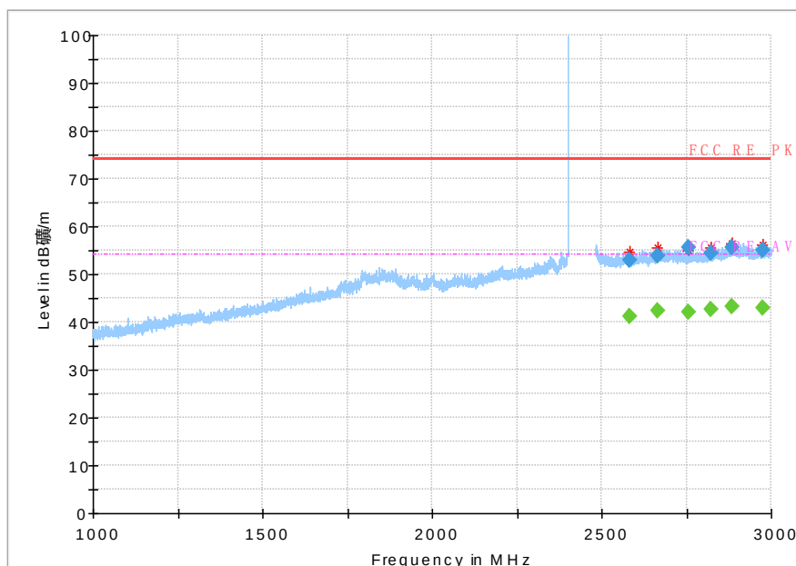
Fig.32 Radiated emission: GFSK, Ch0, 1GHz~3GHz
