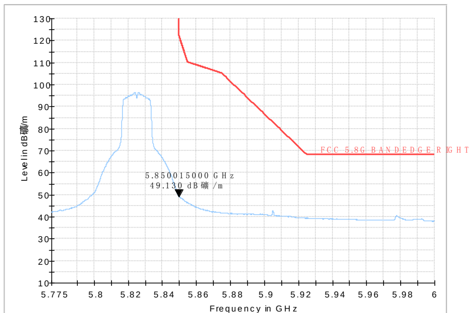
Fig. 43 Band Edges (802.11a, 5825MHz)
