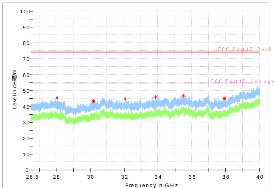
Fig. 35 Radiated emission: 802.11n, (802.11n-HT20, Ch165, 26.5 GHz - 40 GHz)
