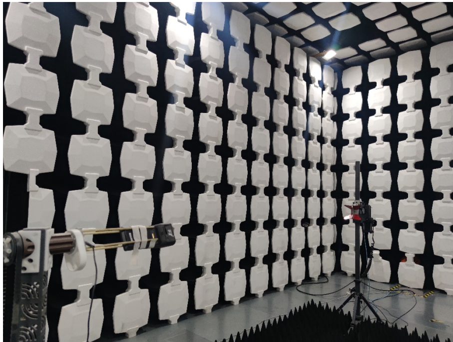
Description: Substitution Antenna for Radiated Emissions above1GHz Test
