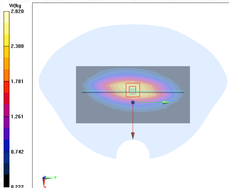
Figure A.2-1 System Check Head 750MHz
