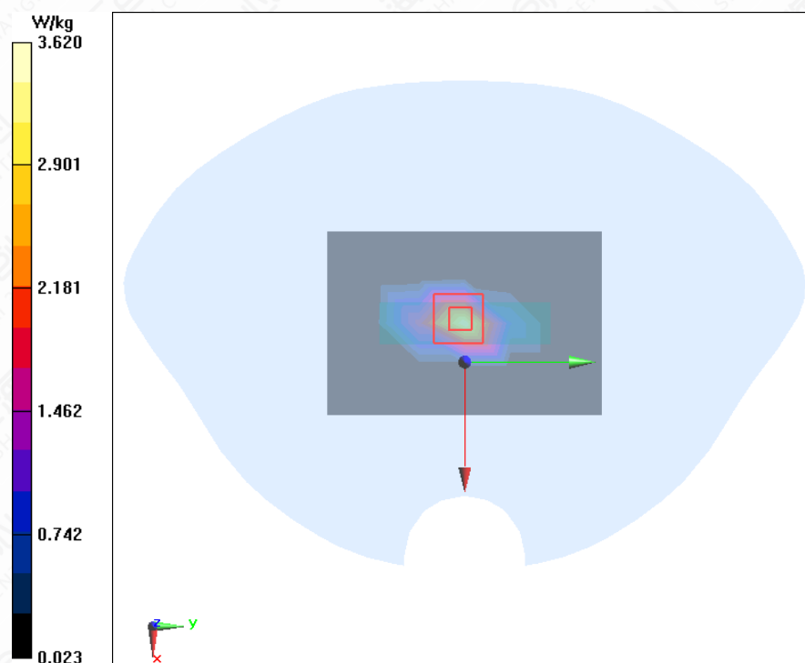
Figure A.1-8 LTE B66 20MHz 1RB 50offset Bottom Mode High 0mm
