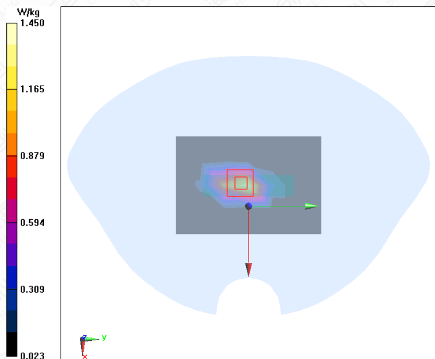
Figure A.1-7 LTE B66 20MHz 1RB 50offset Bottom Mode High 5mm
