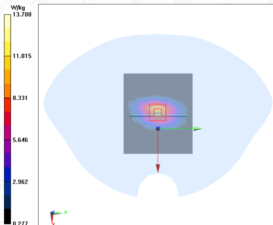
Figure A.2-3 System Check Head 1750MHz
