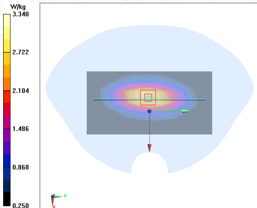
Figure A.2-2 System Check Head 835MHz
