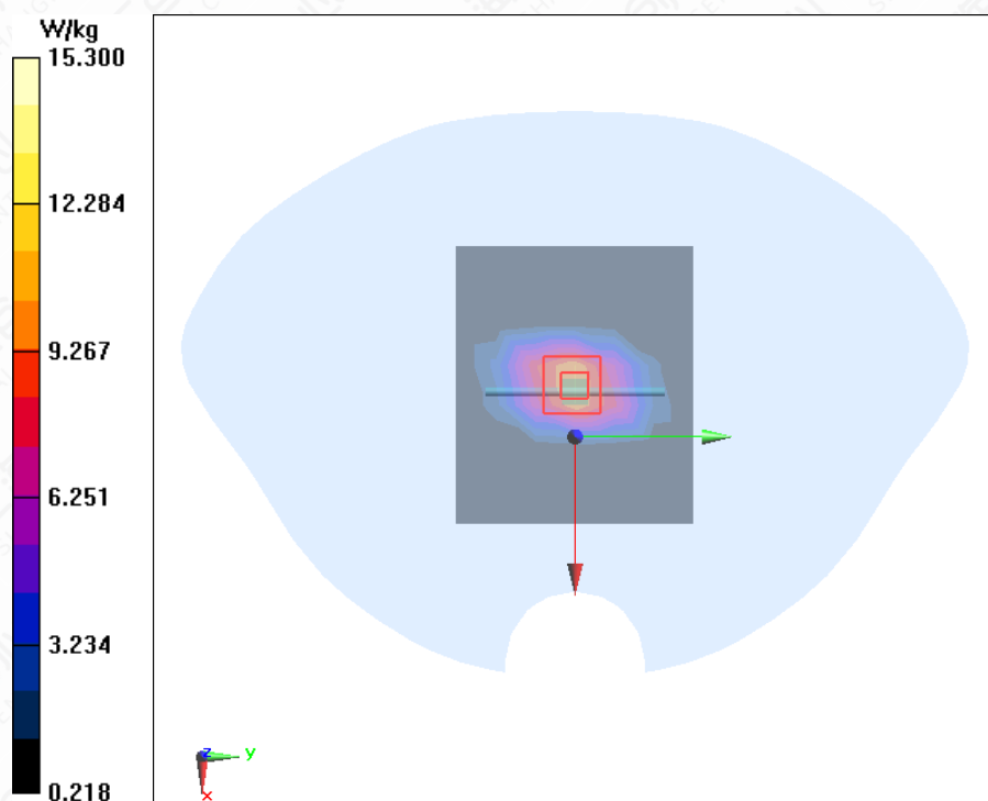
Figure A.2-4 System Check Head 1900MHz
