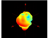
LTE7(Frequency=2660MHz)
