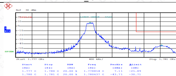
FDD66HighRange_1.4MHz_QPSK_OneRB _low
