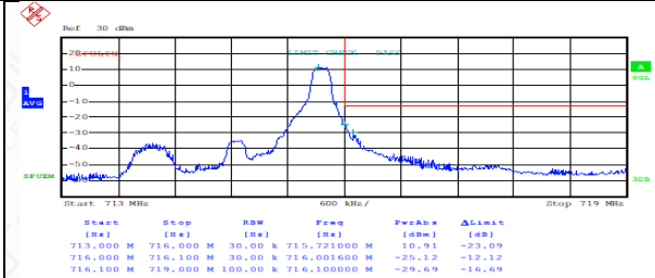
FDD12HighRange_1.4MHz_QPSK_OneRB _high
