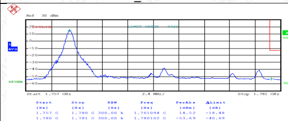
FDD66HighRange_20MHz_QPSK_OneRB _low
