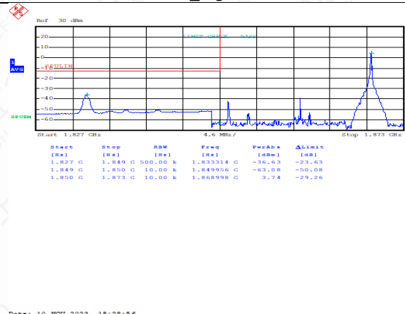
FDD25LowRange_20MHz_QPSK_FullRB _Low
