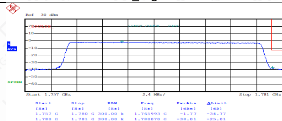
FDD66HighRange_20MHz_QPSK_FullRB _High
