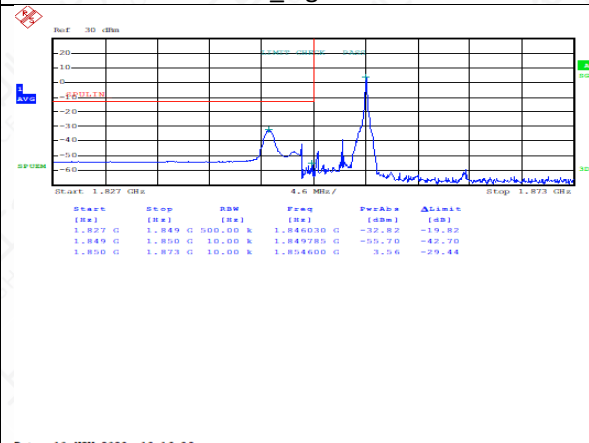
FDD25LowRange_1.4MHz_QPSK_FullRB _Low
