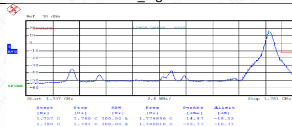
FDD66HighRange_20MHz_QPSK_OneRB _high
