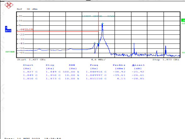
FDD25LowRange_1.4MHz_QPSK_OneRB _high
