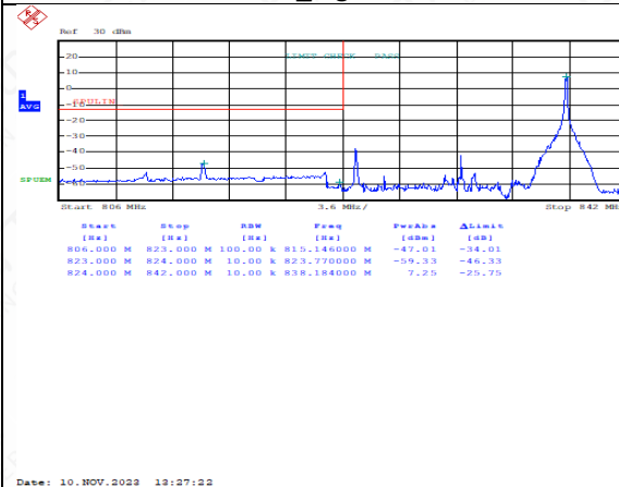
FDD26Part22LowRange_15MHz_QPSK_FullRB _Low
