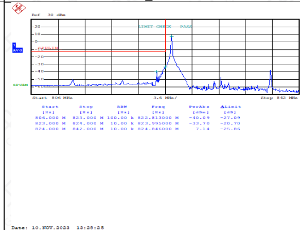
FDD26Part22HighRange_15MHz_QPSK_OneRB _high
