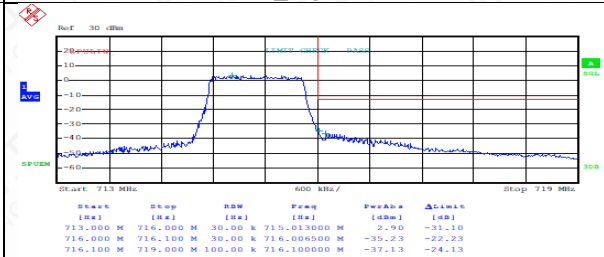
FDD12HighRange_1.4MHz_QPSK_FullRB _high
