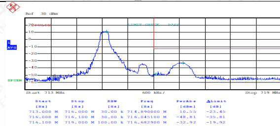
FDD12HighRange_1.4MHz_QPSK_OneRB _low
