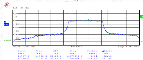
FDD66HighRange_1.4MHz_QPSK_FullRB _High
