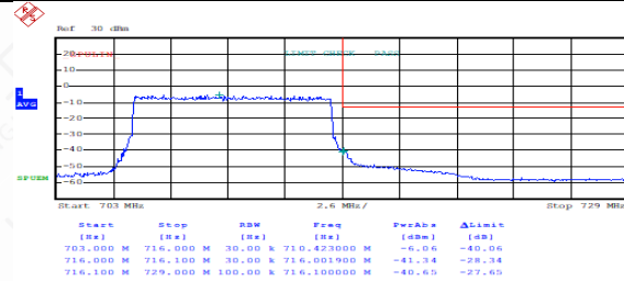
FDD12HighRange_10MHz_QPSK_FullRB _high
