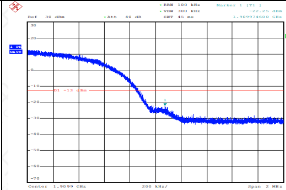
WCDMA_OB2,1907.4MHz_BandEdge
