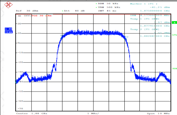
Channel 9400-Occupied Bandwidth (99%)
