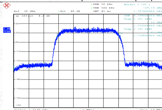
Channel 1313-Occupied Bandwidth (99%)
