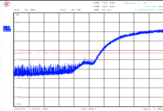
WCDMA_OB2,1852.6MHz_BandEdge
