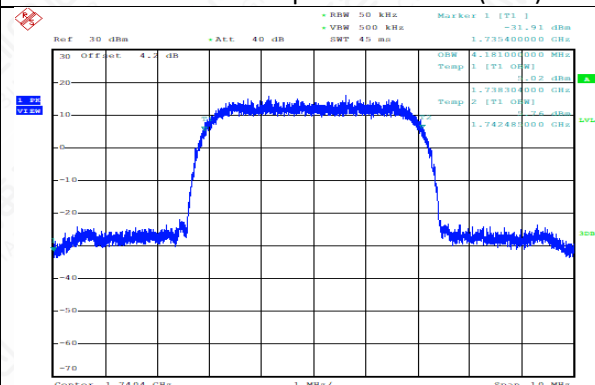
Channel 1450-Occupied Bandwidth (99%)
