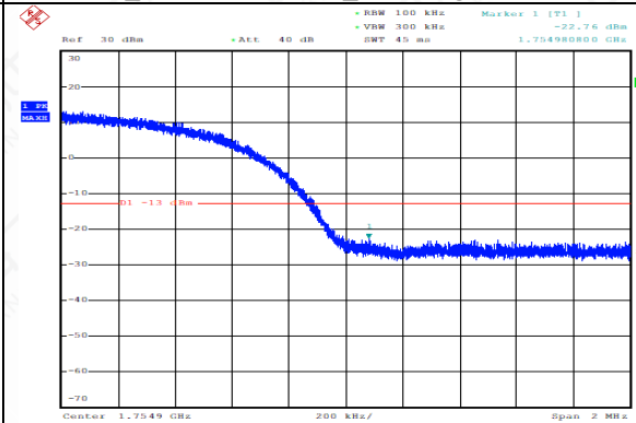
WCDMA_OB4,1752.4MHz_BandEdge
