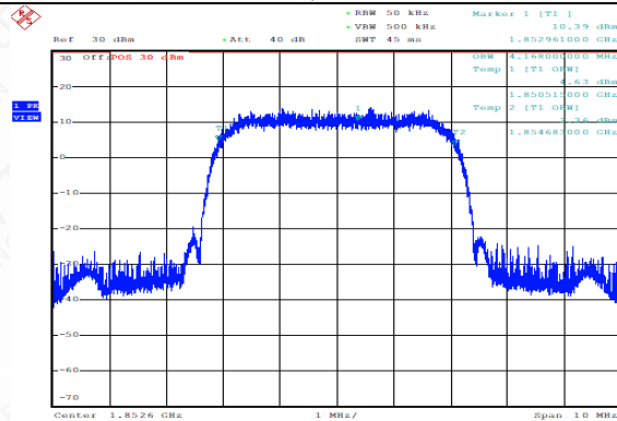
Channel 9263-Occupied Bandwidth (99%)
