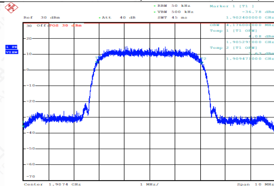
Channel 9537-Occupied Bandwidth (99%)
