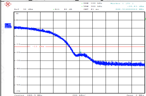
WCDMA_OB5,846.4MHz_BandEdge
