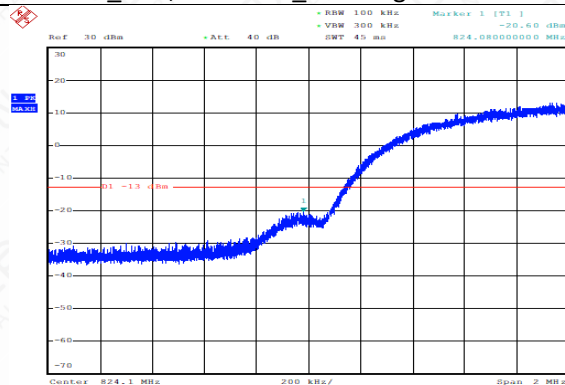
WCDMA_OB5,826.6MHz_BandEdge
