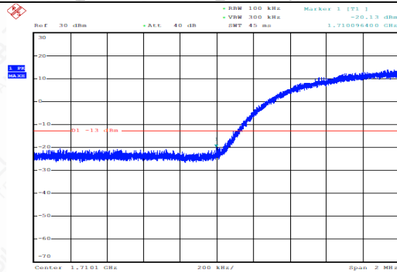
WCDMA_OB4,1712.6MHz_BandEdge
