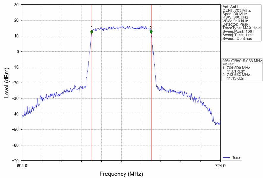
Band17_10MHz_16QAM_LCH_709MHz_RB_50_0_NTNV
