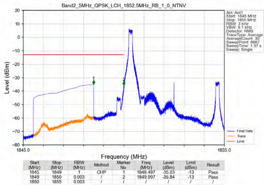
Band2_5MHz_QPSK_LCH_1852.5MHz_RB_1_0_NTNV
