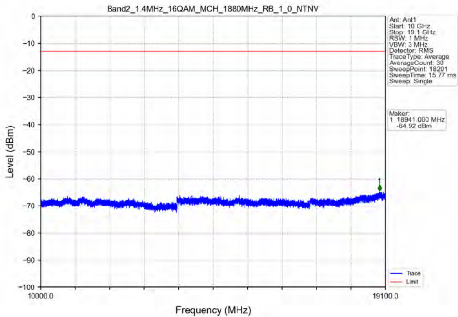
Band2_1.4MHz_16QAM_MCH_1880MHz_RB_1_0_NTNV
