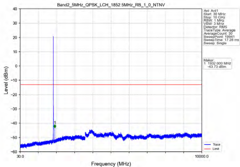
Band2_5MHz_QPSK_LCH_1852.5MHz_RB_1_0_NTNV
