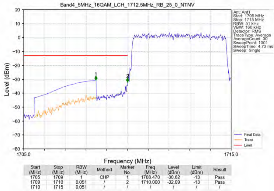
Band4_5MHz_16QAM_LCH_1712.5MHz_RB_25_0_NTNV
