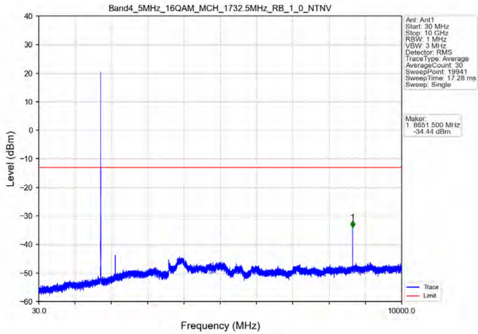
Band4_5MHz_16QAM_MCH_1732.5MHz_RB_1_0_NTNV
