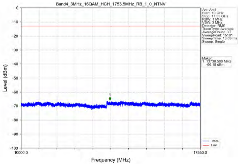
Band4_3MHz_16QAM_HCH_1753.5MHz_RB_1_0_NTNV
