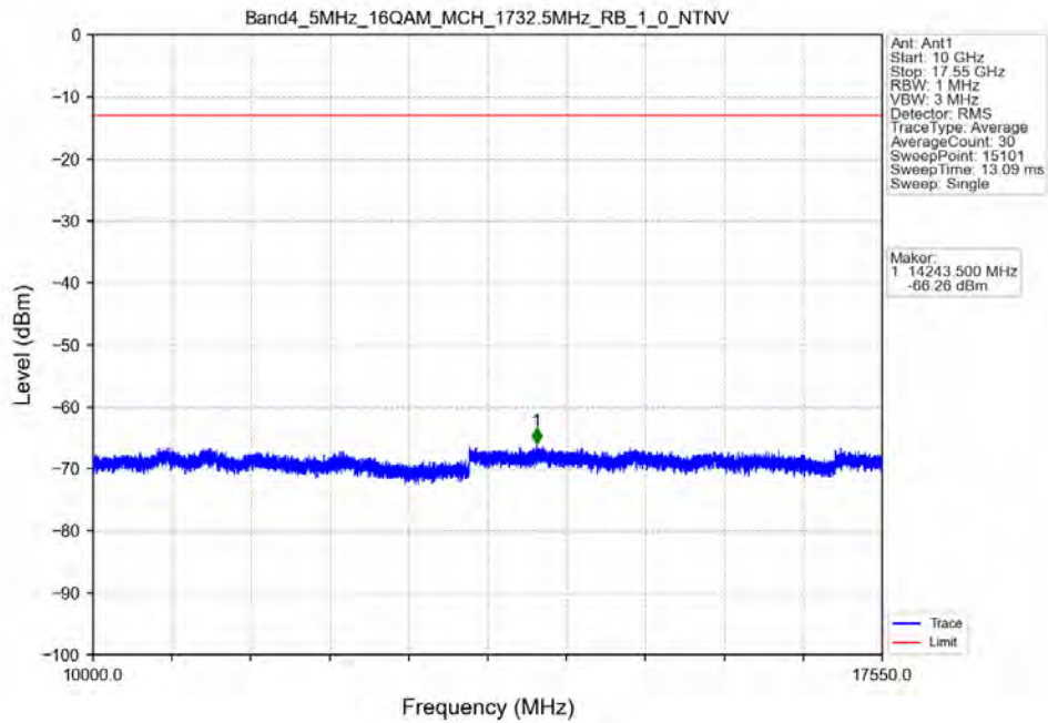
Band4_5MHz_16QAM_MCH_1732.5MHz_RB_1_0_NTNV
