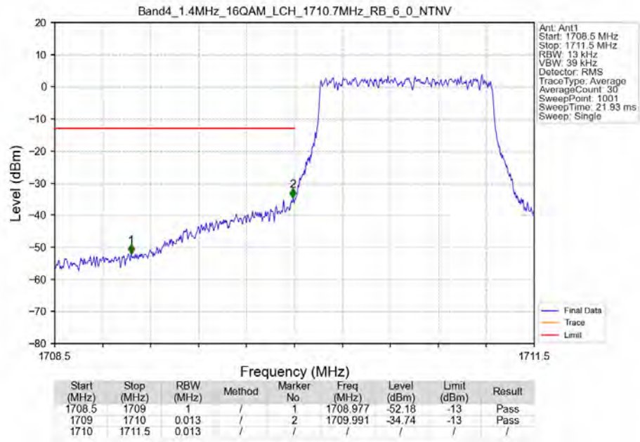
Band4_1.4MHz_16QAM_LCH_1710.7MHz_RB_6_0_NTNV
