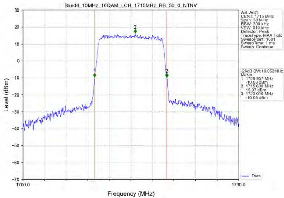
Band4_10MHz_16QAM_LCH_1715MHz_RB_50_0_NTNV
