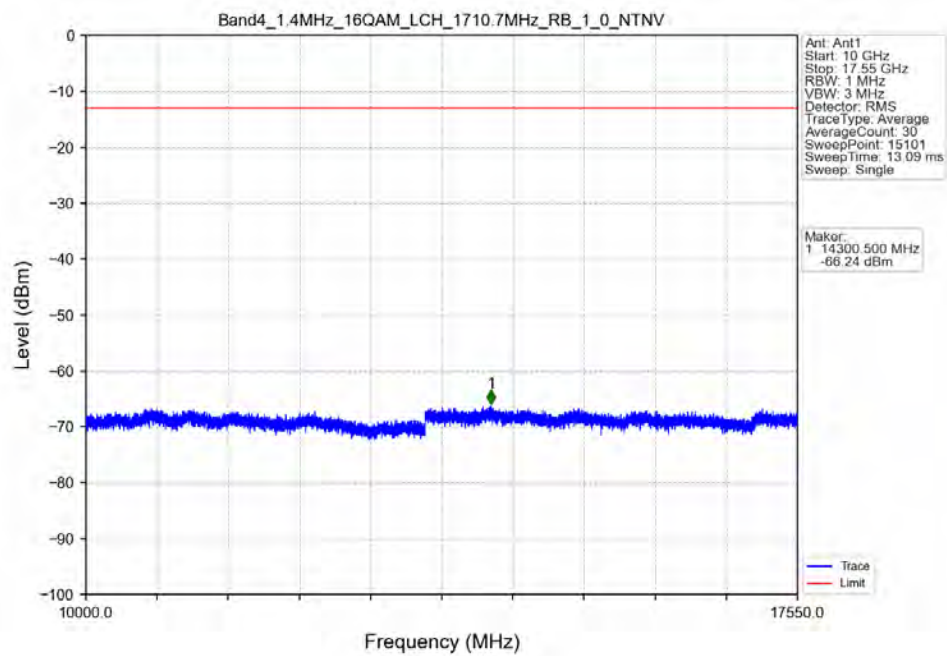
Band4_1.4MHz_16QAM_LCH_1710.7MHz_RB_1_0_NTNV
