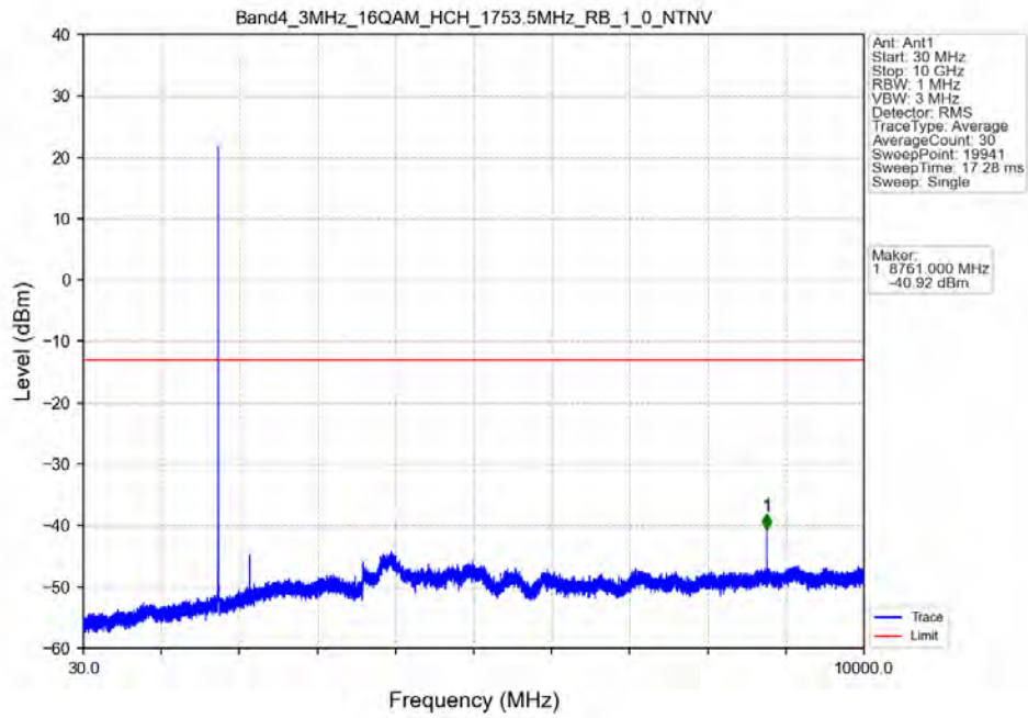
Band4_3MHz_16QAM_HCH_1753.5MHz_RB_1_0_NTNV
