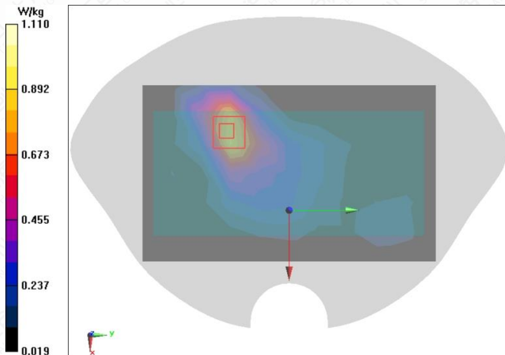
Figure A.1-13 LTE B4 20MHz 1RB 50offset Front Side Mode High 5mm
