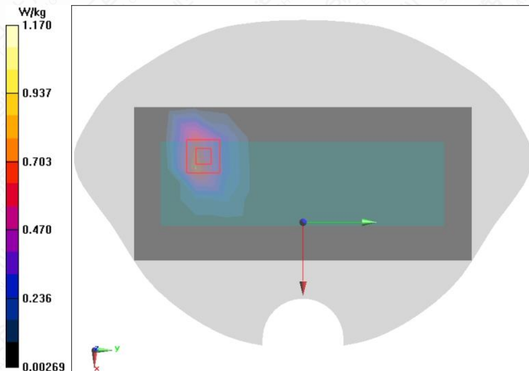
Figure A.1-23 LTE B41 20MHz 1RB 50offset Right Side Mode Low 5mm
