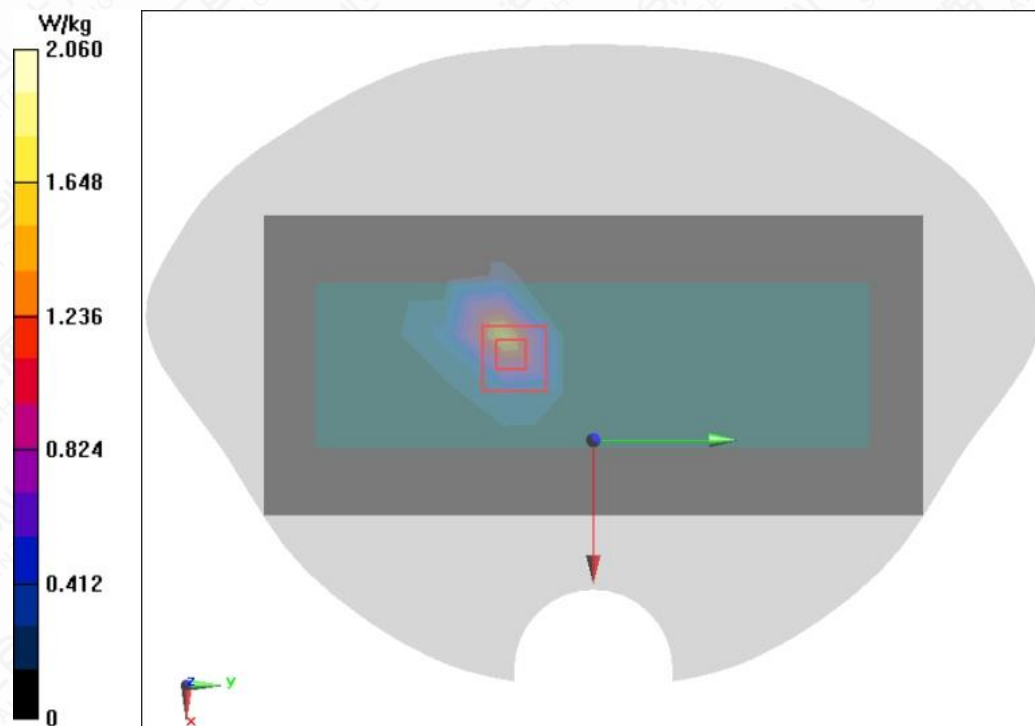
Figure A.1-34 Wi-Fi 5G 802.11a Right Side Mode Low 0mm
