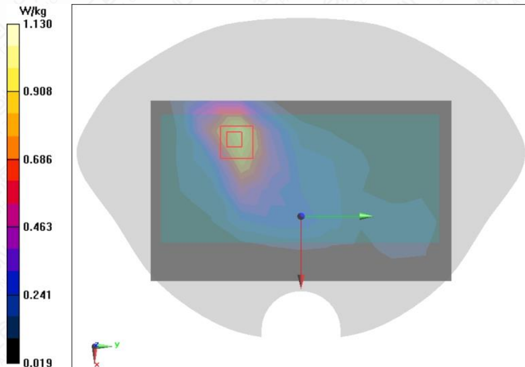
Figure A.1-5 WCDMA Band II RMC Front Side Mode Middle 5mm
