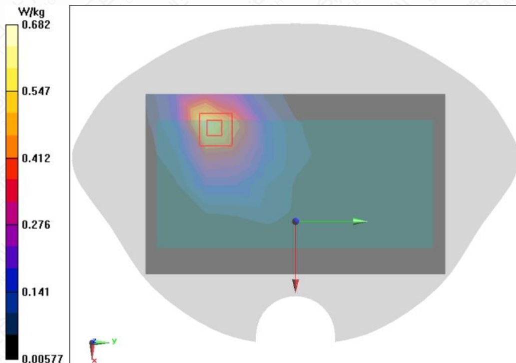
Figure A.1-19 LTE B40 20MHz 1RB 50offset Front Side Mode Middle 5mm
