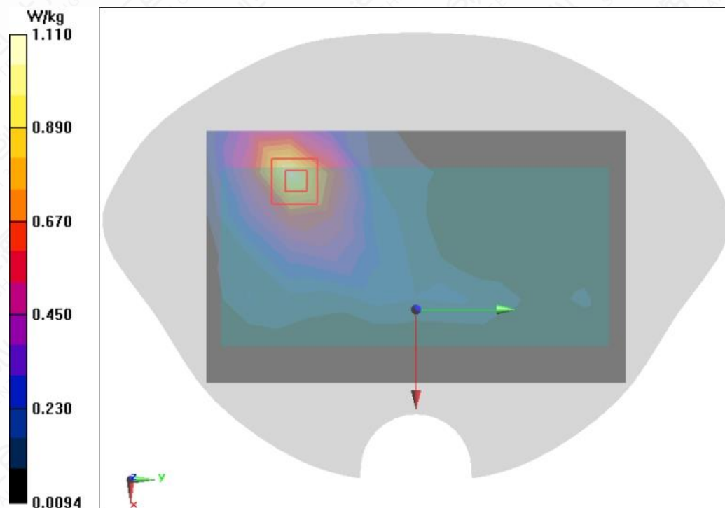
Figure A.1-15 LTE B7 20MHz 1RB 50offset Front Side Mode Low 5mm
