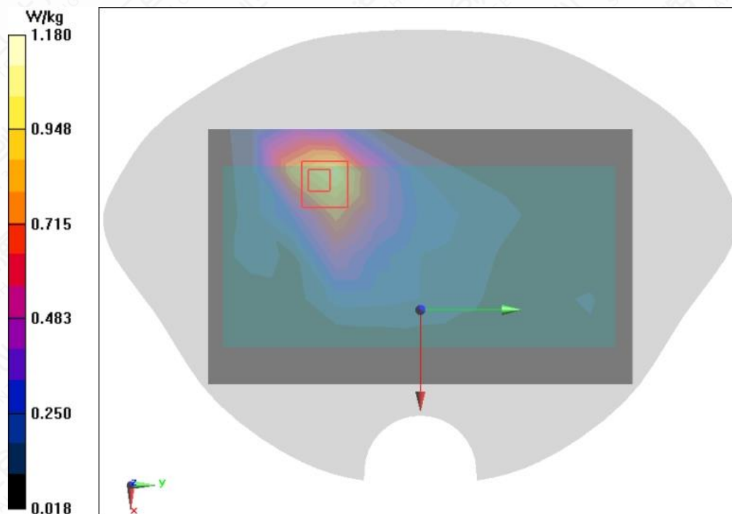
Figure A.1-11 LTE B2 20MHz 1RB 50offset Front Side Mode High 5mm
