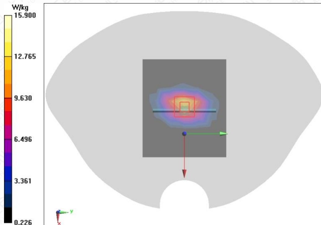
Figure A.2-6 System Check 1900MHz
