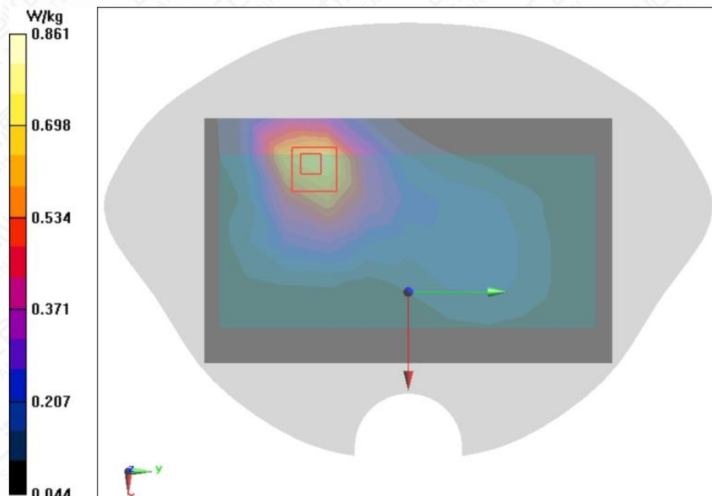
Figure A.1-1 GSM850 GPRS 4TS Front Side Mode Low 5mm
