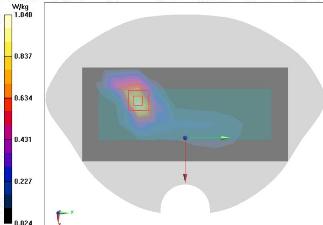
Figure A.1-17 LTE B26 15MHz 1RB 0offset Right Side Mode High 5mm
