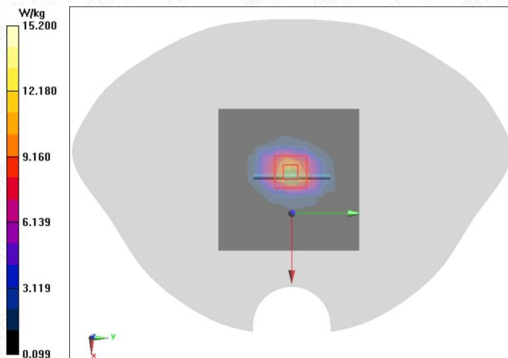
Figure A.2-8 System Check 2450MHz
