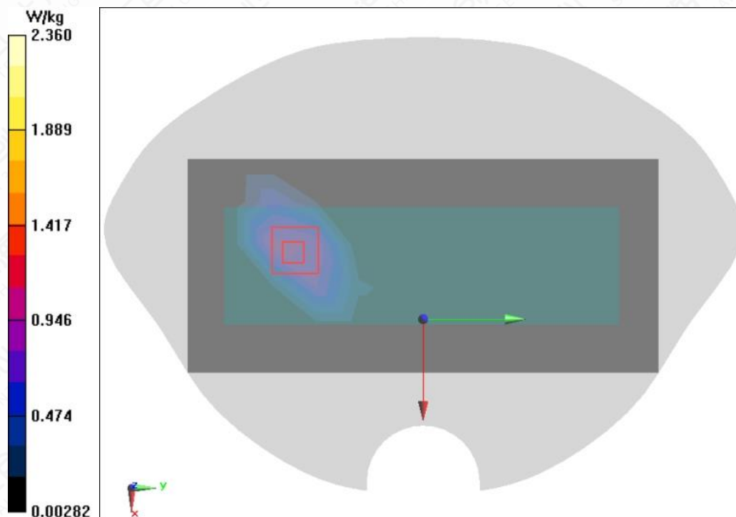
Figure A.1-24 LTE B41 20MHz 1RB 50offset Right Side Mode Middle 0mm
