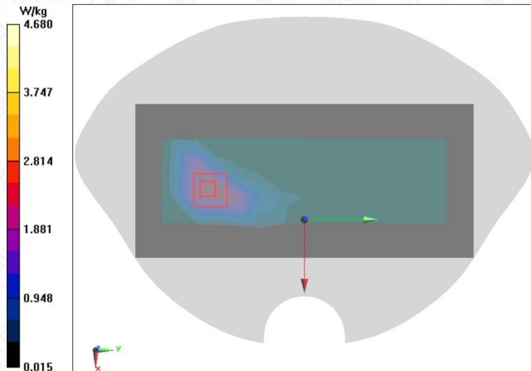
Figure A.1-8 WCDMA Band IV RMC Right Side Mode Middle 0mm
