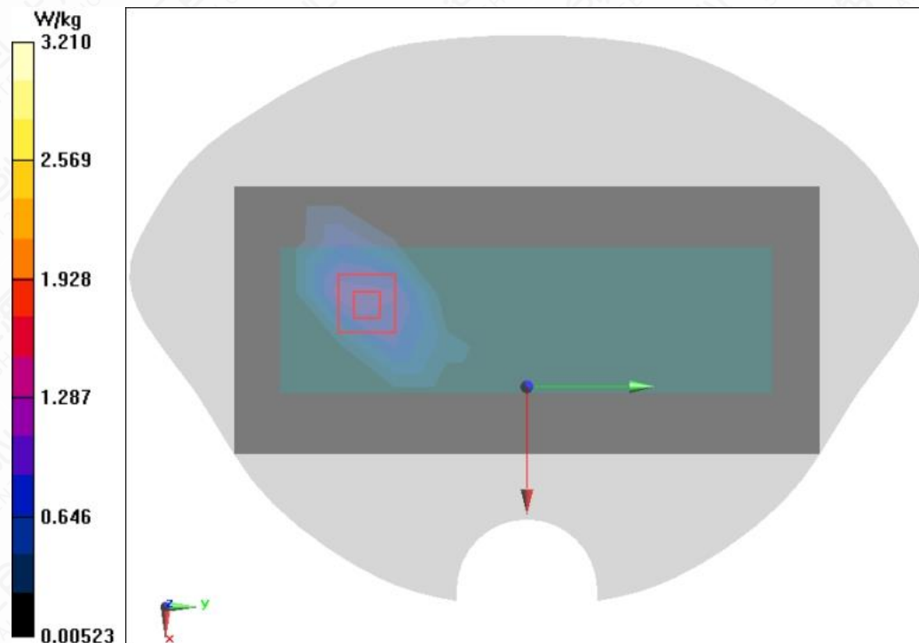
Figure A.1-16 LTE B7 20MHz 1RB 50offset Right Side Mode Middle 0mm
