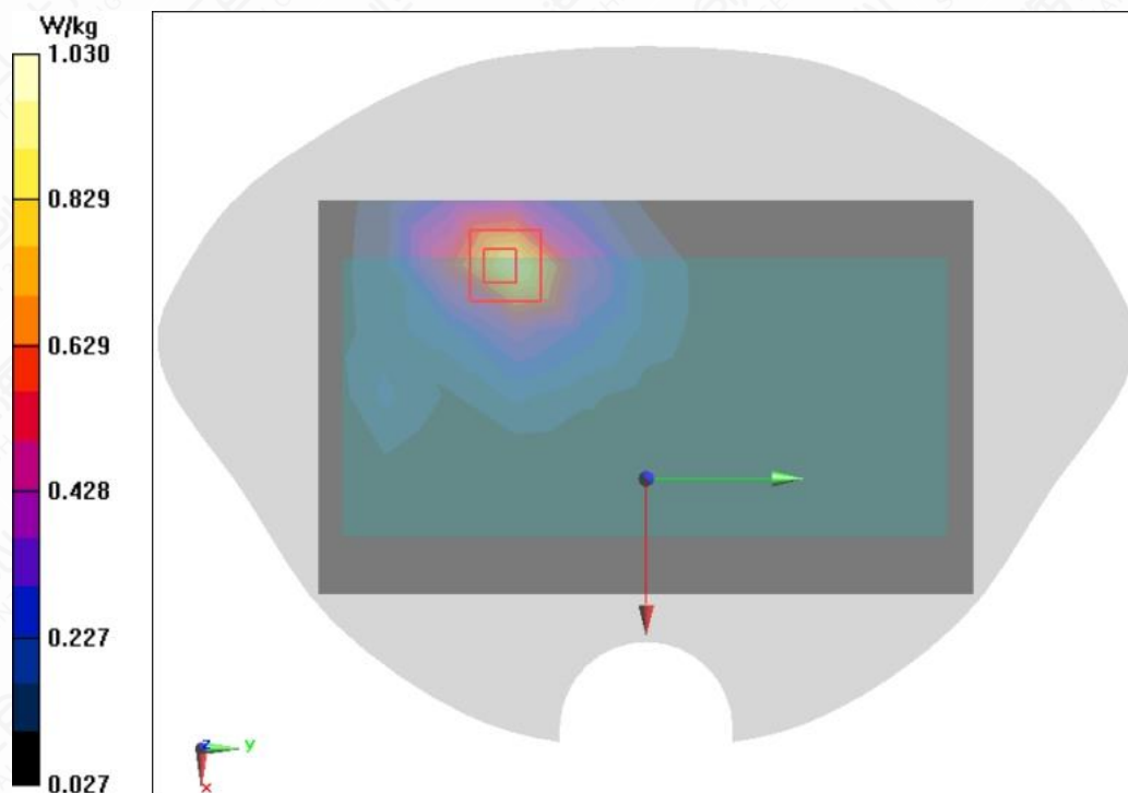
Figure A.1-10 WCDMA Band V RMC Front Side Mode Middle 0mm
