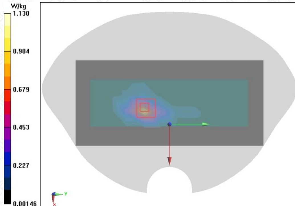
Figure A.1-26 Wi-Fi 2.4G 802.11b Right Side Mode Middle 0mm
