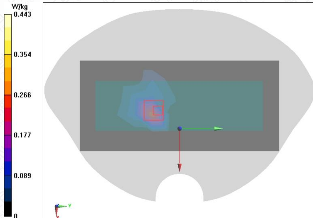
Figure A.1-27 Wi-Fi 5G 802.11a Right Side Mode Low 5mm
