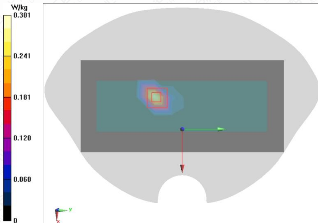
Figure A.1-36 BT DH5 Right Side Mode High 0mm
