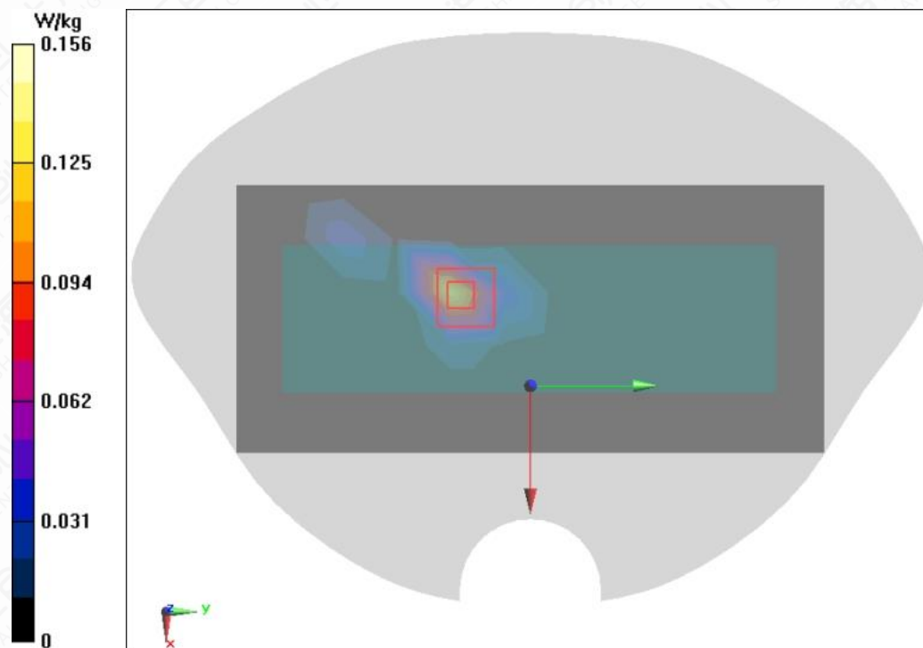
Figure A.1-35 BT DH5 Right Side Mode High 5mm
