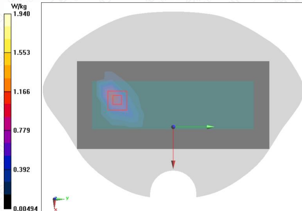
Figure A.1-20 LTE B40 20MHz 1RB 50offset Right Side Mode Middle 0mm
