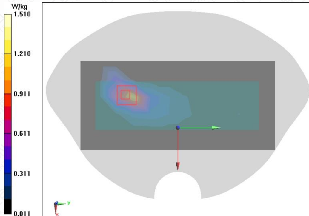
Figure A.1-3 GSM1900 GPRS 4TS Right Side Mode High 5mm
