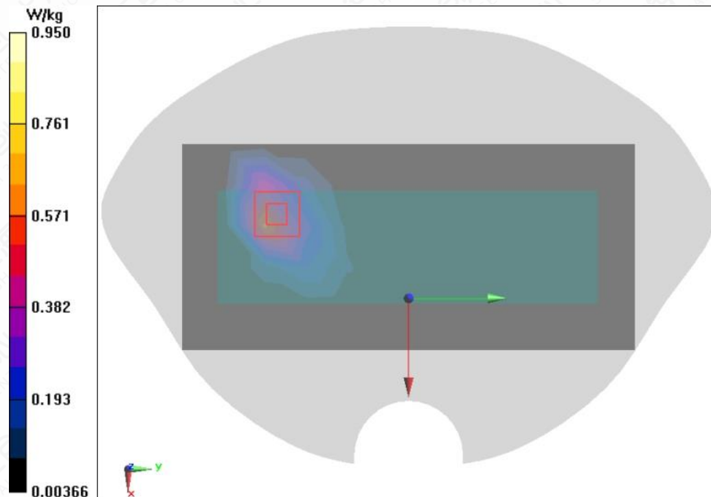
Figure A.1-21 LTE B40 20MHz 1RB 50offset Right Side Mode Middle 5mm
