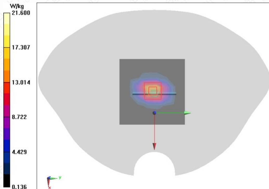
Figure A.2-7 System Check 2300MHz
