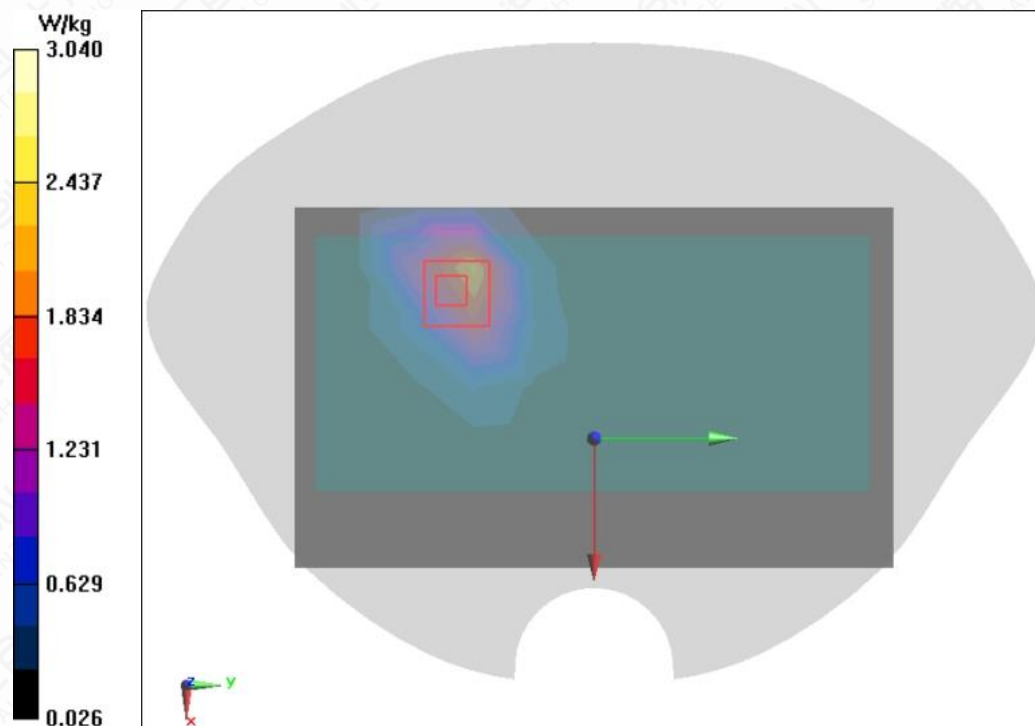
Figure A.1-6 WCDMA Band II RMC Front Side Mode Middle 0mm
