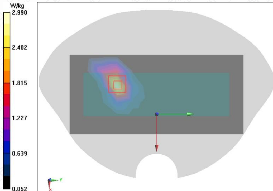
Figure A.1-18 LTE B26 15MHz 36RB 0offset Right Side Mode Middle 0mm
