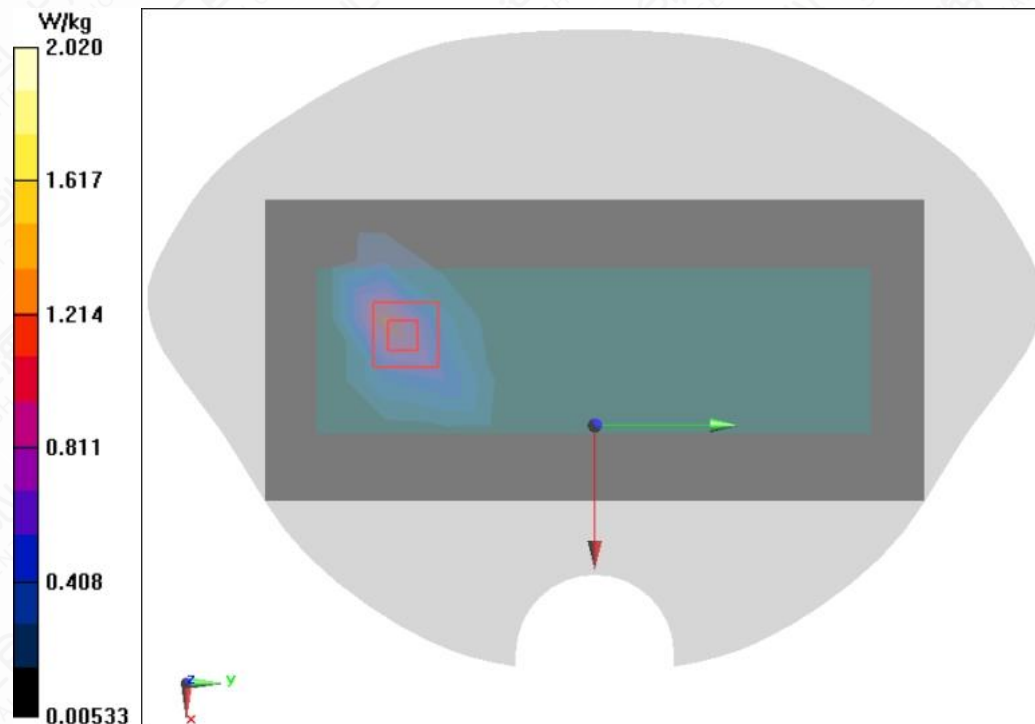
Figure A.1-22 LTE B40 20MHz 1RB 50offset Right Side Mode Middle 0mm
