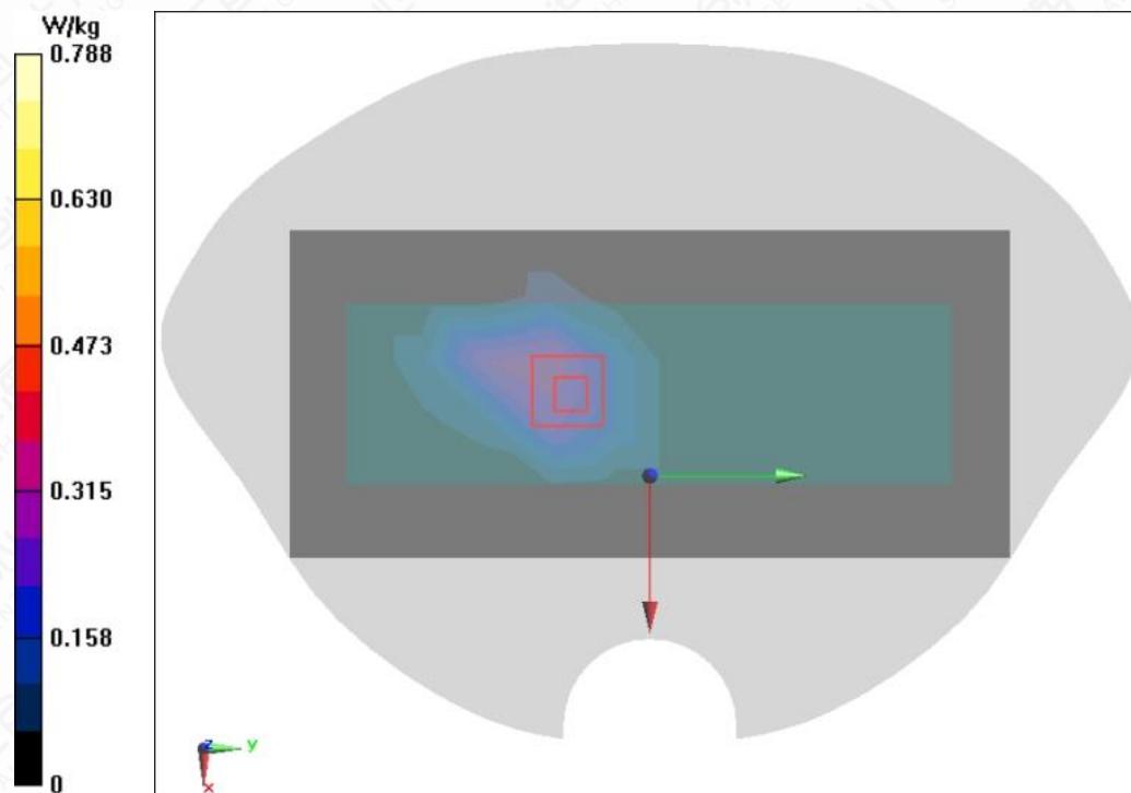
Figure A.1-33 Wi-Fi 5G 802.11a Right Side Mode Low 5mm
