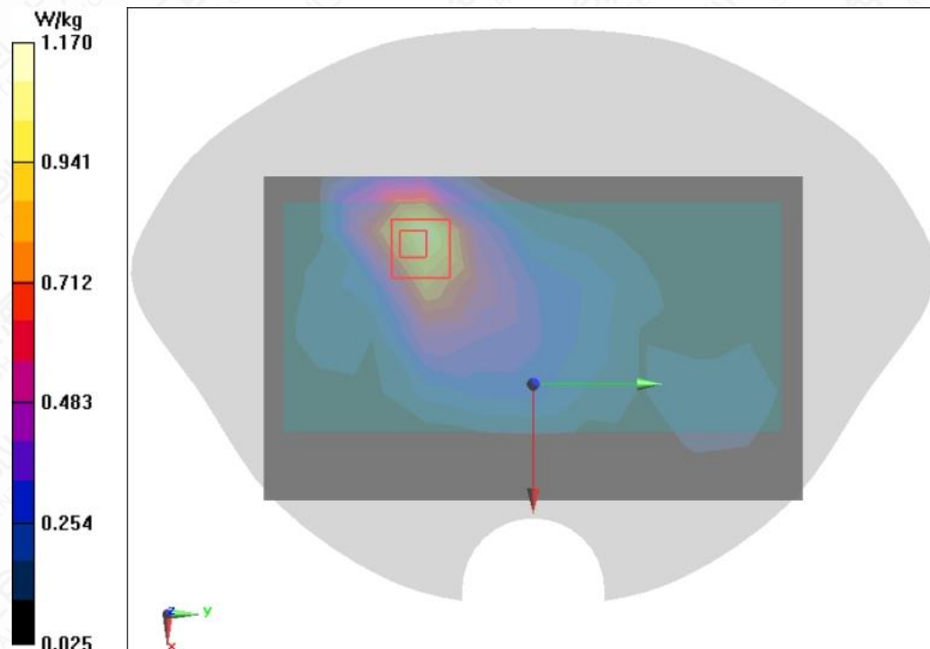
Figure A.1-7 WCDMA Band IV RMC Front Side Mode Middle 5mm
