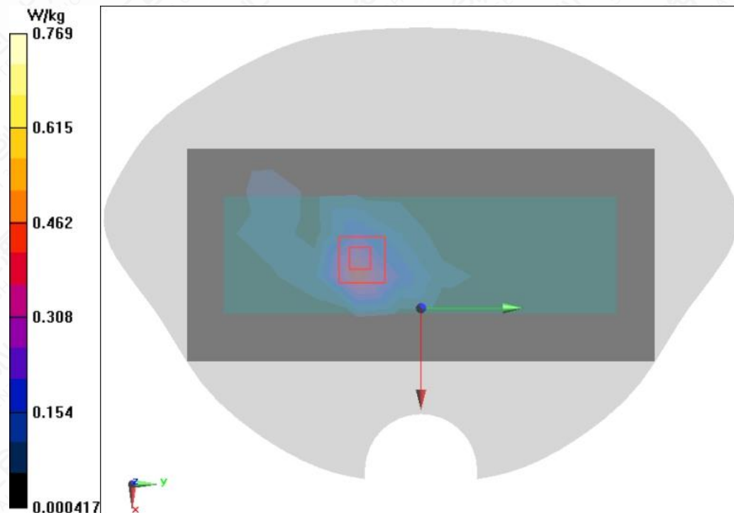
Figure A.1-25 Wi-Fi 2.4G 802.11b Right Side Mode Middle 5mm
