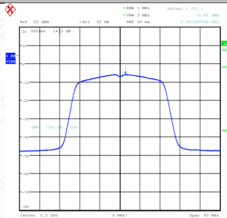
11N20SISO-Ant1-5500-PASS
