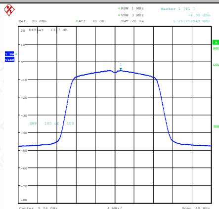
11AC20SISO-Ant1-5260-PASS
