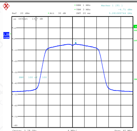
11AC20SISO-Ant1-5280-PASS
