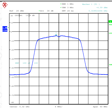
11N20SISO-Ant1-5320-PASS
