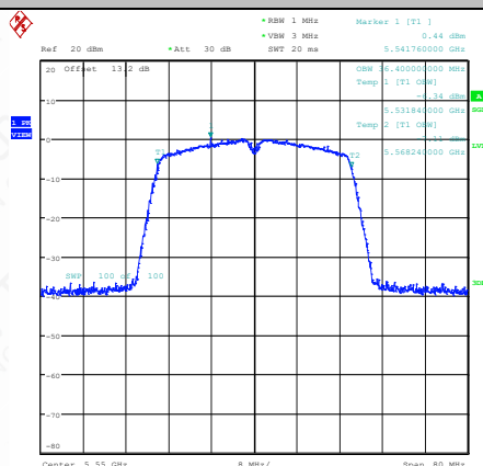
11AC40SISO-Ant1-5550
