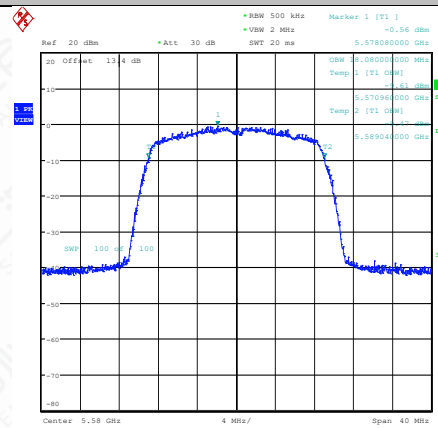
11AC20SISO-Ant1-5580
