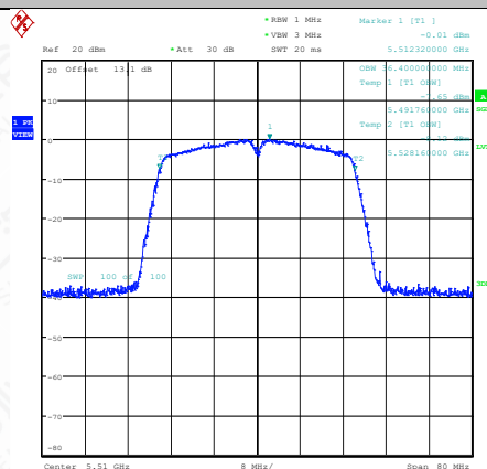
11AC40SISO-Ant1-5510
