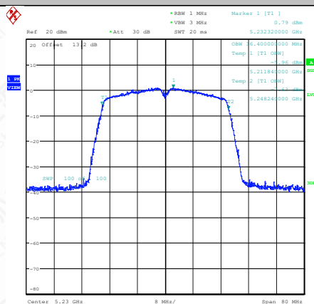
11AC40SISO-Ant1-5230
