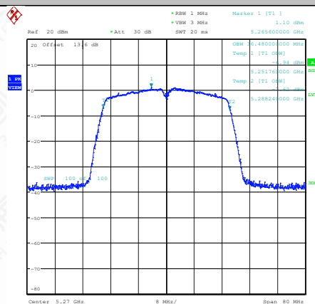
11AC40SISO-Ant1-5270
