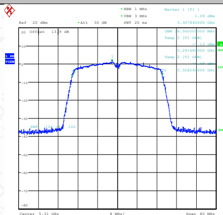
11AC40SISO-Ant1-5310
