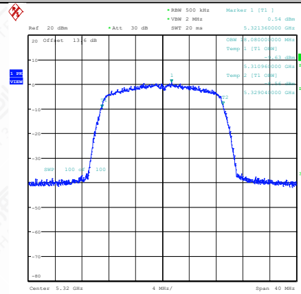
11AC20SISO-Ant1-5320
