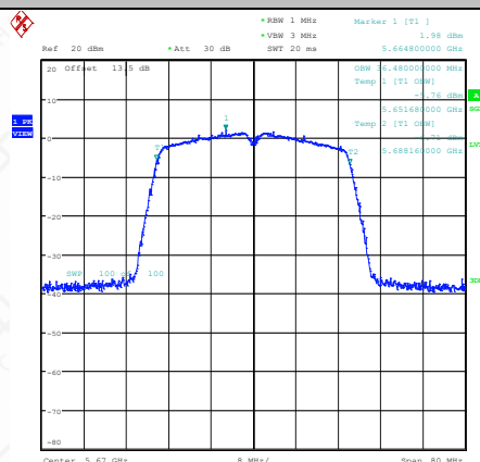
11AC40SISO-Ant1-5670
