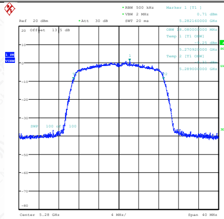
11AC20SISO-Ant1-5280
