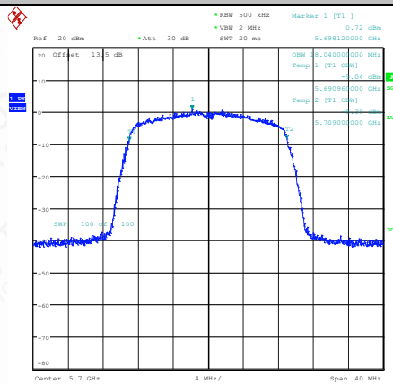
11AC20SISO-Ant1-5700
