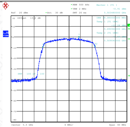
11AC20SISO-Ant1-5500
