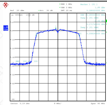
11AC40SISO-Ant1-5190
