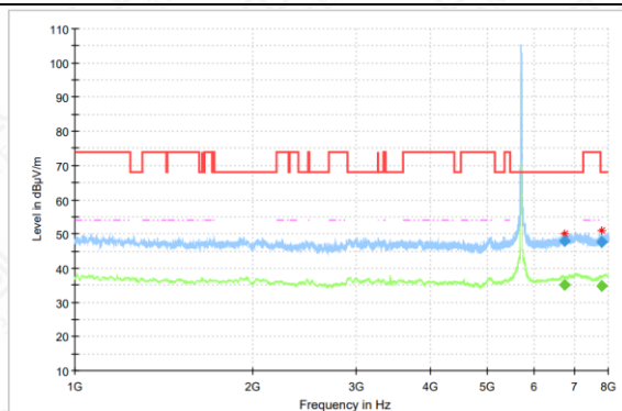
Radiated Spurious Emission (802.11n 20M, ch140, 1 GHz-8 GHz)
