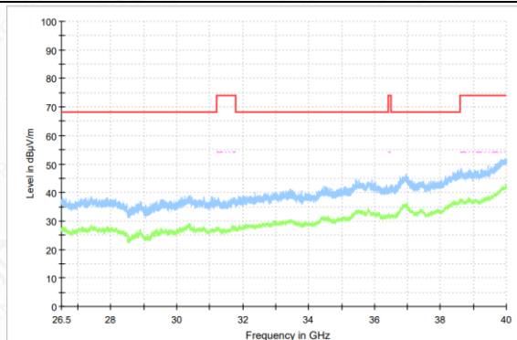
Radiated Spurious Emission (802.11n 20M, ch52, 26.5 GHz-40 GHz)
