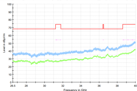
Radiated Spurious Emission (802.11a, ch140, 26.5 GHz-40 GHz)
