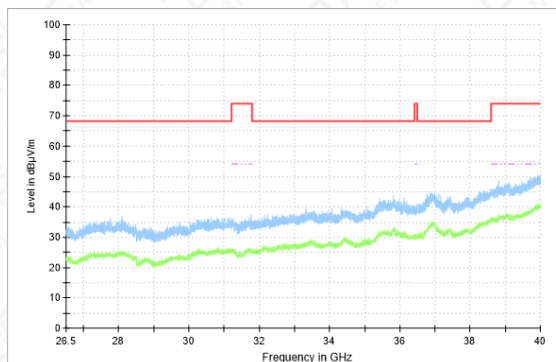
Radiated Spurious Emission (802.11a ch52, 26.5GHz-40GHz)
