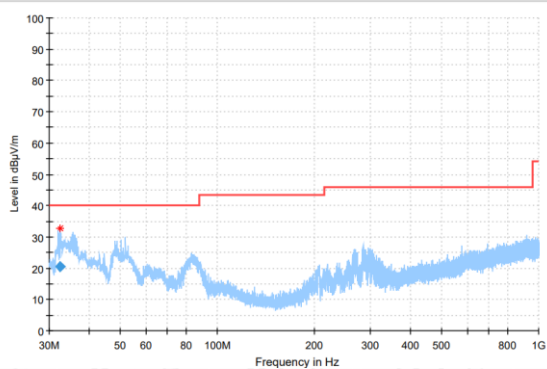
Radiated Spurious Emission (802.11a, ch140, 30MHz-1GHz)
