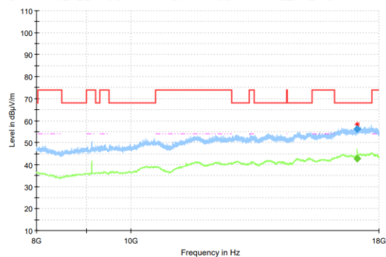
Radiated Spurious Emission (802.11a, ch140, 8GHz-18GHz)
