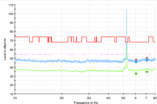
Radiated Spurious Emission (802.11n 20m, ch48, 1 GHz-8 GHz)
