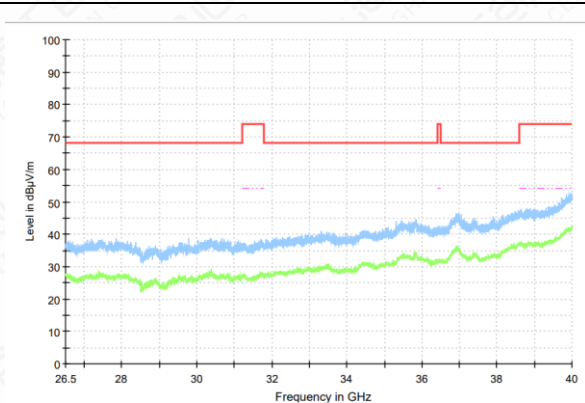
Radiated Spurious Emission (802.11n 20M, ch140, 26.5 GHz-40 GHz)
