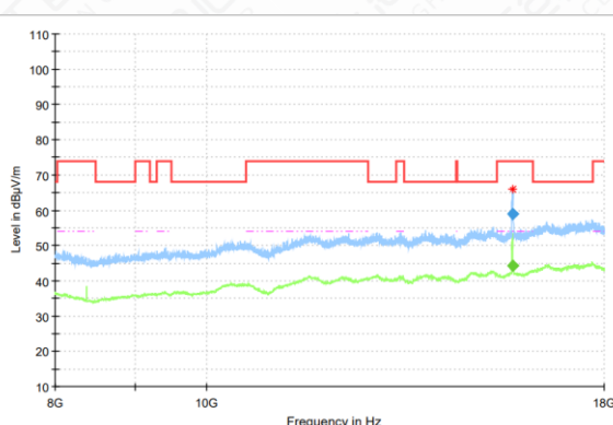
Radiated Spurious Emission (802.11n 20m, ch48, 8GHz-18GHz)
