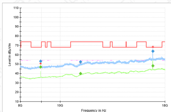
Radiated Spurious Emission (802.11a, ch52, 8GHz-18GHz)
