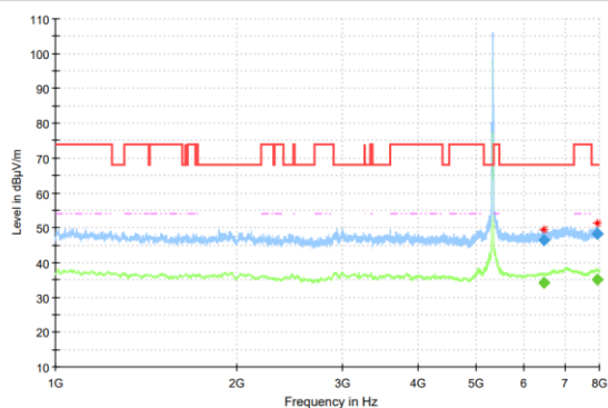
Radiated Spurious Emission (802.11a, ch64, 1 GHz-8 GHz)
