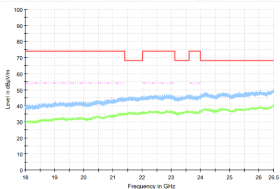
Radiated Spurious Emission (802.11a, ch64, 18GHz-26.5GHz)
