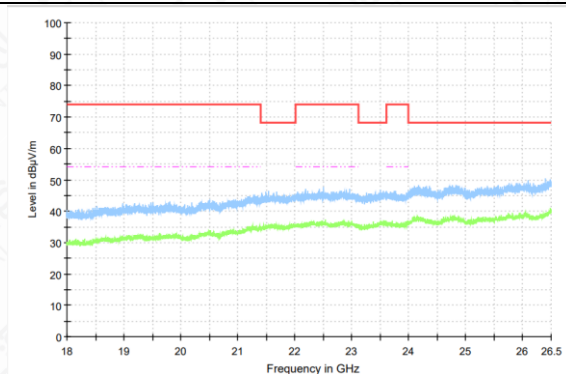
Radiated Spurious Emission (802.11n 20M, ch140, 18GHz-26.5GHz)
