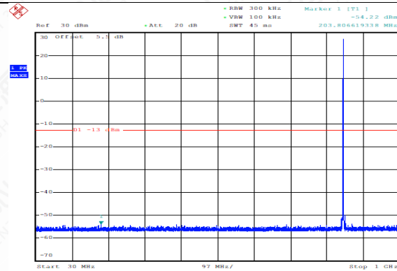
GSM850_EDGE_251_30MHz-1000MHz_CSE
