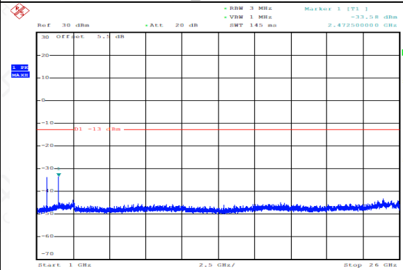
GSM850_EDGE_128_1000MHz-26000MHz_CSE
