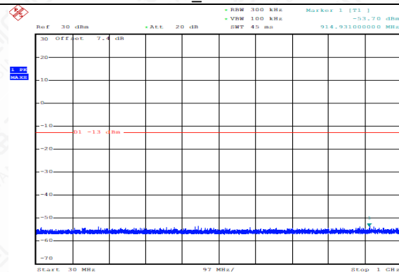
GSM1900_EDGE_661_30MHz-1000MHz _CSE
