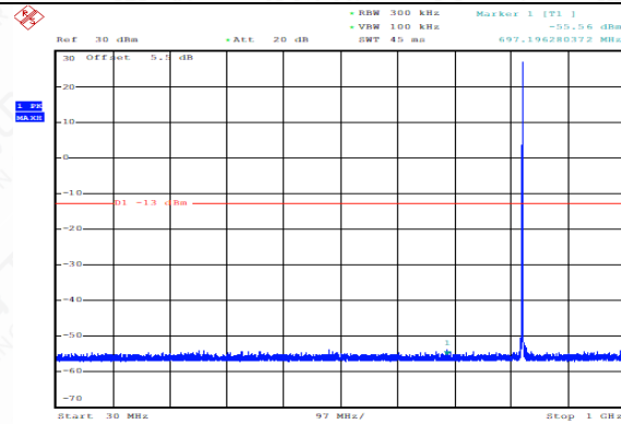
GSM850_EDGE_128_30MHz-1000MHz_CSE
